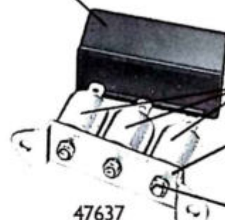
Nut 165033 Washer 185006
