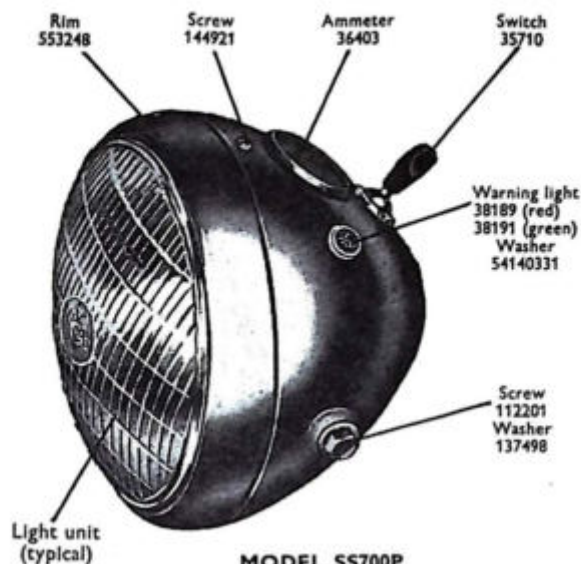
MODEL SS700P
