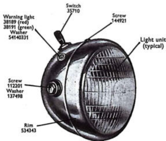
MODEL MCH66
