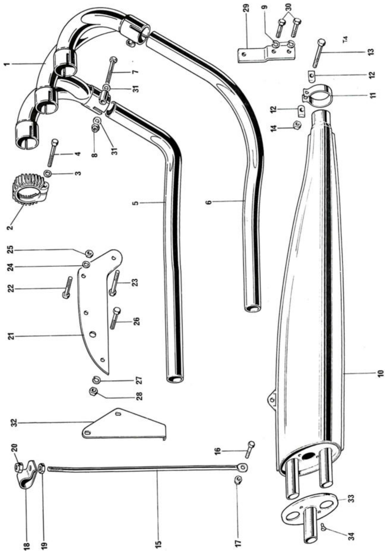
Fig. 17. EXHAUST PIPES AND SILENCERS
