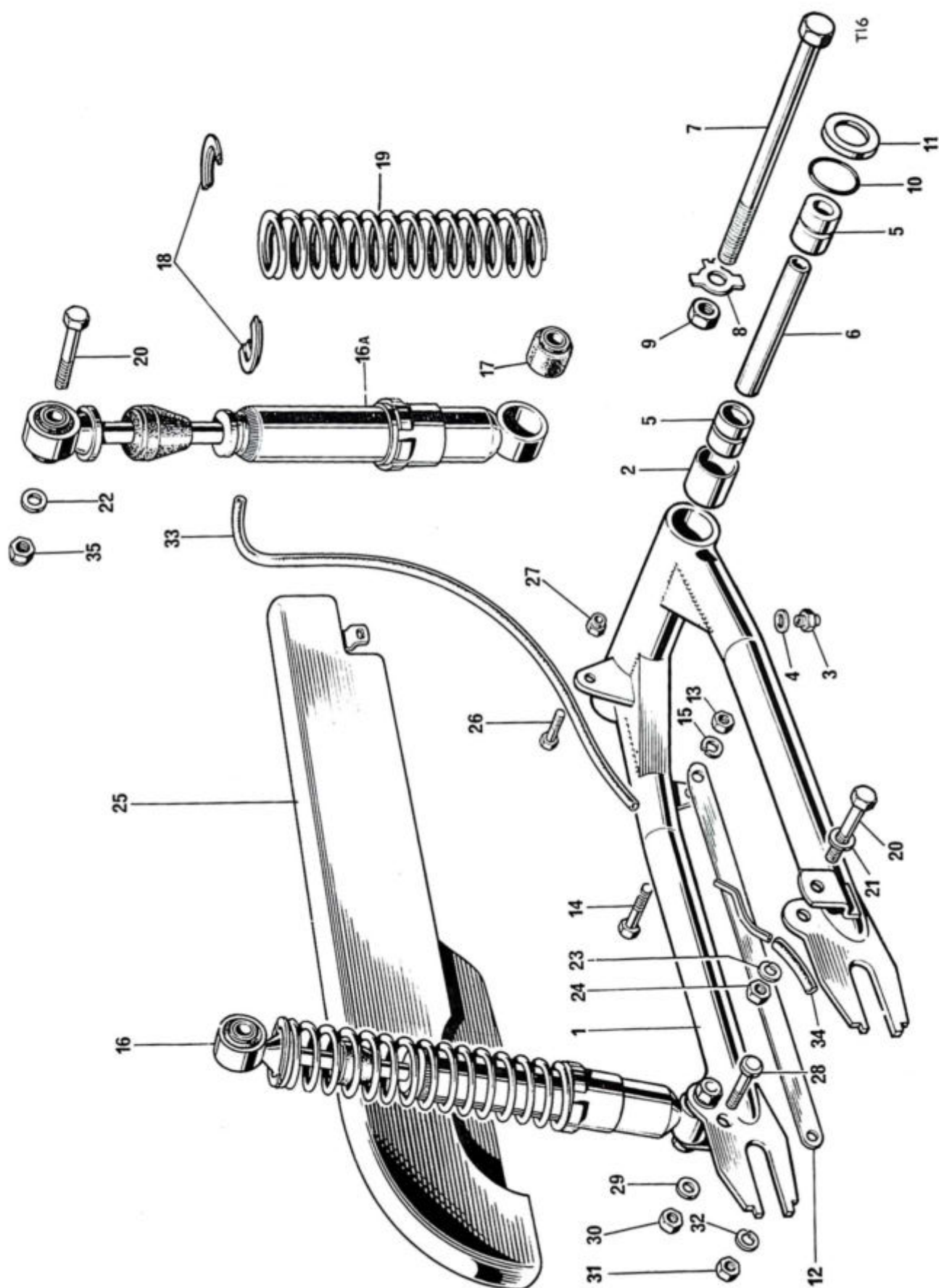
Fig. 15. SWINGING FORK AND SUSPENSION UNITS
