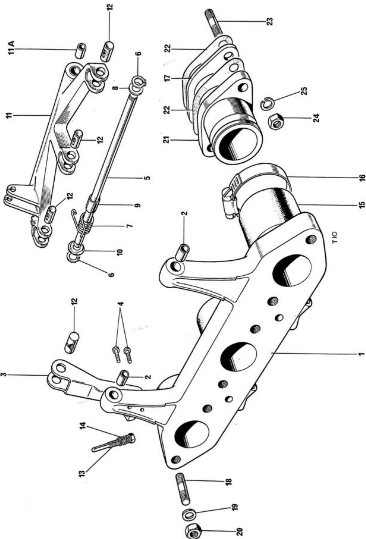
Fig. 7. MANIFOLD AND THROTTLE LINKAGE
