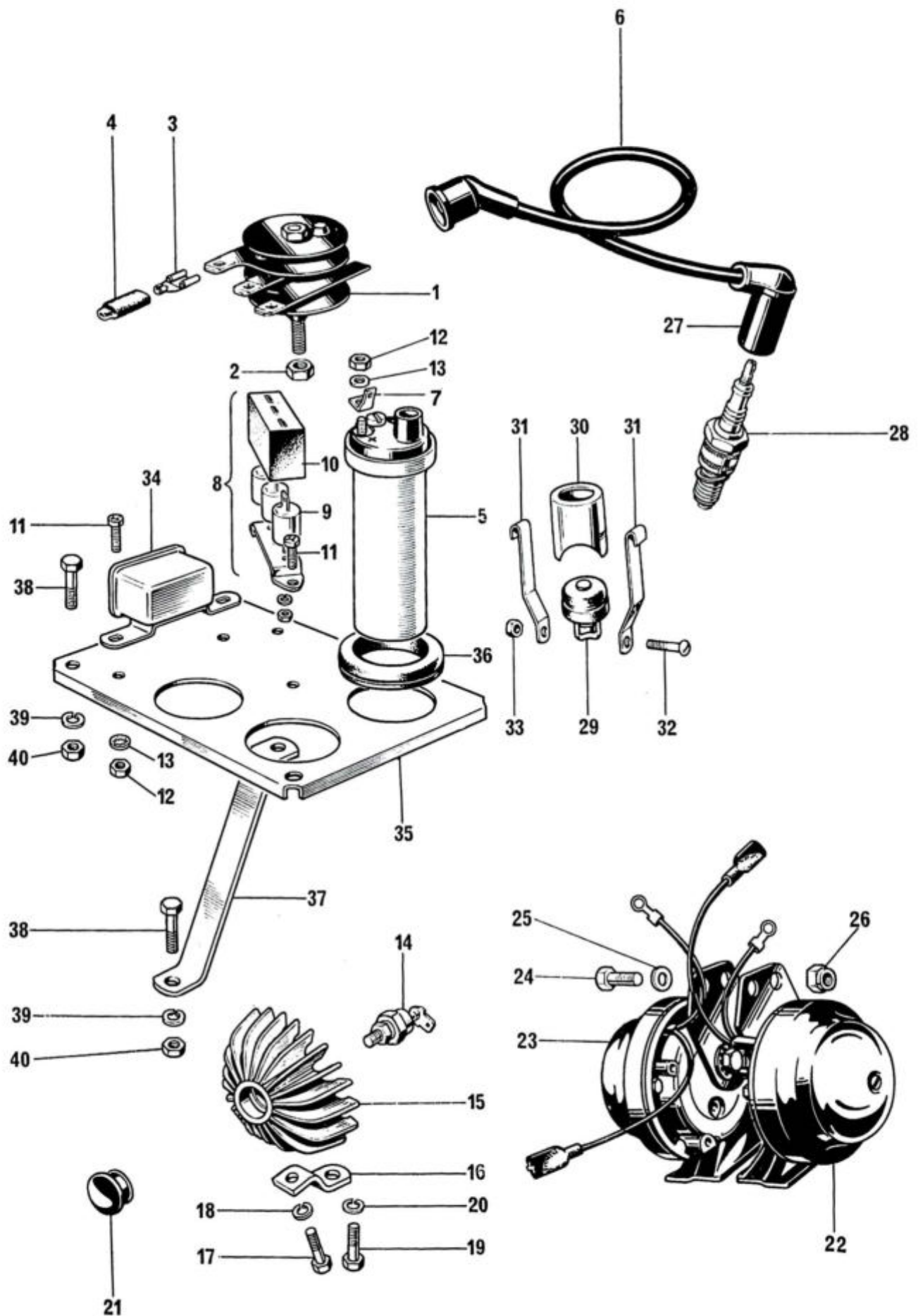
Fig. 34. IGNITION COILS, HORNS, RECTIFIER AND ZENER DIODE
