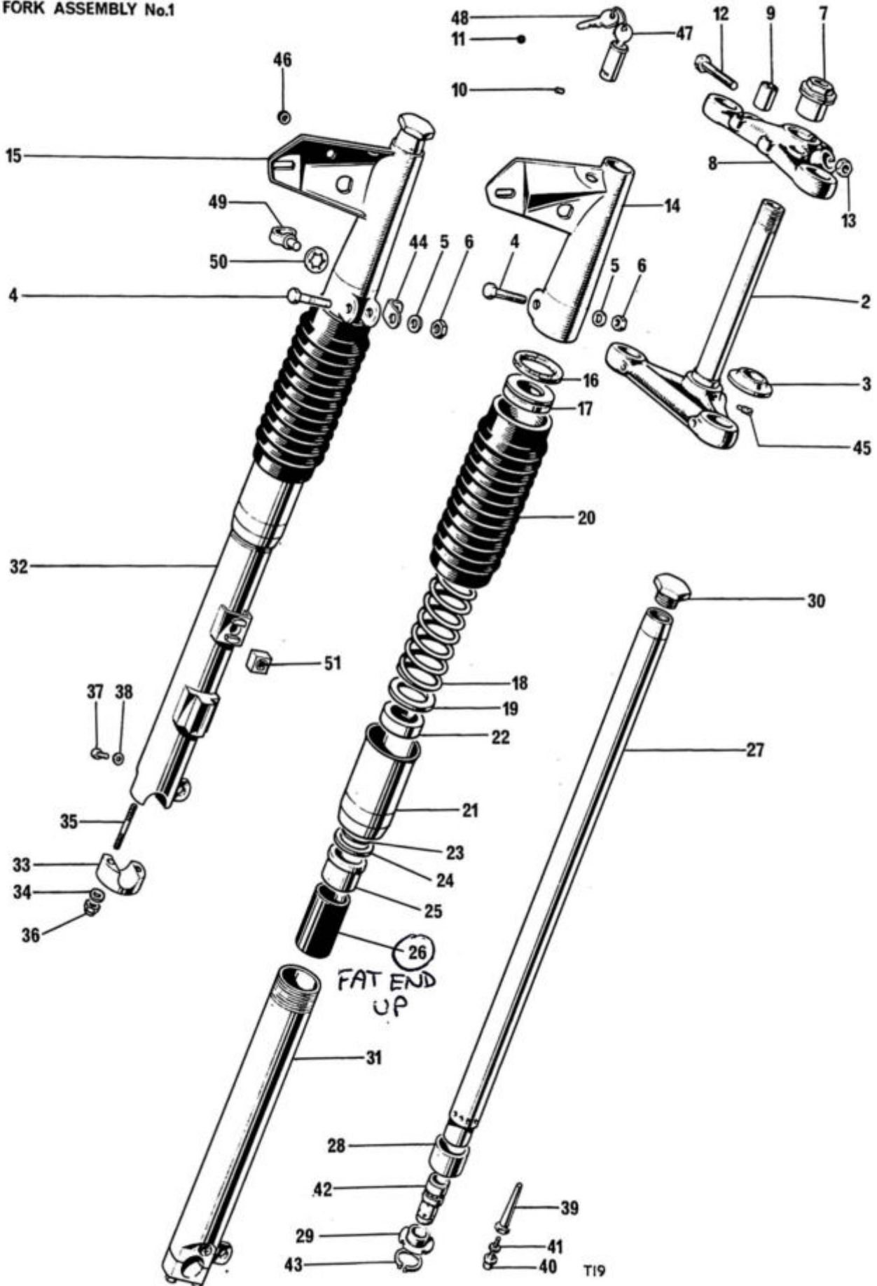
Fig. 18. TELESCOPIC FRONT FORK
