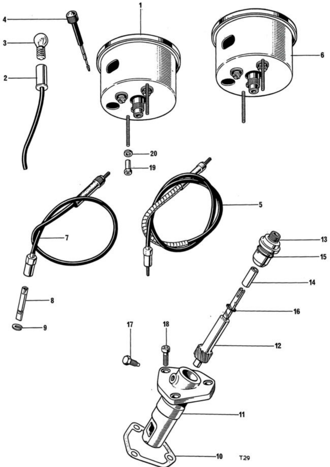
Fig. 33. SPEEDOMETER AND TACHOMETER
