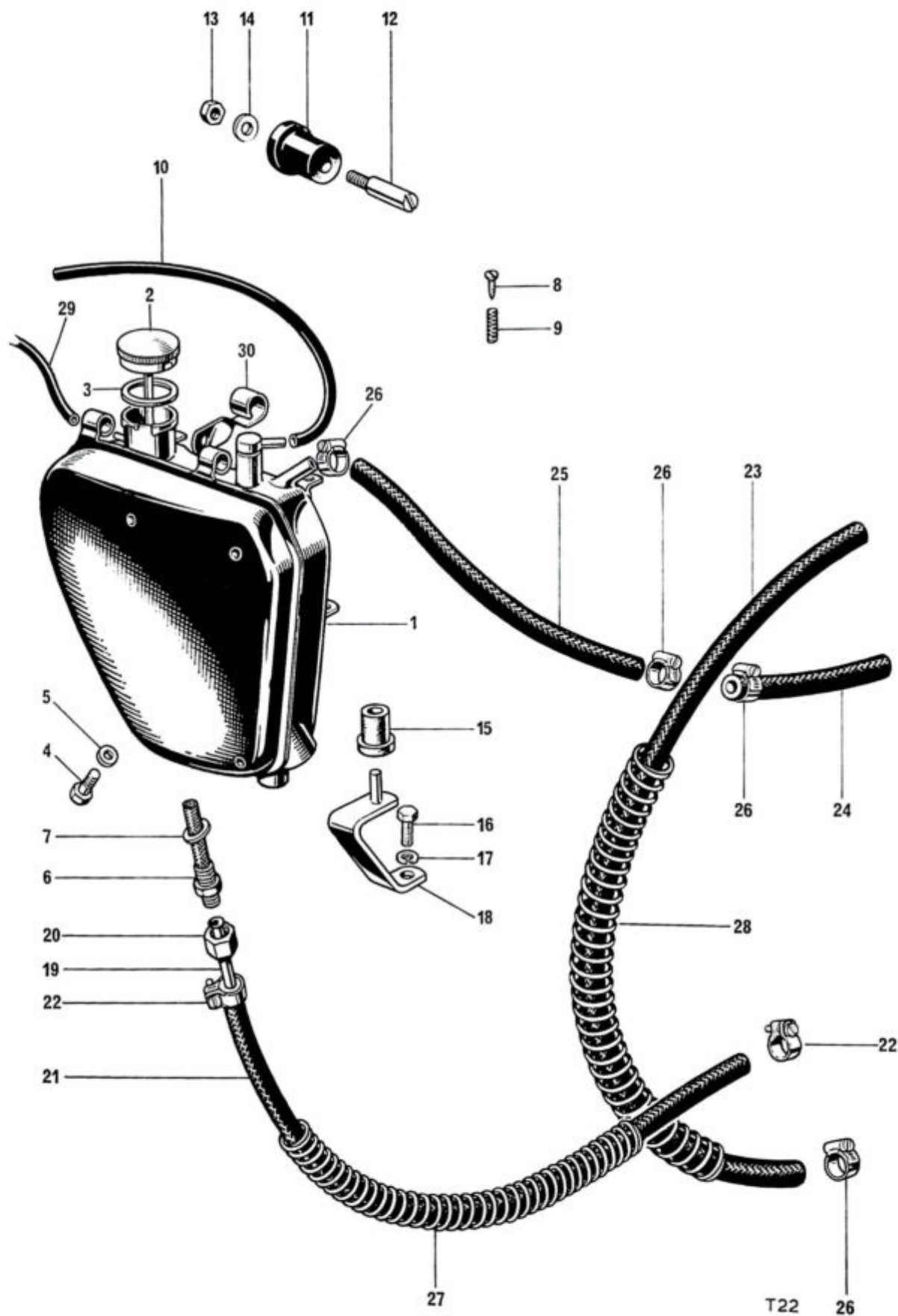
Fig. 24. OIL TANK
