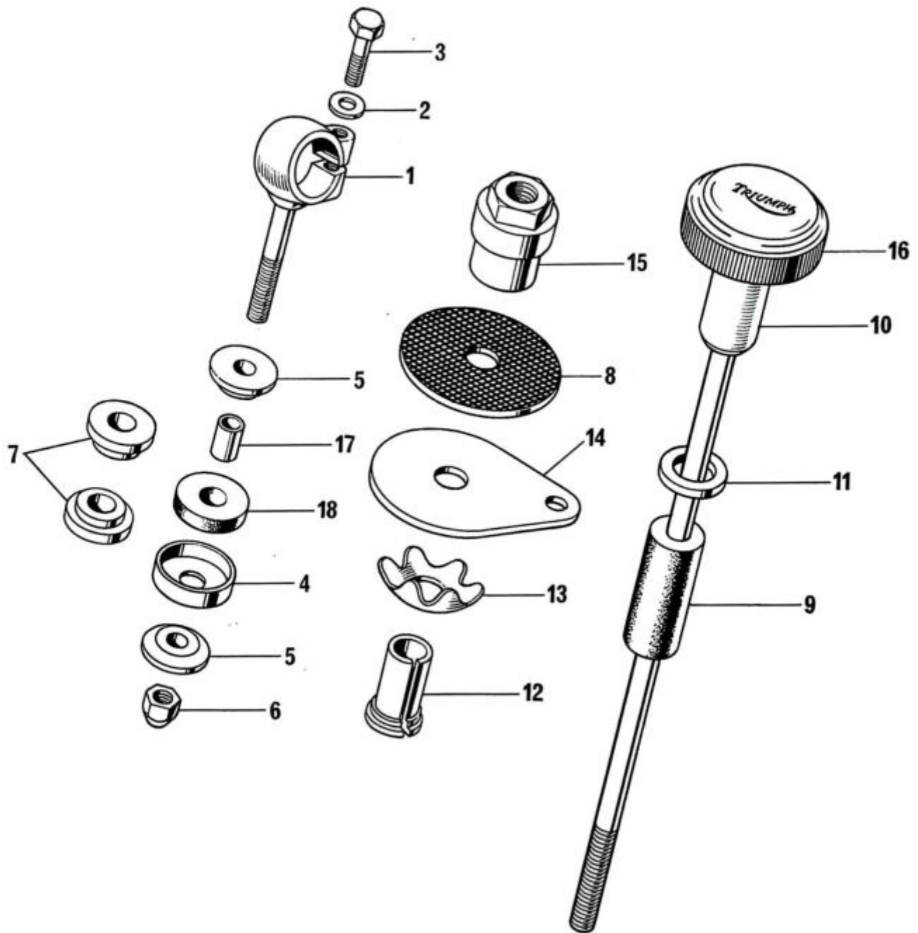
Fig. 19. HANDLEBAR MOUNTINGS AND STEERING DAMPER
