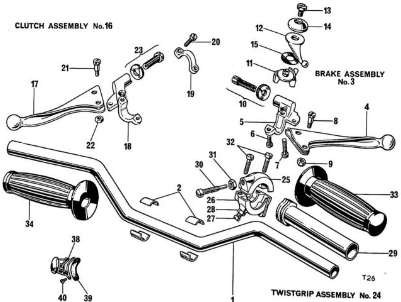
Fig. 29. HANDLEBARS, CONTROLS, BINNACLE AND OIL WARNING LIGHT
