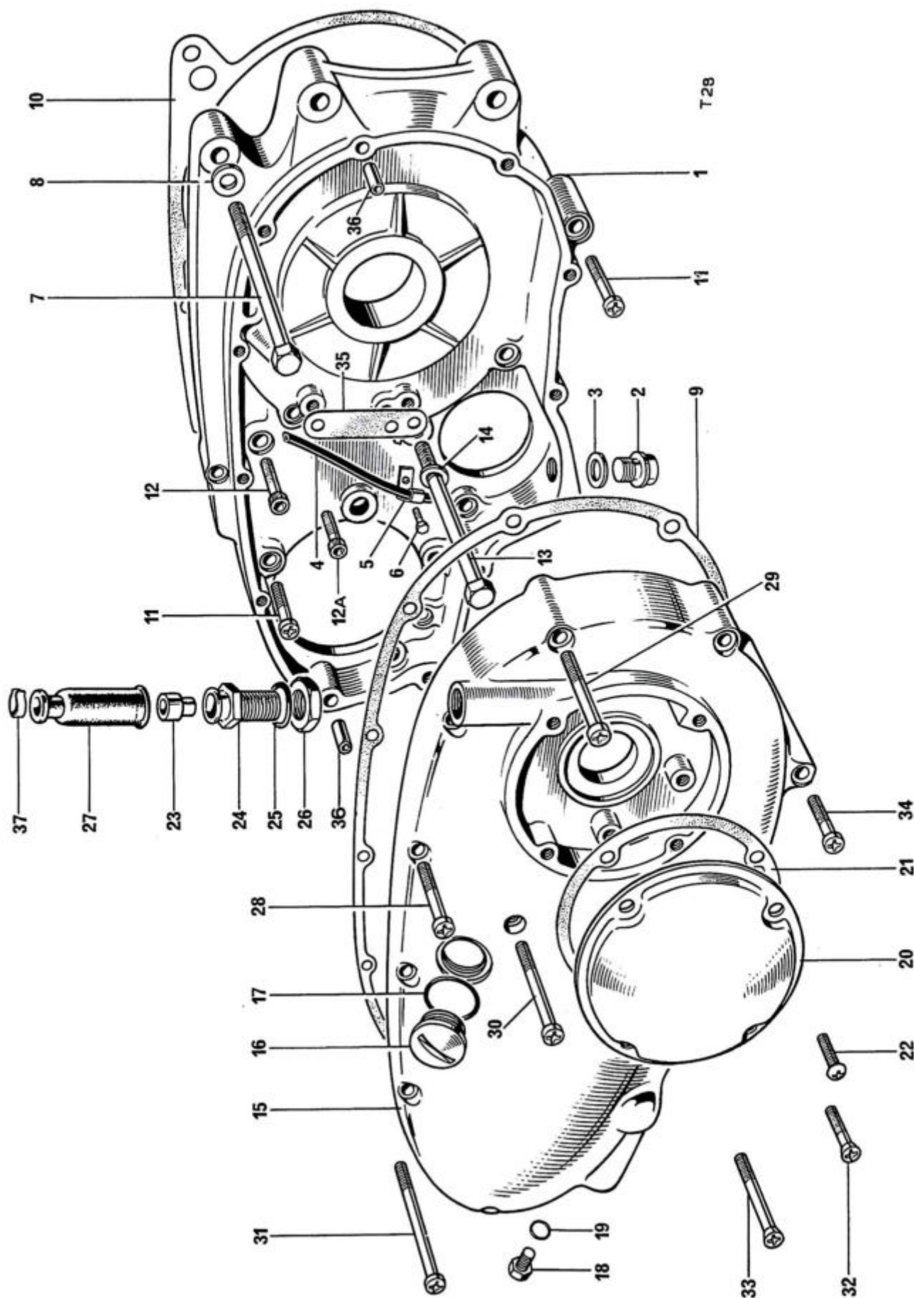
Fig. 12. INNER AND OUTER CHAINCASE
