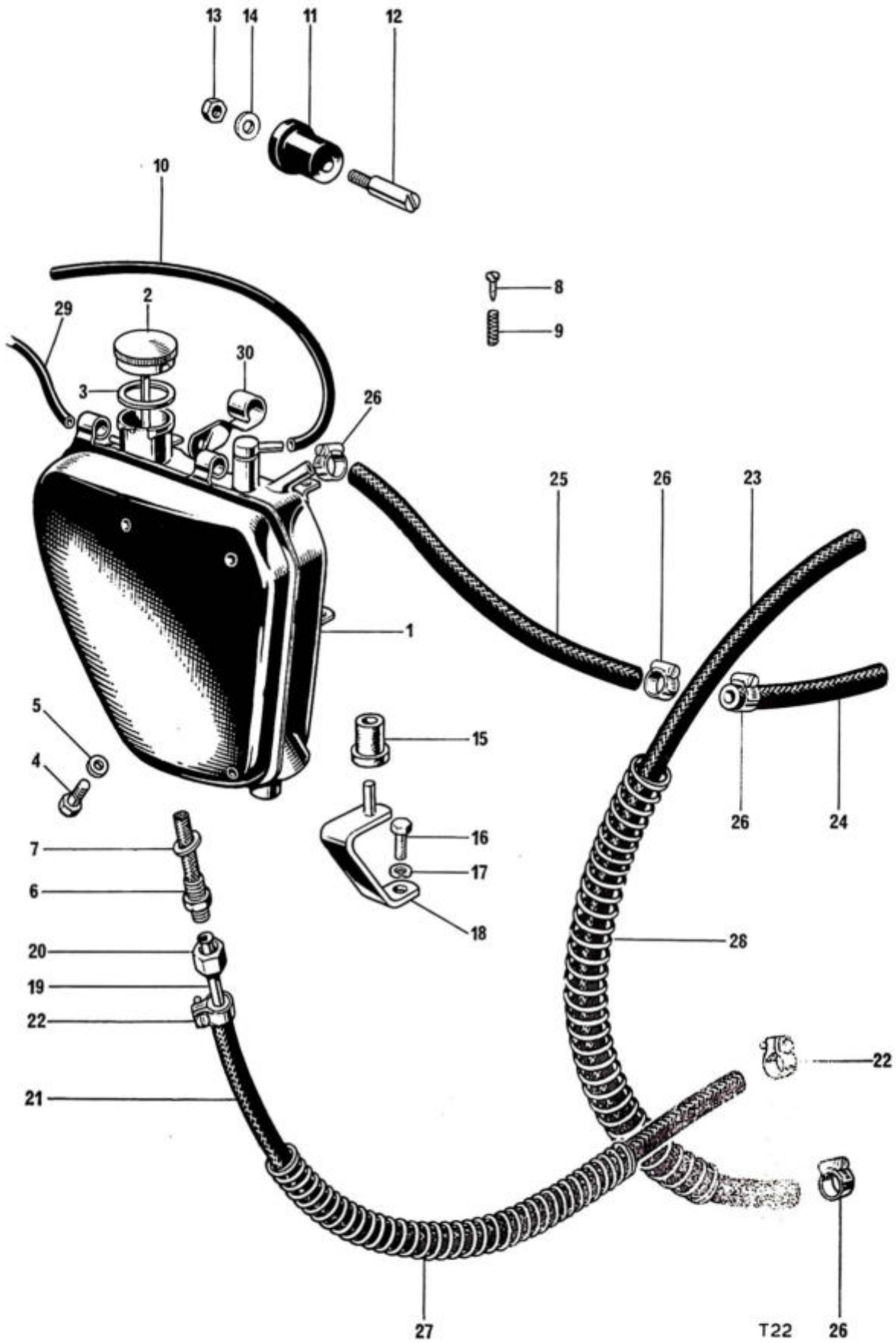
Fig. 26. OIL TANK
