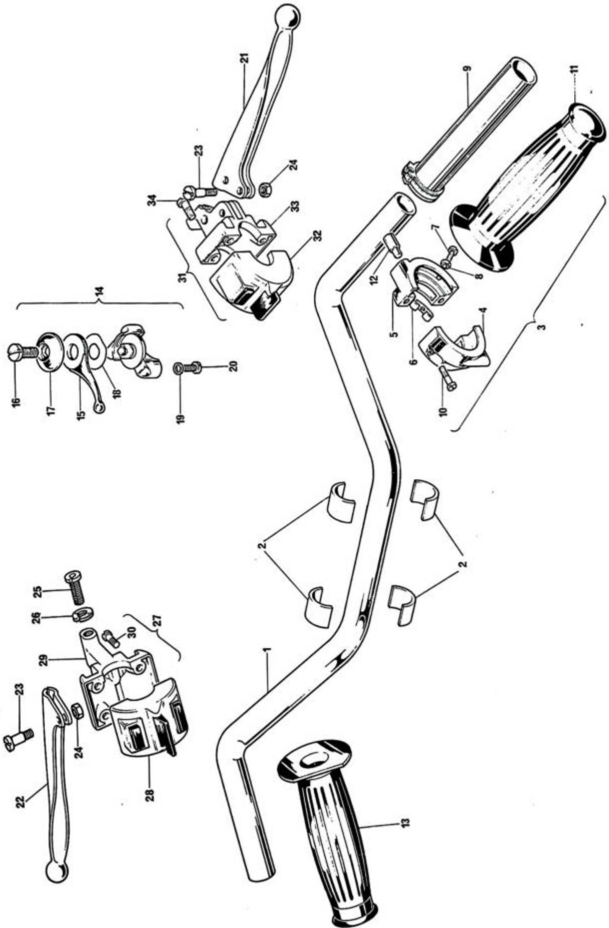
FIG. 30. HANDLEBAR AND CONTROL LEVERS
