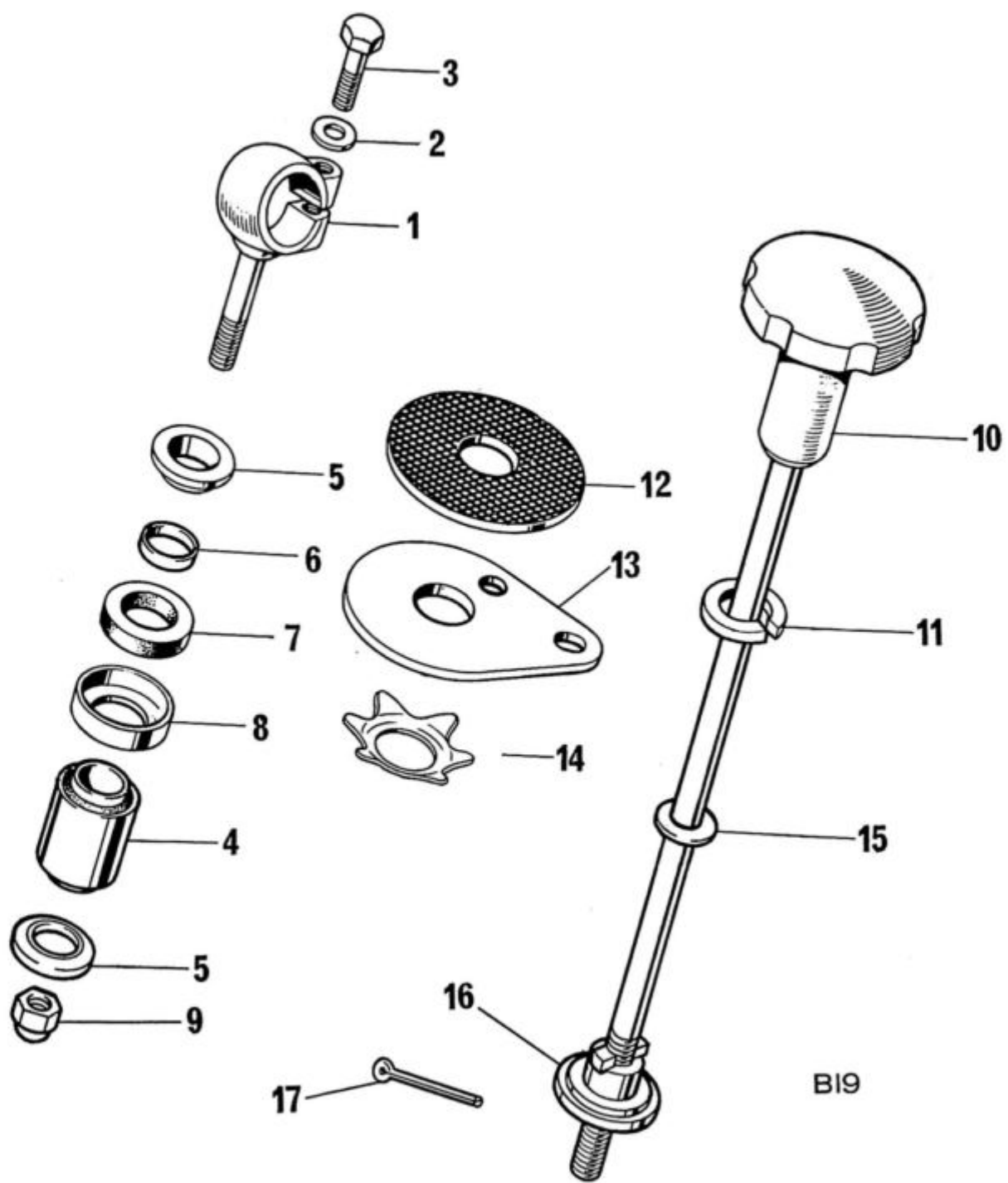
Fig. 21. HANDLEBAR MOUNTINGS AND STEERING DAMPER
