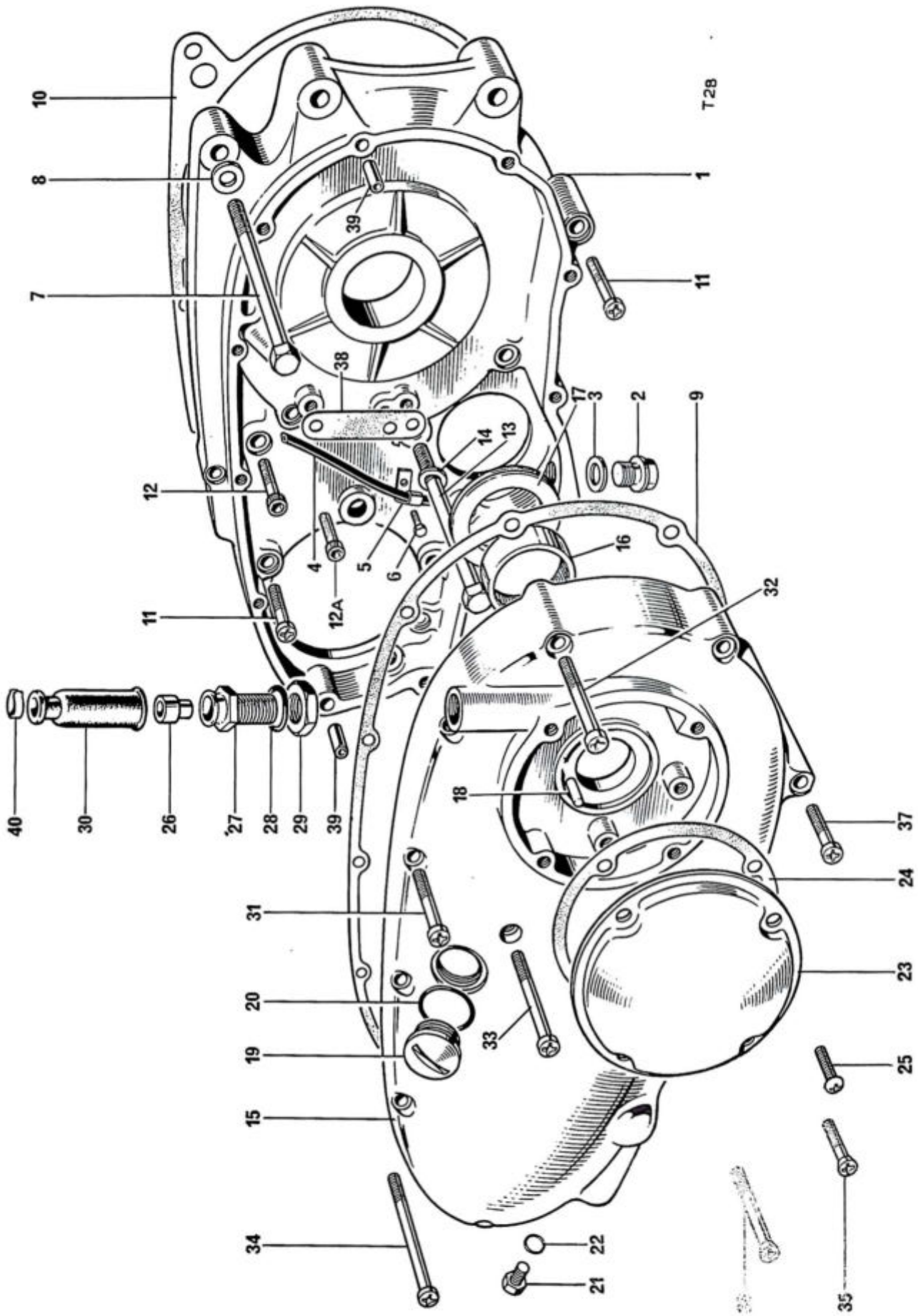
FIG. 14. INNER AND OUTER CHAINCASE
