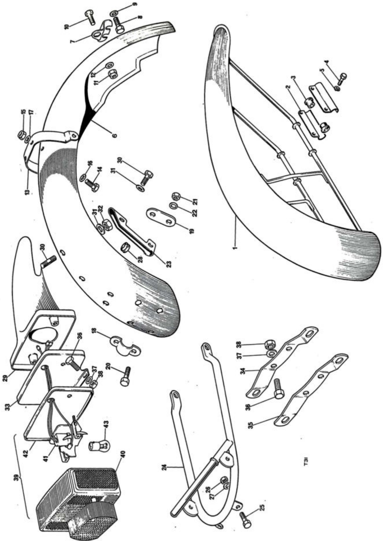
Fig. 29. FENDERS AND TAIL LAMP
