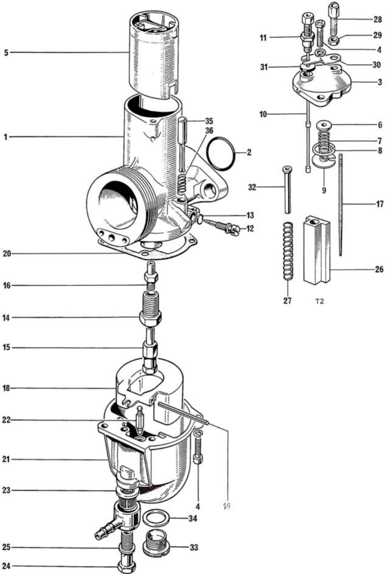
Fig. 5. CARBURETORS
