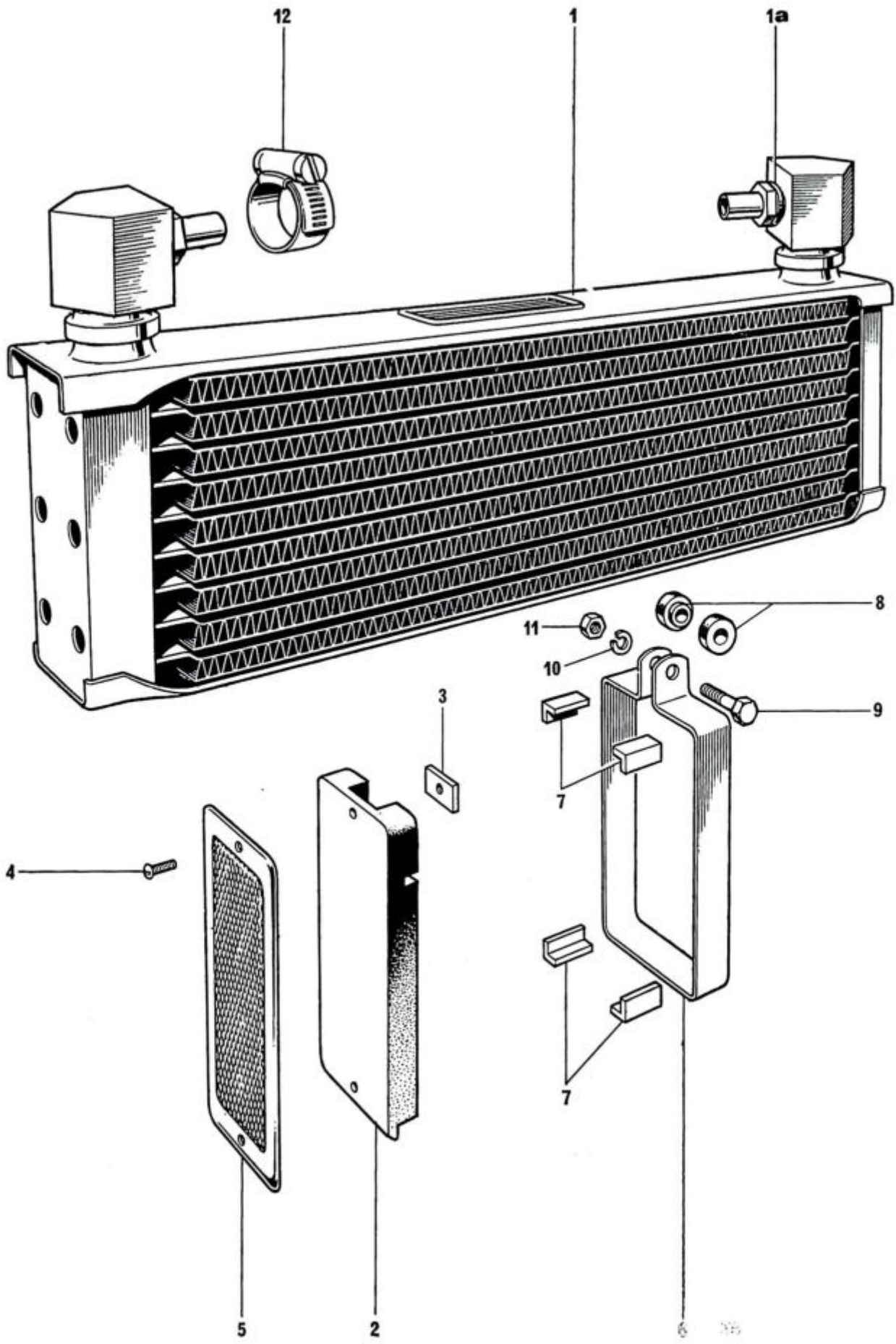
Fig. 24. OIL COOLER
