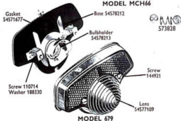
MODEL 679
