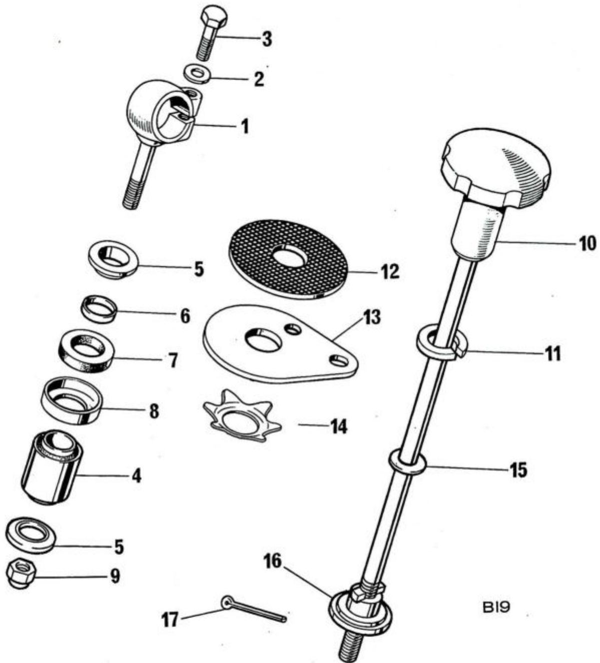
Fig. 21. HANDLEBAR MOUNTINGS AND STEERING DAMPER
