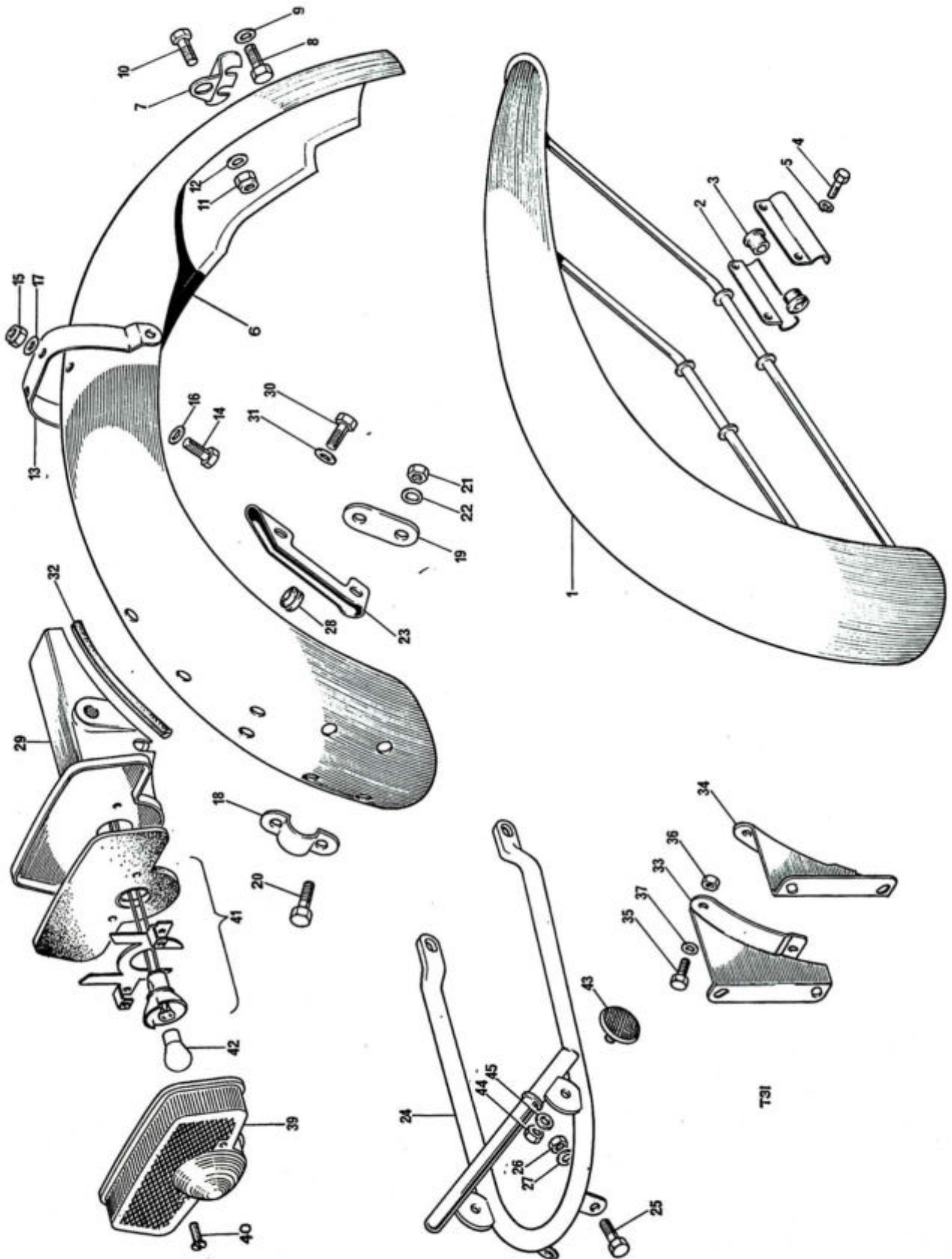
Fig. 29. FENDERS AND TAIL LAMP
