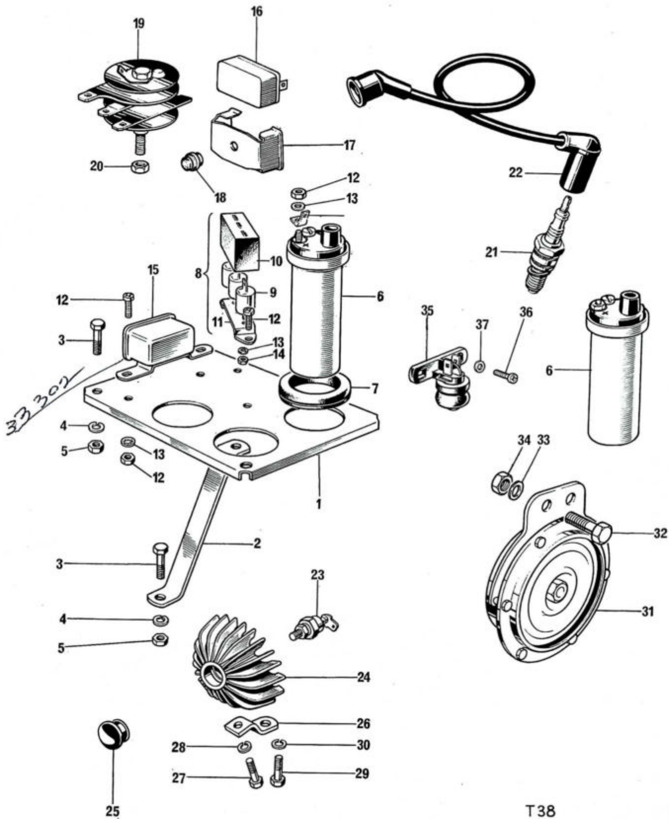
Fig. 34. IGNITION COILS, HORNS, RECTIFIER AND ZENER DIODE
