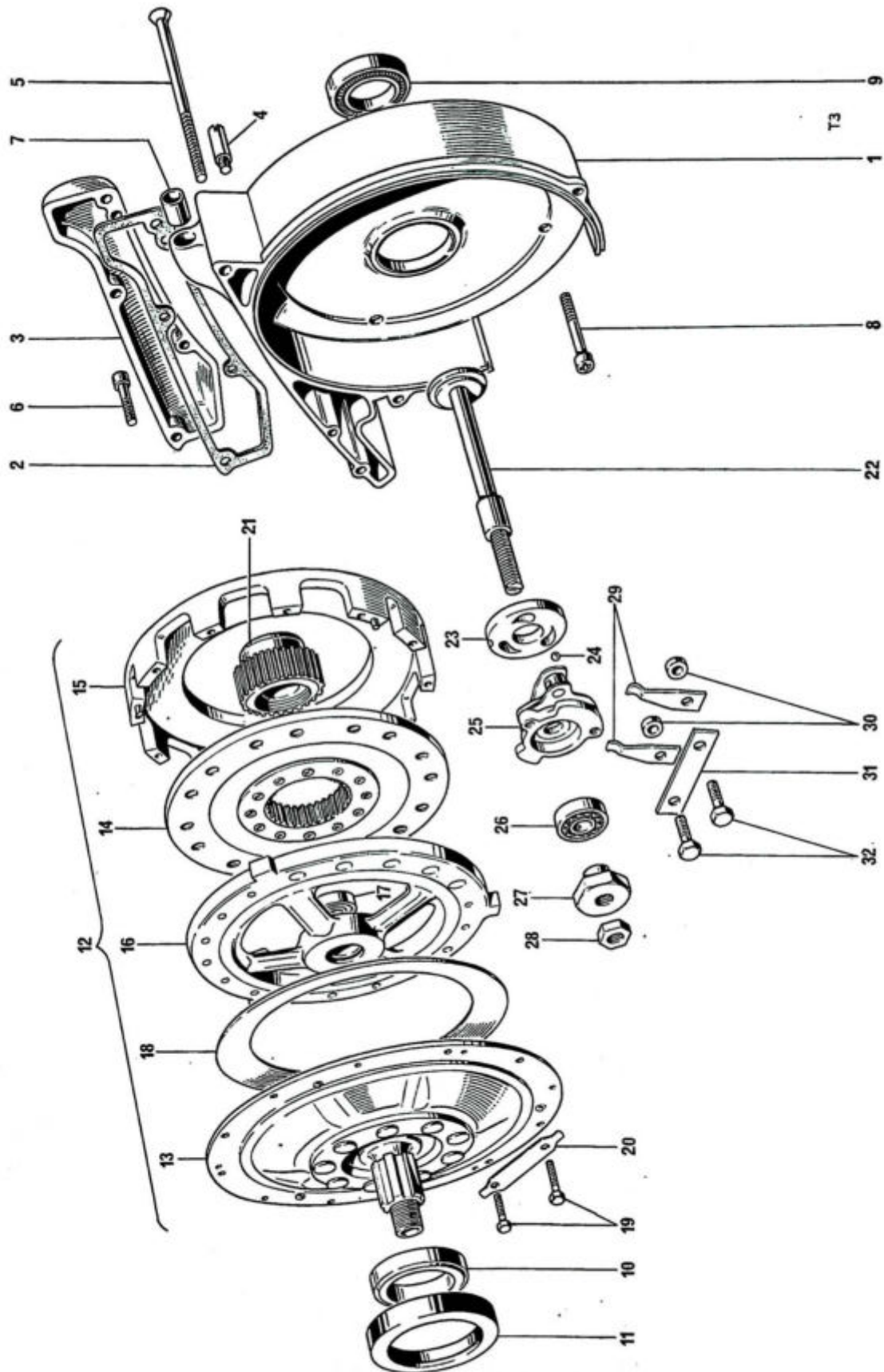
Fig. 13. CLUTCH AND CLUTCH OPERATING MECHANISM
