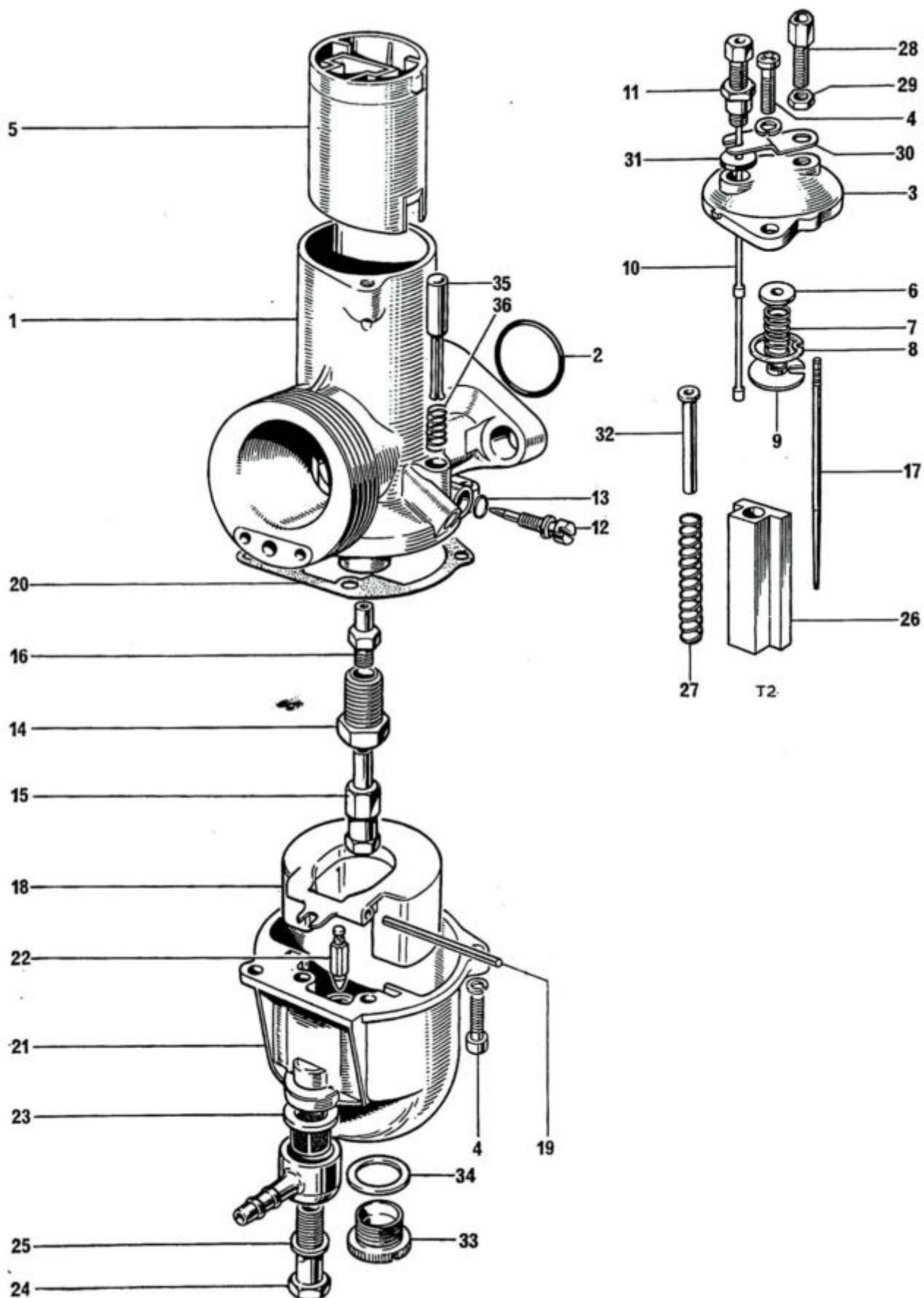
Fig. 5. CARBURETORS
