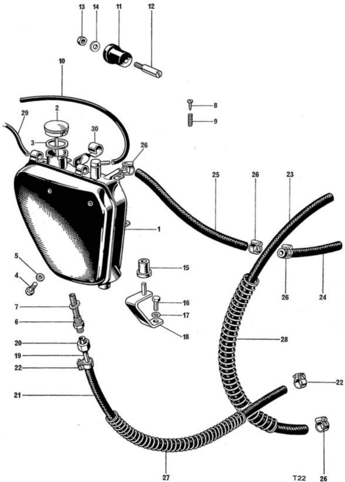
Fig. 26. OIL TANK
