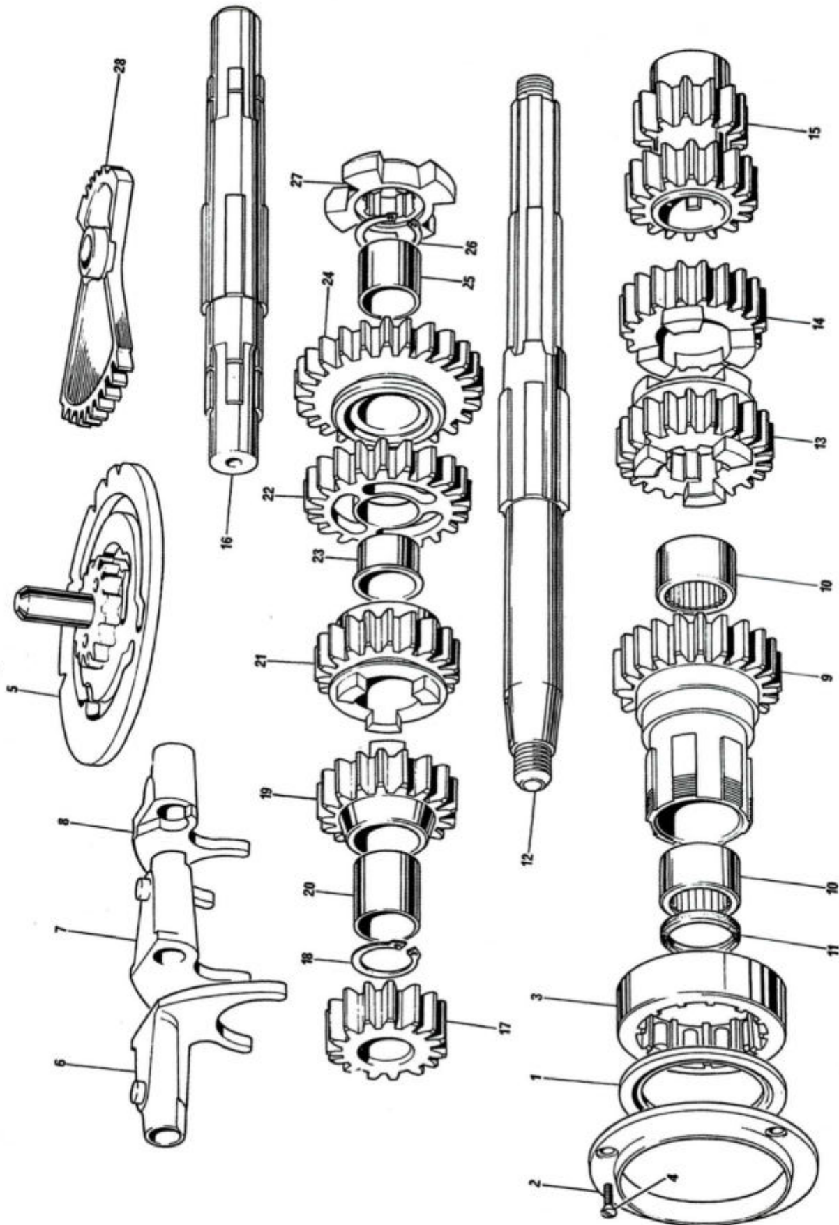
FIG. 12. PARTS REQUIRED FOR OPTIONAL 5 SPEED GEARBOX
