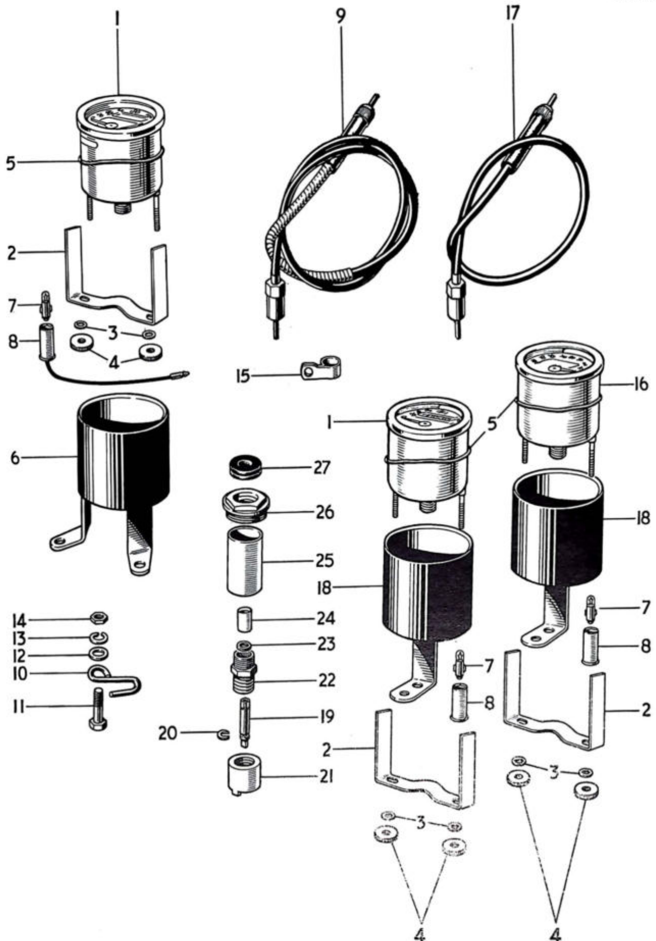
Fig. 26. SPEEDOMETER AND TACHOMETER EQUIPMENT
