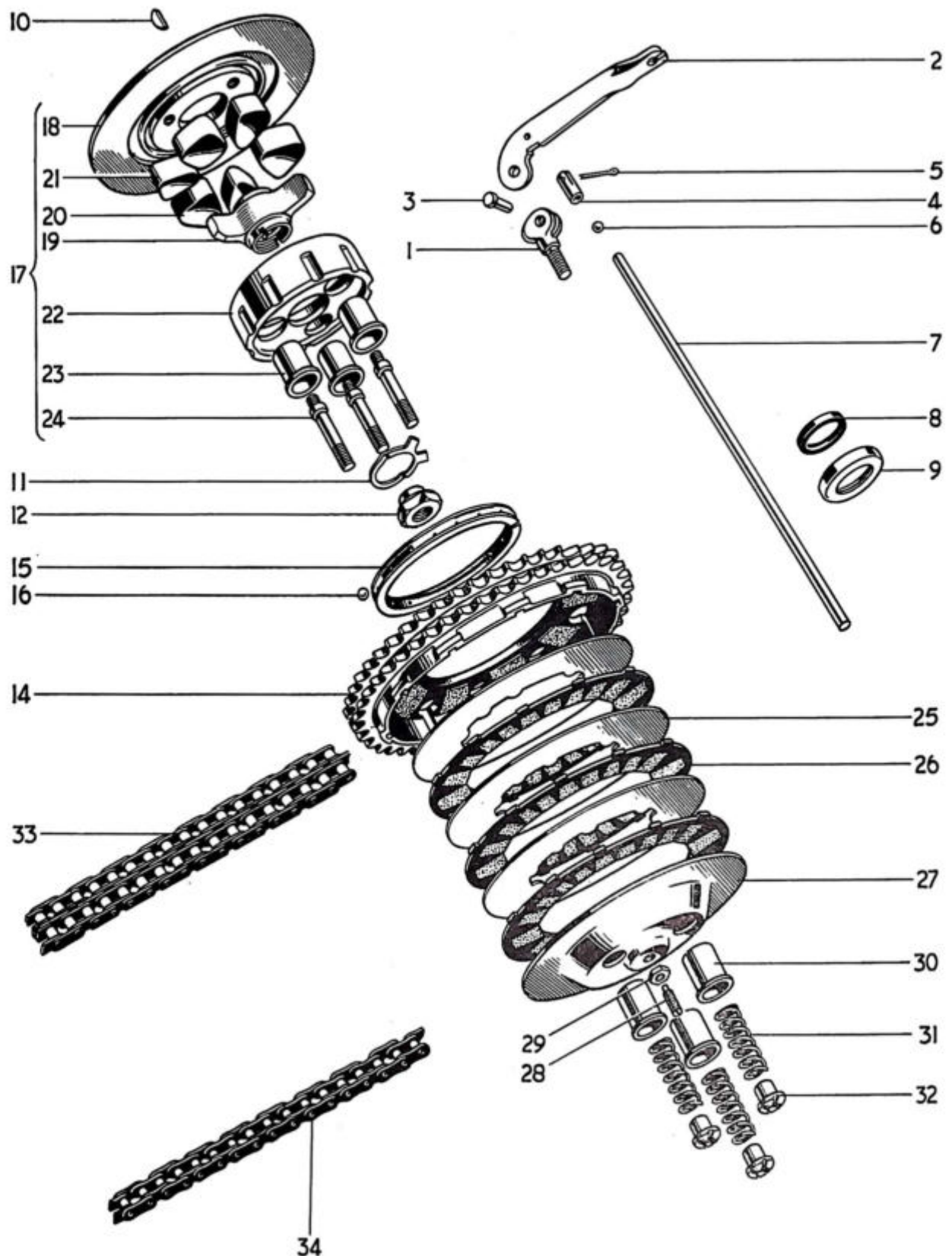
Fig. 6. CLUTCH AND CHAINS
