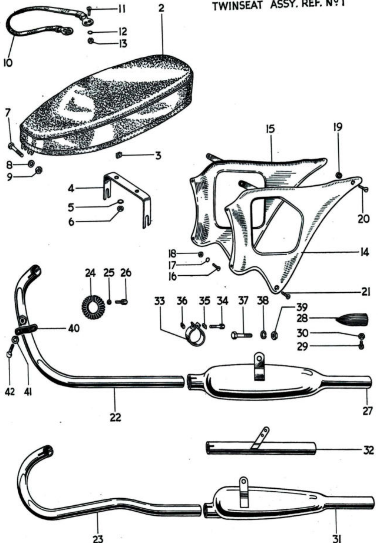
Fig. 15. TWINSEAT, REAR PANELS AND EXHAUST SYSTEM
