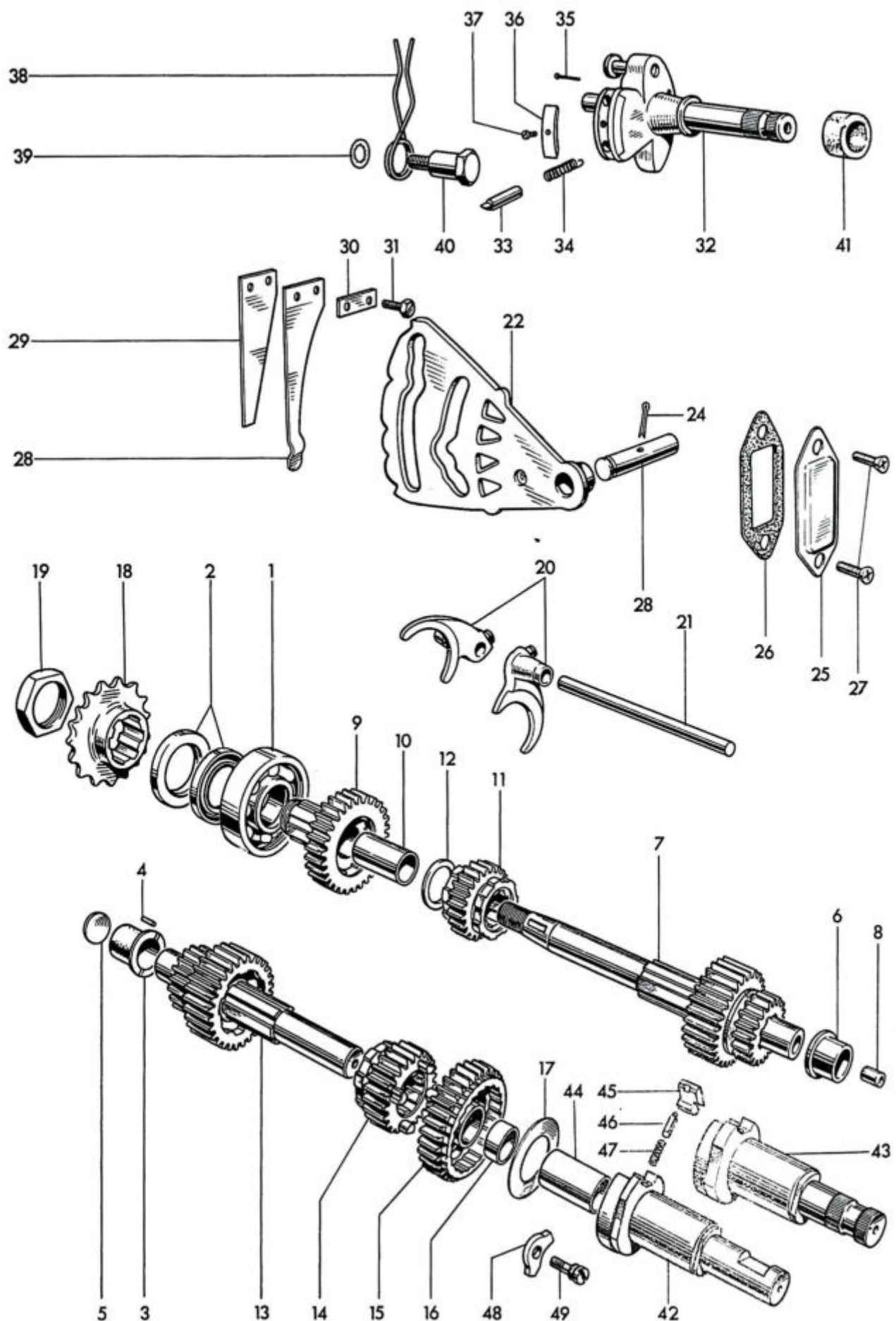
Fig. 5. GEARBOX SHAFTS AND GEARS
