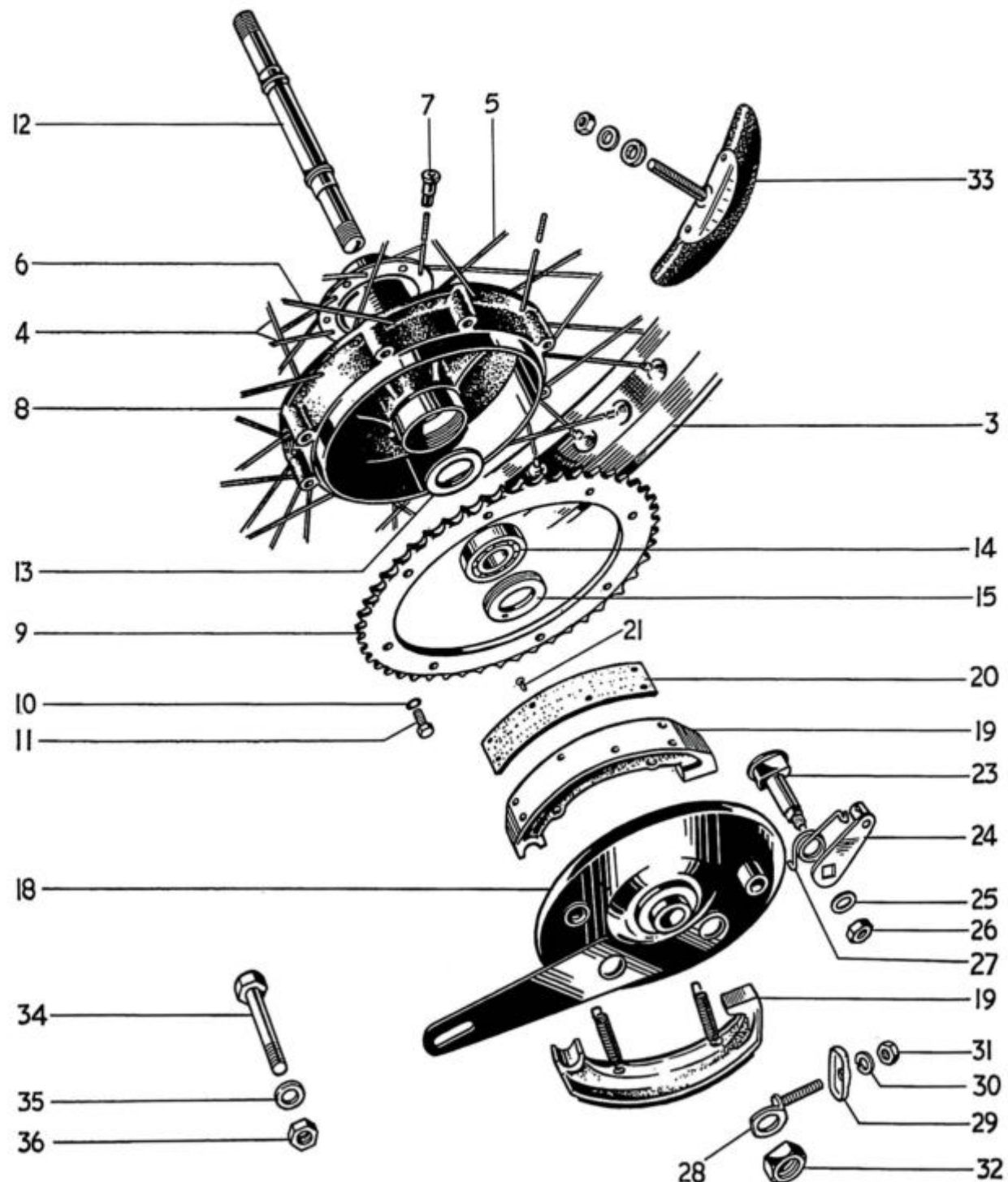
Fig. 13. REAR WHEEL
