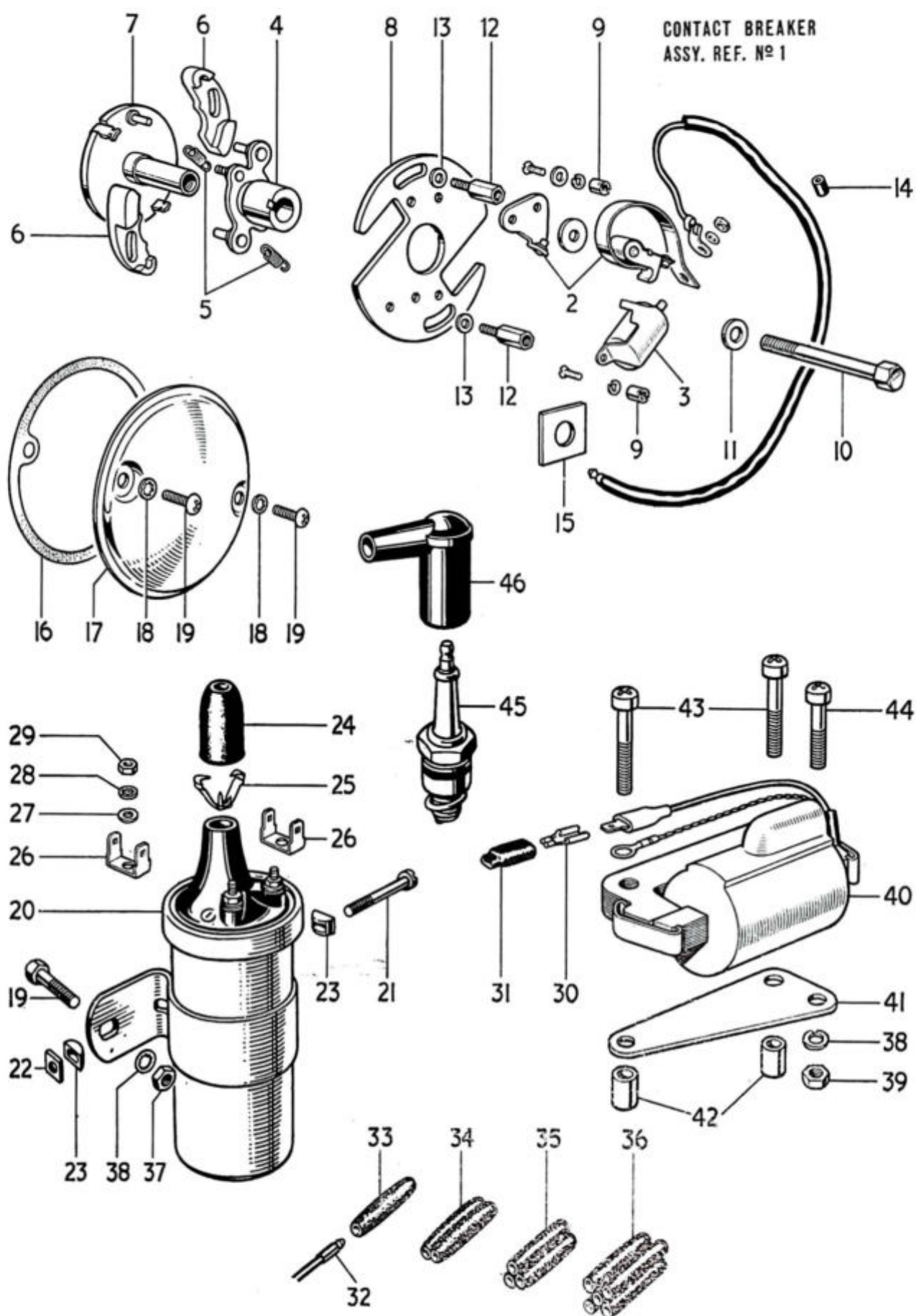
Fig. 24. CONTACT BREAKER AND IGNITION COILS
