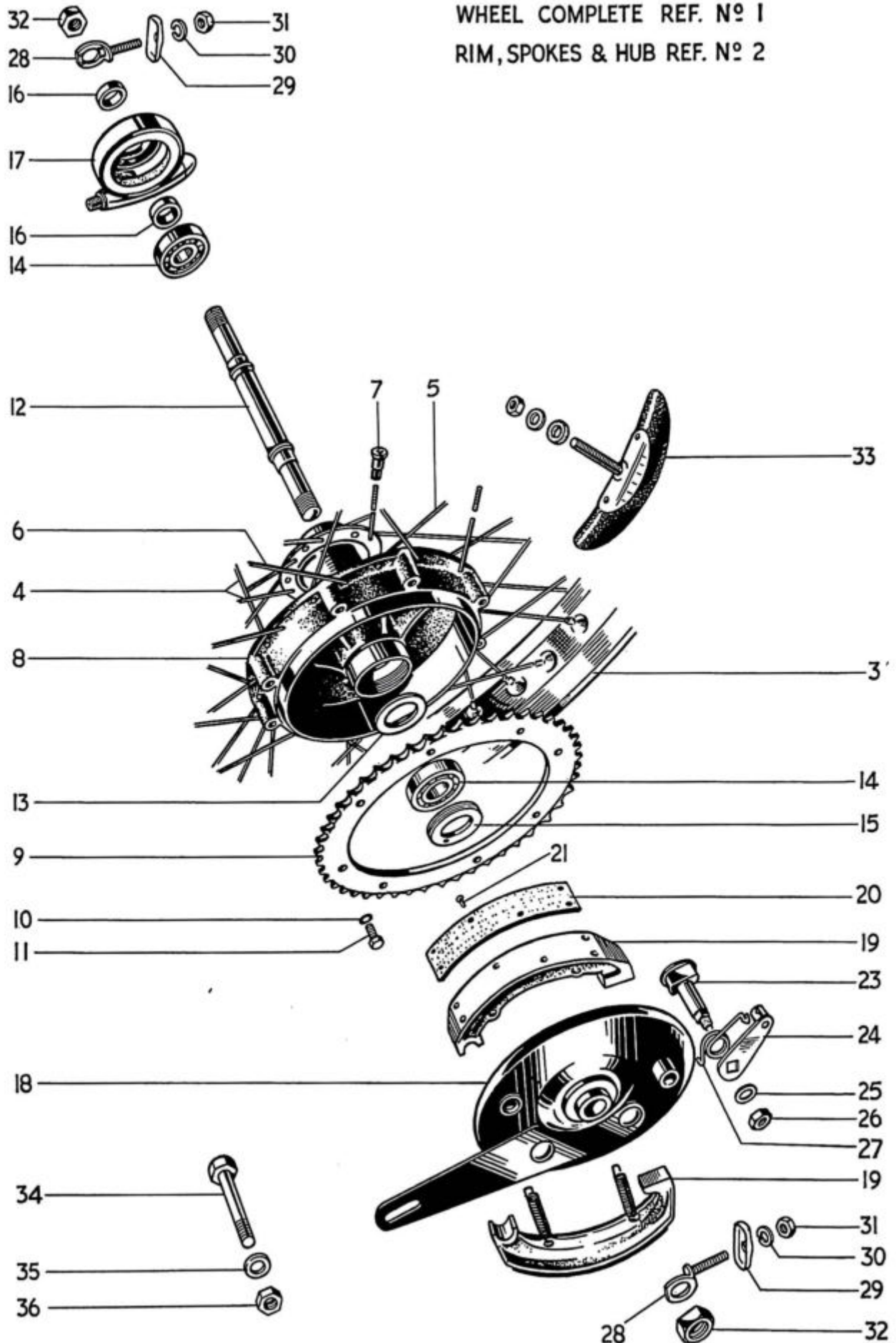
Fig. 13. REAR WHEEL
