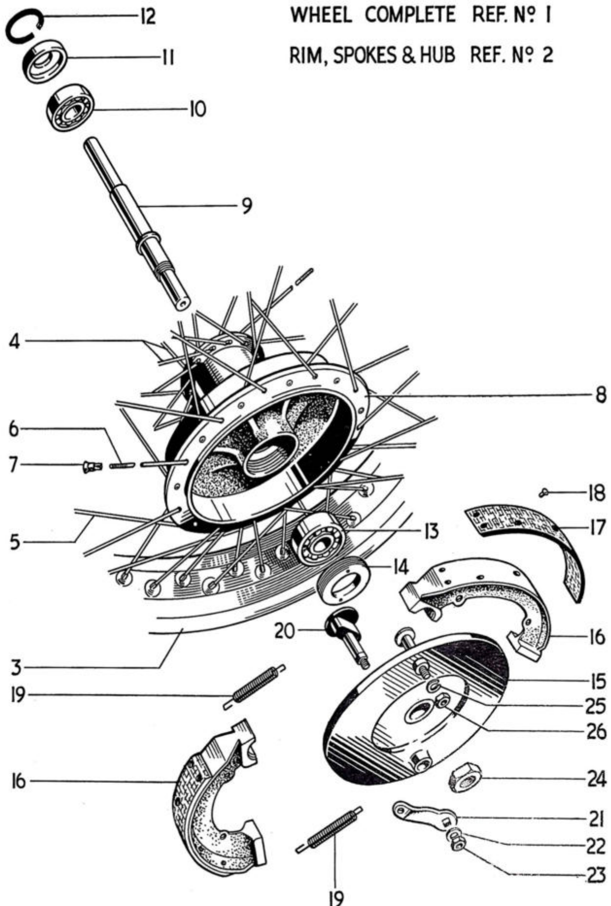
Fig. 11. FRONT WHEEL, T20.
