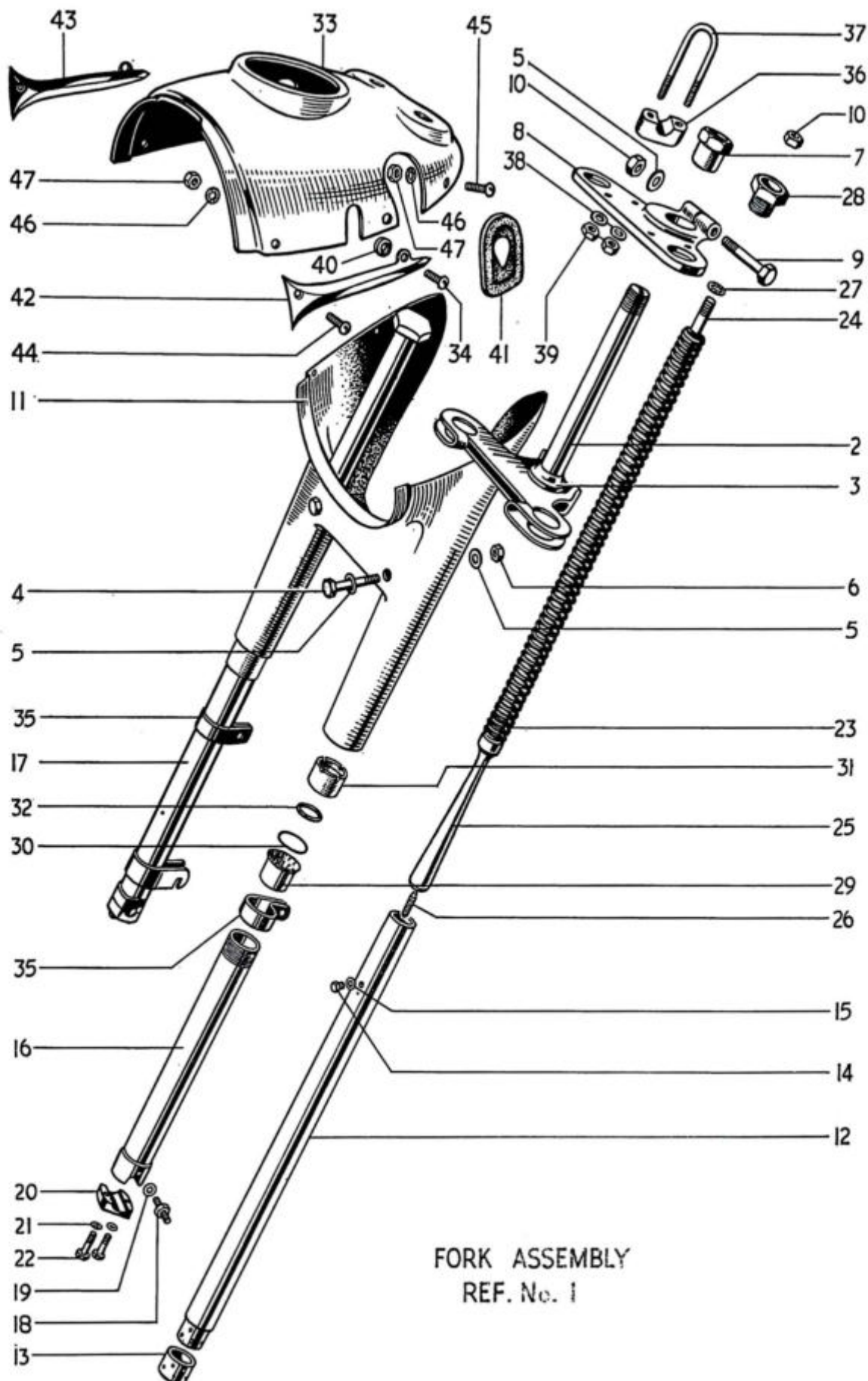
Fig. 9. TELESCOPIC FRONT FORK T20
