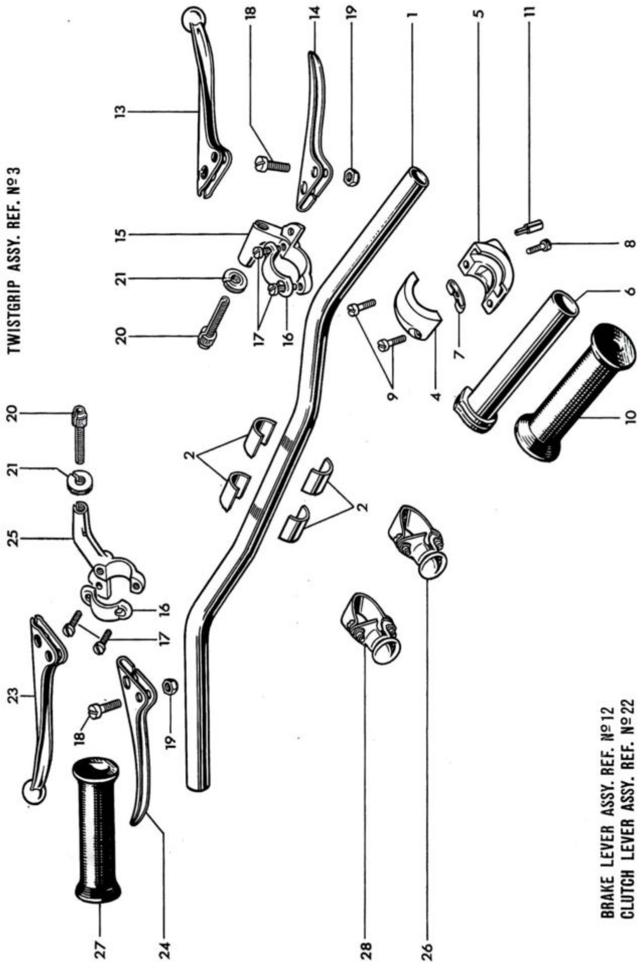
Fig. 19. HANDLEBARS AND CONTROL LEVERS. T20SS AND T20SH
