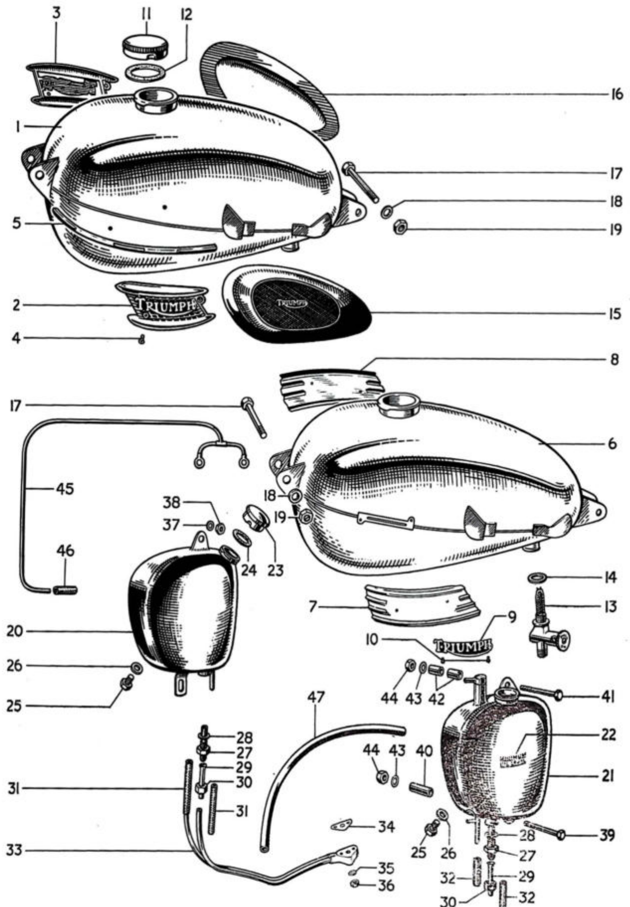
Fig. 16. PETROL AND OIL TANKS
