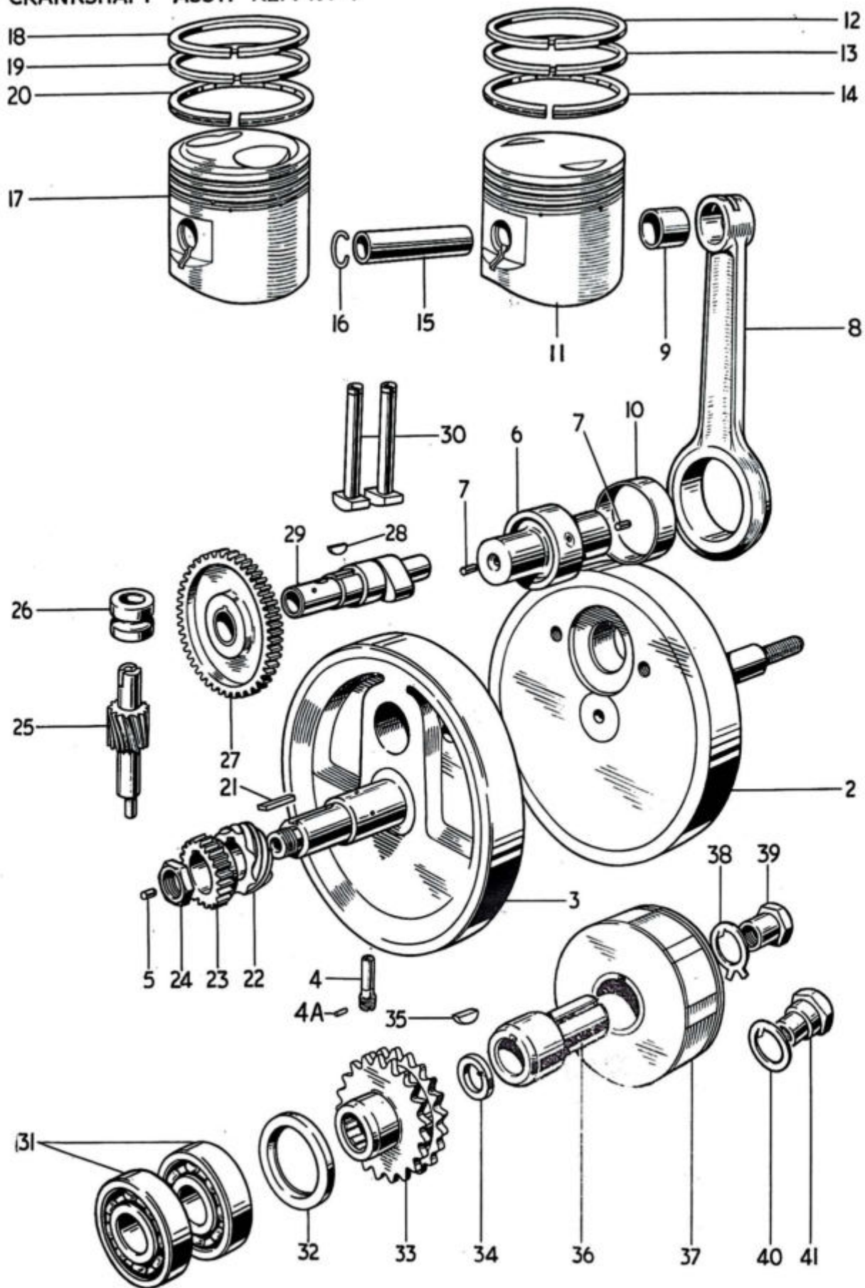
Fig. 1. CRANKSHAFT, PISTON AND TIMING GEARS
