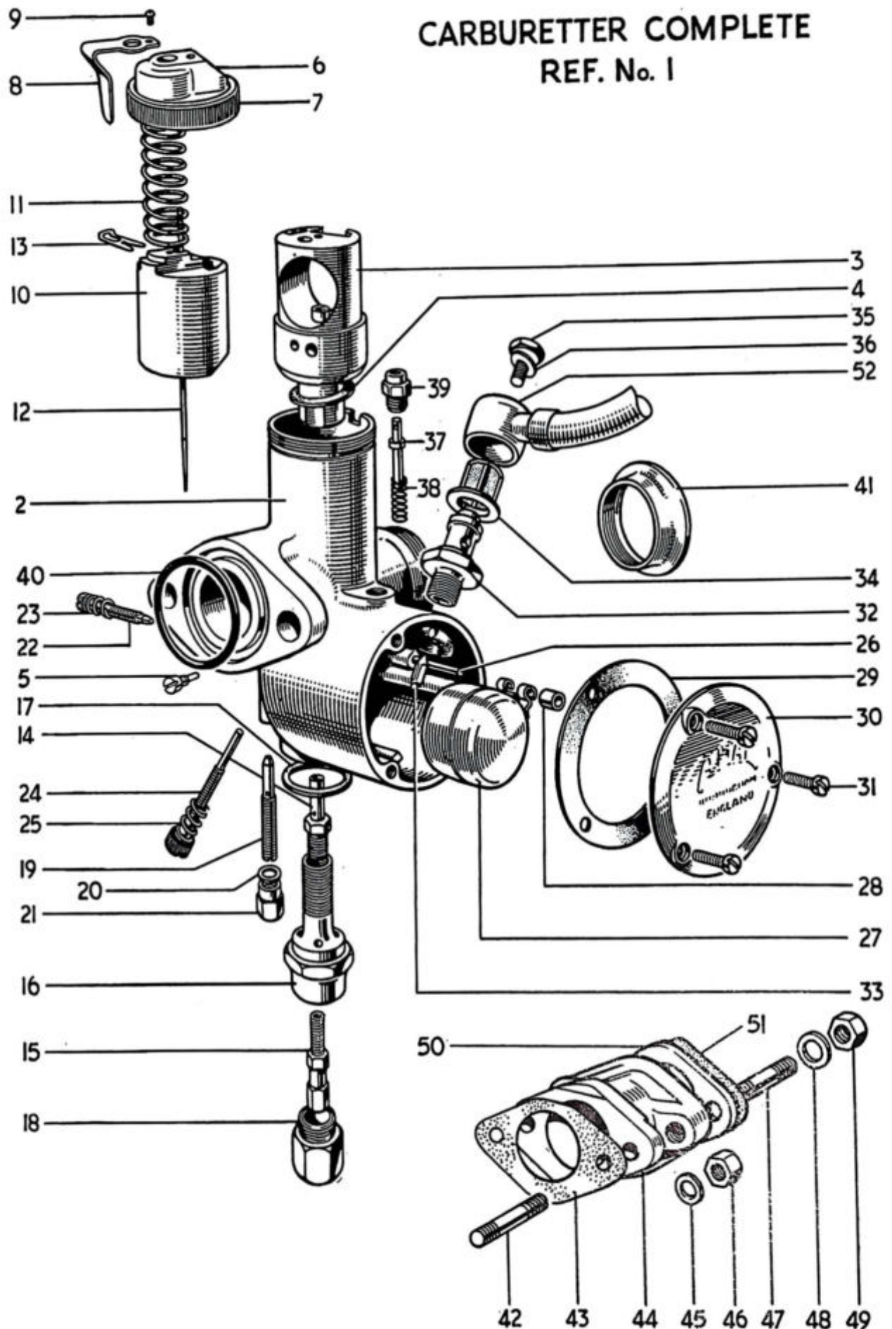
Fig. 21. AMAL CARBURETTER, TYPE 376
