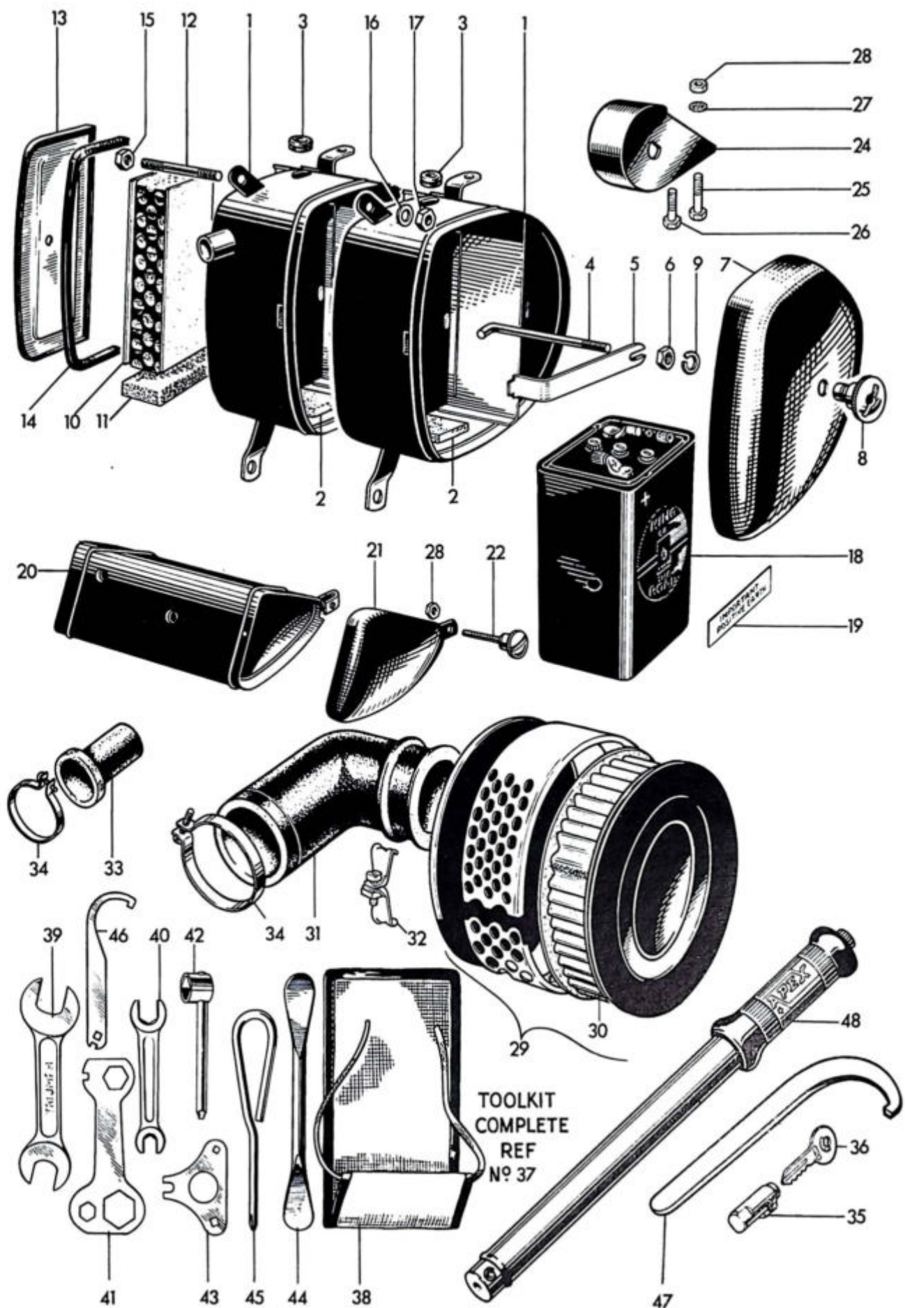
Fig. 17. BATTERY CASE, TOOLBOX AND AIR FILTER
