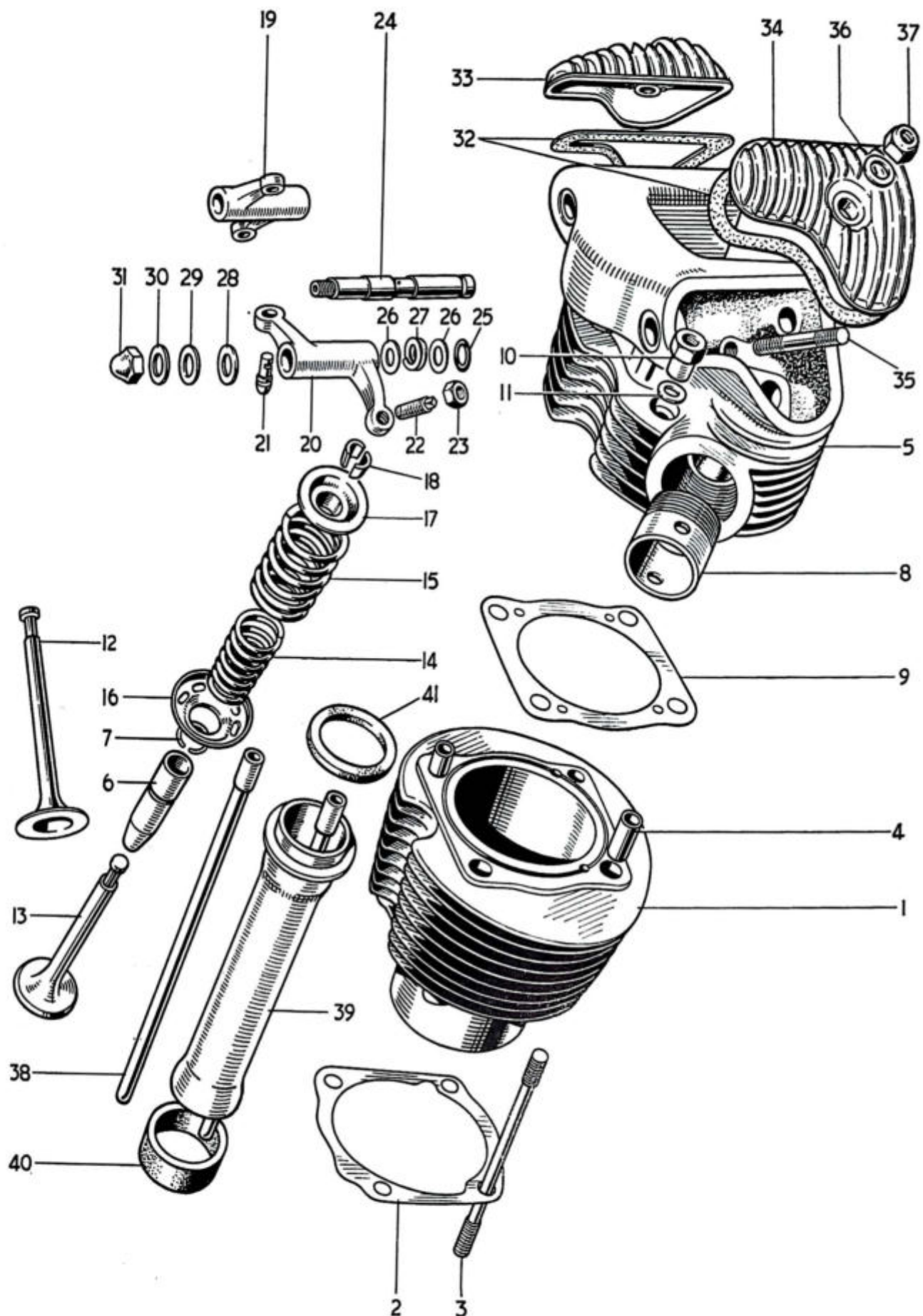
Fig. 3. CYLINDER BARREL AND HEAD
