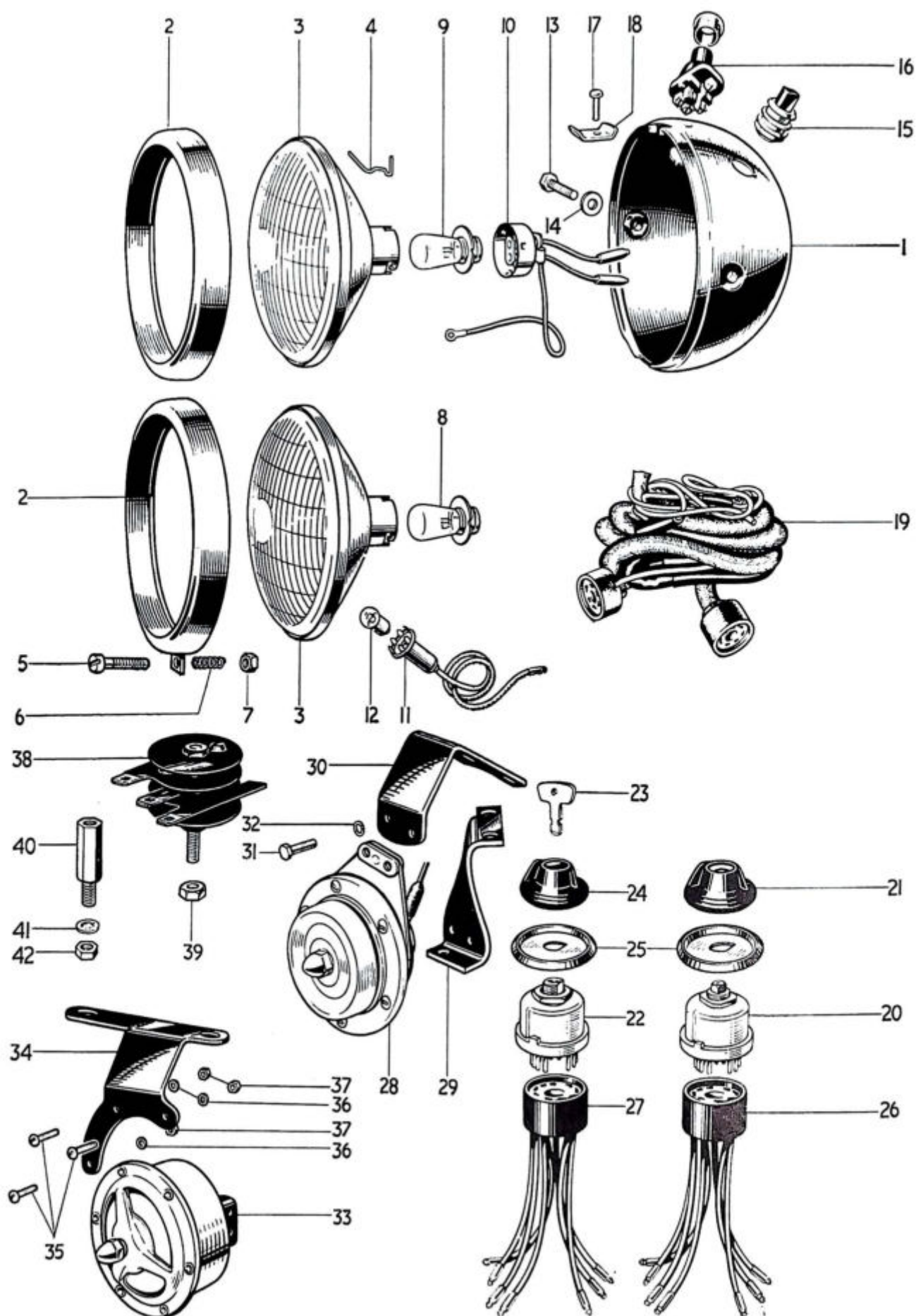
Fig. 23. ELECTRICAL EQUIPMENT, T20, T20SS AND T20SH
