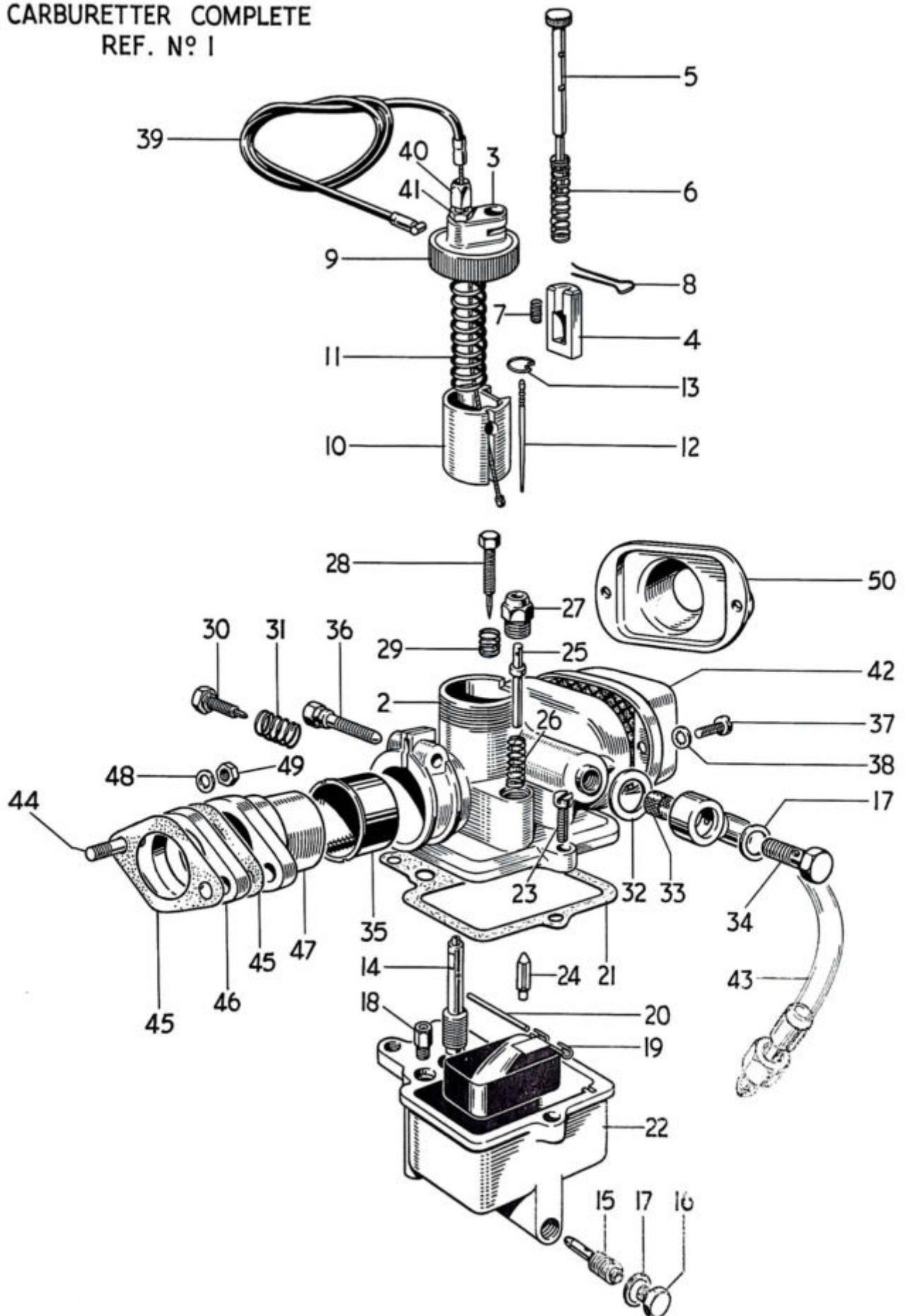
Fig. 22. AMAL CARBURETTER, TYPE 32
