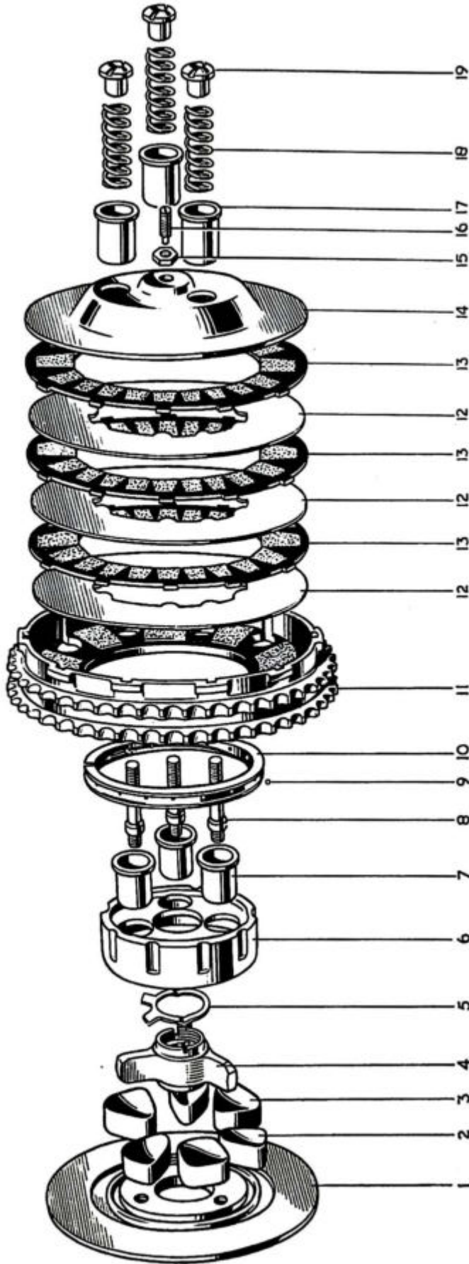
FIG. 3. CLUTCH AND SHOCK ABSORBER UNIT.
