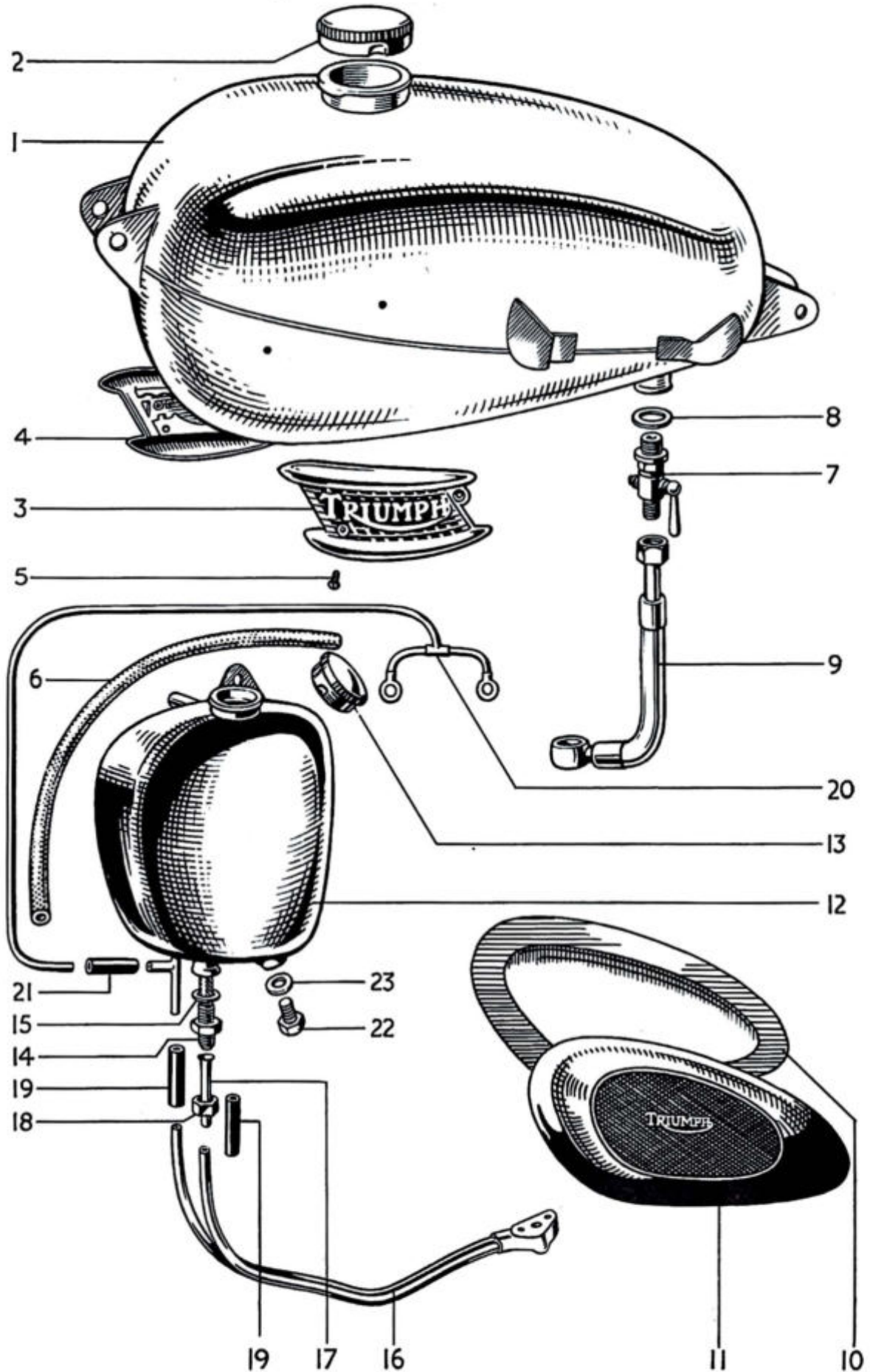
FIG. 13. PETROL AND OIL TANKS. For Index See Page 41.
