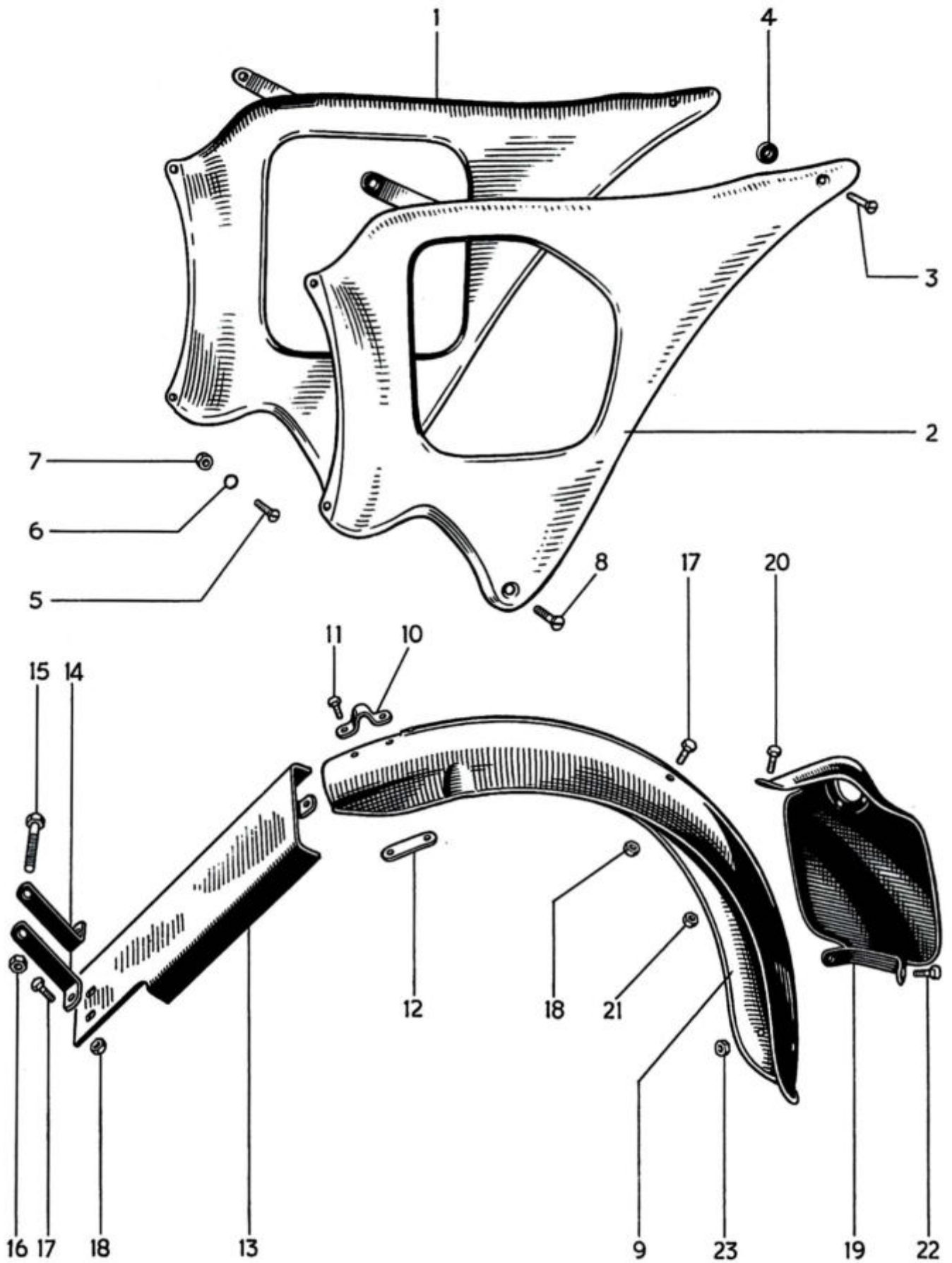
FIG. 10. REAR PANELS.
