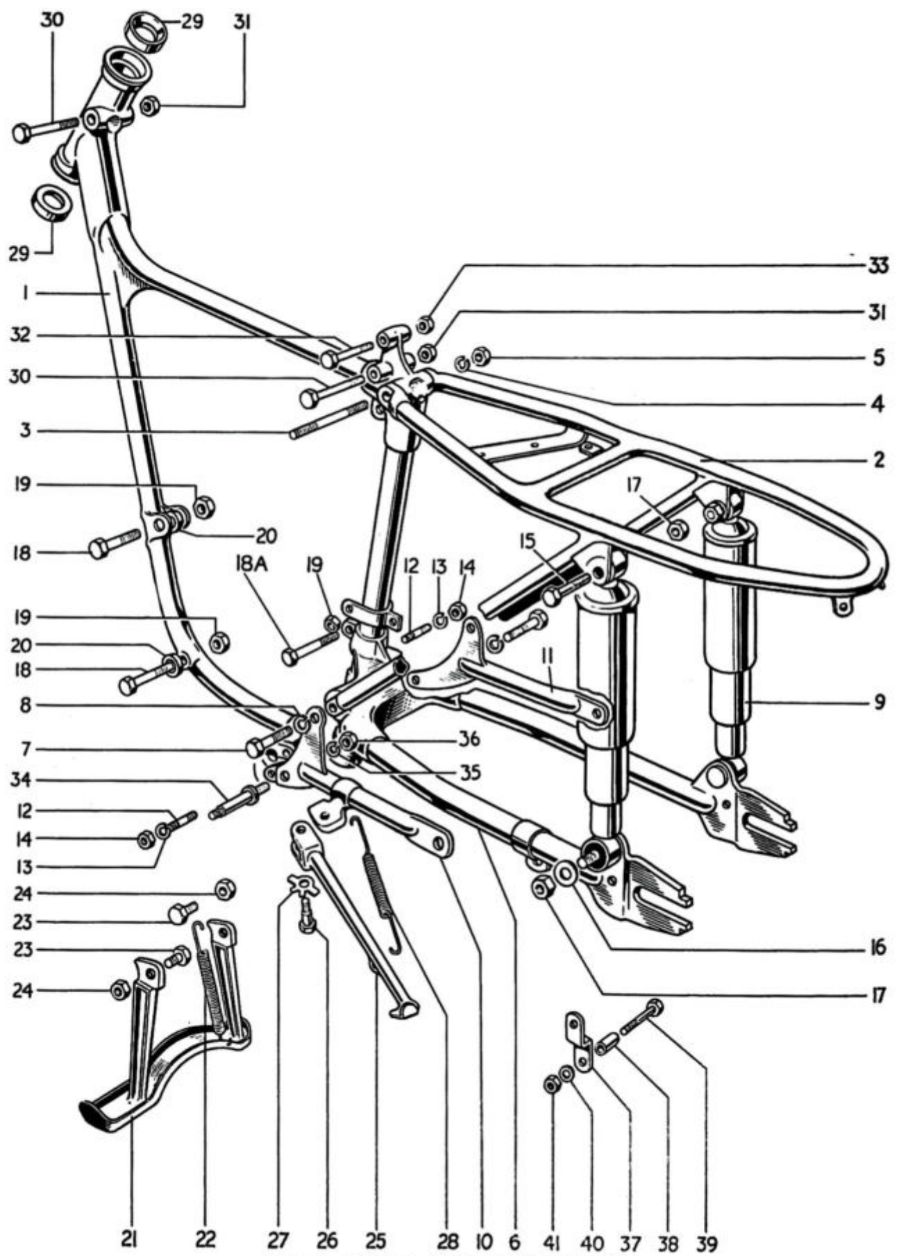
FIG. 4. FRAME AND COMPONENTS.
