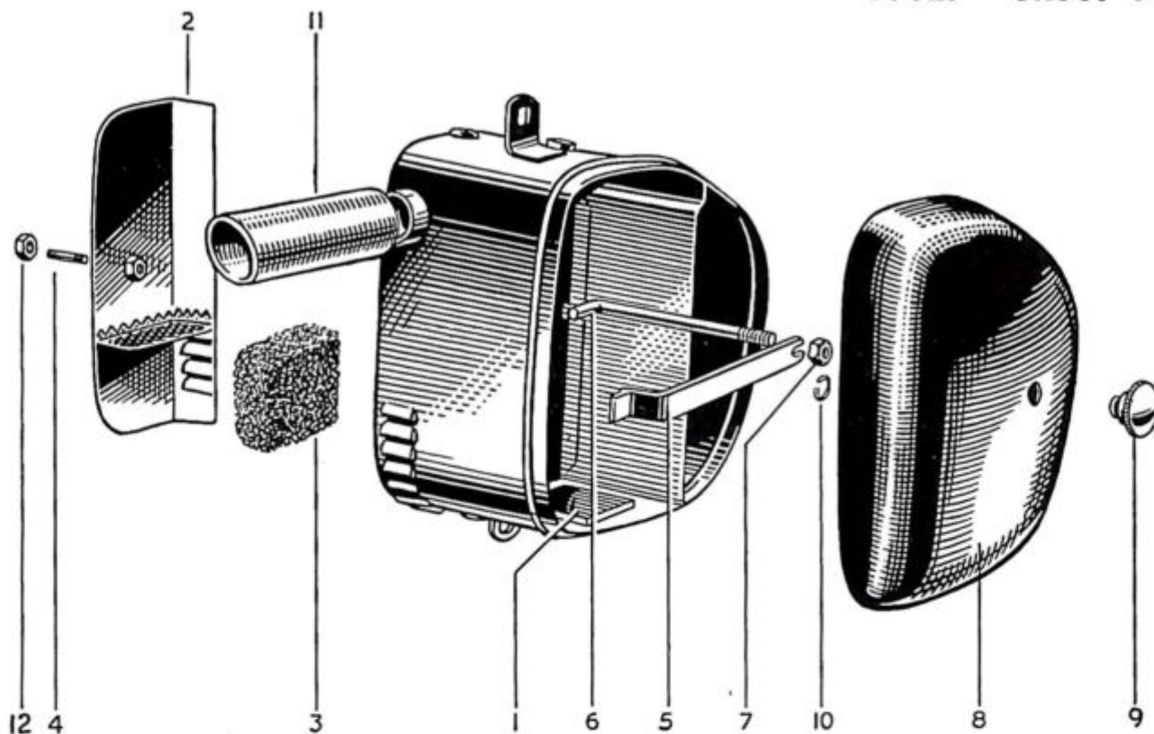
FIG. 11. TOOLBOX, BATTERY CARRIER AND AIR CLEANER.
