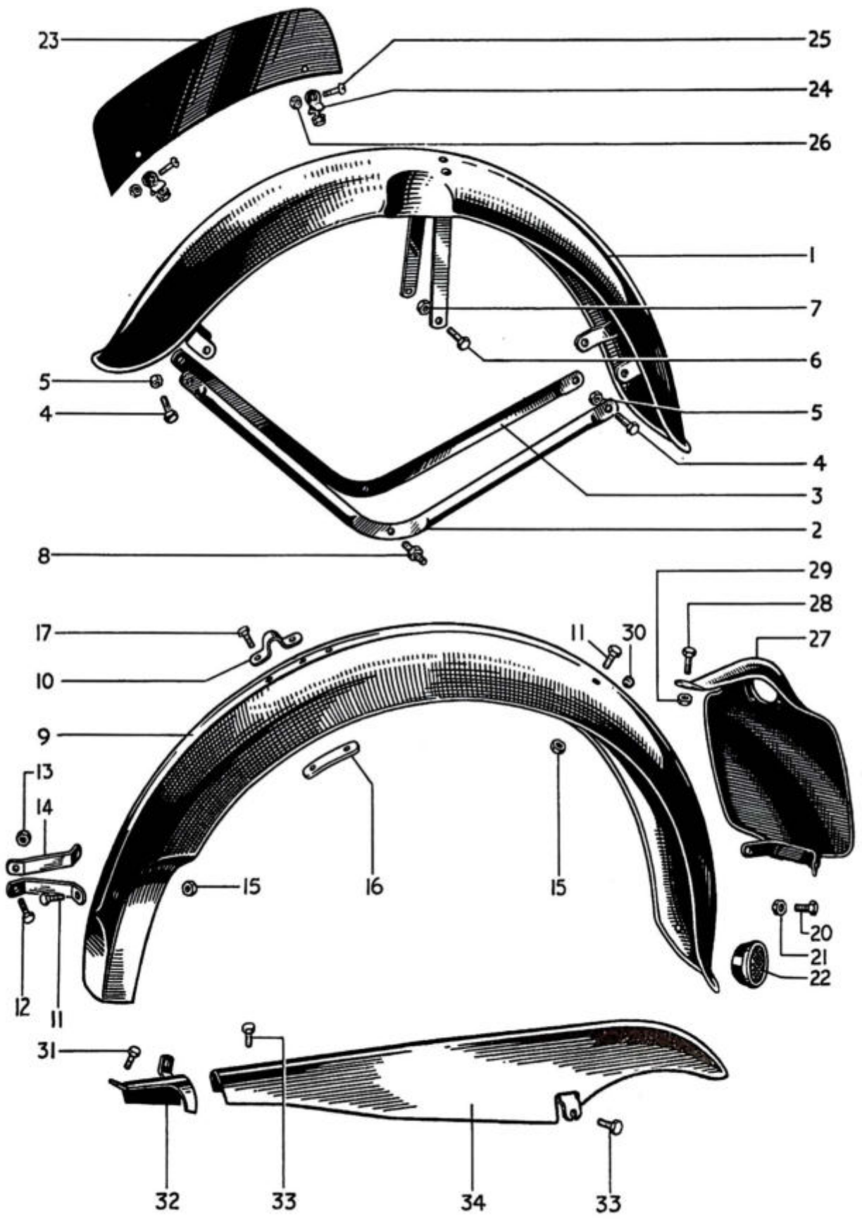
FIG. 9. MUDGUARDS, NUMBER PLATES AND REAR CHAINGUARD. See Page 36 for Rear Panels.
