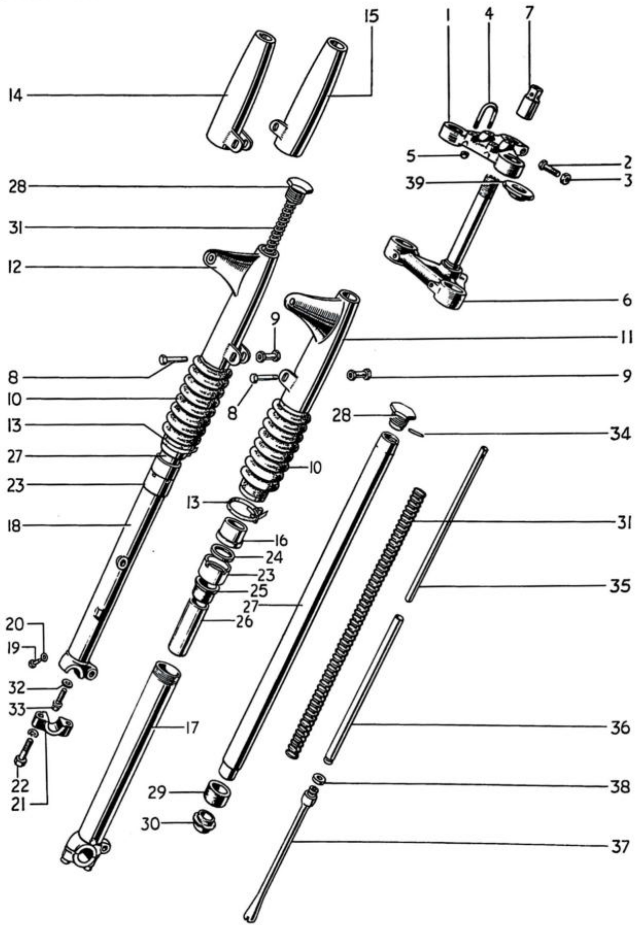
FIG. 16. TELESCOPIC FRONT FORK. T20S.
