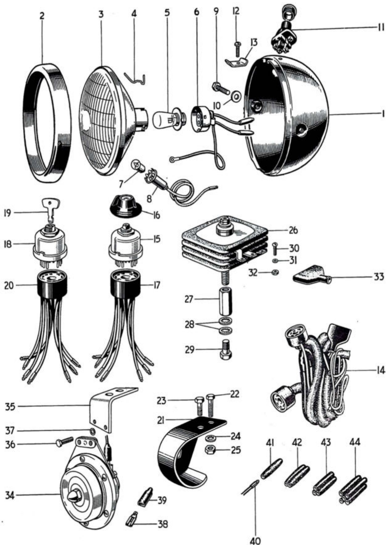
Fig. 28. T20SH ELECTRICAL EQUIPMENT.
