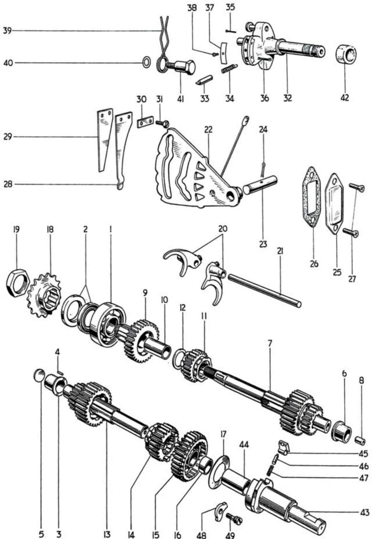
Fig. 7. GEARBOX SHAFTS AND GEARS
