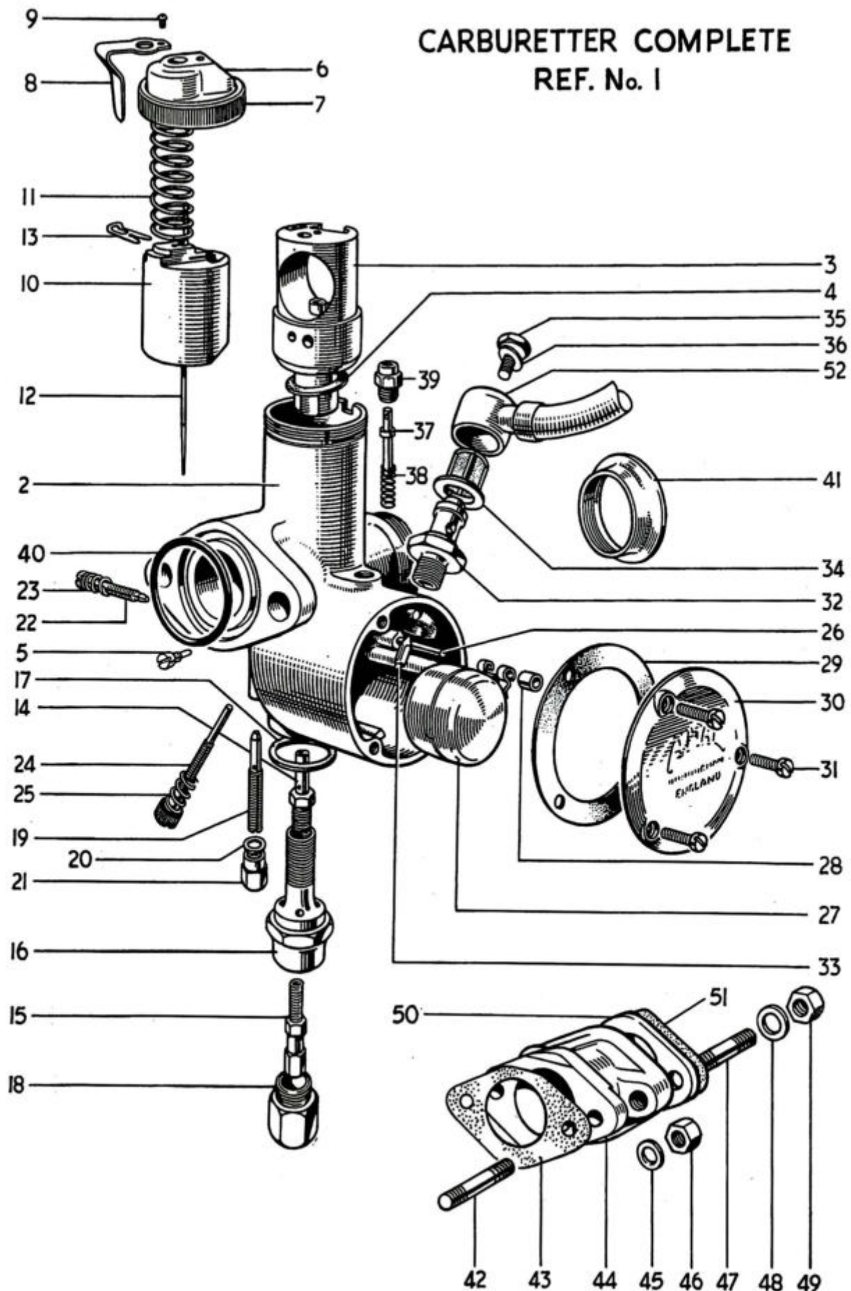
Fig. 24. AMAL CARBURETTER, TYPE 376.
