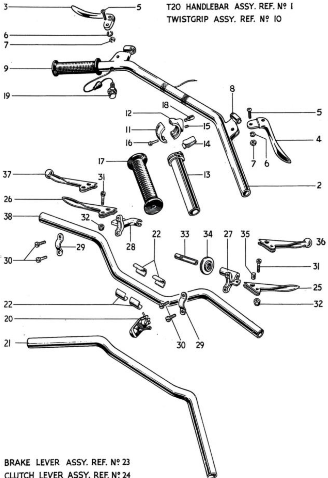
Fig. 22. HANDLEBARS AND CONTROL LEVERS.
