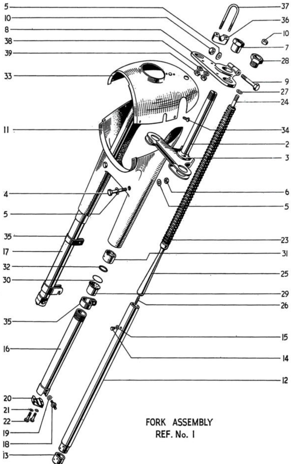
Fig. 11. TELESCOPIC FRONT FORK T20
