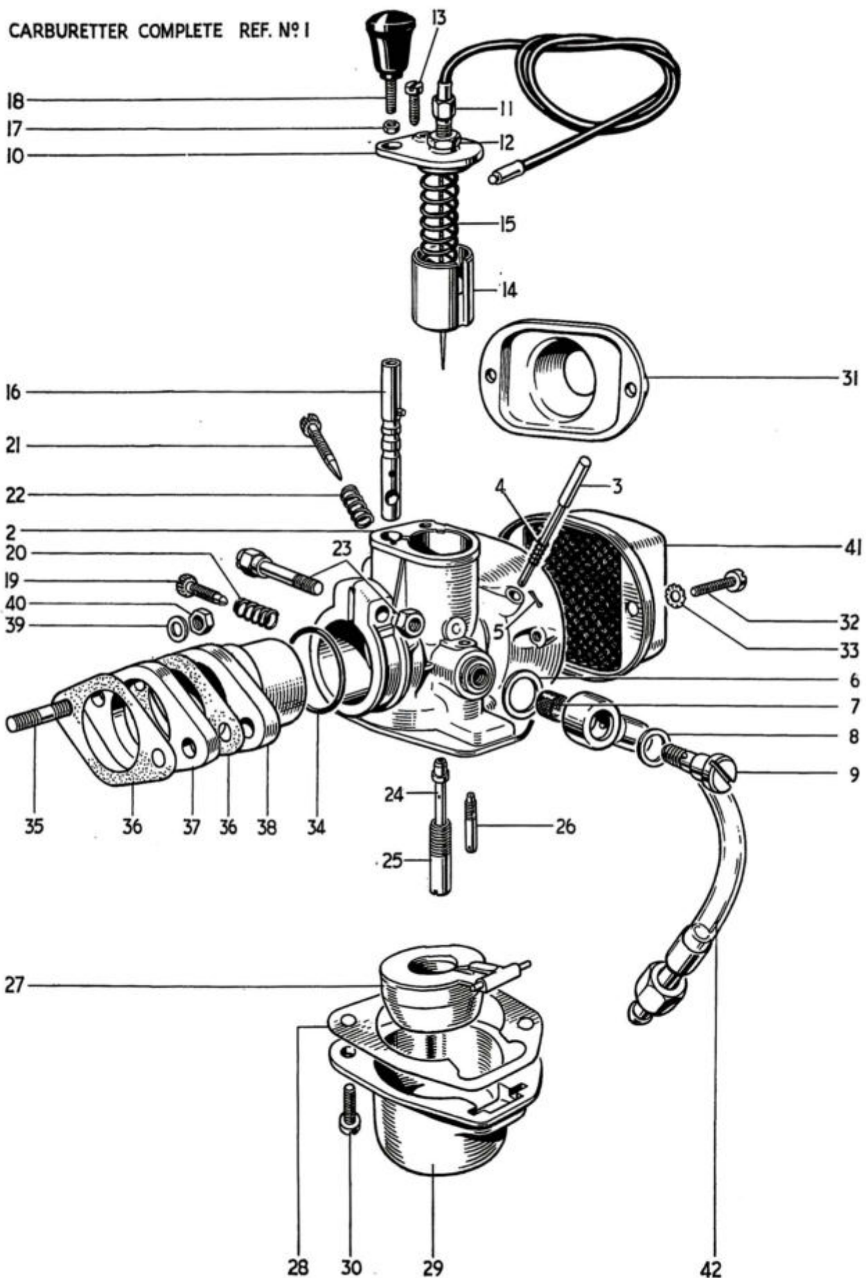
Fig. 25. ZENITH CARBURETTER.
