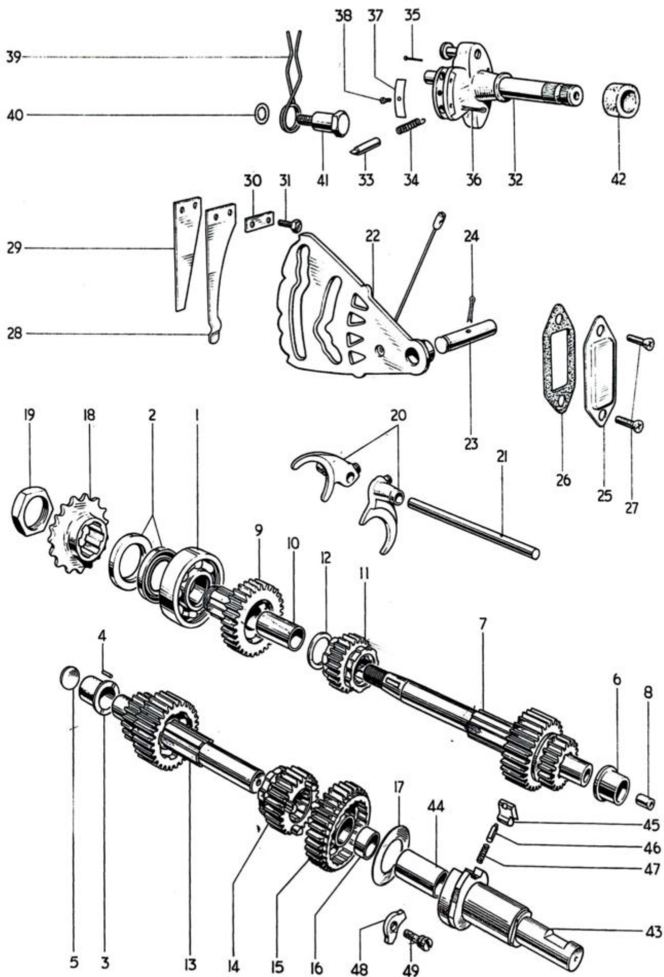
Fig. 7. GEARBOX SHAFTS AND GEARS
