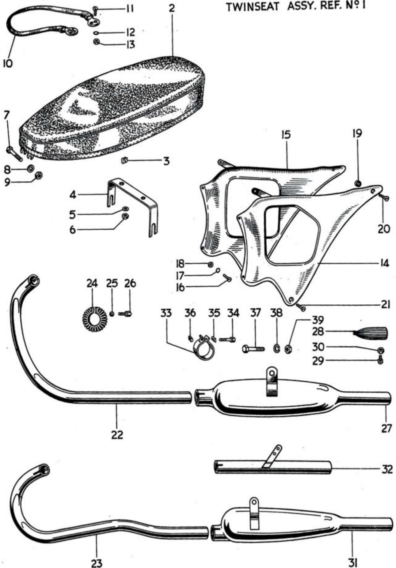
Fig. 21. TWINSEAT, REAR PANELS AND EXHAUST SYSTEM.
