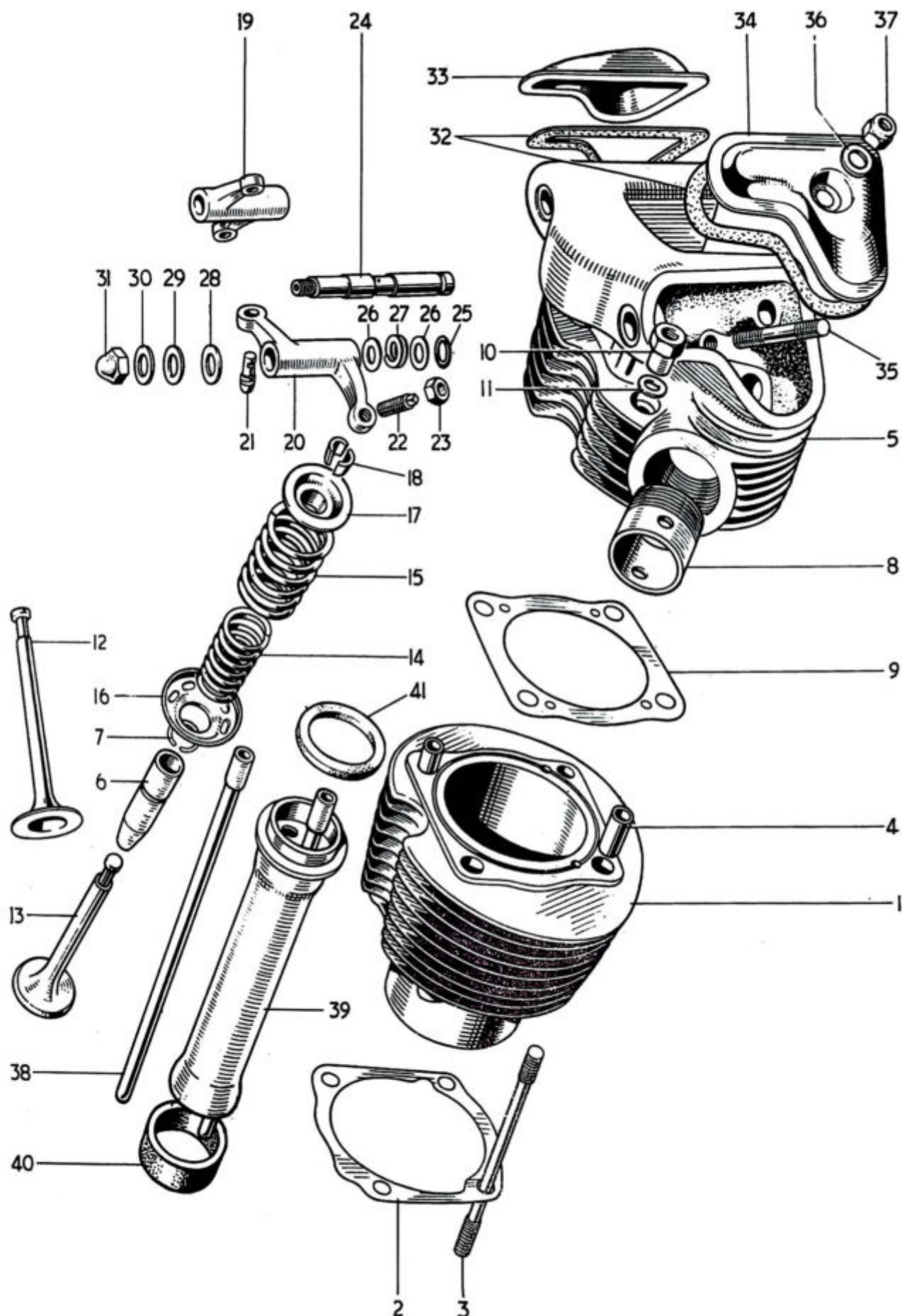
Fig. 5. CYLINDER BARREL AND HEAD
