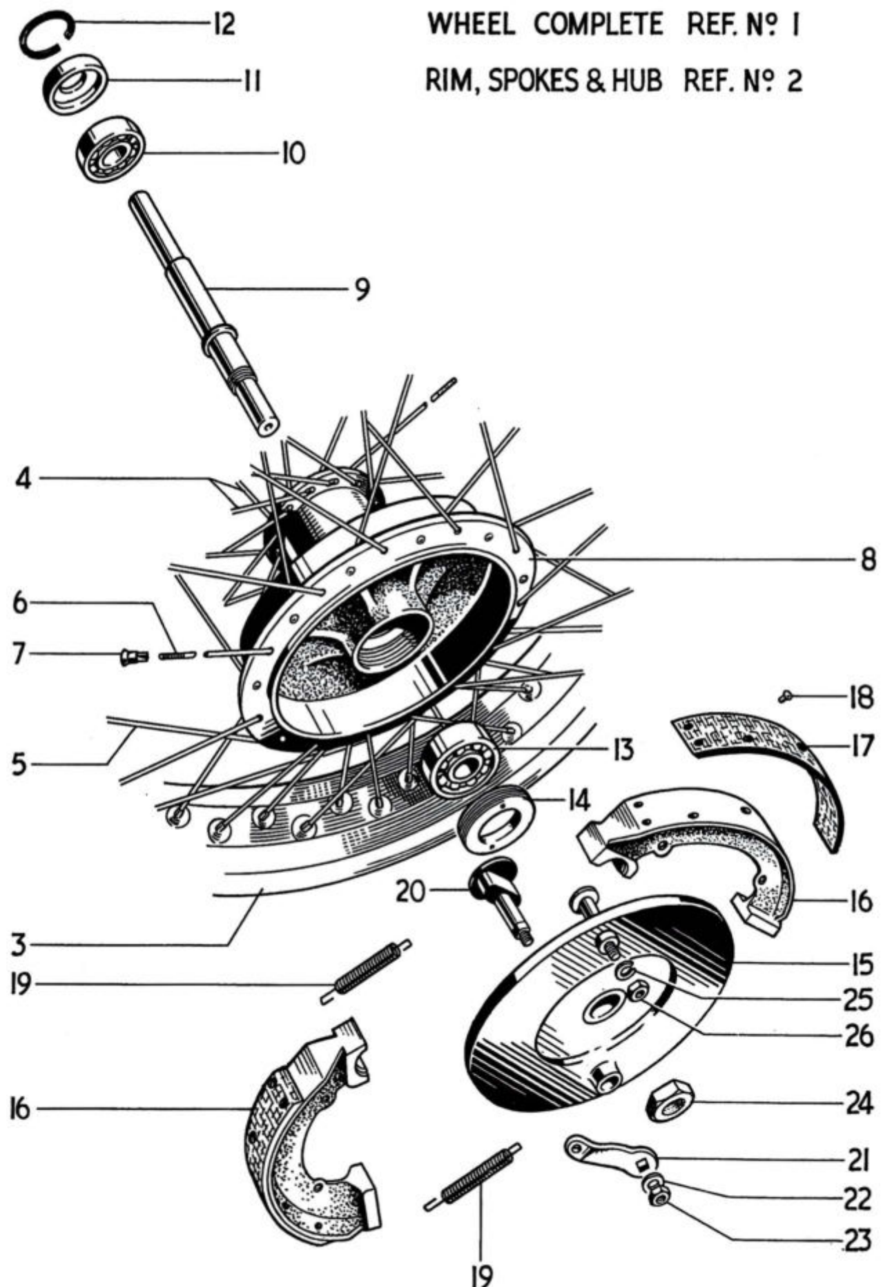
Fig. 15. FRONT WHEEL, T20.
