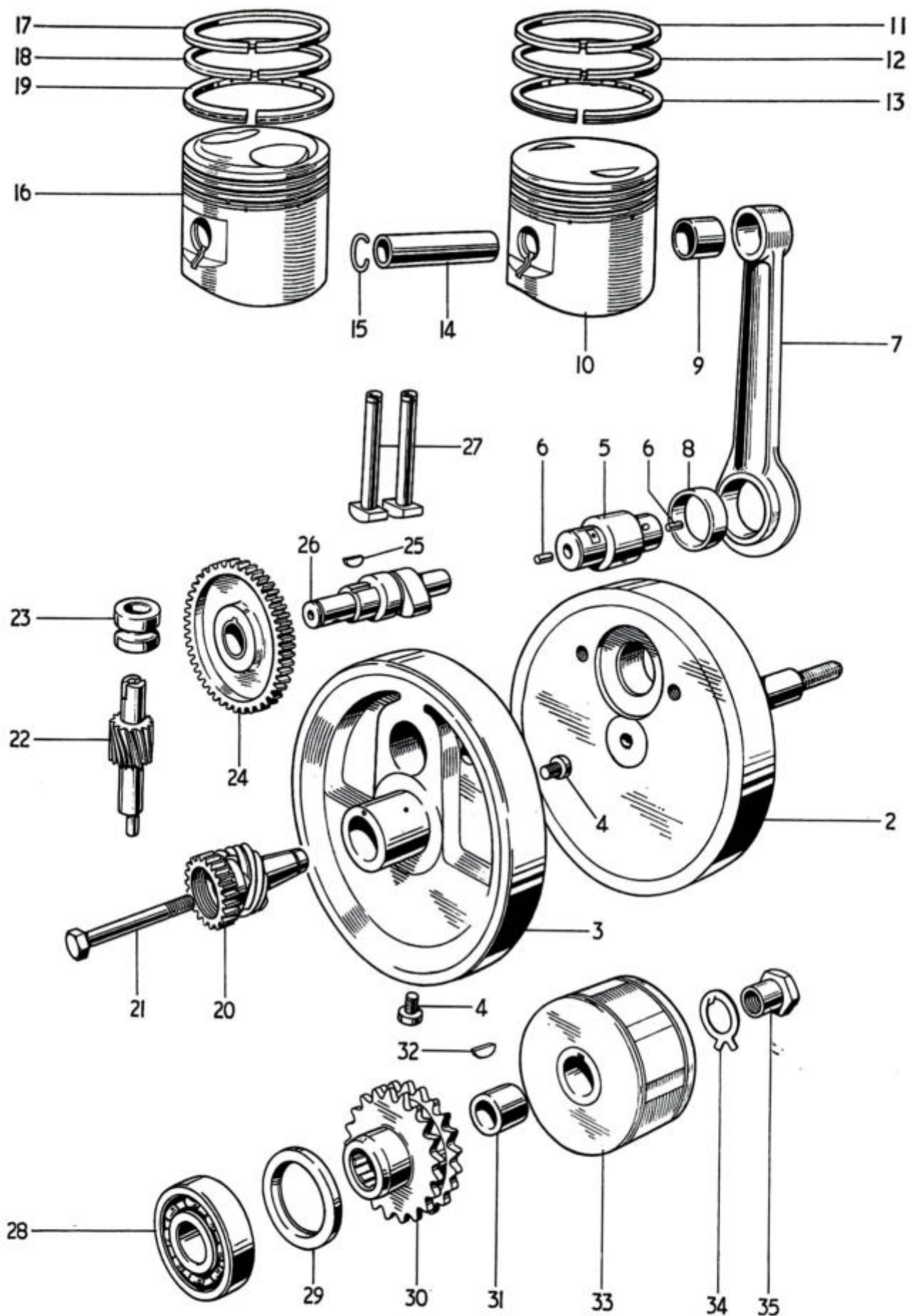
Fig. 1. CRANKSHAFT, PISTON AND TIMING GEARS Prior to Engine No. 84269
