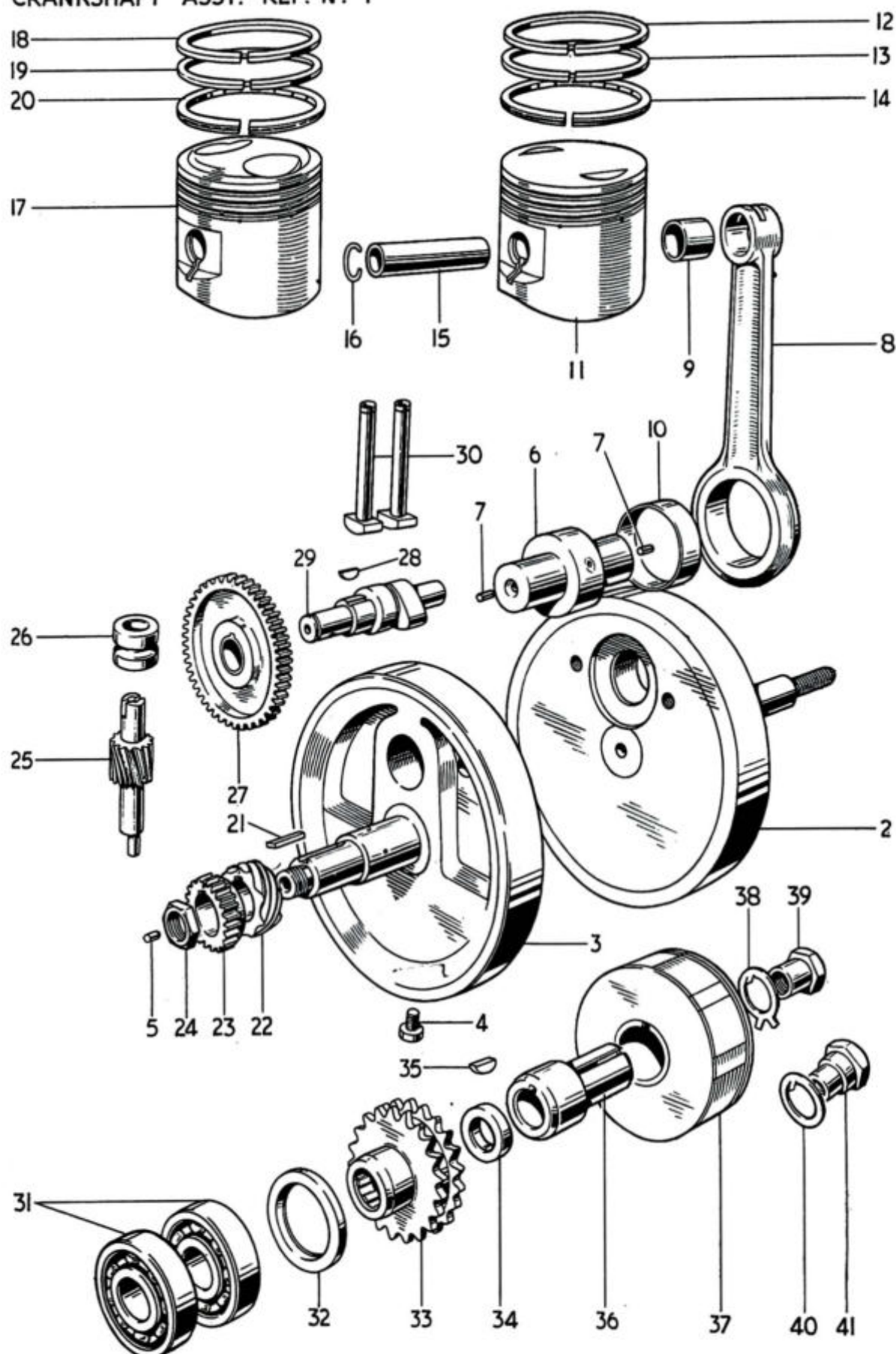
Fig. 3. CRANKSHAFT, PISTON AND TIMING GEARS From Engine No. 84269
