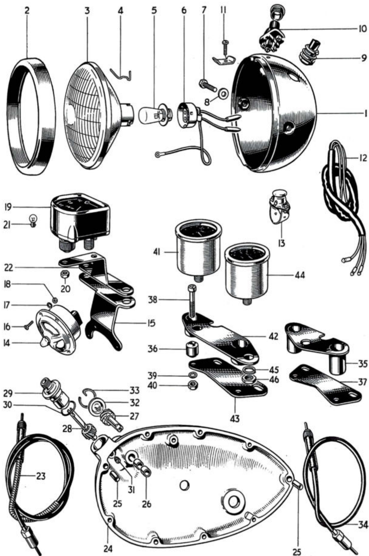
Fig. 14. T20SS HEADLAMP, TACHOMETER, Etc.
