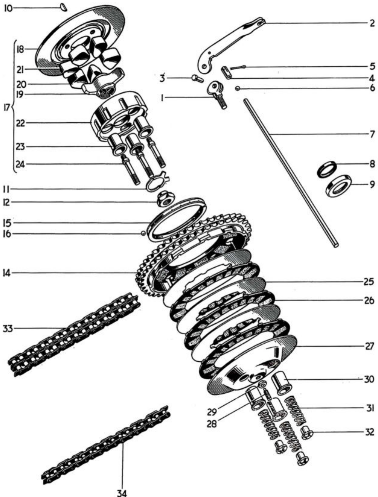
Fig. 8. CLUTCH AND CHAINS.
