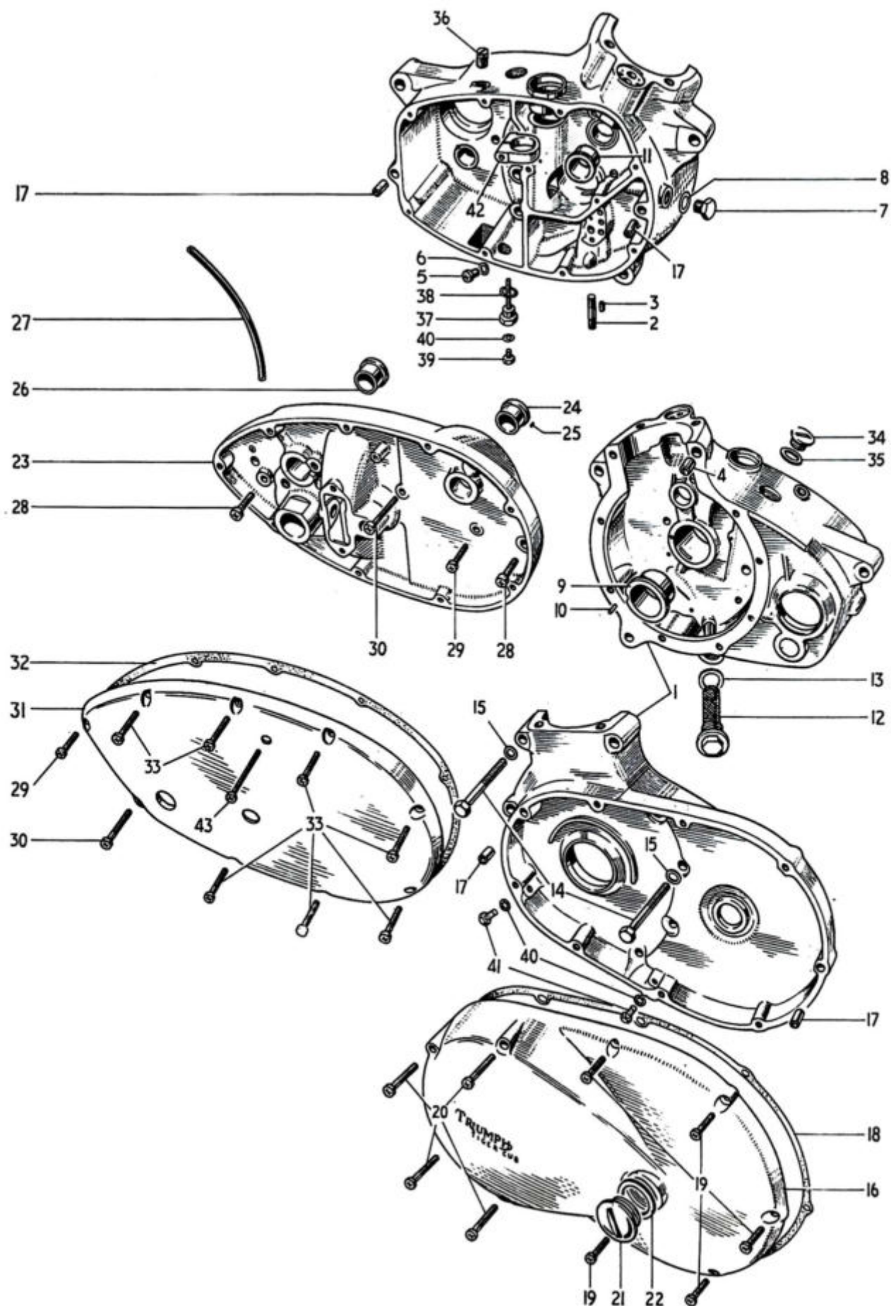
Fig. 2. CRANKCASE Prior to Engine No. 84269
