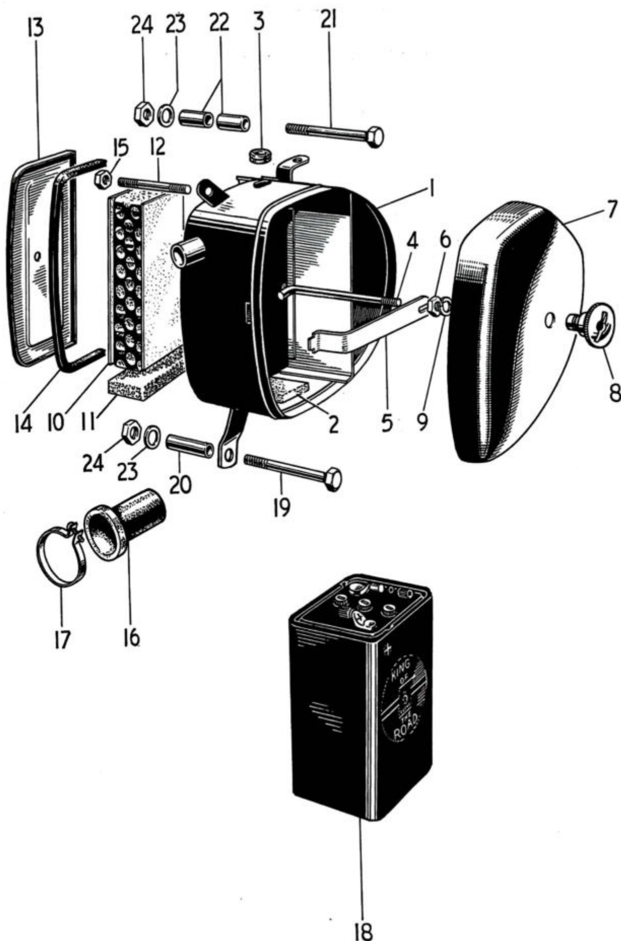
Fig. 29. T20SH BATTERY CARRIER AND AIR FILTER.
