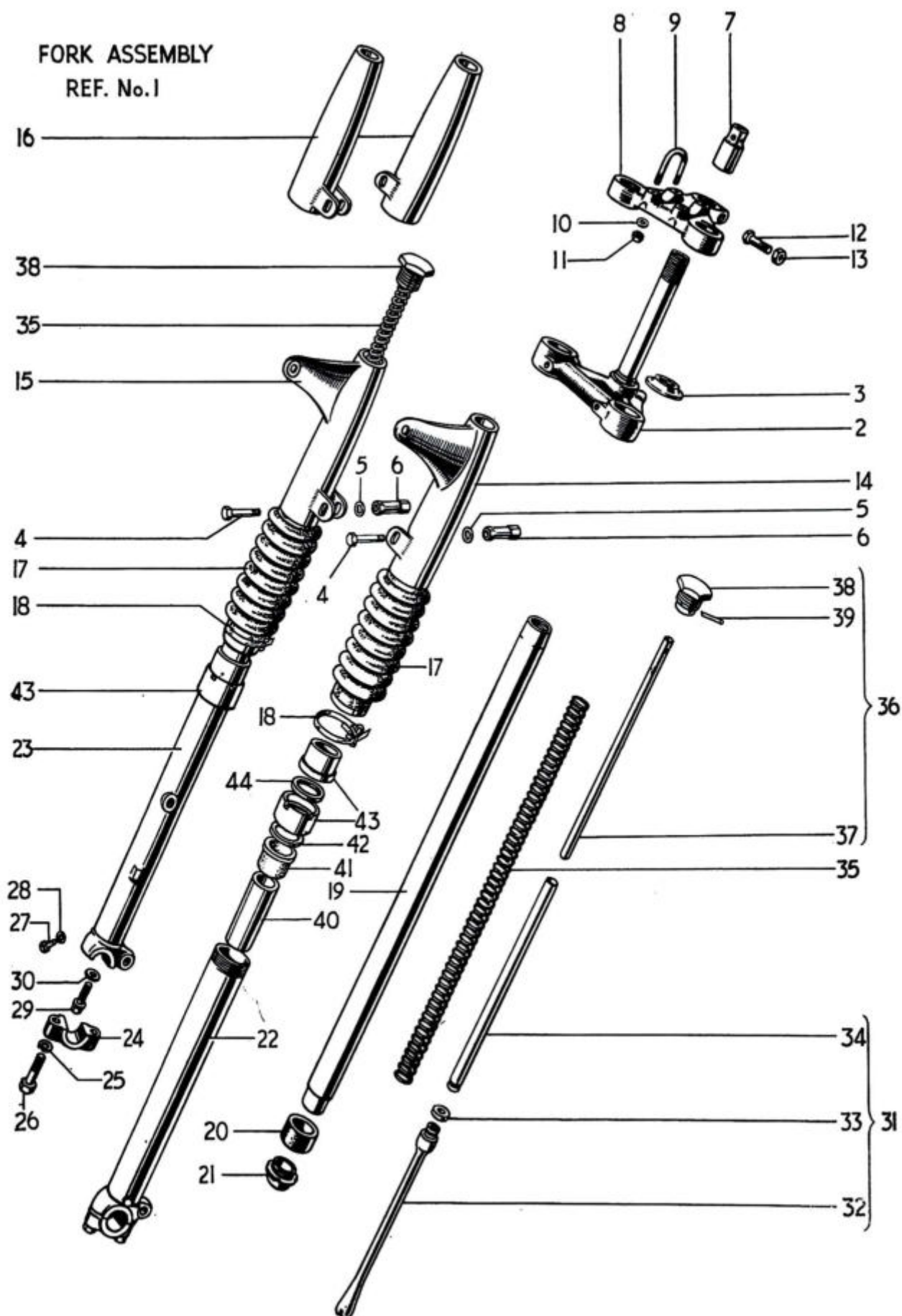
Fig. 13. TELESCOPIC FRONT FORK T20SS and T20SH
