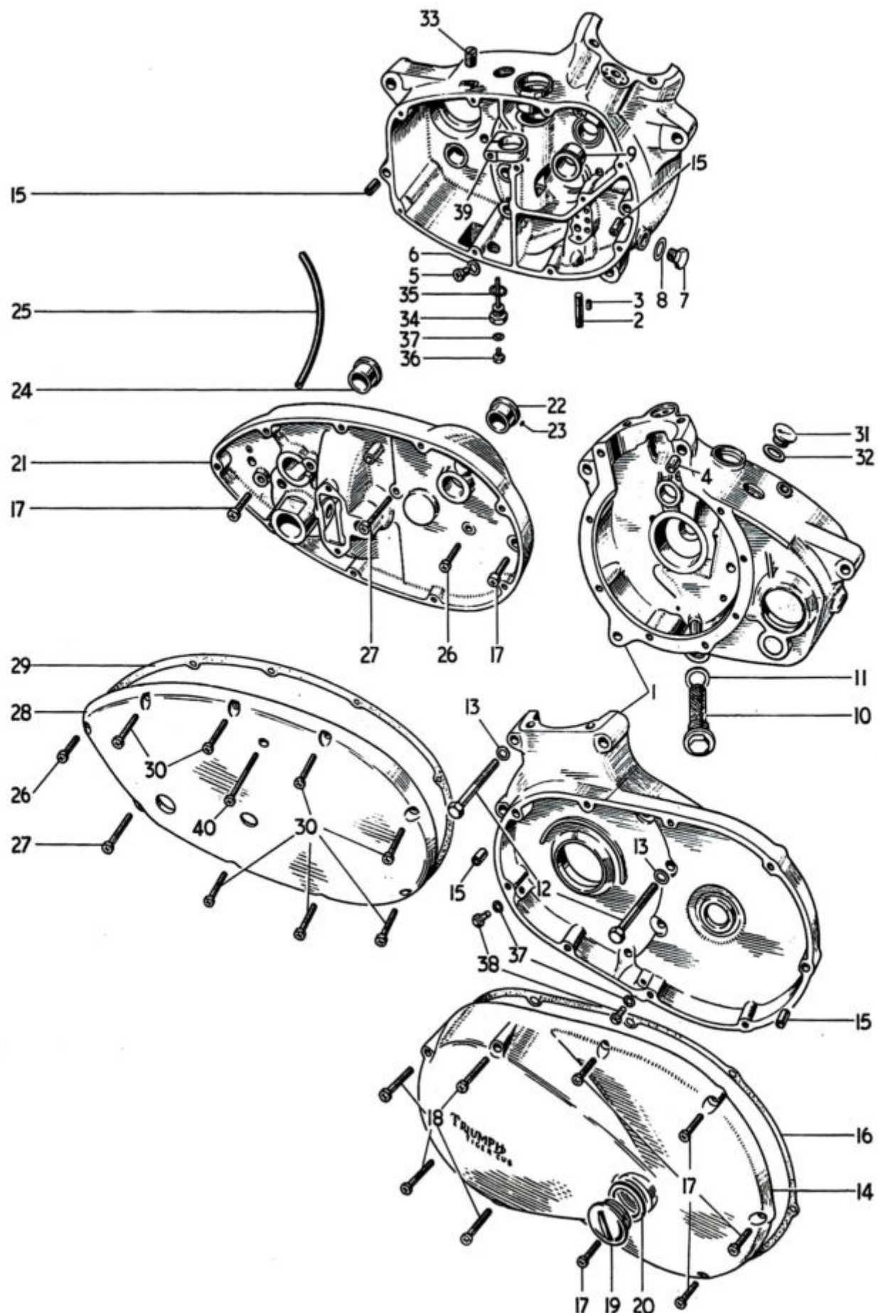
Fig. 4. CRANKCASE. From Engine No. 84269
