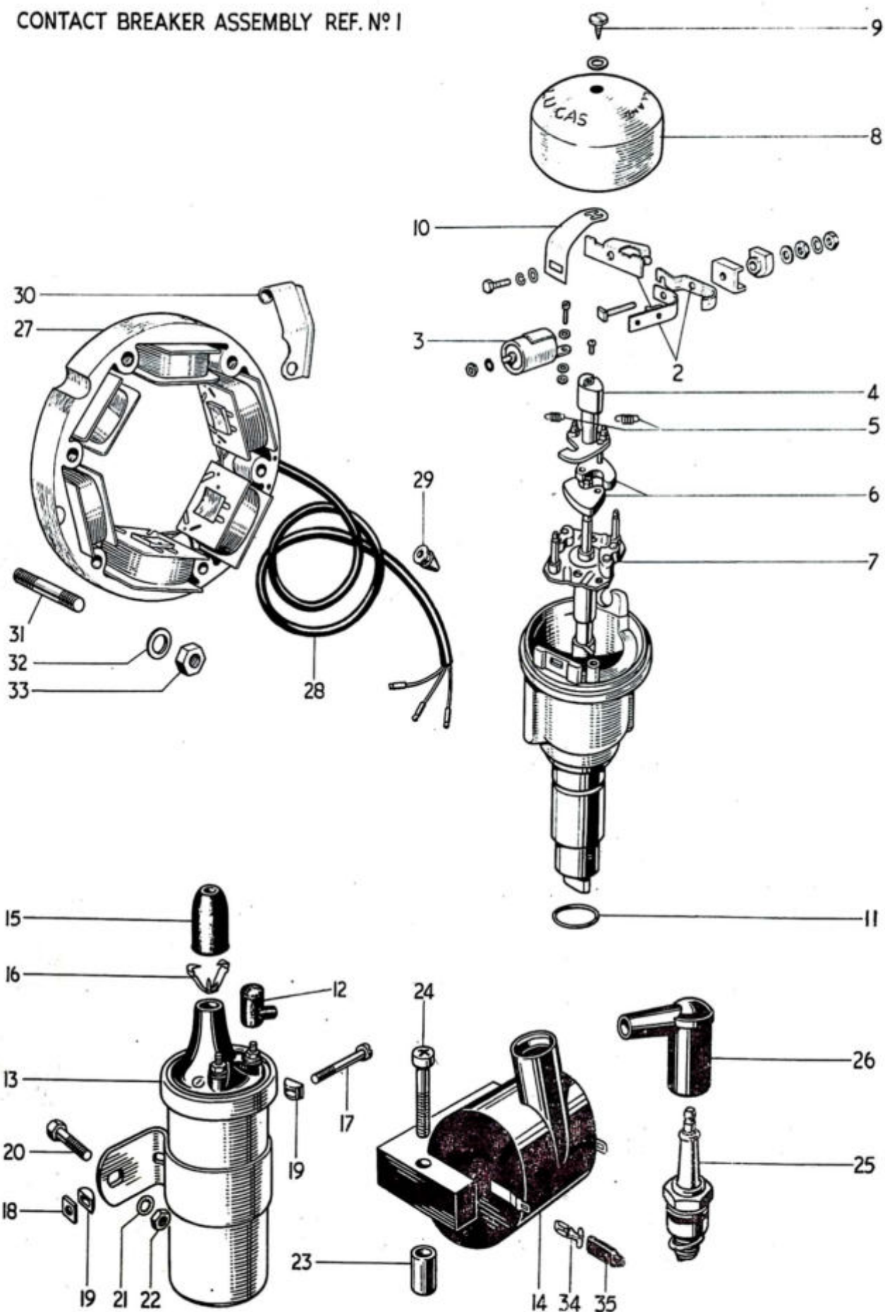
Fig. 27. CONTACT BREAKER, COIL AND STATOR.
