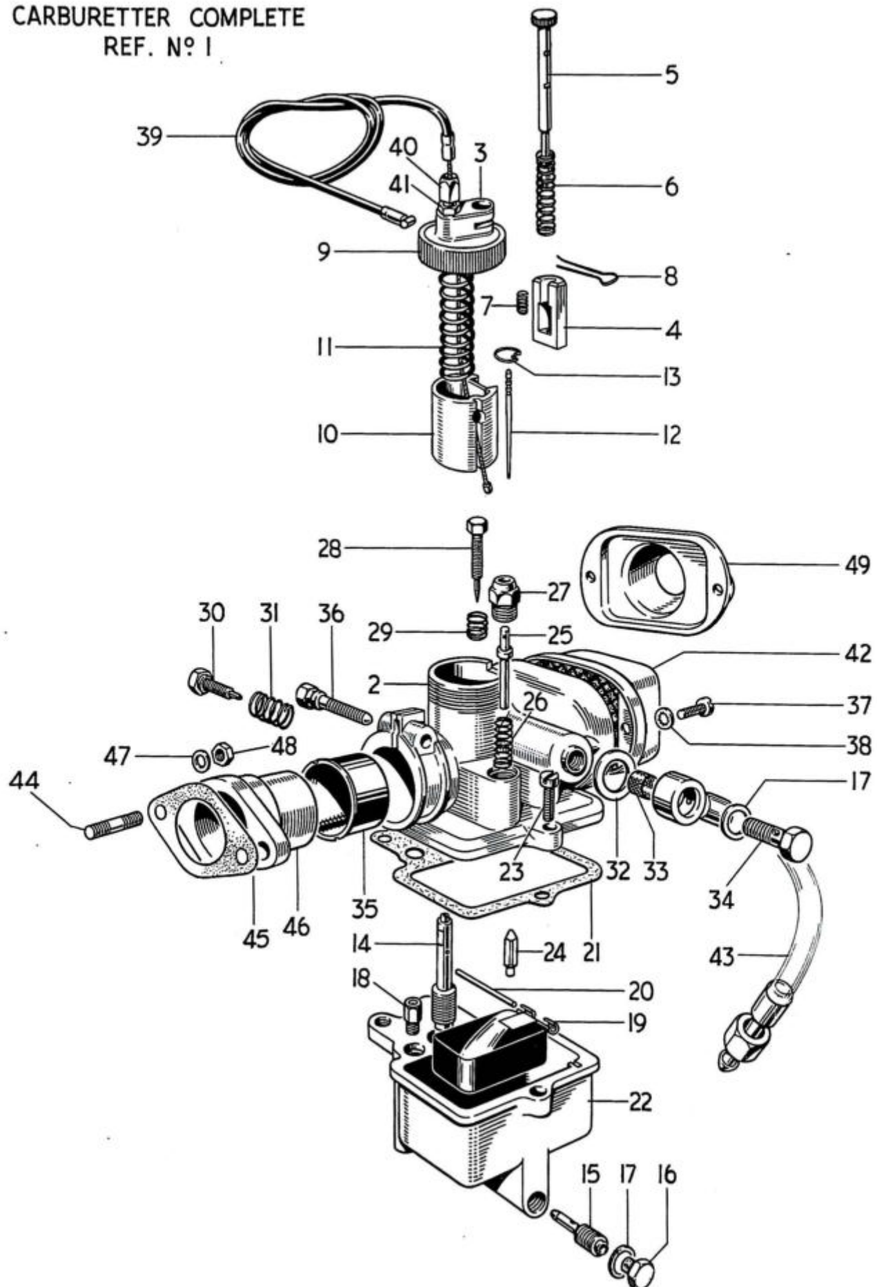
Fig. 26. AMAL CARBURETTER, TYPE 32.
