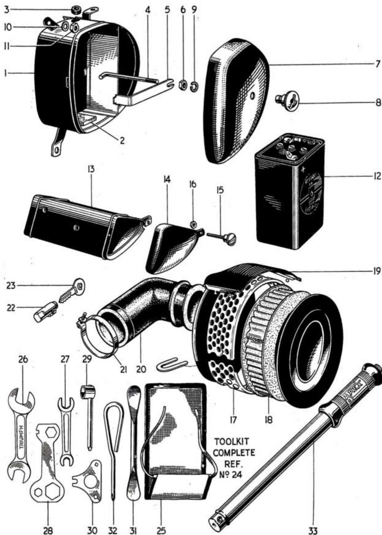
Fig. 19. BATTERY CASE, TOOLBOX AND AIR FILTER.
