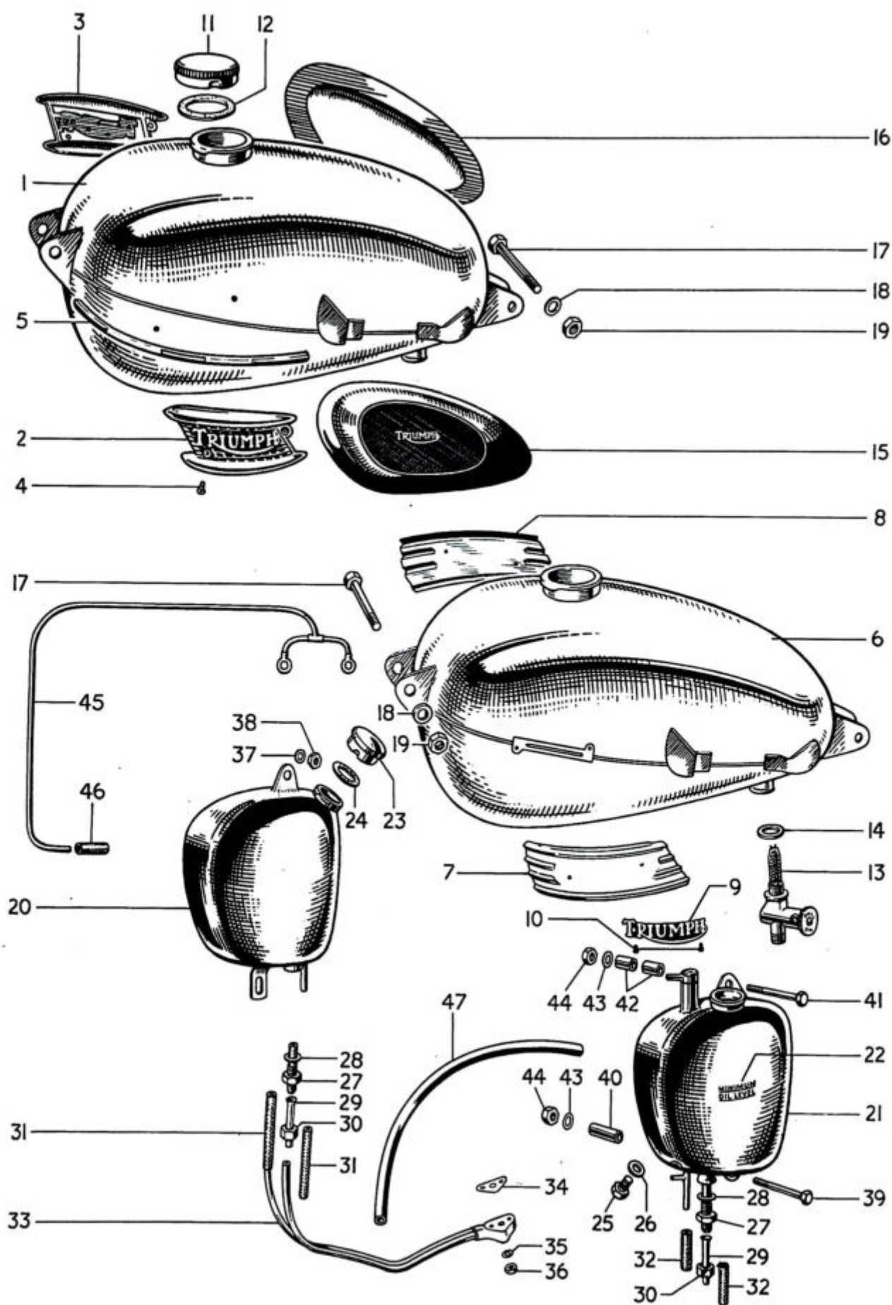
Fig. 18. PETROL AND OIL TANKS.
