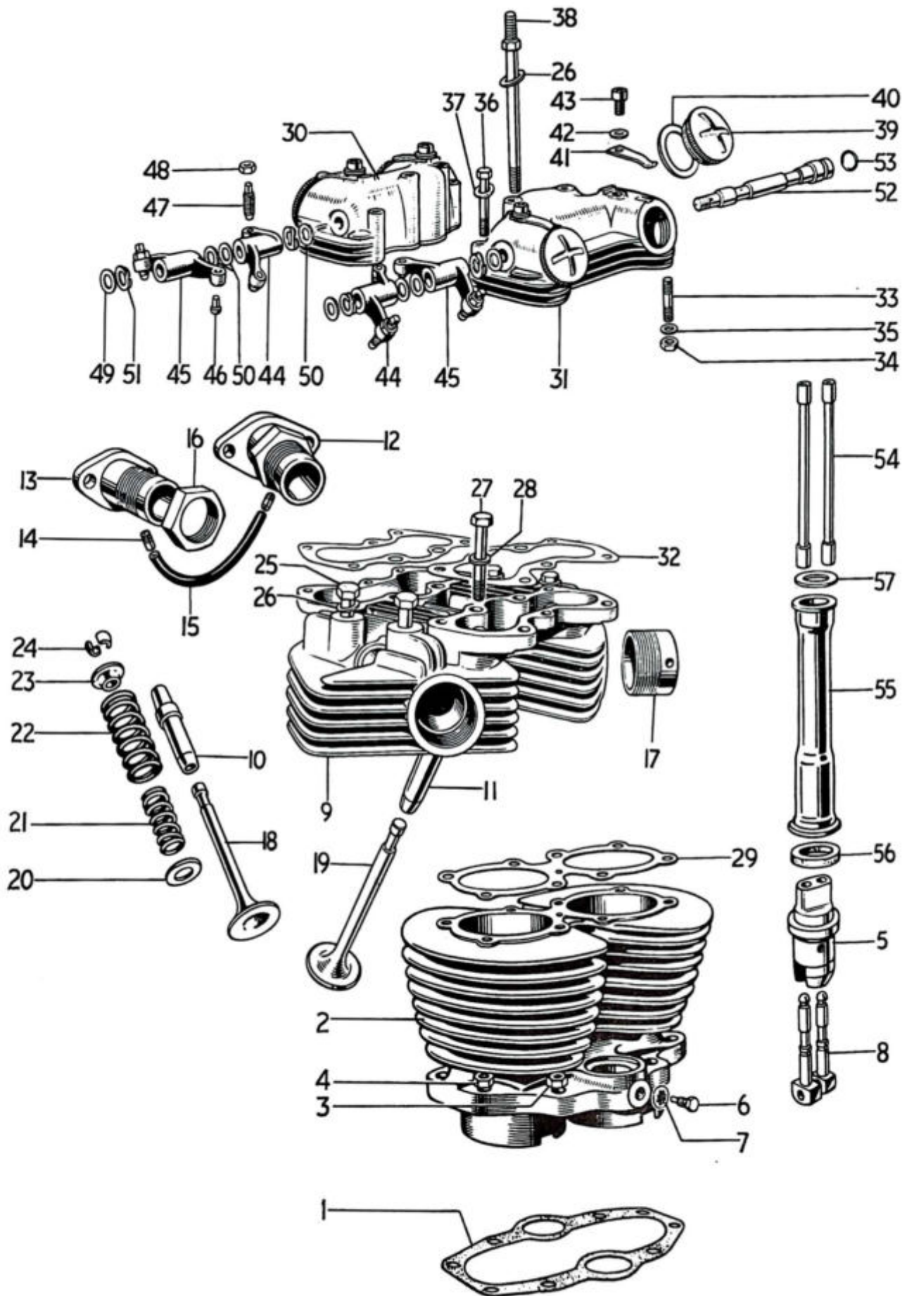
Fig. 5. CYLINDER BLOCK AND HEAD, T120
