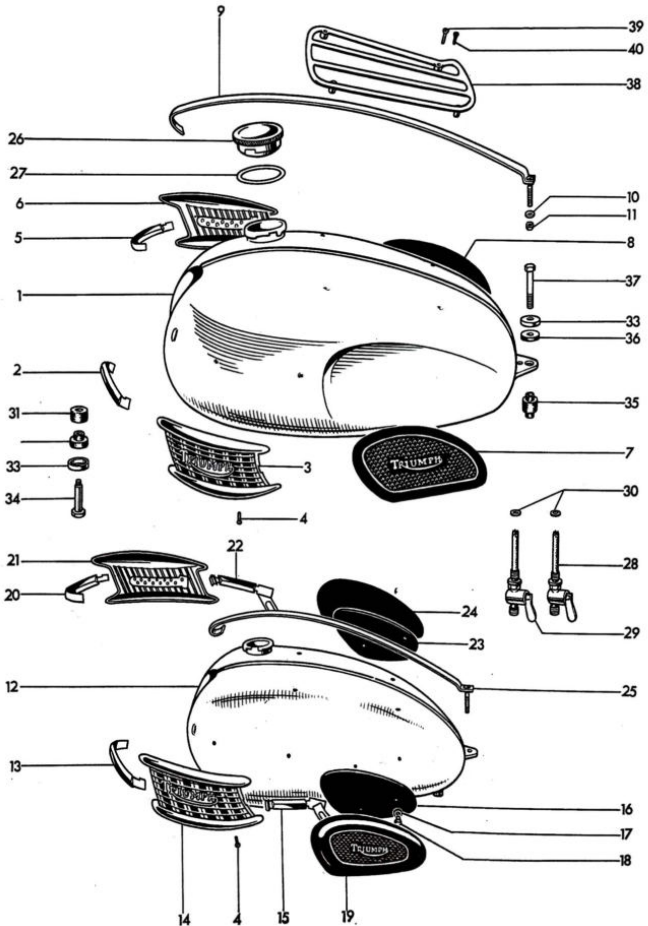
Fig. 22. PETROL TANKS
