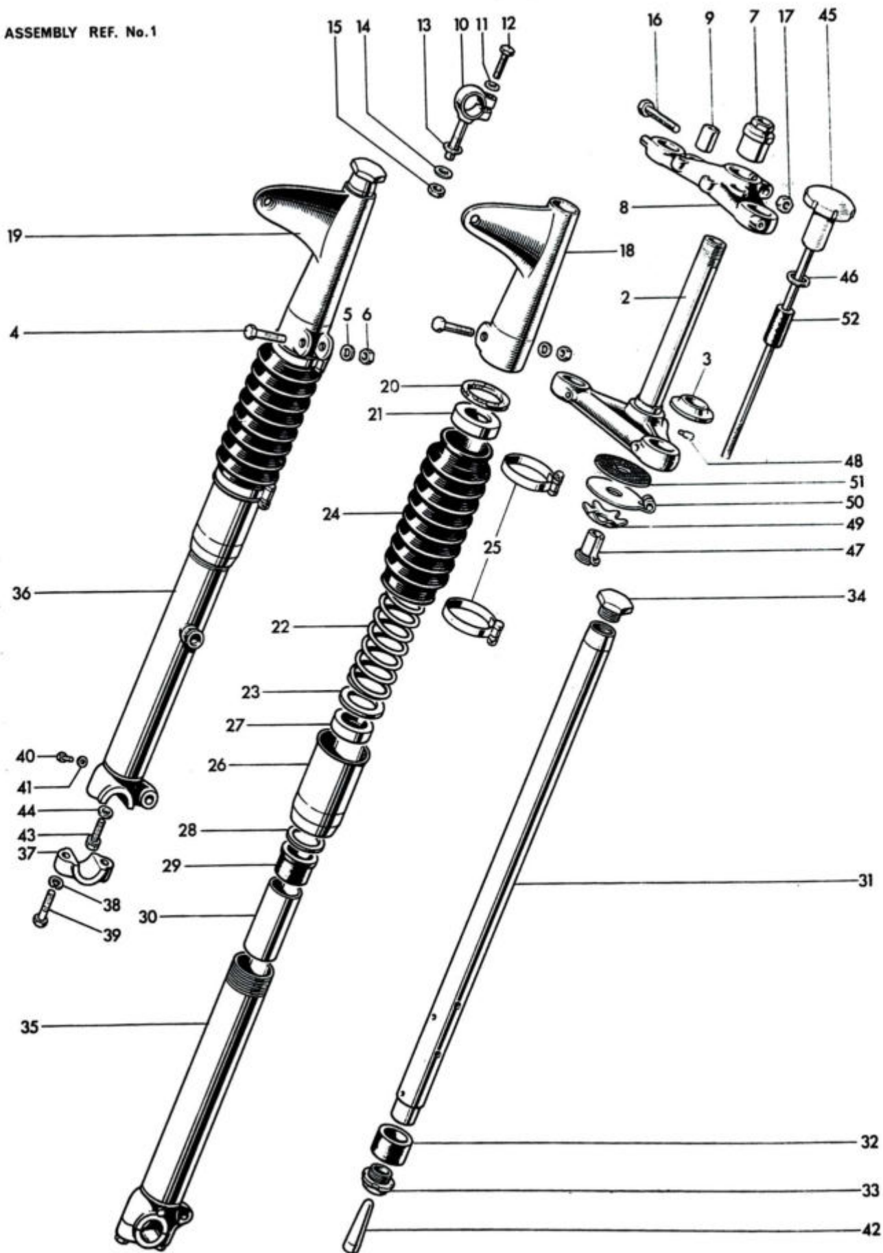
Fig. 18. TELESCOPIC FRONT FORK, TR6 AND T120
