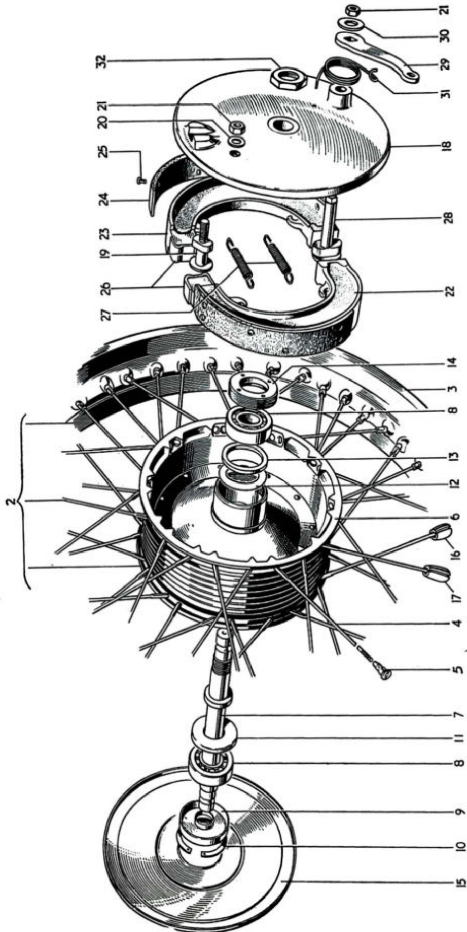
Fig. 19. FRONT WHEEL
