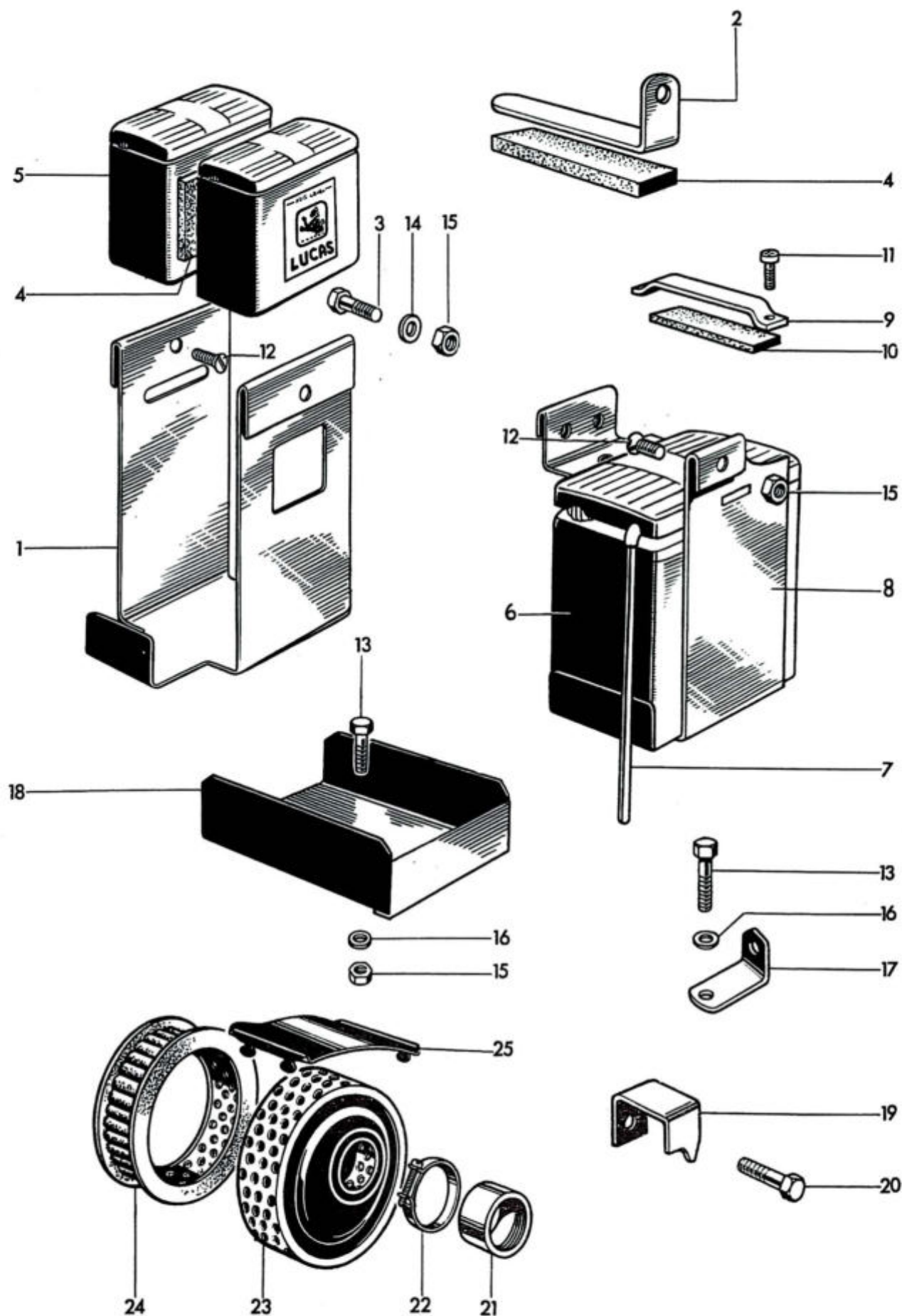
Fig. 24. BATTERY CARRIER AND AIR FILTER
