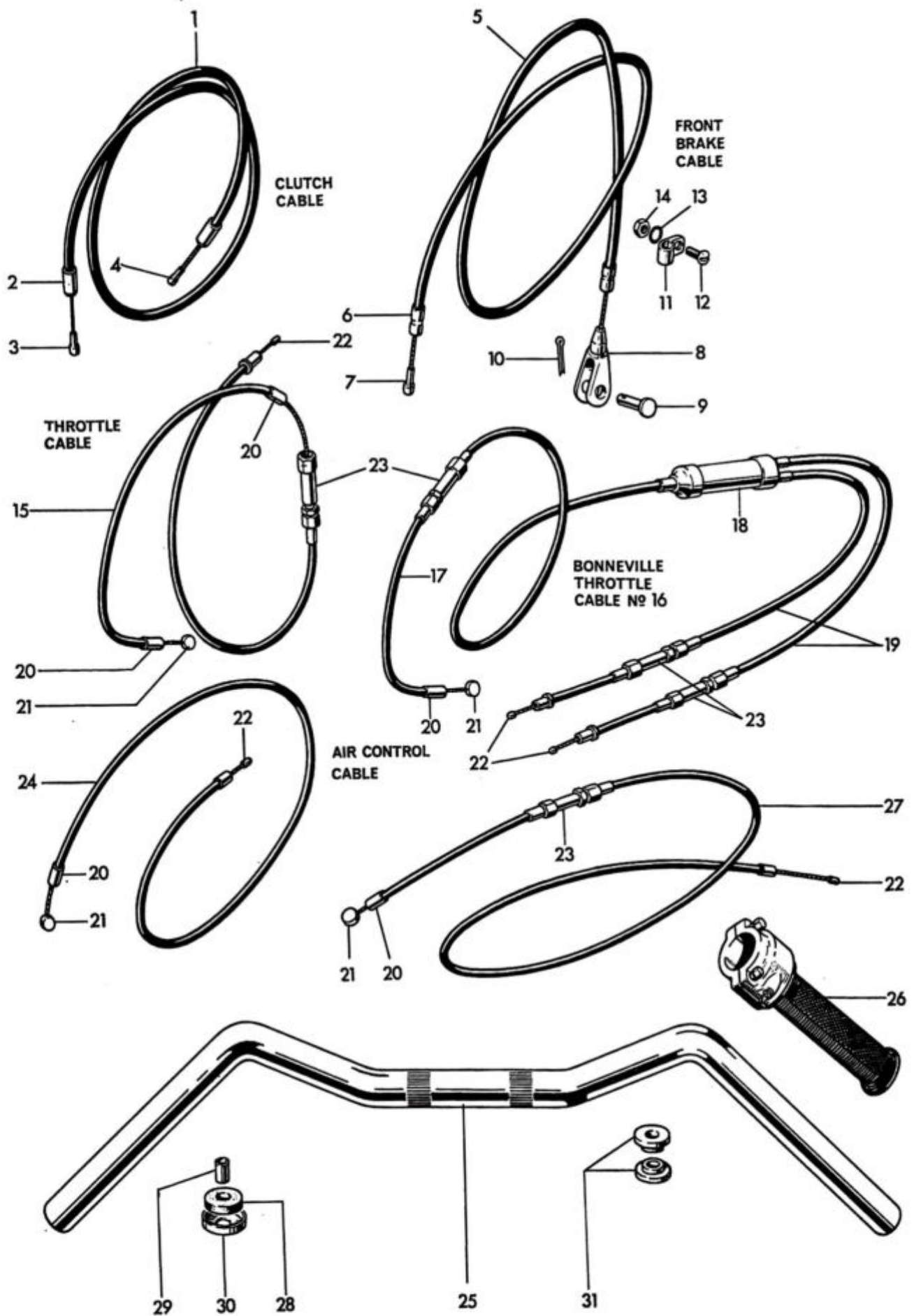
Fig. 28. CONTROL CABLES AND AMERICAN HANDLEBARS
