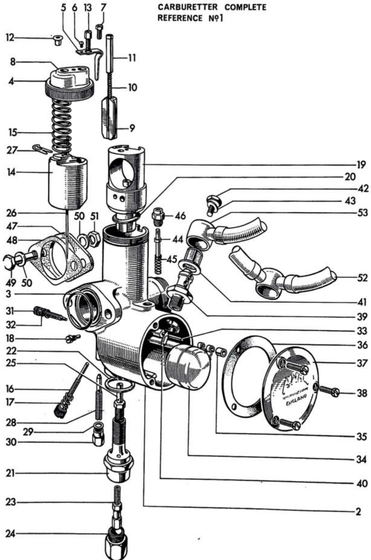
Fig. 31. AMAL CARBURETTER, TR6 AND T120
