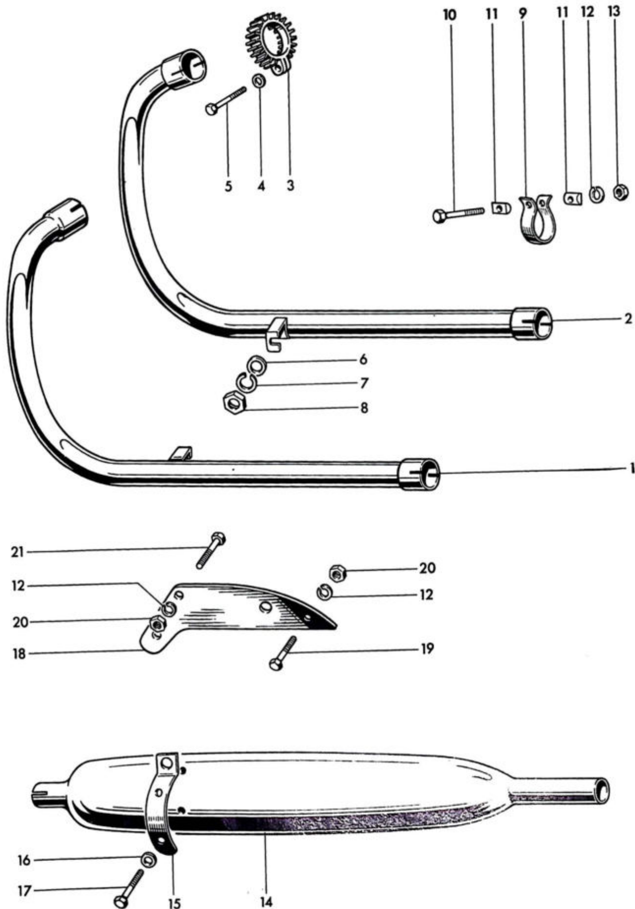
Fig. 15. EXHAUST PIPES AND SILENCERS
