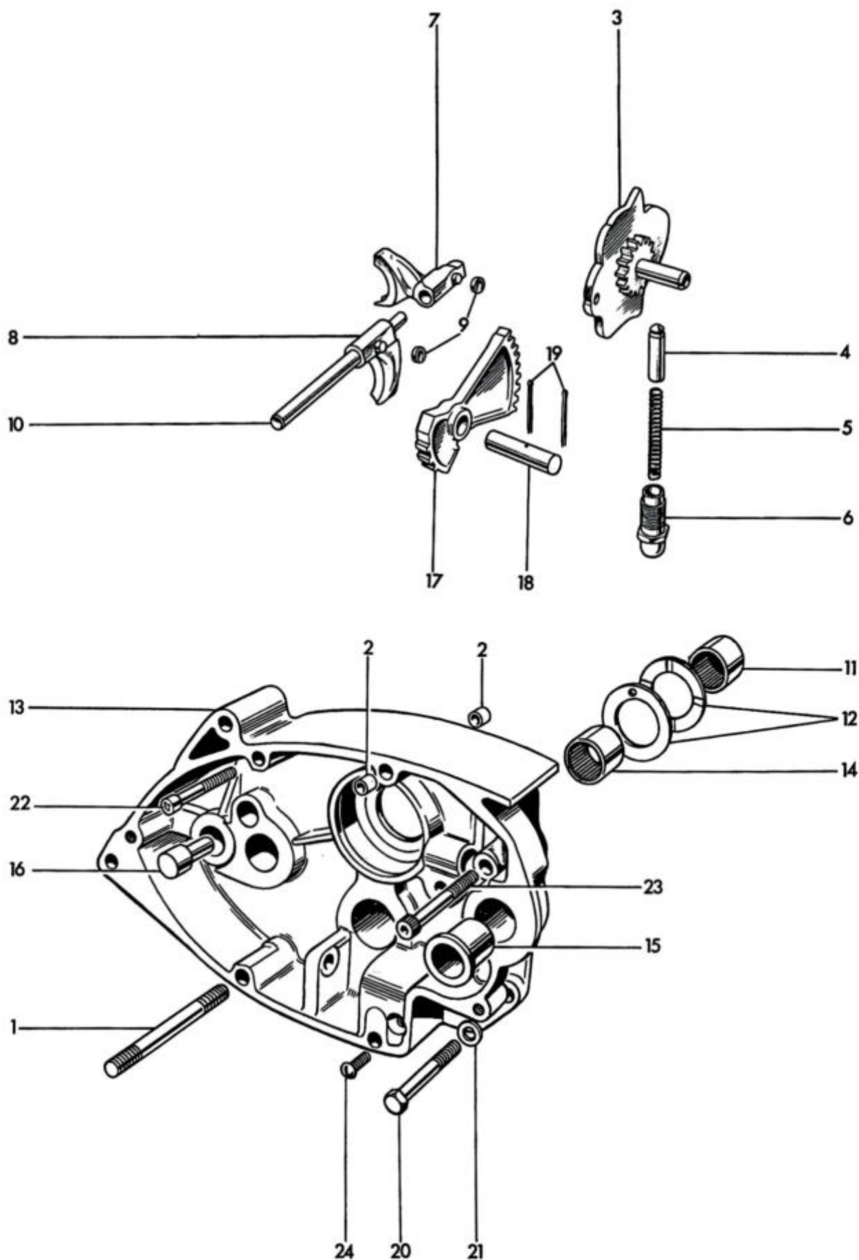
Fig. 7. GEARBOX INNER COVER AND SELECTORS
