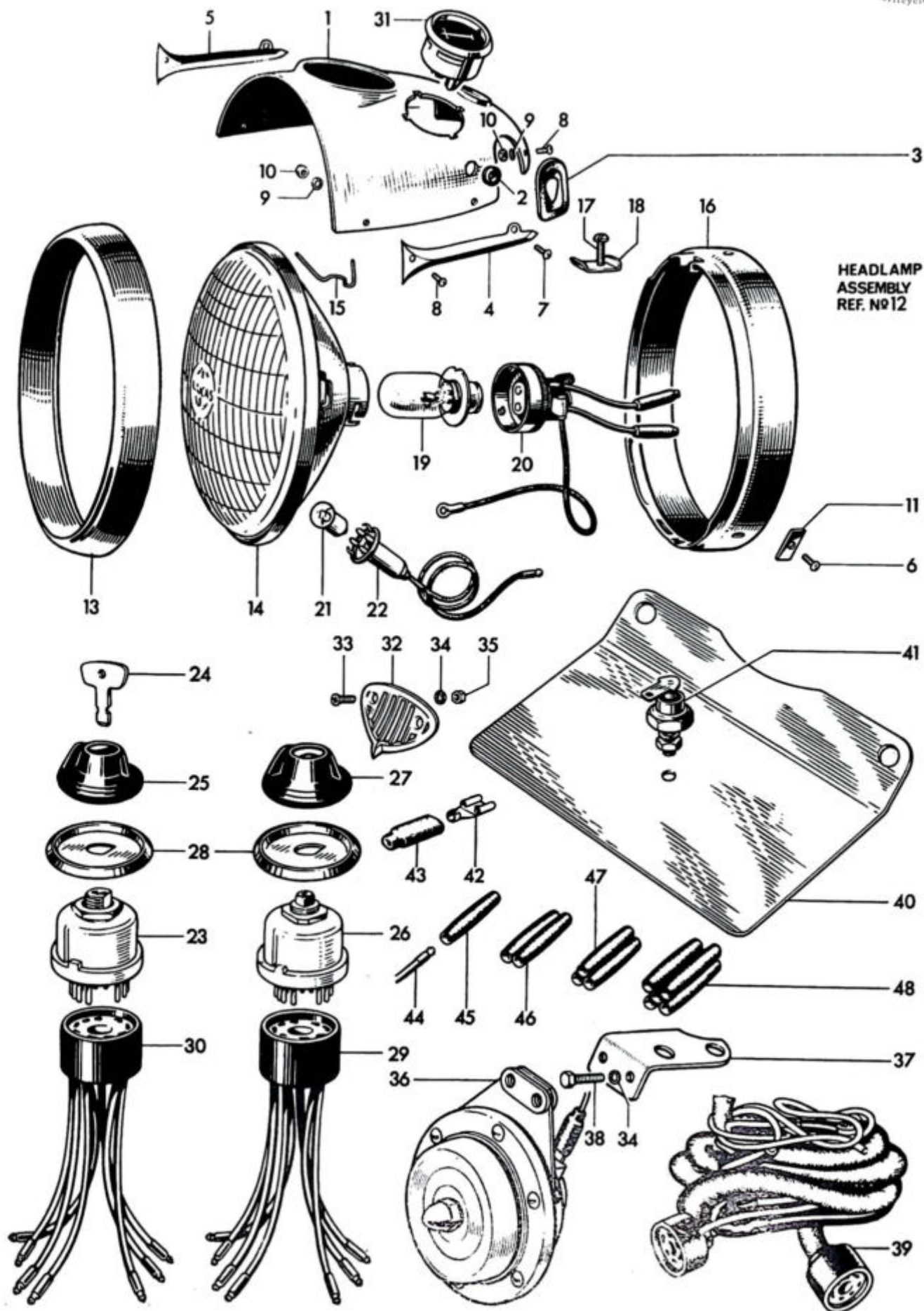
Fig. 17. NACELLE HEADLAMP AND SWITCHES
