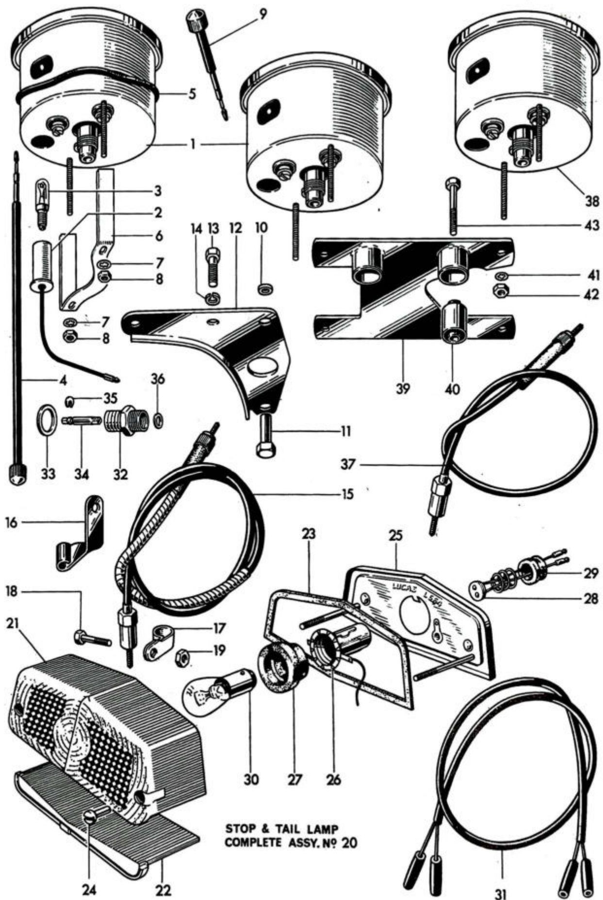
Fig. 33. SPEEDOMETER TACHOMETER AND TAIL LAMP
