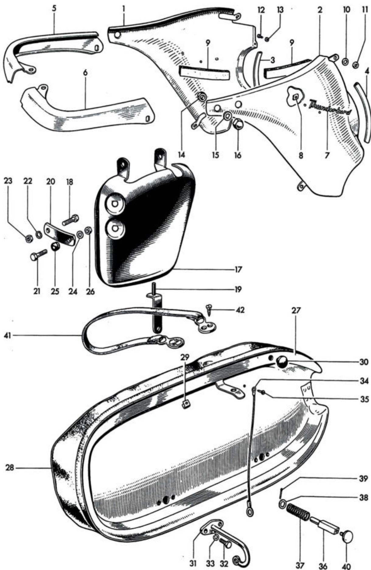
Fig. 25. PANELS AND TWINSEAT
