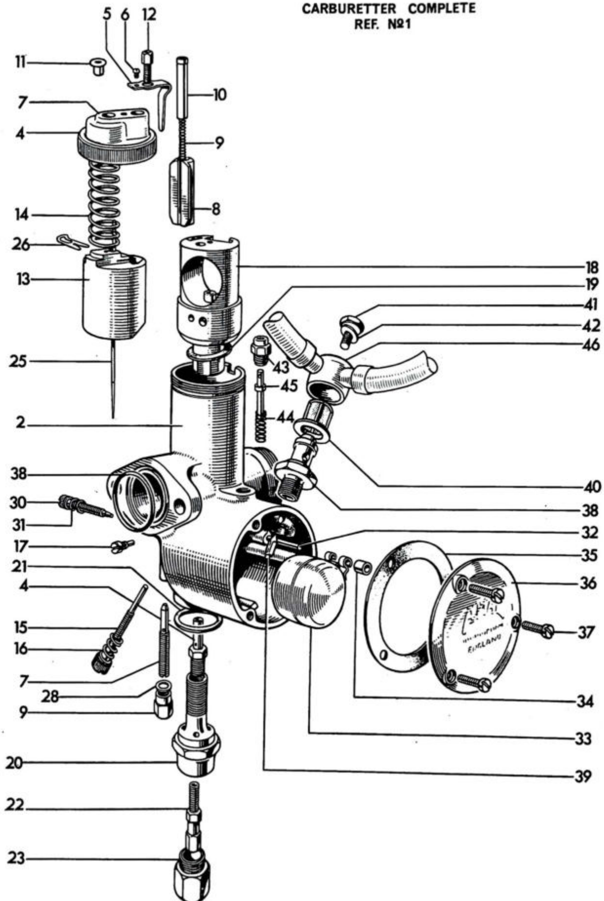
Fig. 30. AMAL CARBURETTER, 6T
