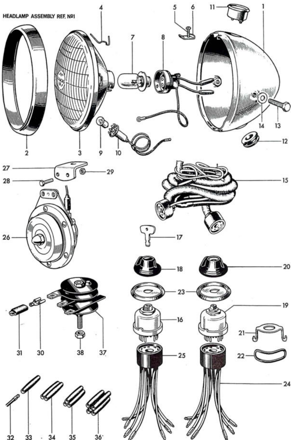
Fig. 32. HEADLAMP, WIRING HARNESS, HORN AND RECTIFIER
