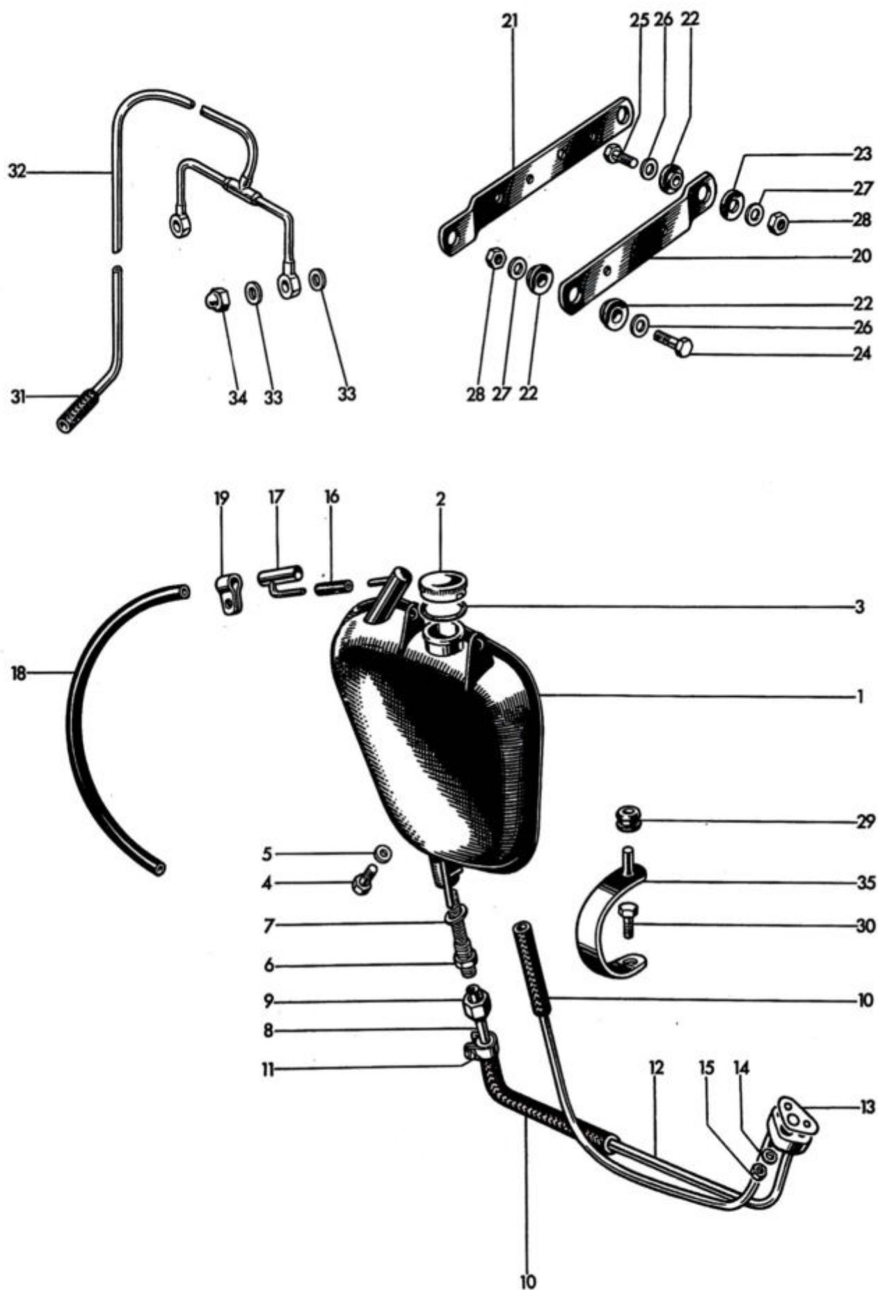
Fig. 23. OIL TANK
