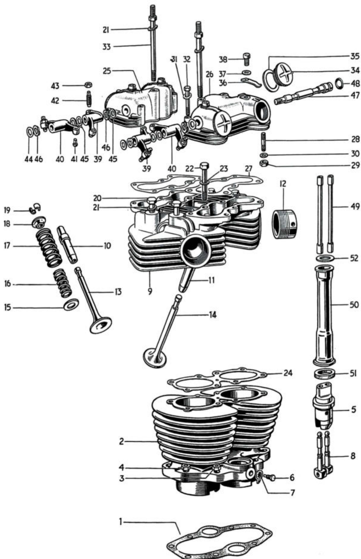
Fig. 4. CYLINDER BLOCK AND HEAD, 6T AND TR6
