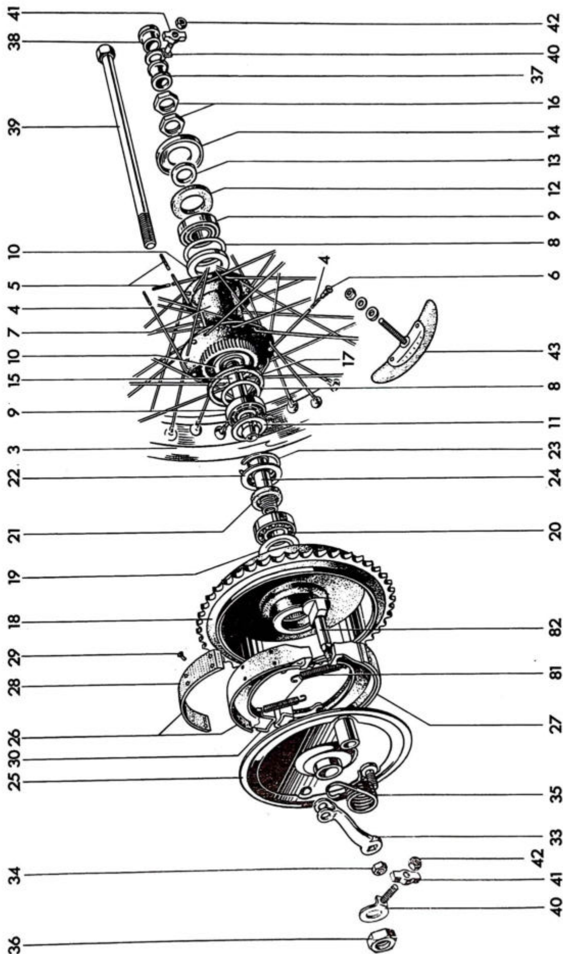
Fig. 21. QUICKLY DETACHABLE REAR WHEEL
