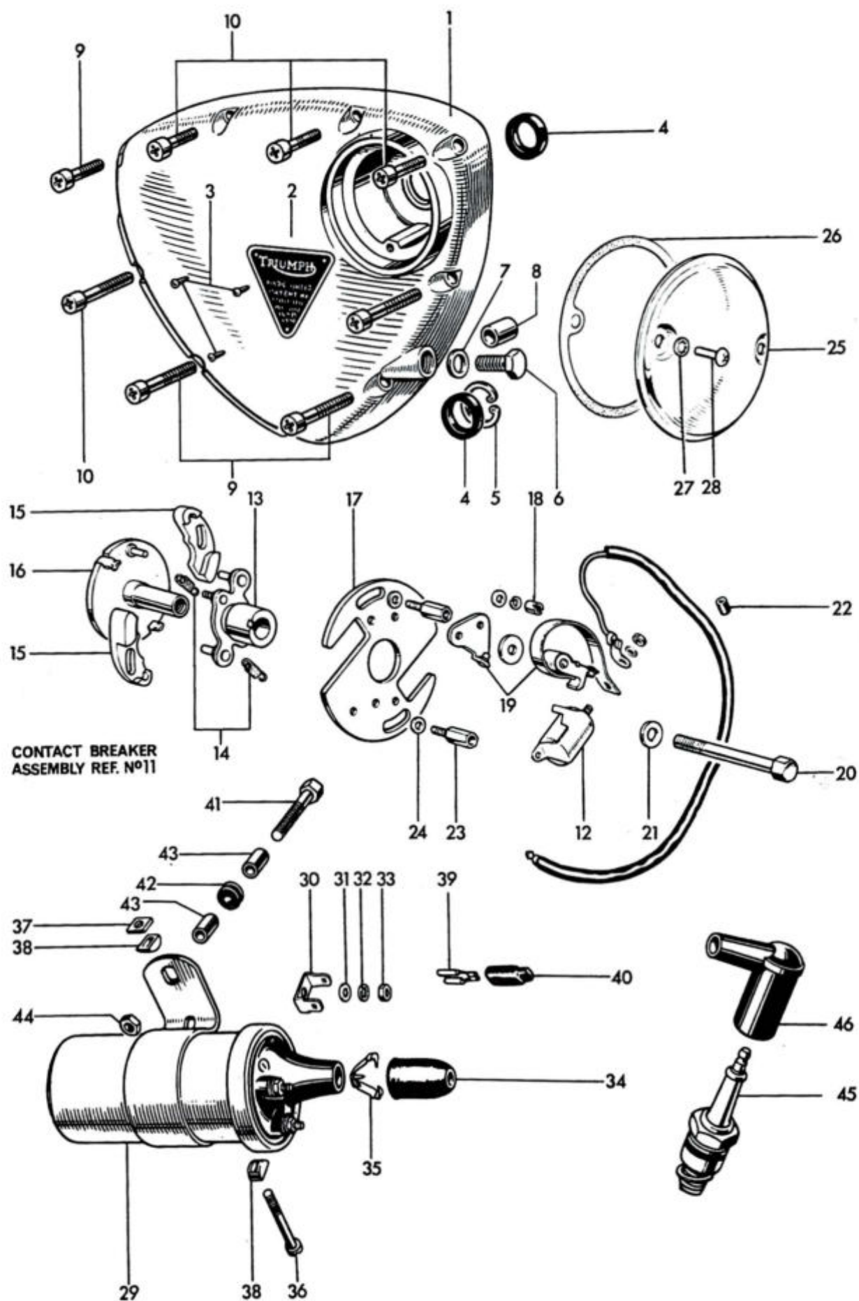
Fig. 6. TIMING COVER, CONTACT BREAKER AND COILS
