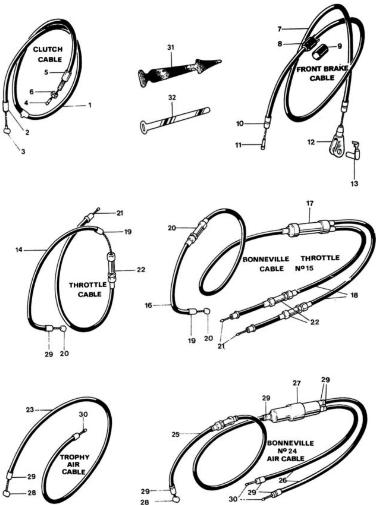
Fig. 27. CONTROL CABLES AND AMERICAN HANDLEBARS
