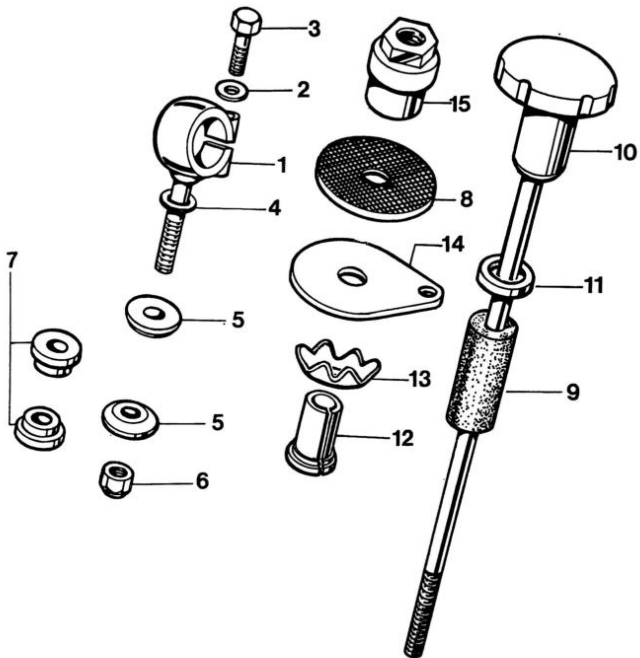
Fig. 17. HANDLEBAR MOUNTINGS AND STEERING DAMPER
