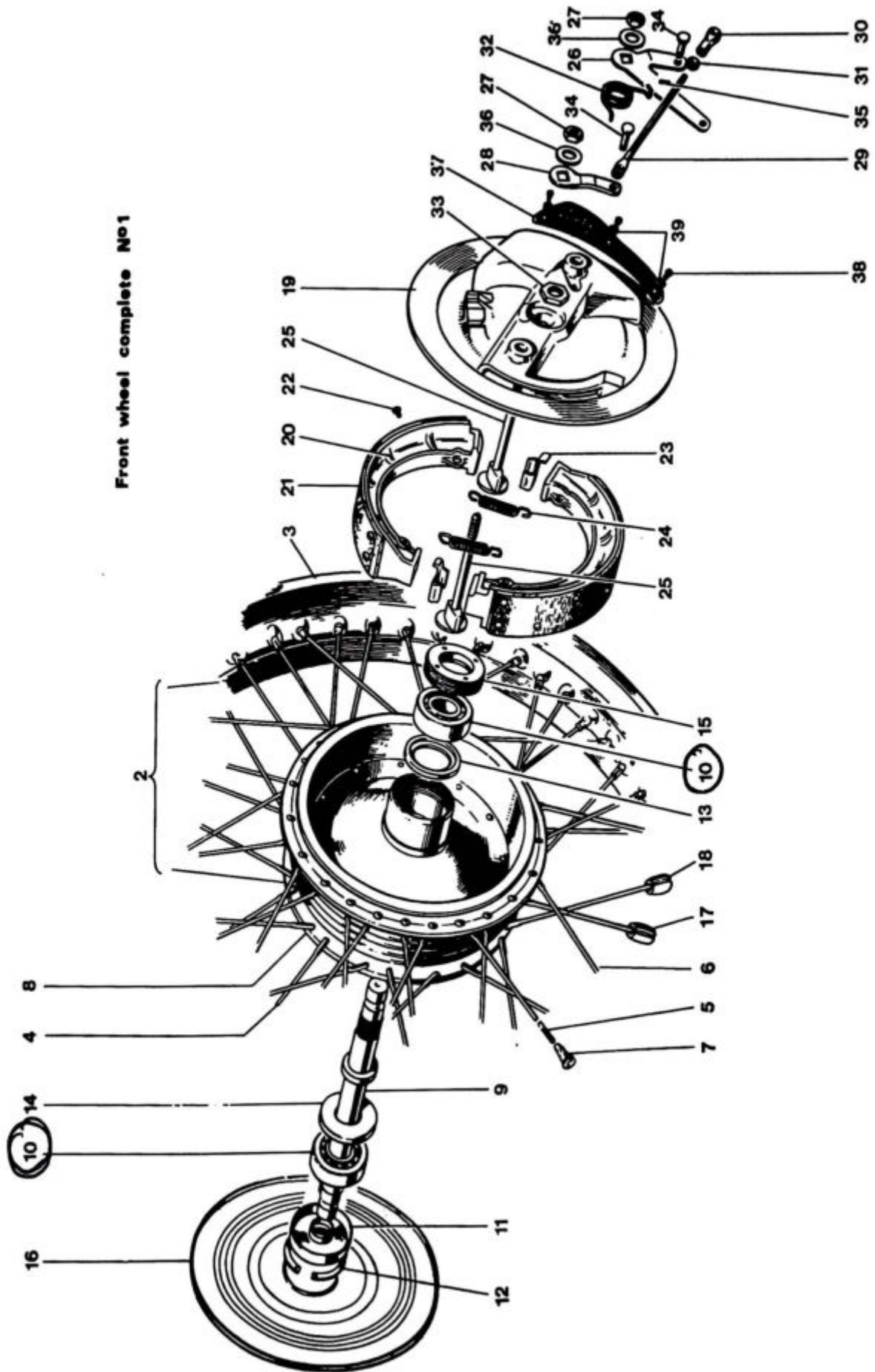
Fig. 19. FRONT WHEEL
