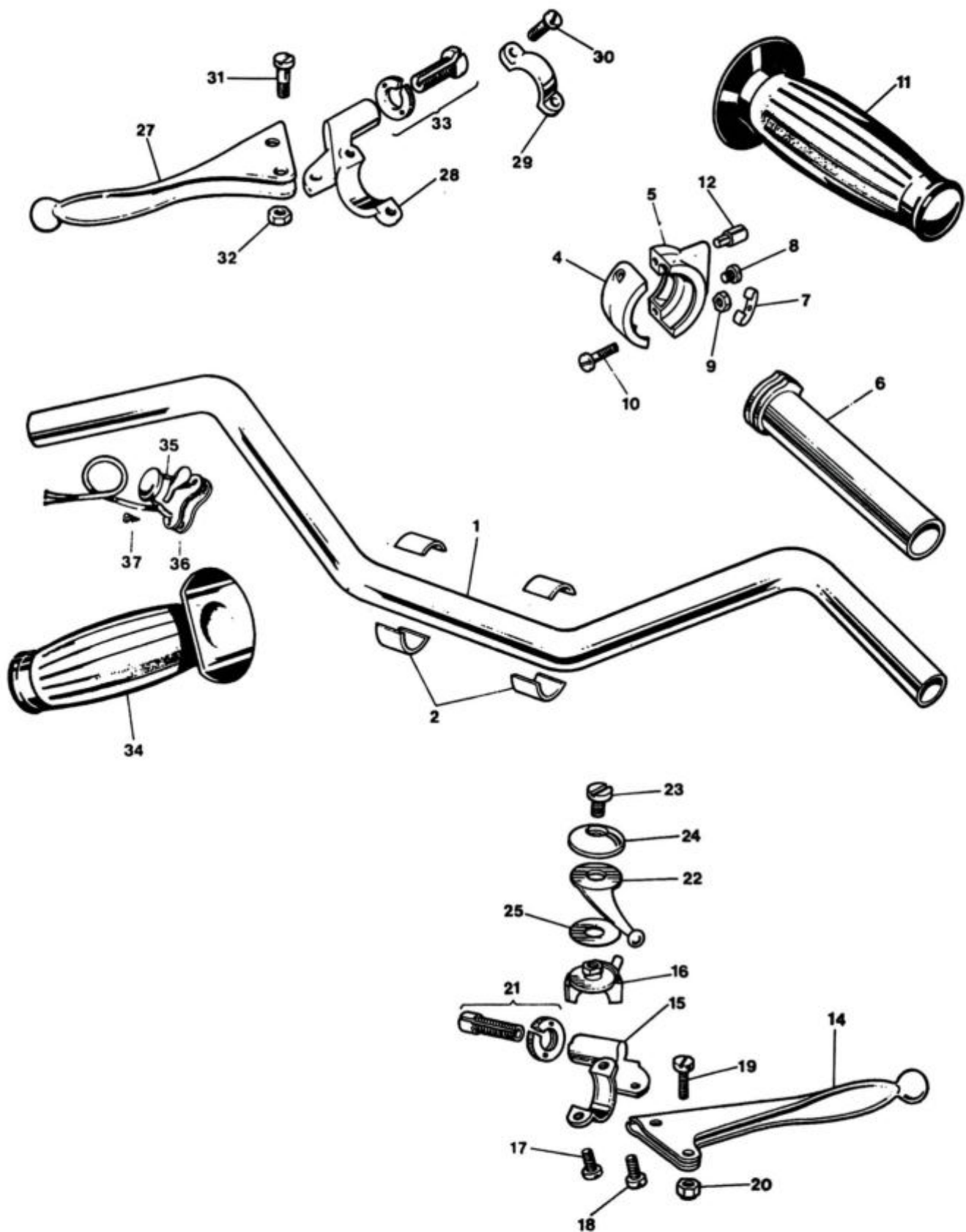
Fig. 2f. HANDLEBARS AND CONTROL LEVERS
