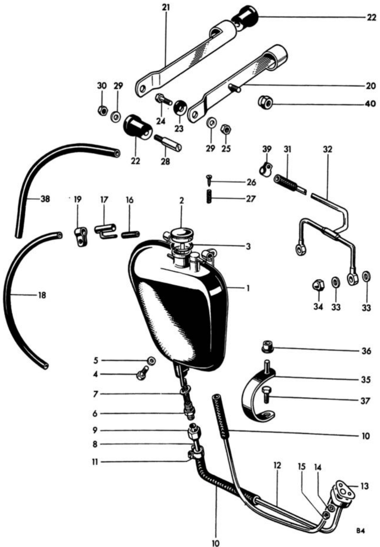
Fig. 23. OIL TANK
