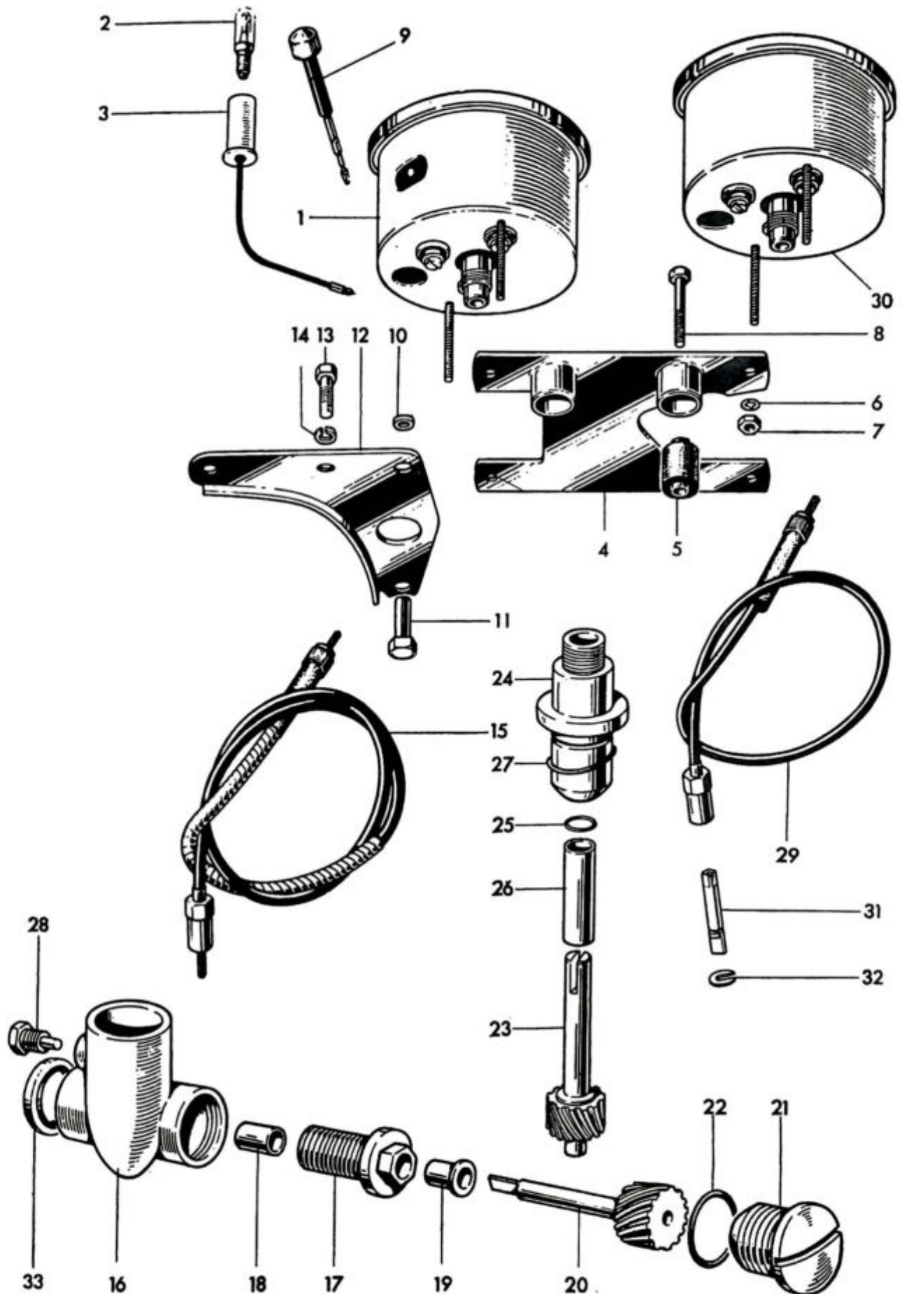
Fig. 31. SPEEDOMETER AND TACHOMETER
