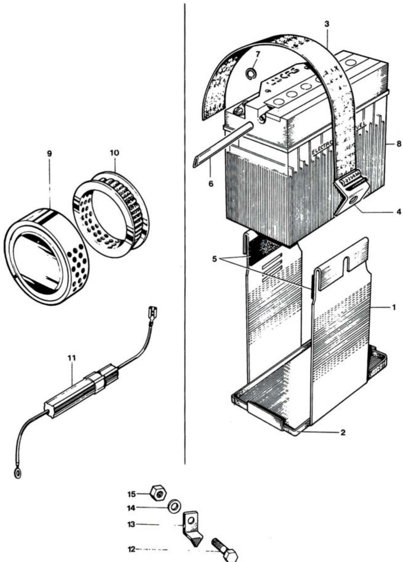
Fig. 23. BATTERY CARRIER AND AIR FILTERS
