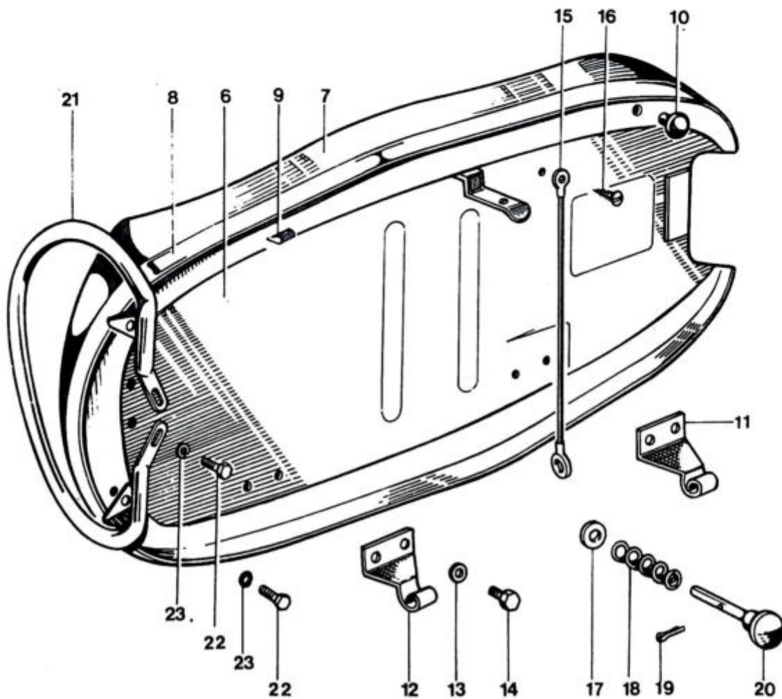
Fig. 24. PANEL AND TWINSEAT
