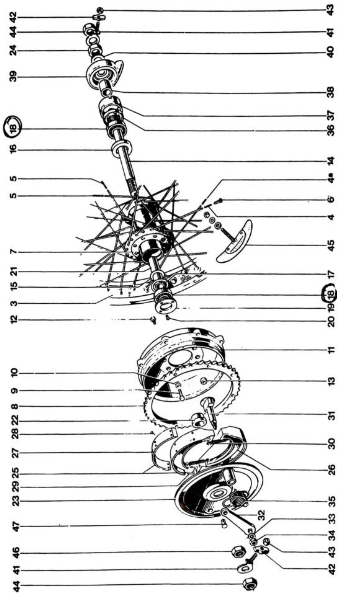
Fig. 19. REAR WHEEL
