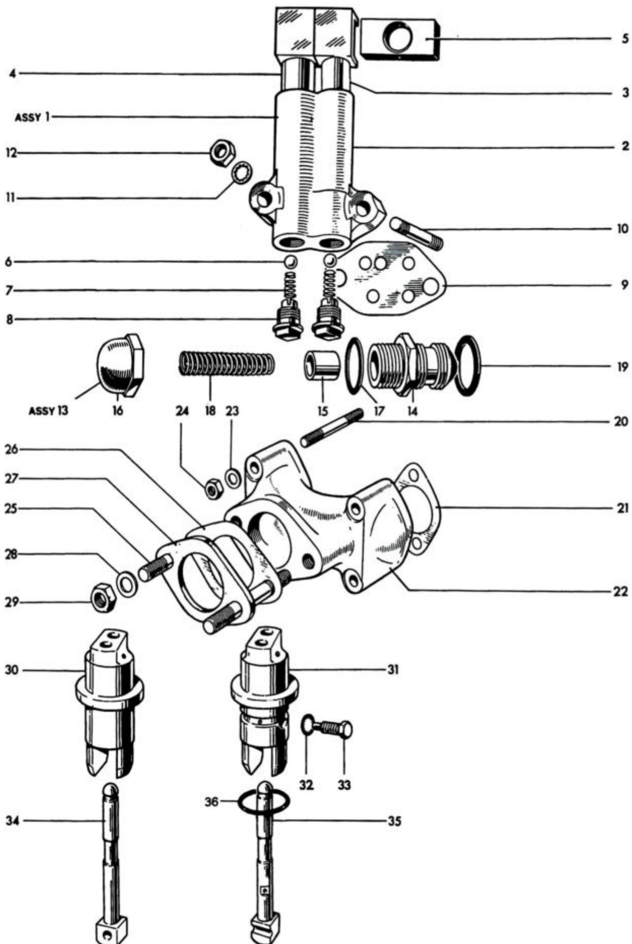
Fig. 3. OIL PUMP, RELEASE VALVE, MANIFOLD AND TAPPETS
