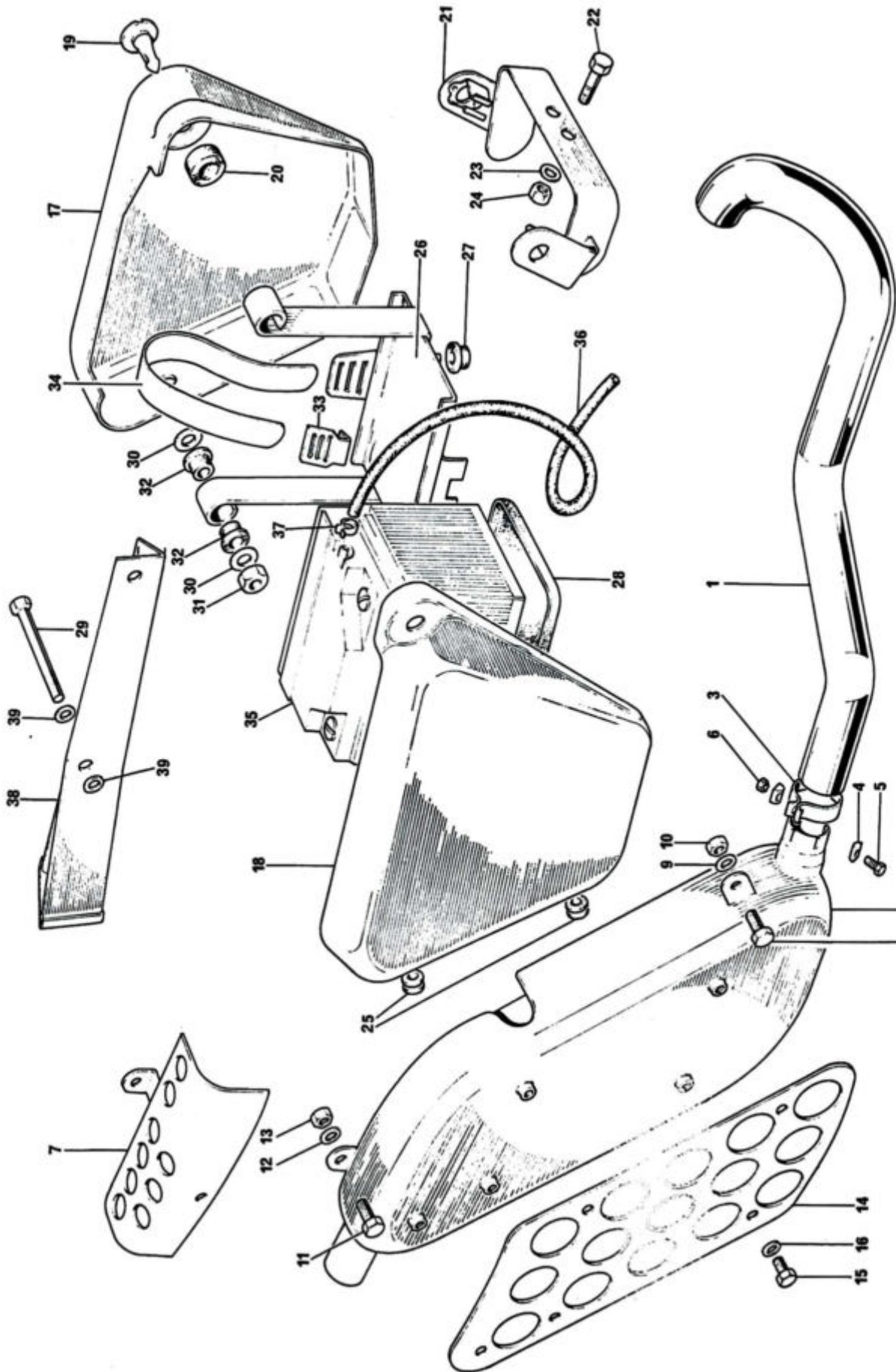
FIG. 7. EXHAUST SYSTEM, SIDE COVERS AND BATTERY
