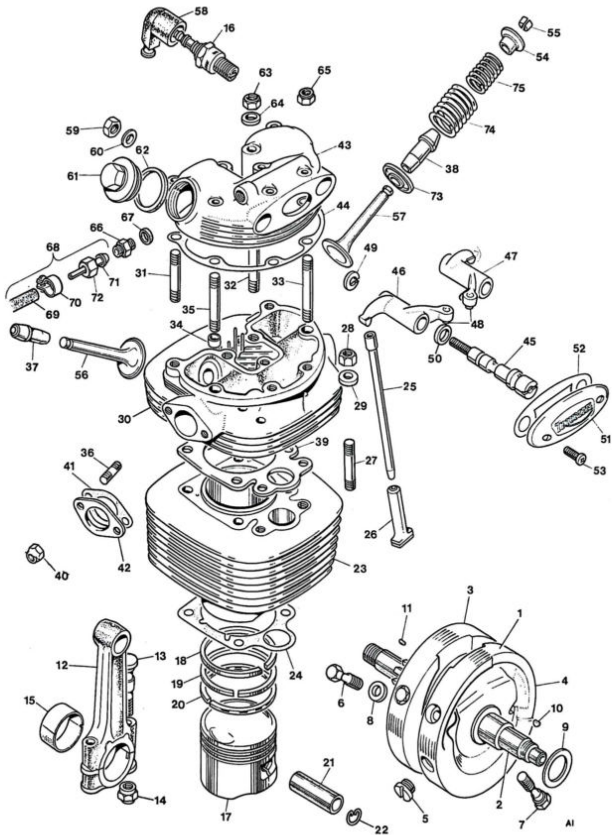
Fig. 1. CYLINDER HEAD, BARREL AND CRANKSHAFT
