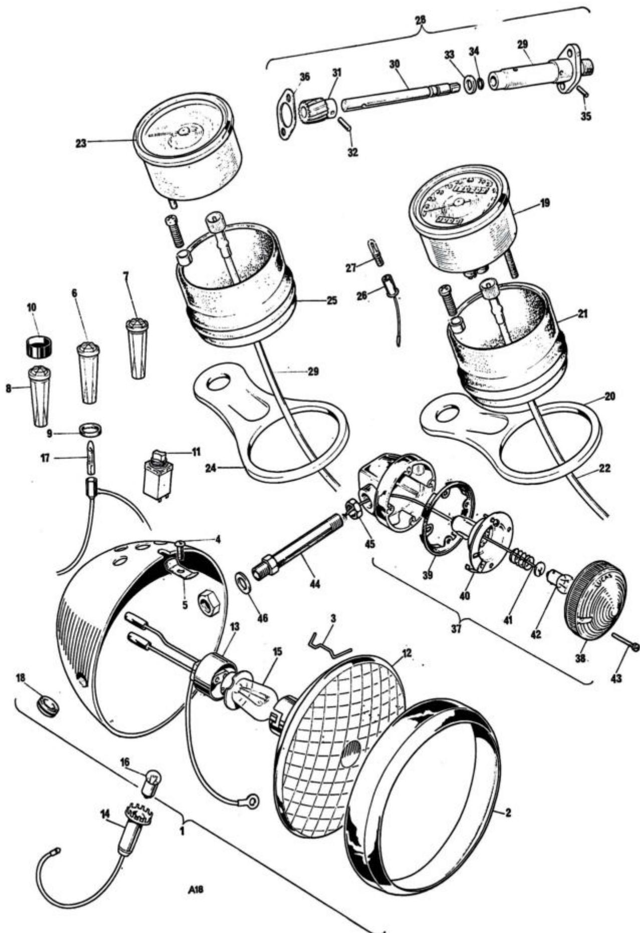
Fig. 18. HEADLAMP, SPEEDOMETER, TACHOMETER
