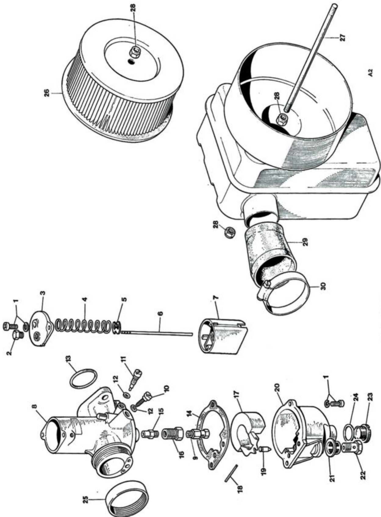
Fig. 2. CARBURETOR AND AIR CLEANER
