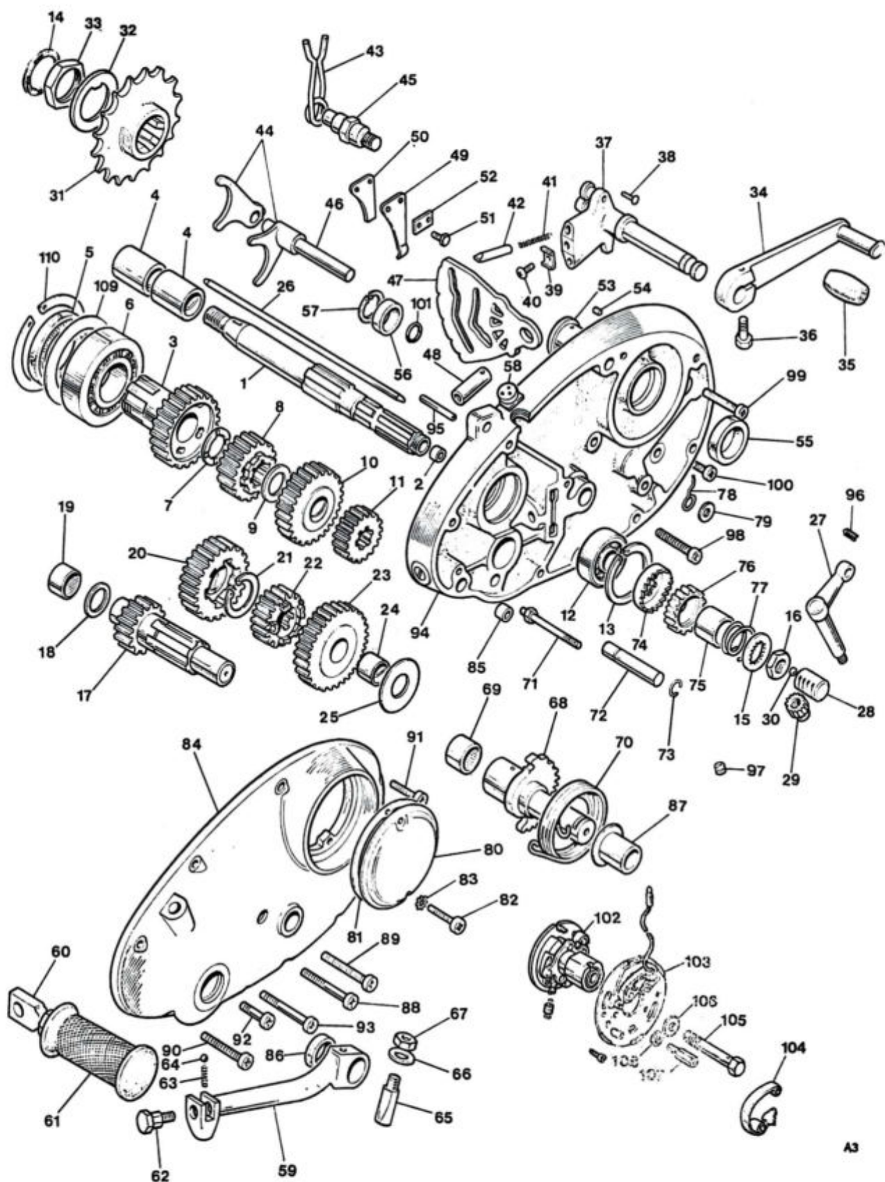
Fig. 4. GEAR CLUSTERS AND TIMING COVERS
