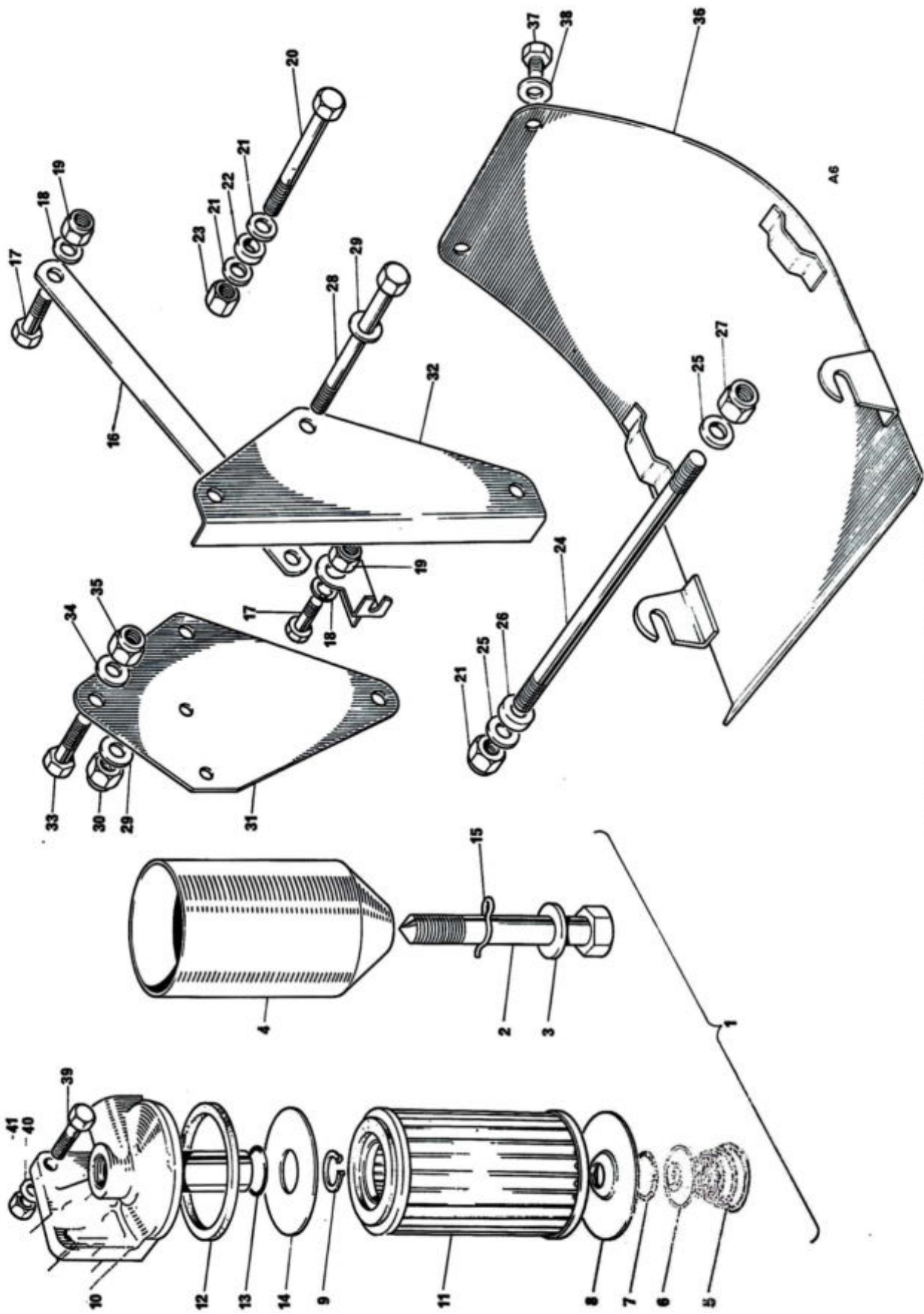
Fig. 6. OIL FILTER, MOTOR FIXINGS
