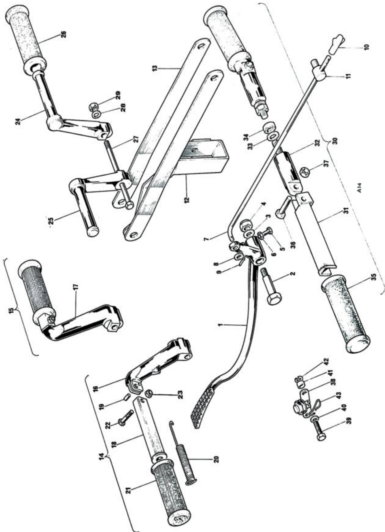
Fig. 14. BRAKE PEDAL AND FOOTRESTS
