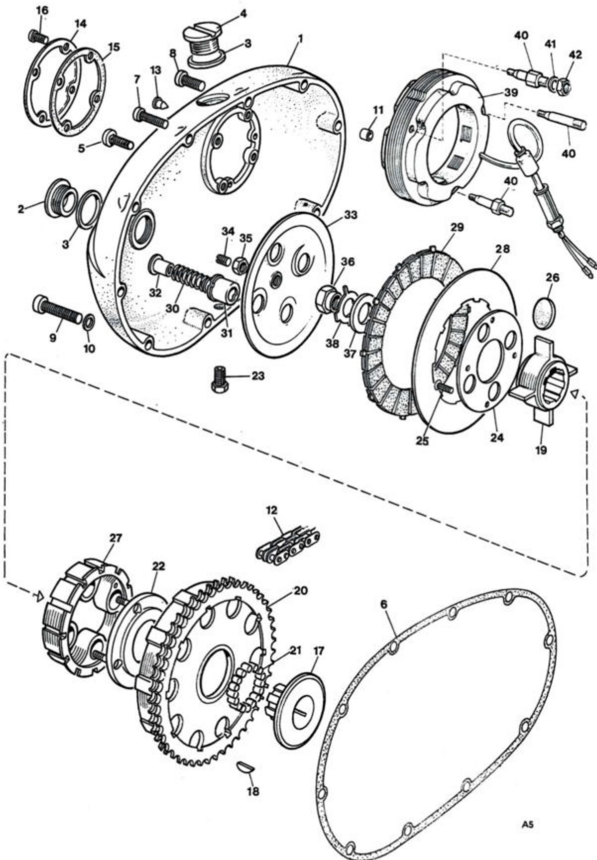
Fig. 5. CLUTCH AND PRIMARY CHAINCASE
