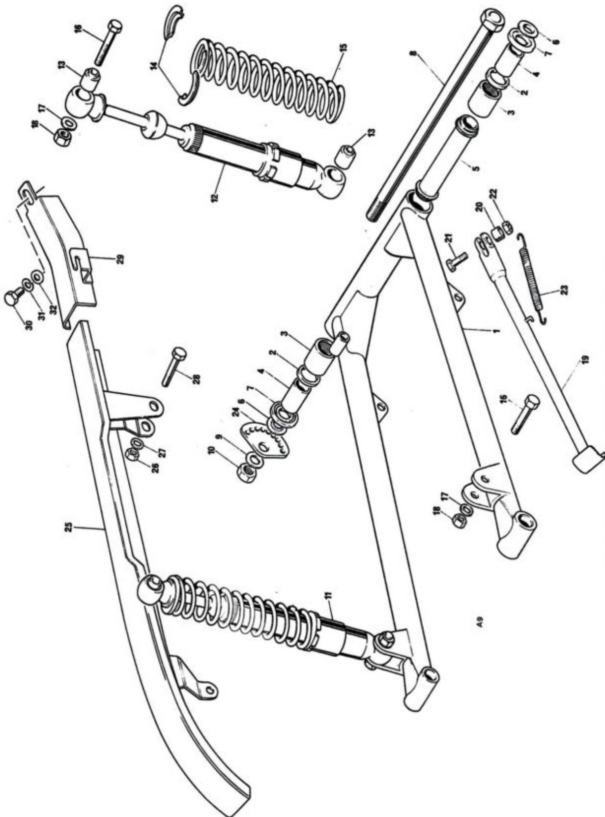
Fig. 9. SWINGING ARM AND SUSPENSION UNITS
