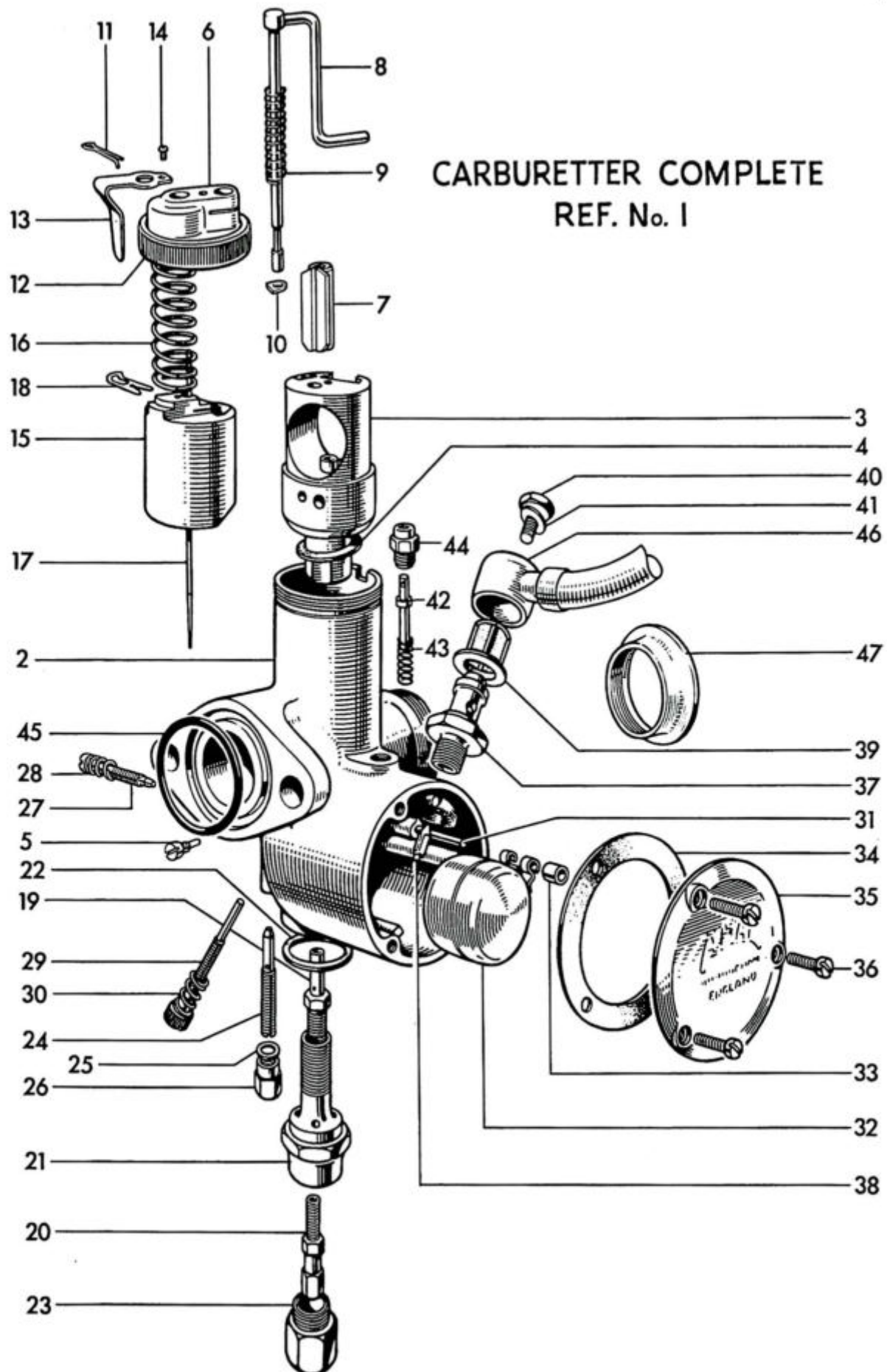
Fig. 27. CARBURETTER, T90 AND T100SS
