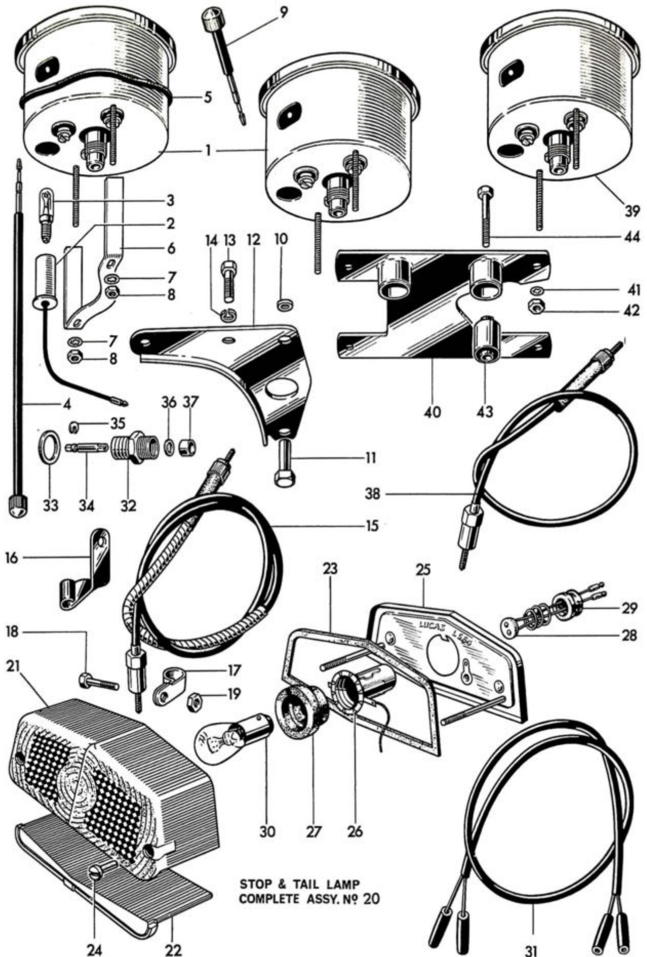
Fig. 29. SPEEDOMETER, TACHOMETER AND TAIL LAMP
