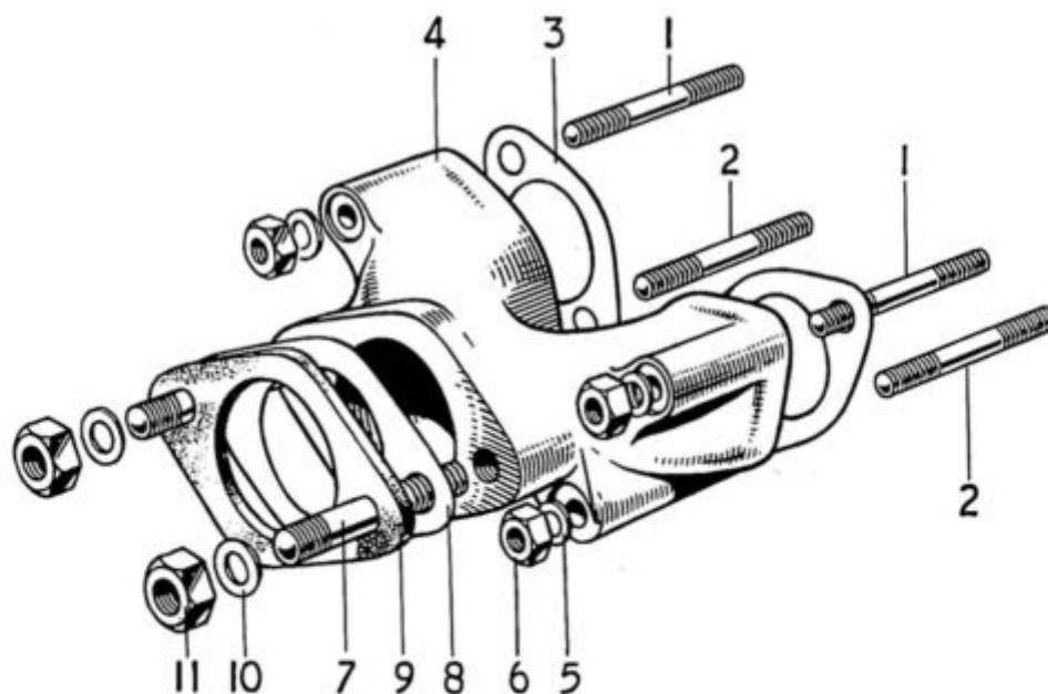
Fig. 3. OIL PUMP, RELEASE VALVE AND INLET MANIFOLD
