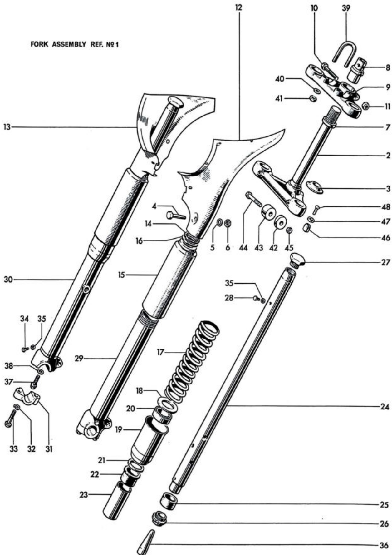
Fig. 14. TELESCOPIC FRONT FORK, 3TA AND 5TA
