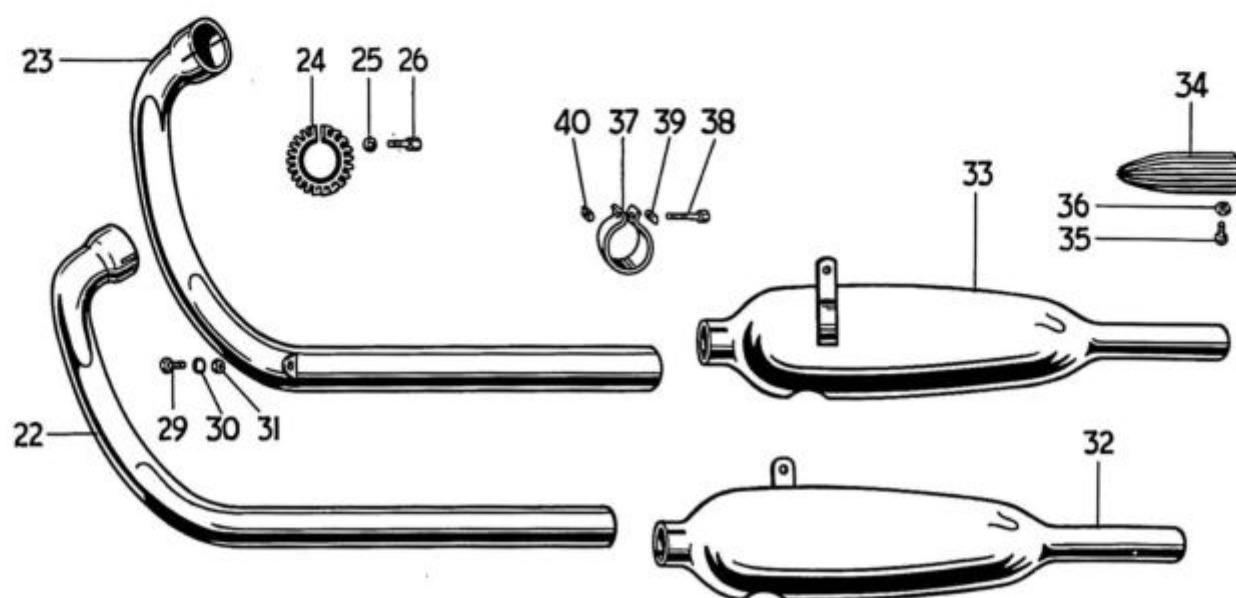
Fig. 11. ENGINE FITTINGS AND EXHAUST SYSTEM
