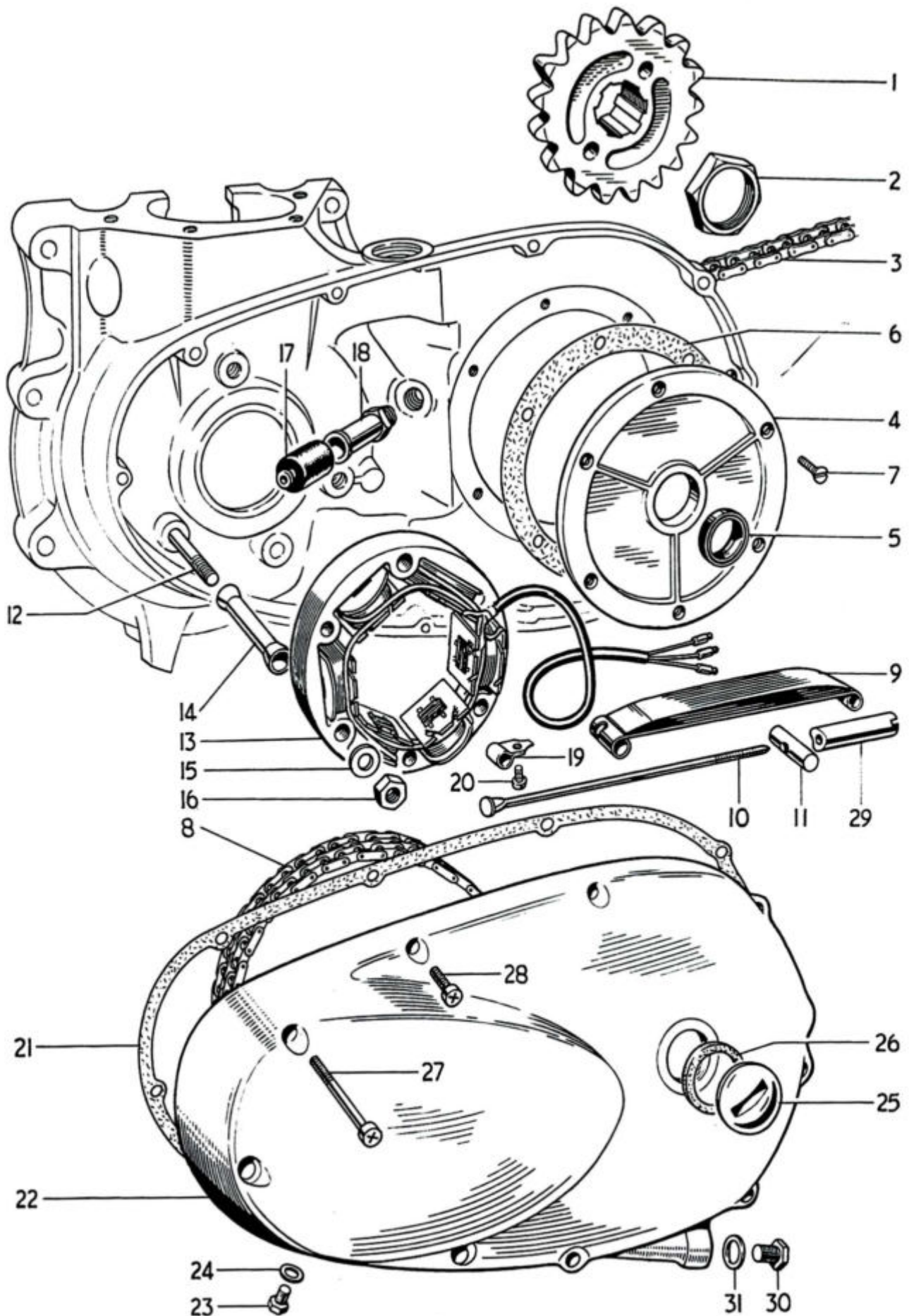
Fig. 10. CHAINCASE AND CHAINS
