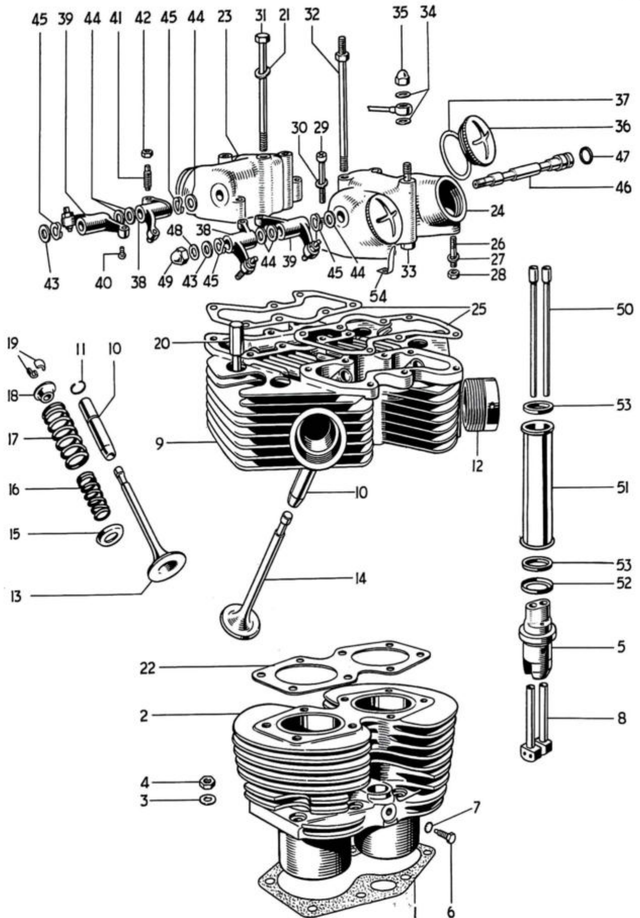
Fig. 5. CYLINDER BLOCK AND HEAD, 5TA AND T100SS
