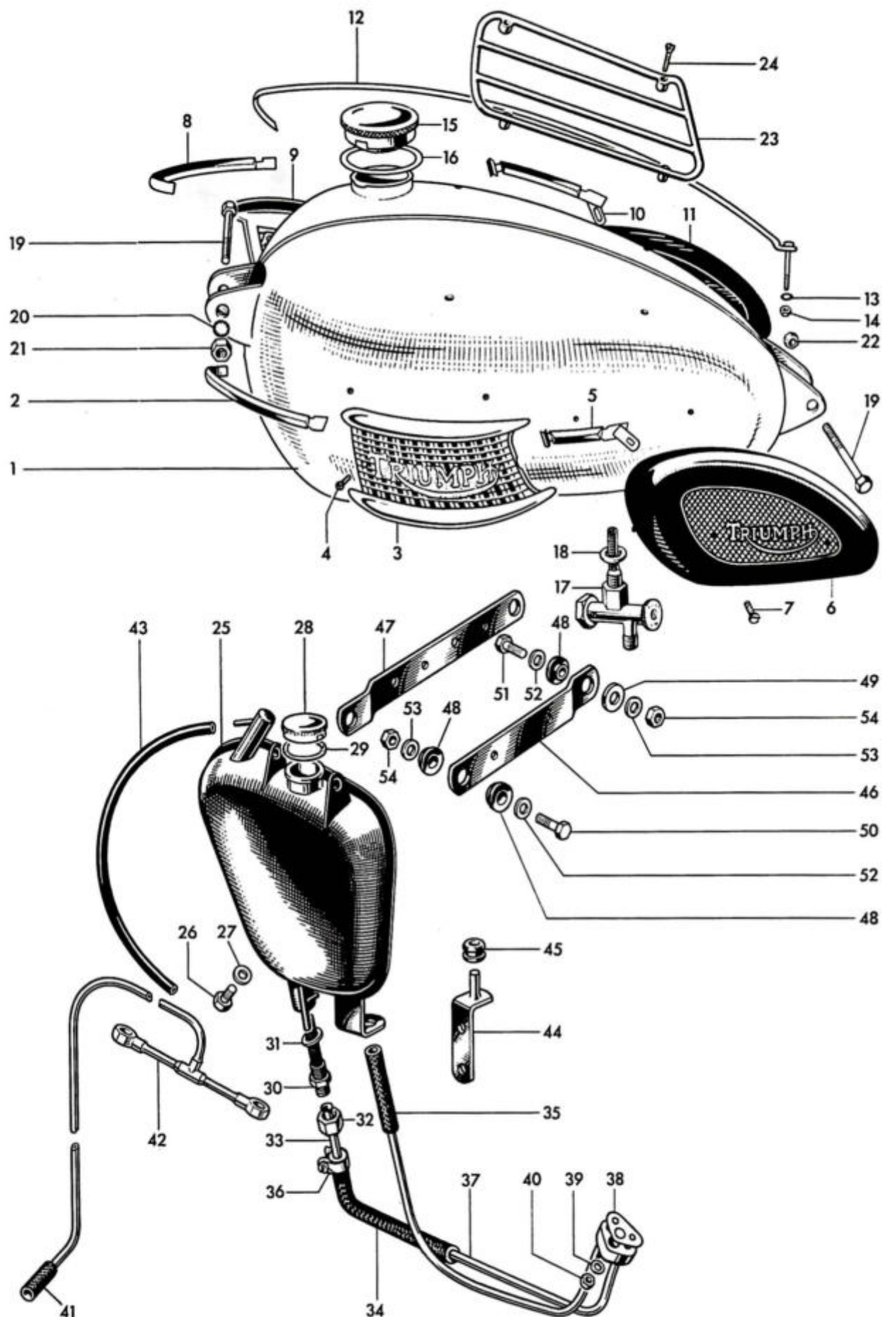
Fig. 22. PETROL AND OIL TANKS.
