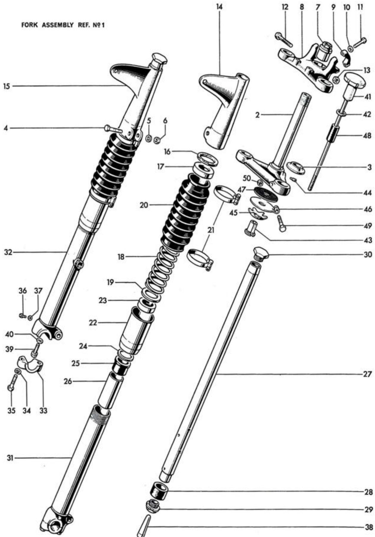
Fig. 16. TELESCOPIC FRONT FORK, T90 AND T100SS
