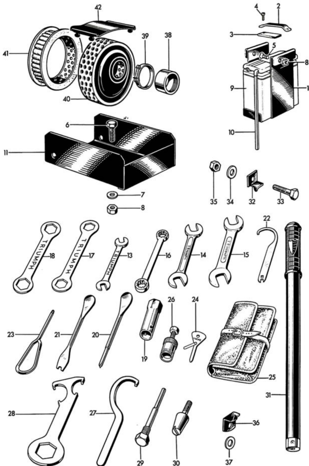
Fig. 23. BATTERY, TOOLKIT AND AIR FILTER
