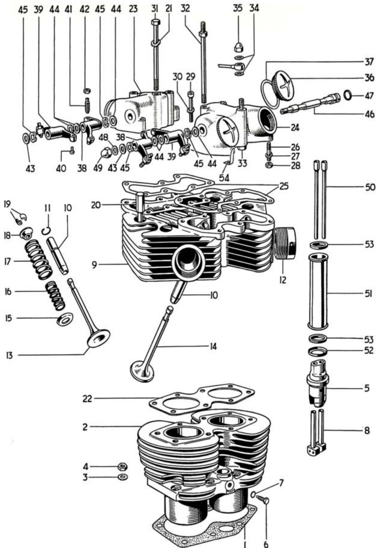
Fig. 4. CYLINDER BLOCK AND HEAD, 3TA AND T90
