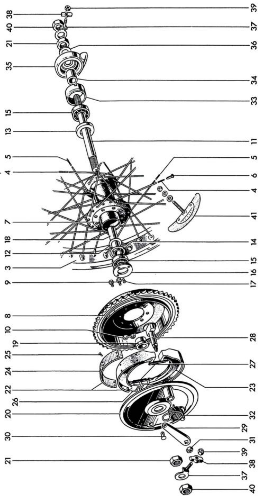
Fig. 18. REAR WHEEL
