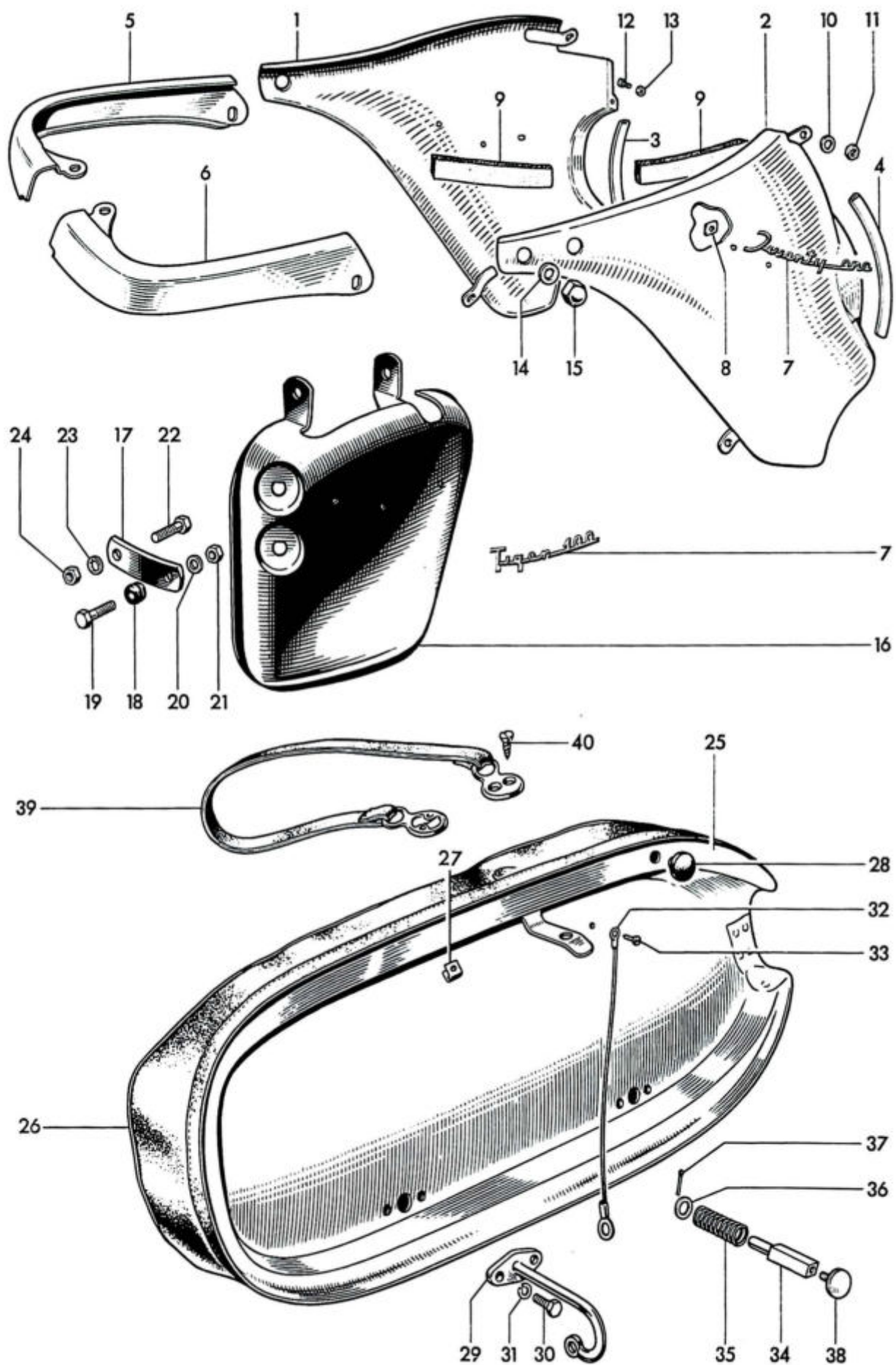
Fig. 21. PANELS AND TWINSEAT
