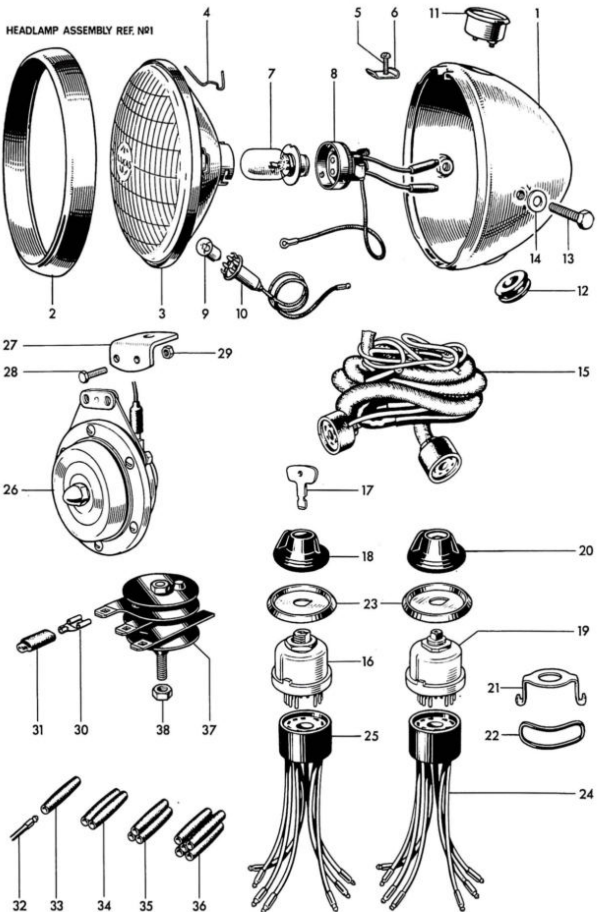
Fig. 28. T90 AND T100SS HEADLAMP, WIRING HARNESS AND SWITCHES
