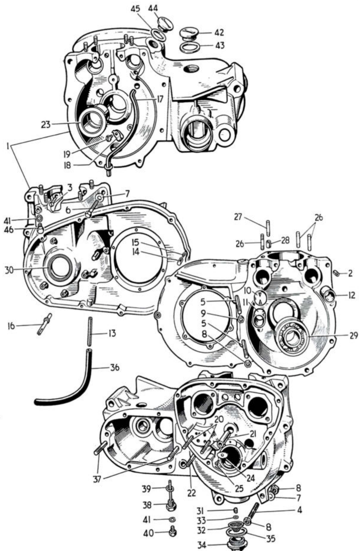
Fig 2. CRANKCASE
