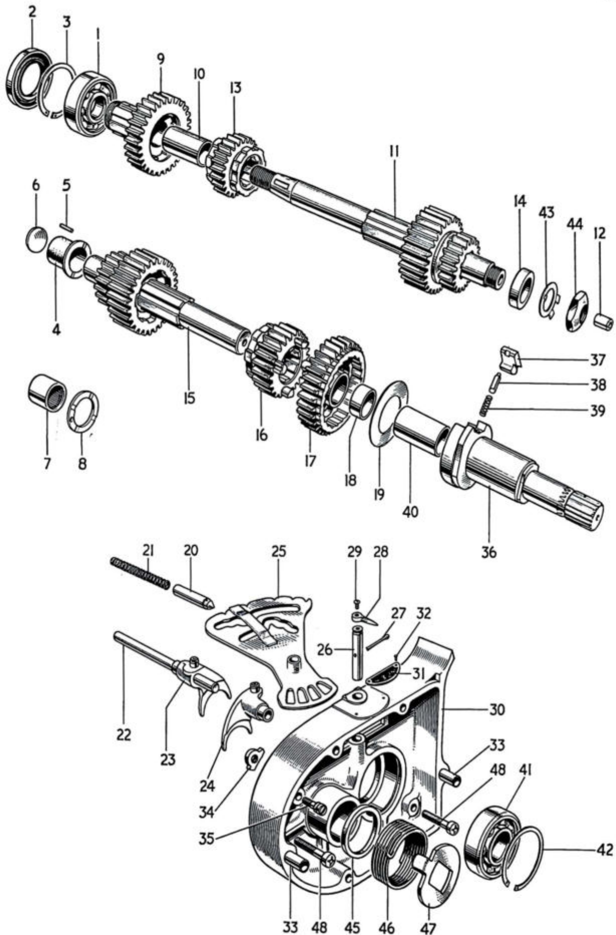
Fig. 7. GEARBOX SHAFTS, BEARINGS AND INNER COVER
