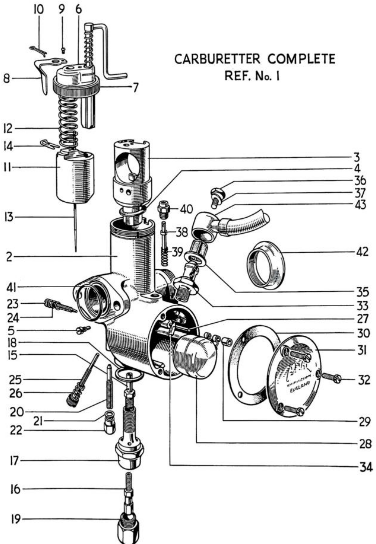
Fig. 26. CARBURETTER, 3TA AND 5TA
