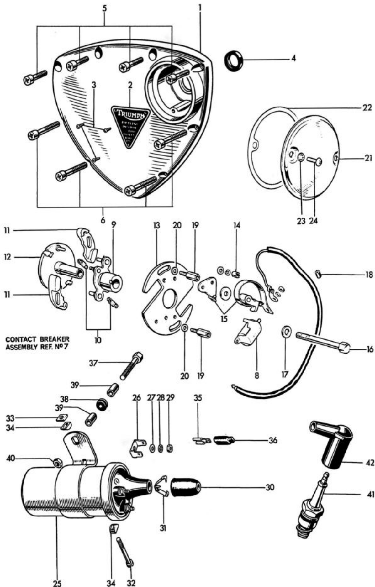
Fig. 6. TIMING COVER, CONTACT BREAKER AND COILS
