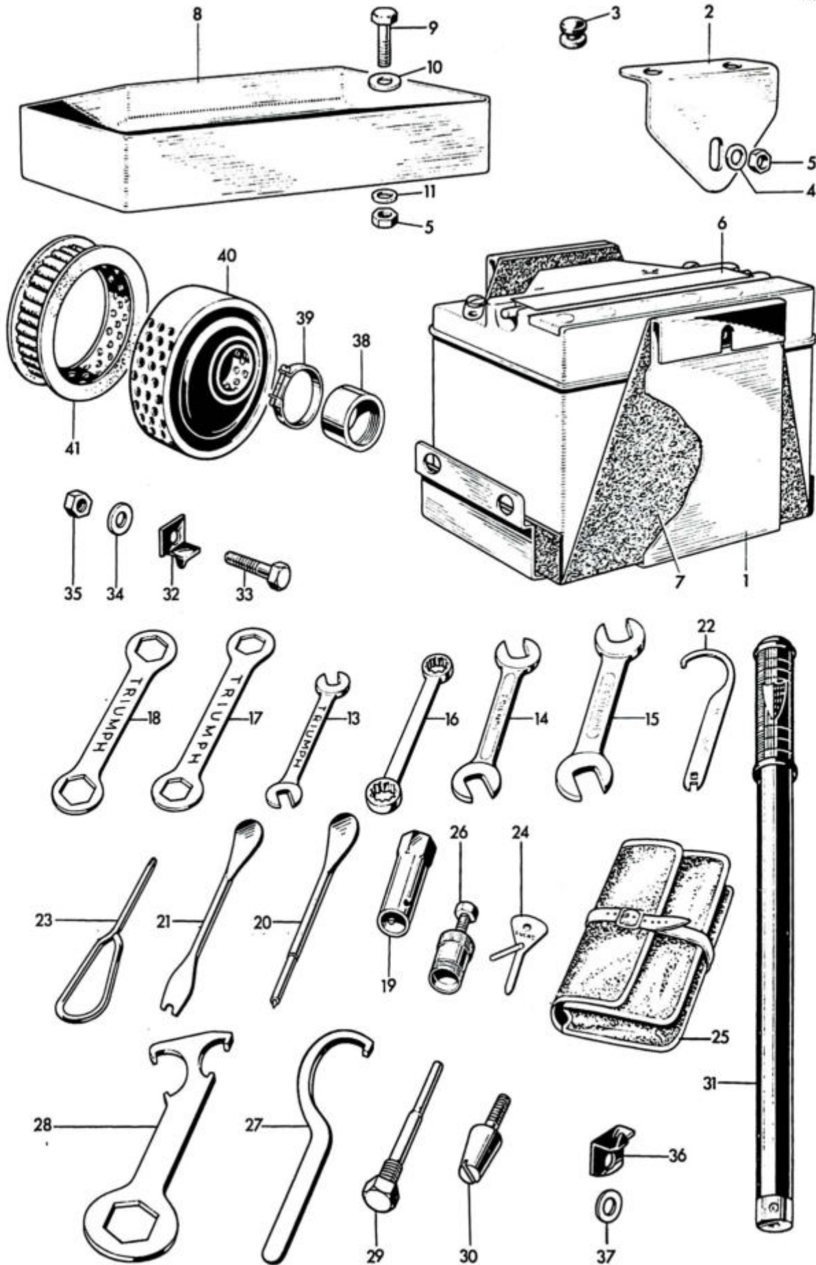
Fig. 27. BATTERY, TOOLKIT AND AIR FILTER
