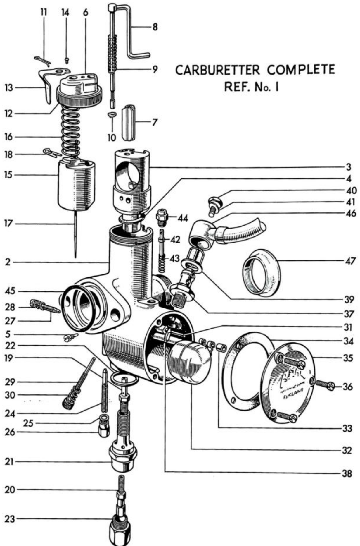
Fig. 31. CARBURETTER, T90 AND T100
