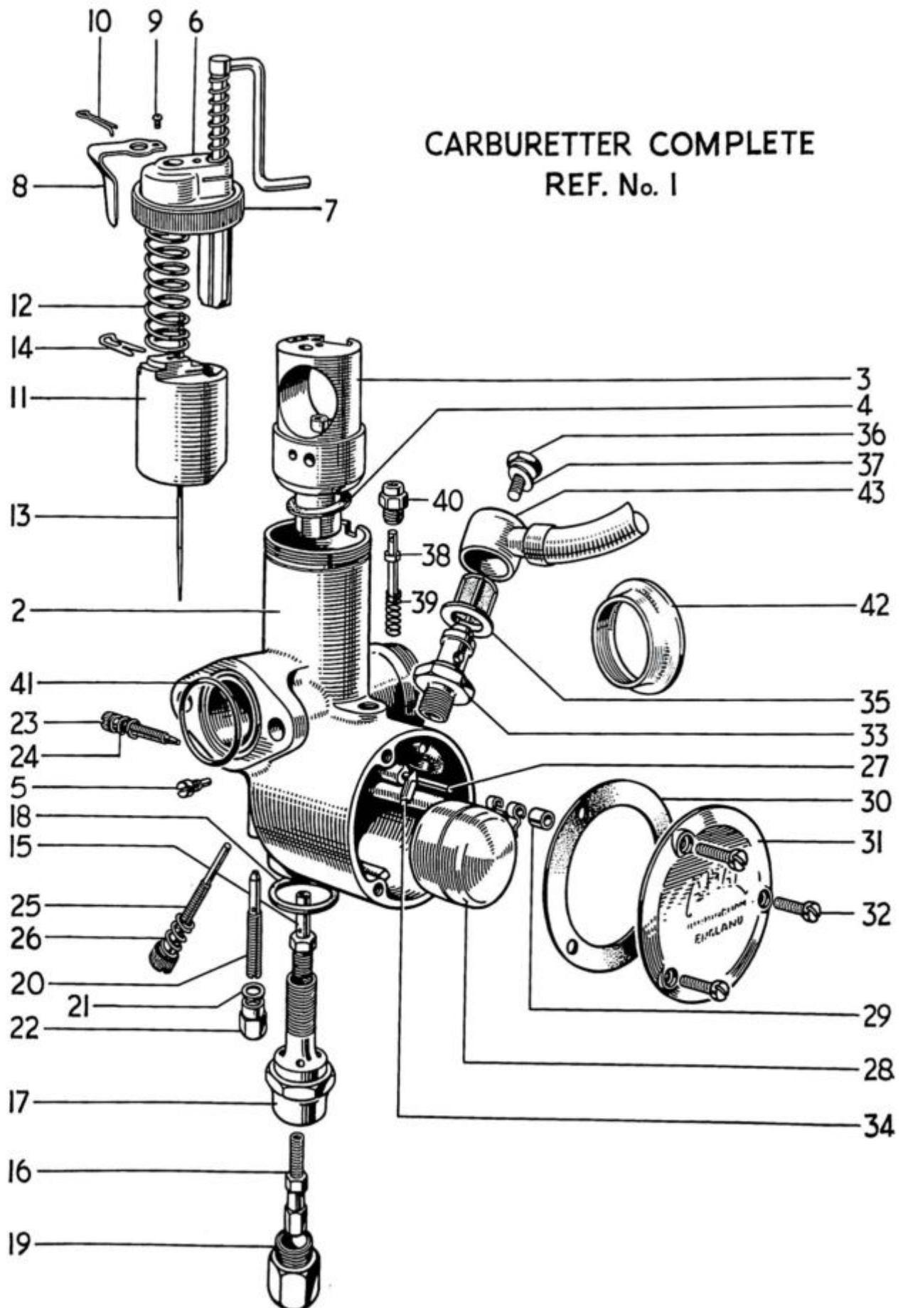
Fig. 30. CARBURETTER, 3TA AND 5TA
