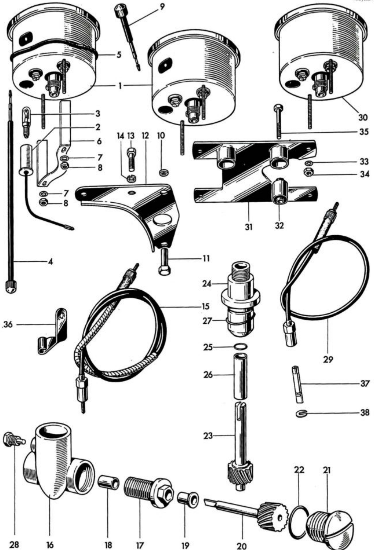
Fig. 35. SPEEDOMETER AND TACHOMETER
