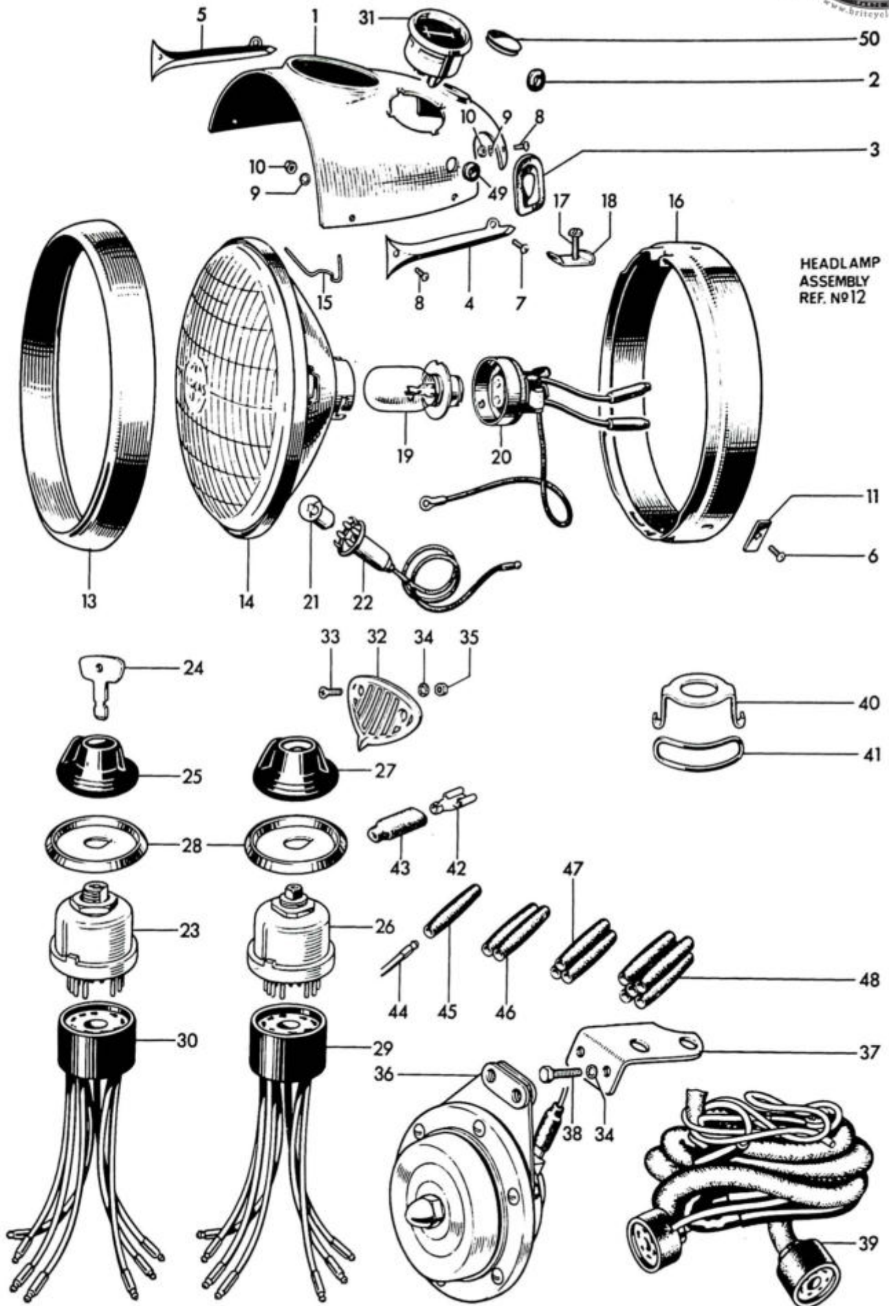
Fig. 16. NACELLE, HEADLAMP AND SWITCHES
