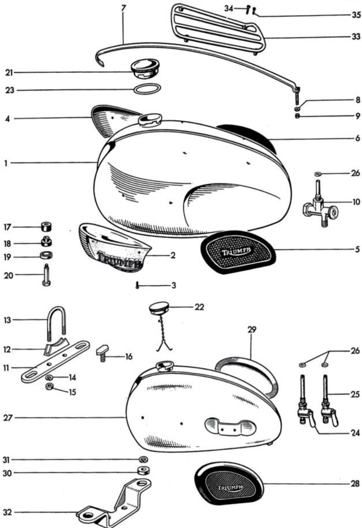
Fig. 25. PETROL TANK
