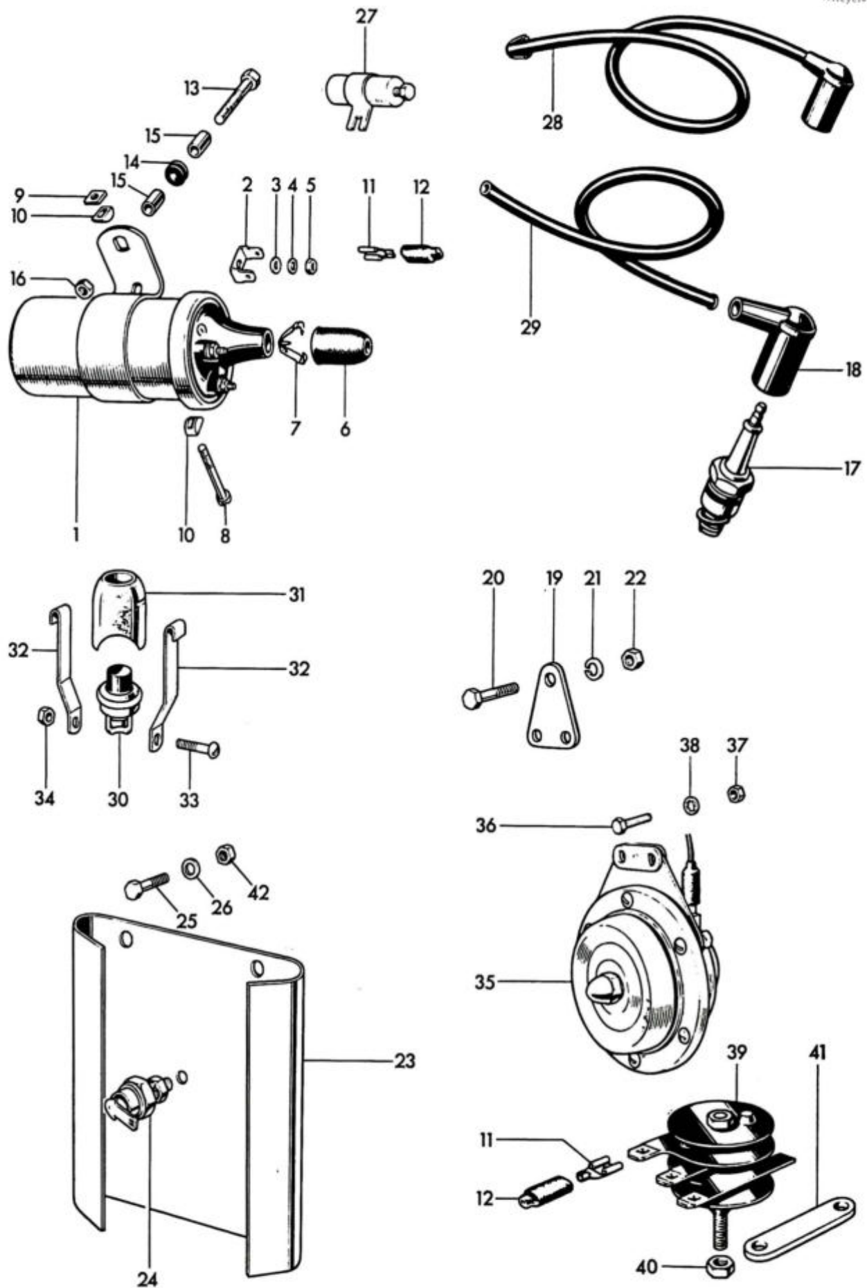
Fig. 33. D.C. IGNITION COILS, HORN, RECTIFIER AND ZENER DIODE
