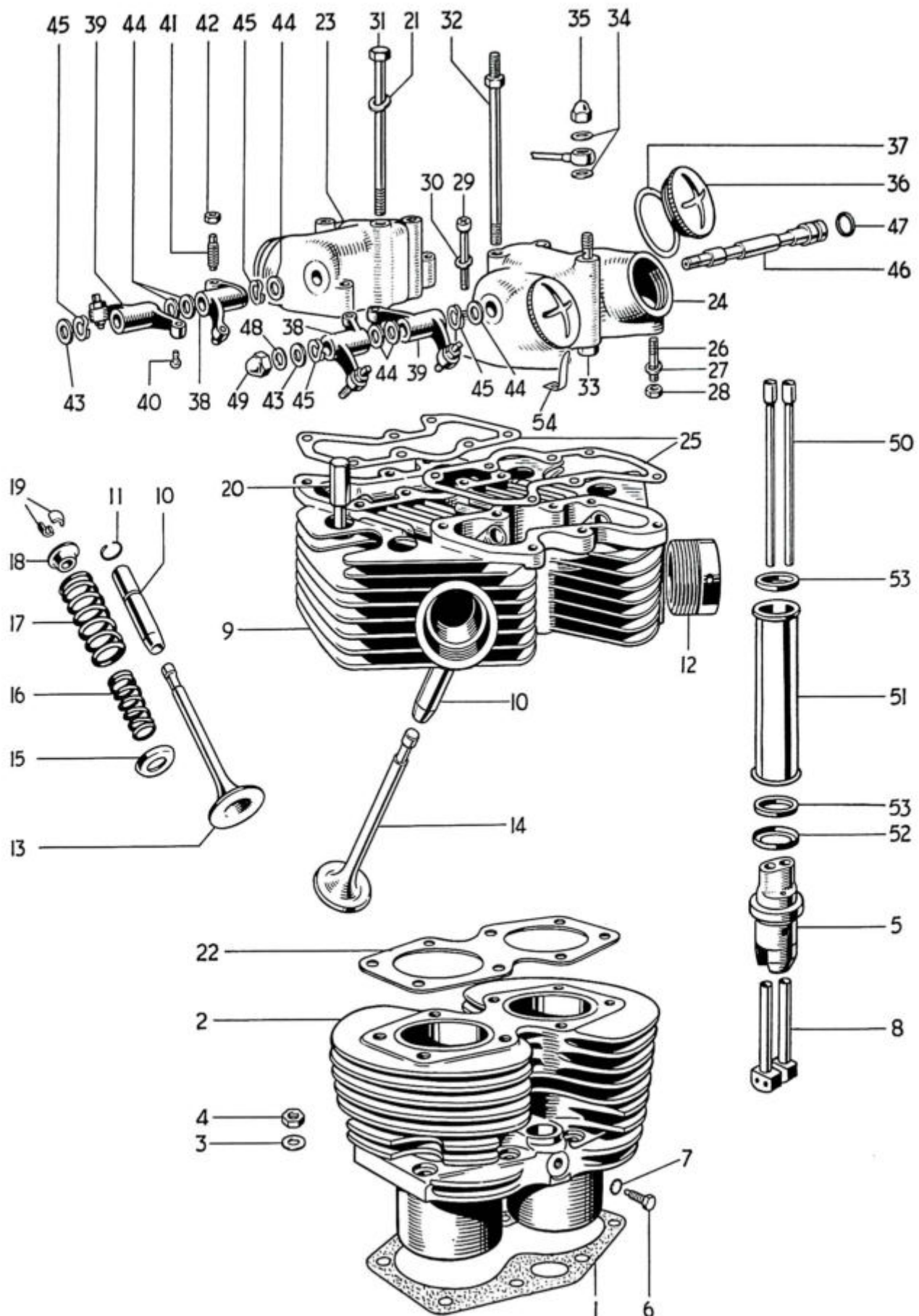
Fig. 5. CYLINDER BLOCK AND HEAD, 5TA AND T100
