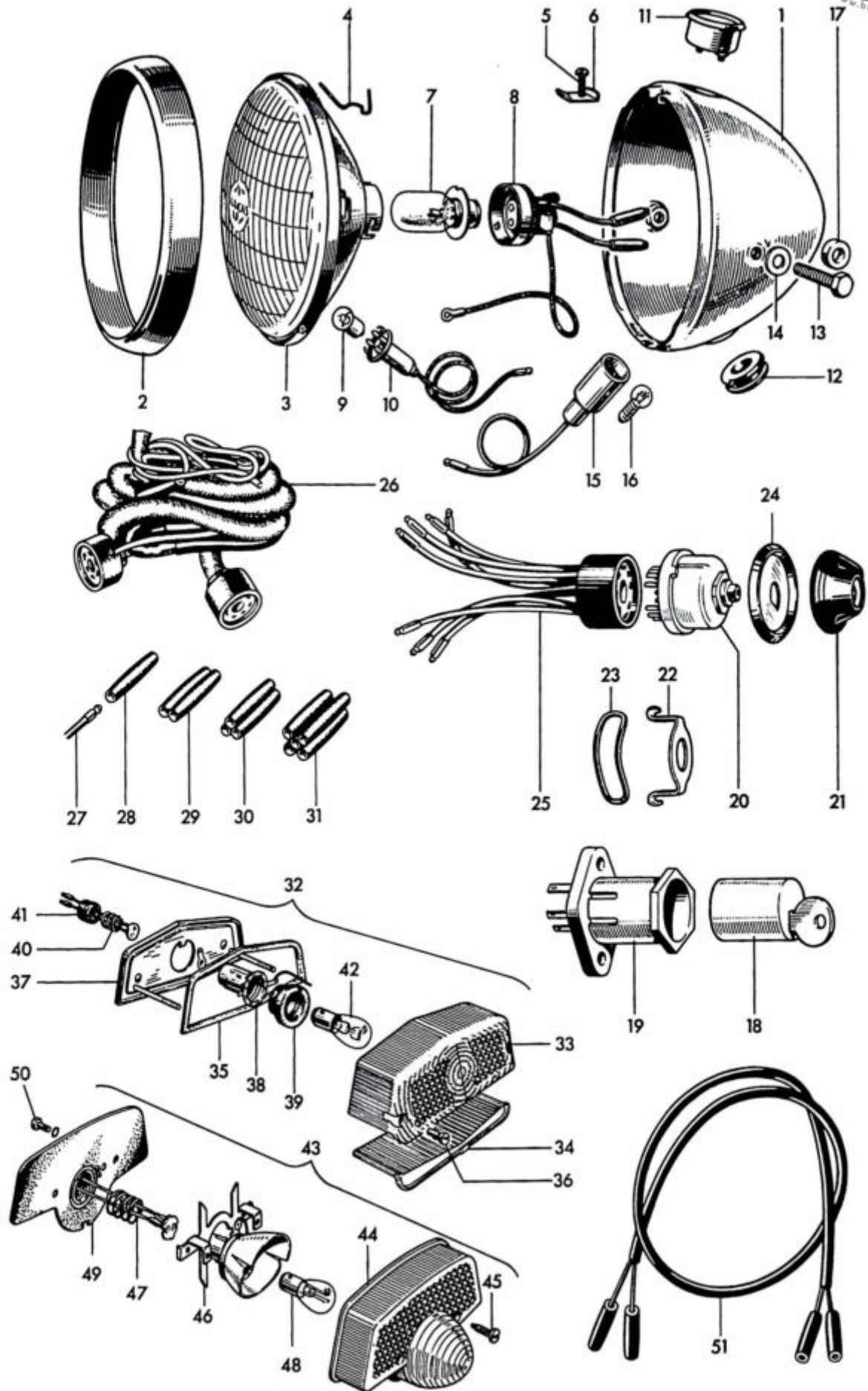
Fig. 34. HEADLAMP, WIRING HARNESS, SWITCHES AND TAIL LAMP
