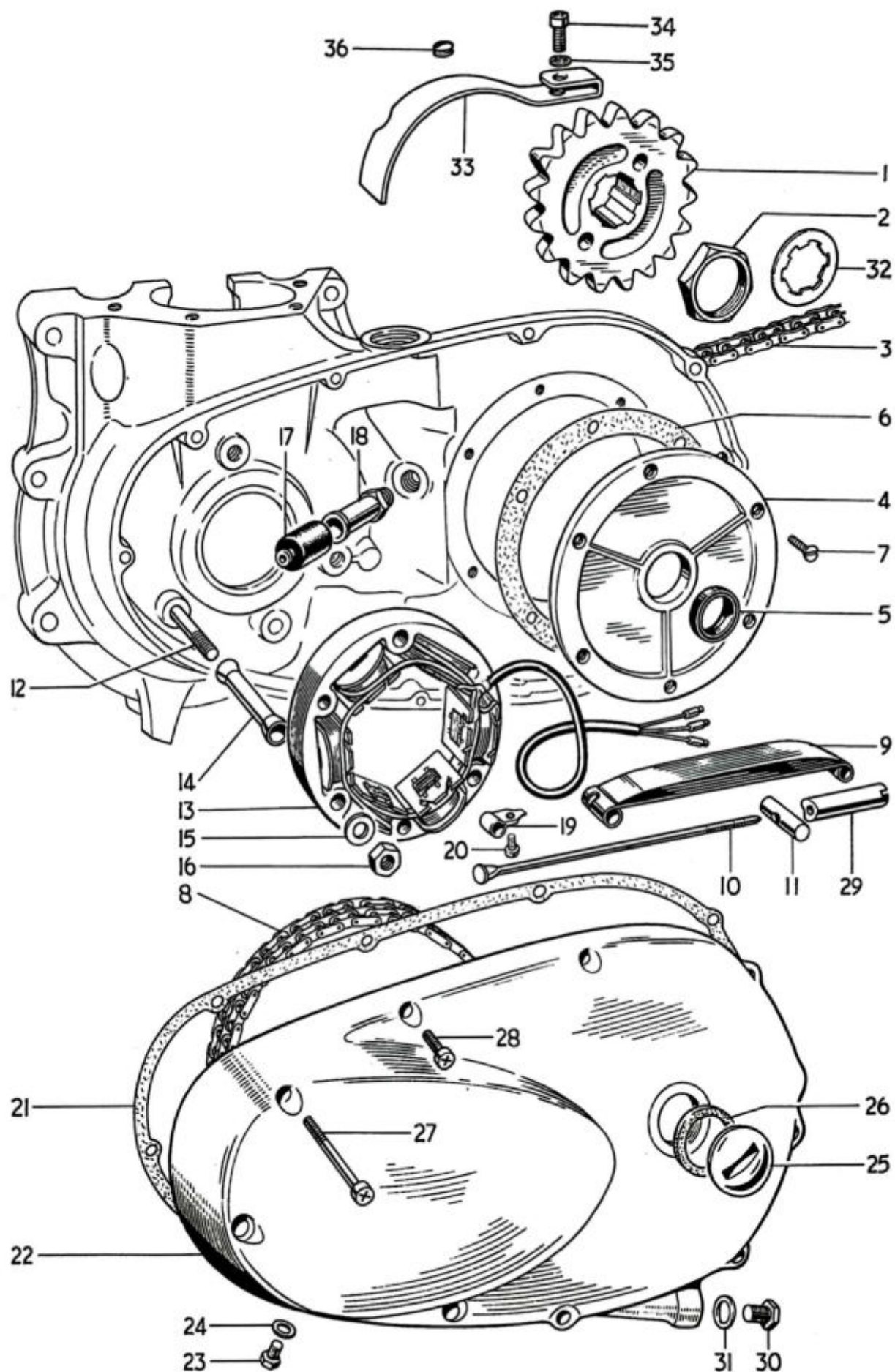
Fig. 10. CHAINCASE AND CHAINS
