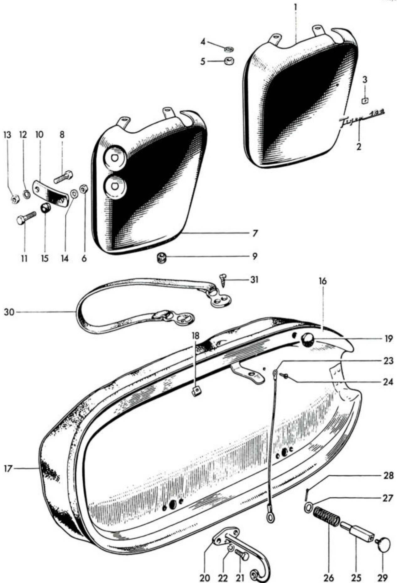
Fig. 24. PANELS AND TWINSEAT
