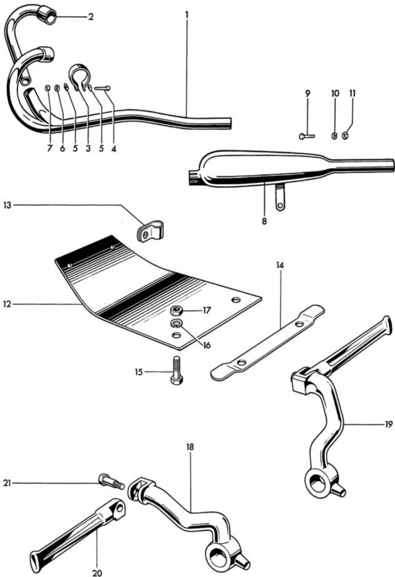
Fig. 12. EXHAUST PIPES, UNDERSHIELD AND FOOTPEGS (T100C)
