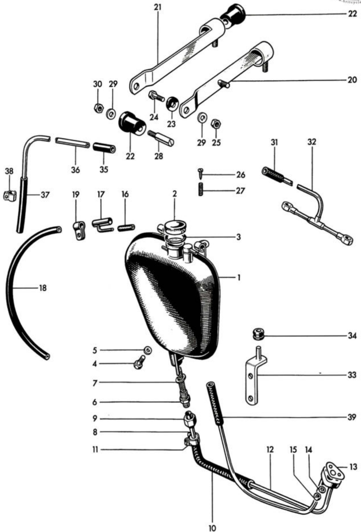
Fig. 26. OIL TANK
