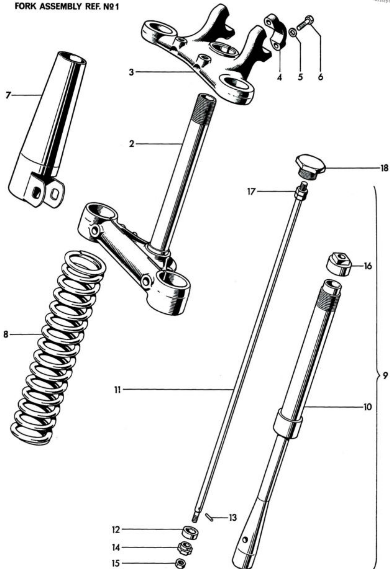
Fig. 18. TELESCOPIC FRONT FORK, U.S.A. EASTERN T100C
