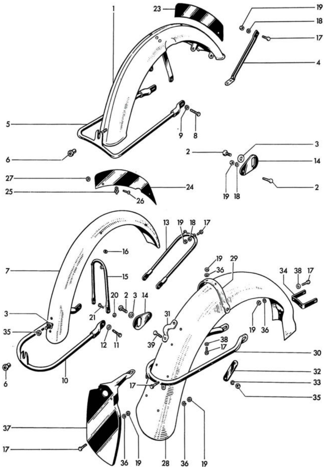
Fig. 22. MUDGUARDS (STANDARD)
