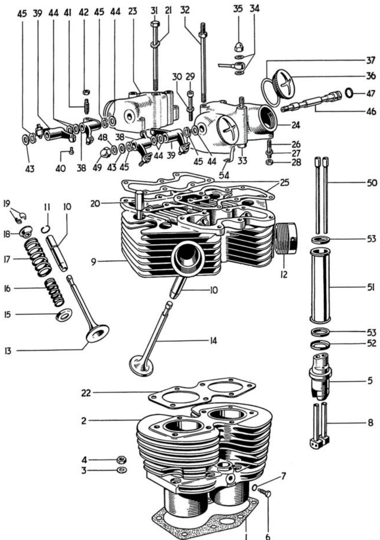
Fig. 4. CYLINDER BLOCK AND HEAD, 3TA AND T90
