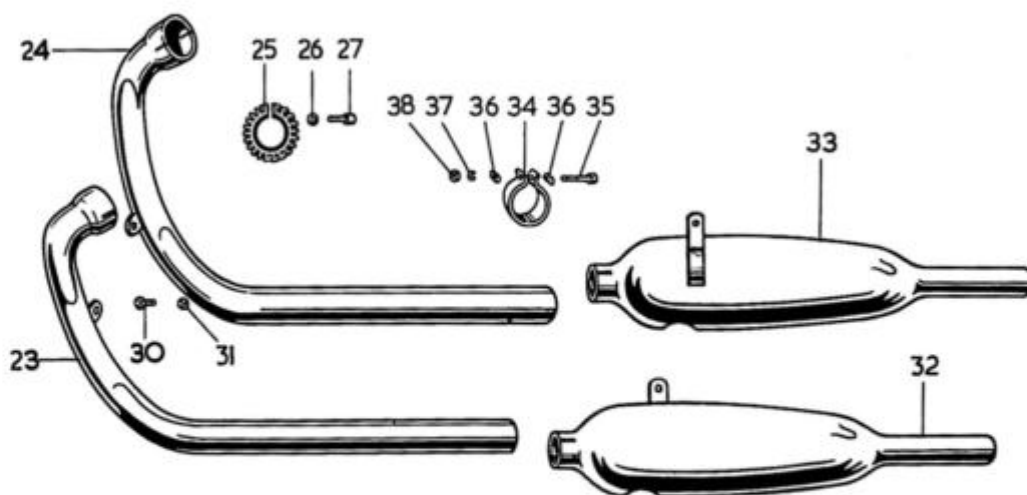
Fig. 13. ENGINE FITTINGS AND EXHAUST SYSTEM
