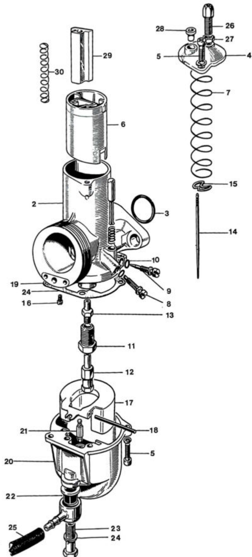
Fig. 29. CARBURETTER, T90, T100 AND T100C
