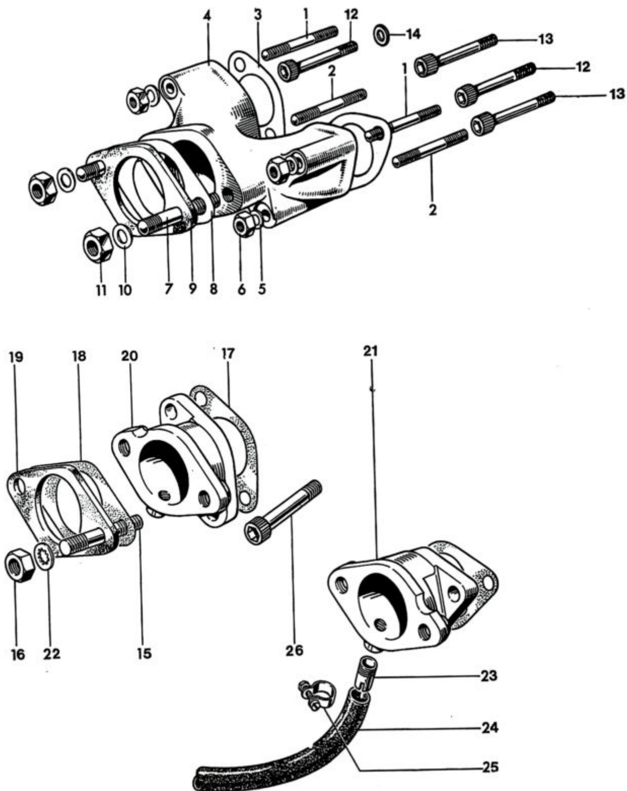
Fig. 4. INLET MANIFOLDS
