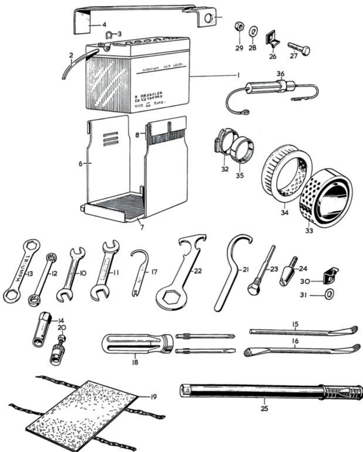
Fig. 26. BATTERY, TOOLKIT AND AIR FILTER
