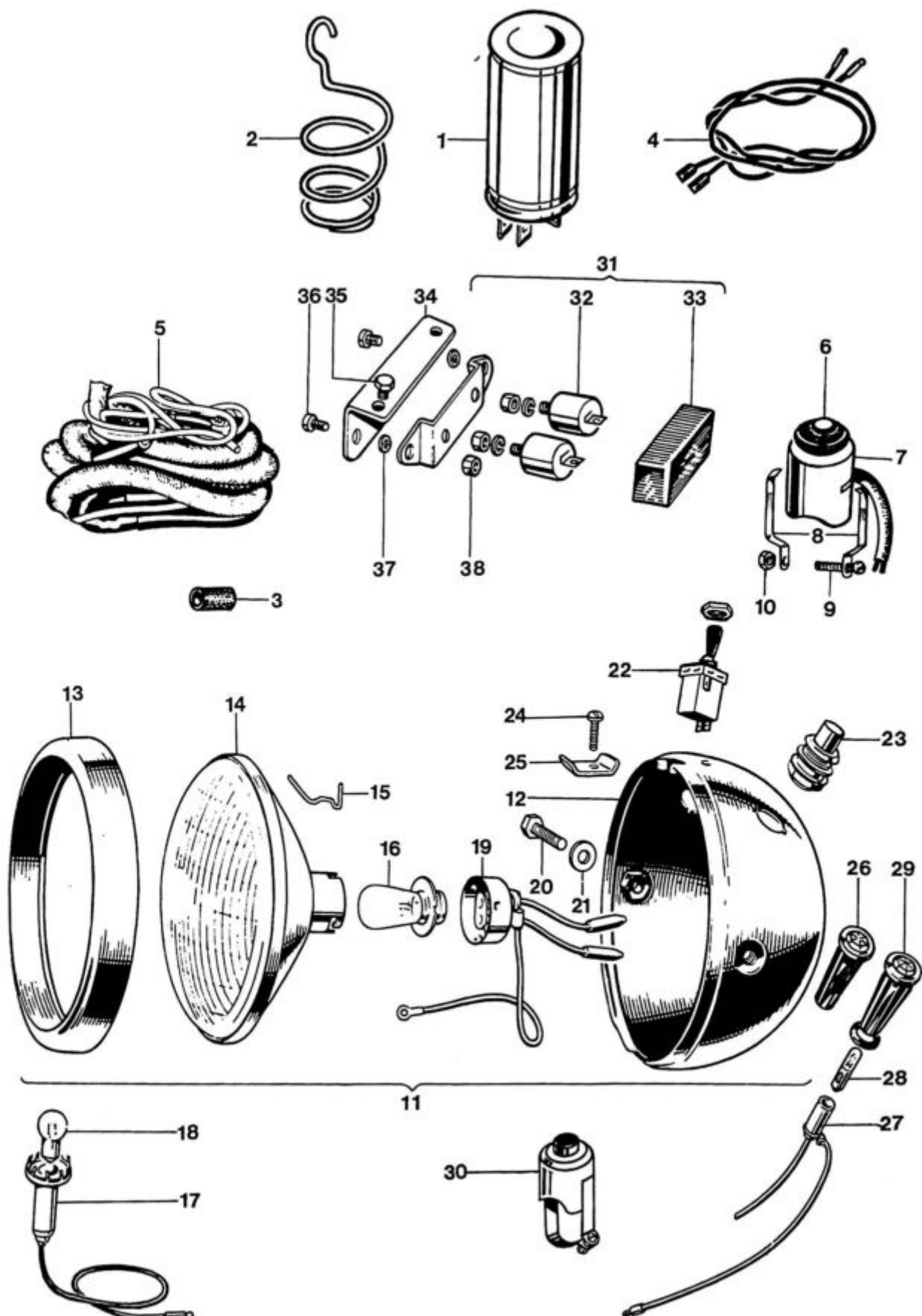
Fig. 31. IGNITION CAPACITOR AND T100C HEADLAMP
