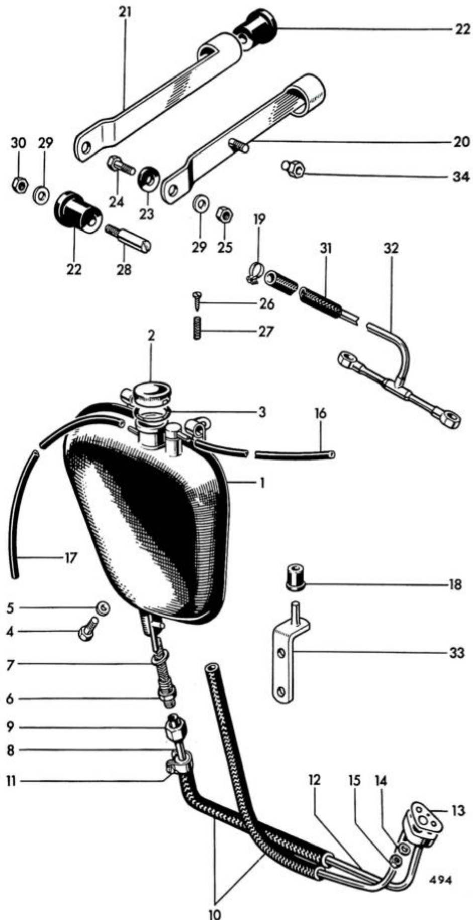
Fig. 25. OIL TANK
