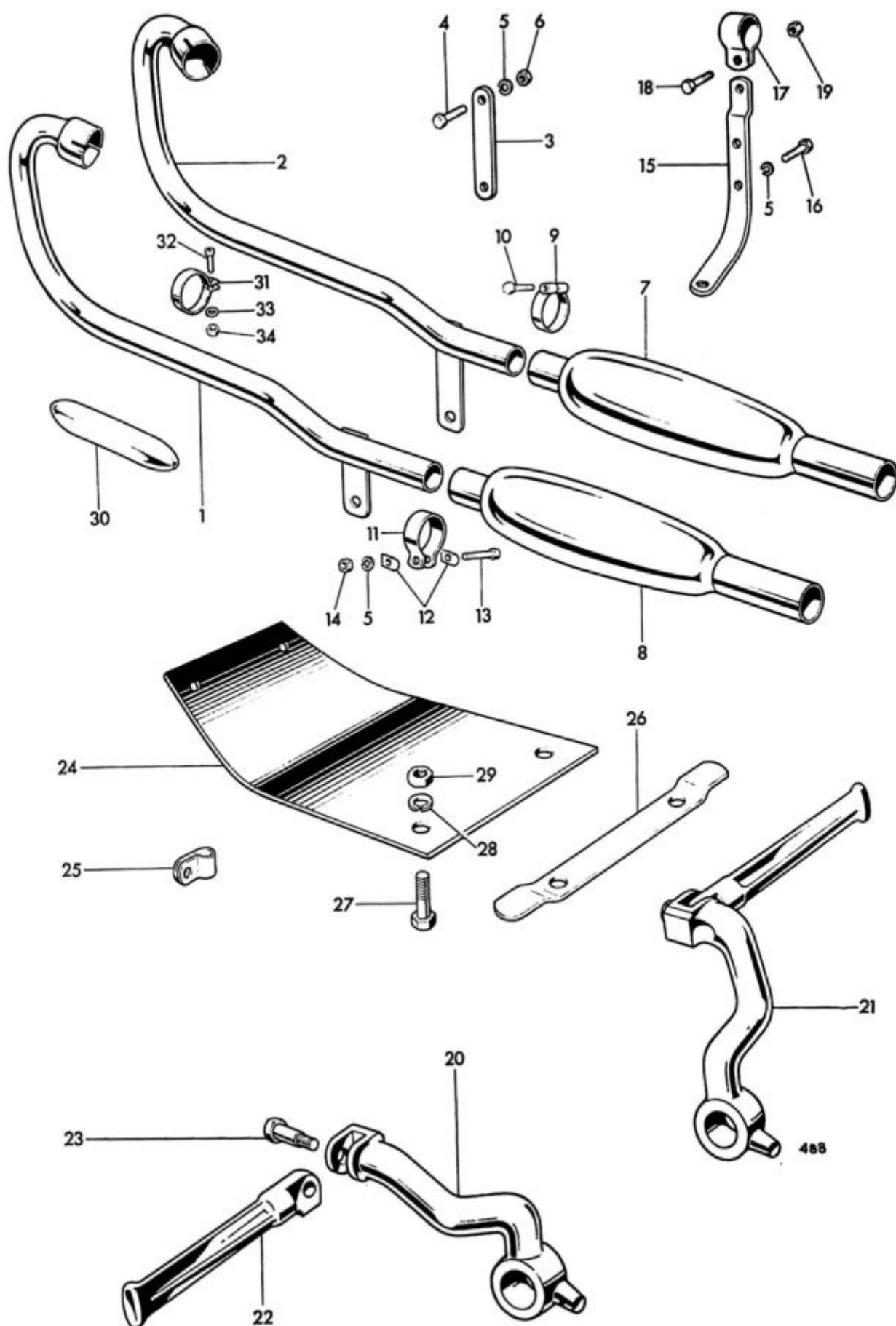
Fig. 14. EXHAUST PIPES, UNDERSHIELD AND FOOTPEGS (T100C)
