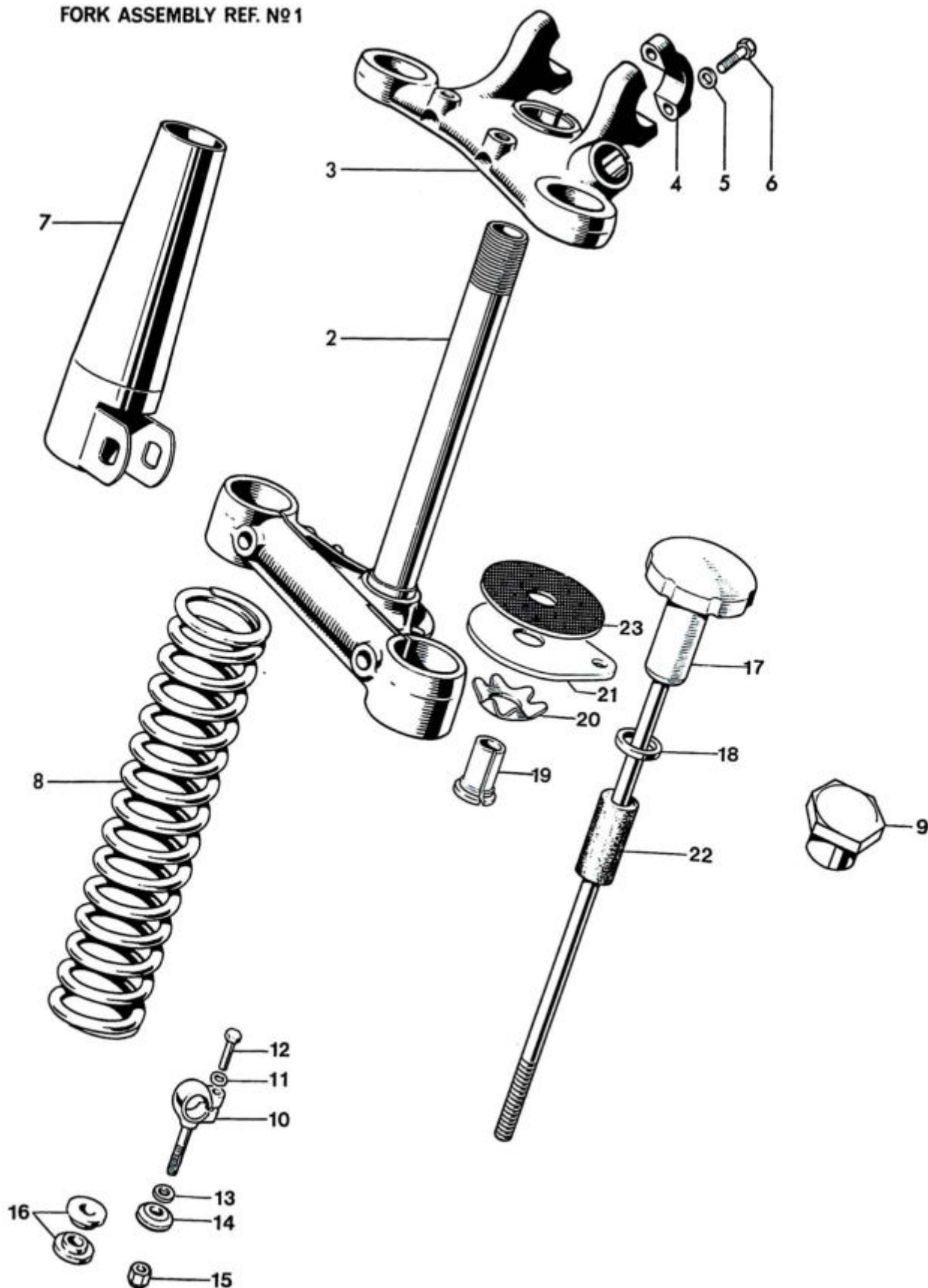
Fig. 18. TELESCOPIC FRONT FORK, U.S.A. T100C AND T100R
