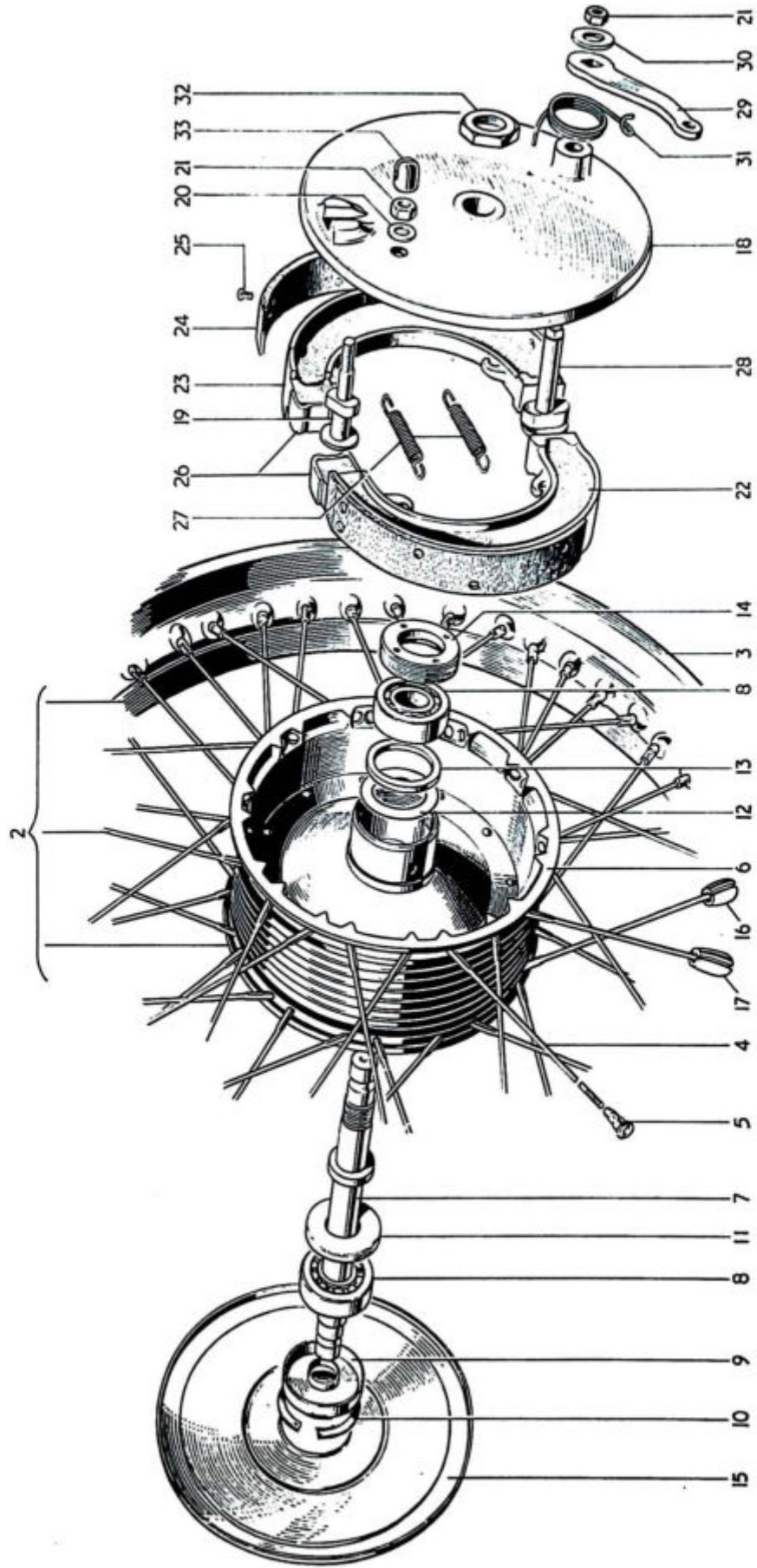
Fig. 19. FRONT WHEEL
