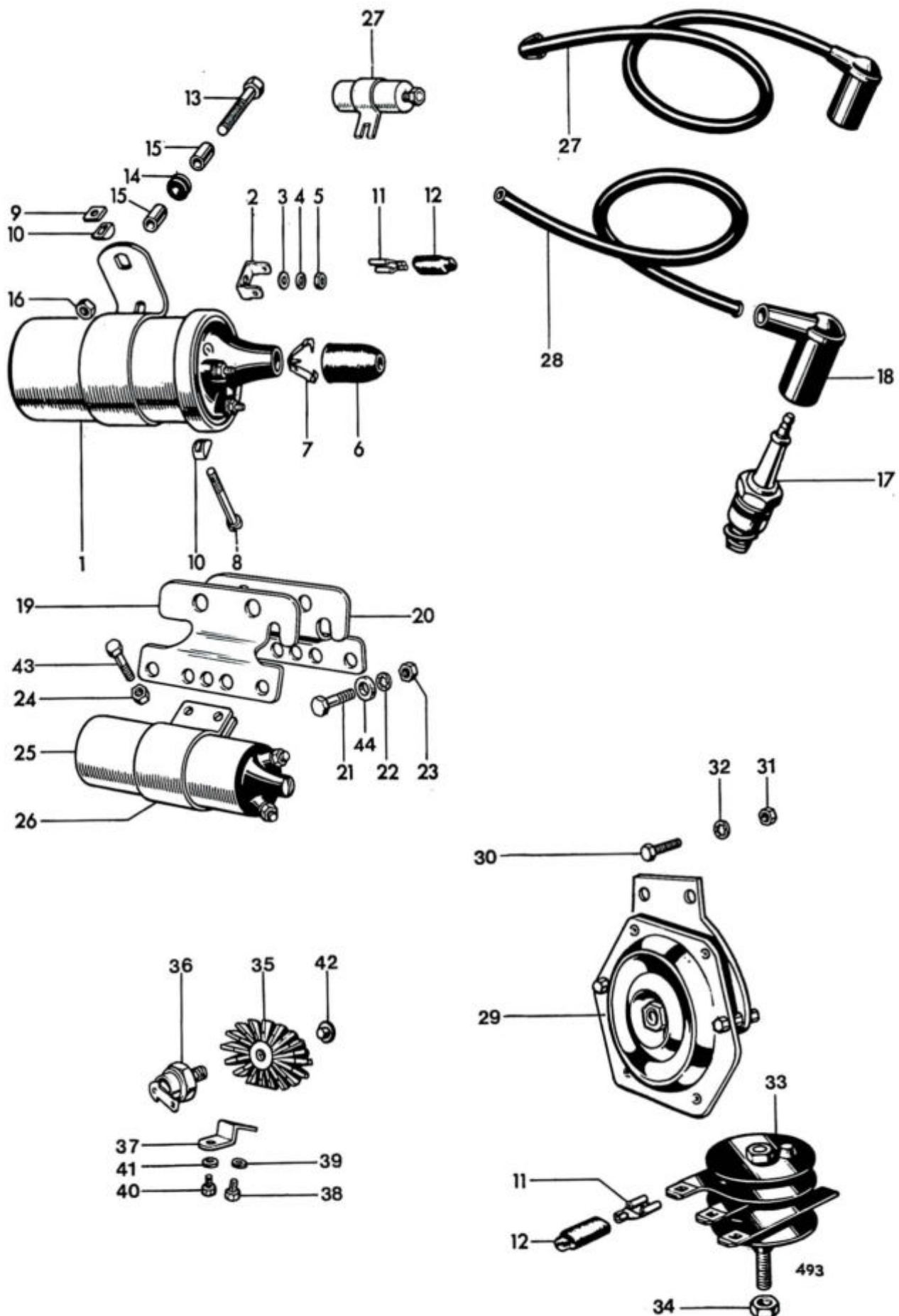
Fig. 32. IGNITION COILS, HORN, RECTIFIER AND ZENER DIODE
