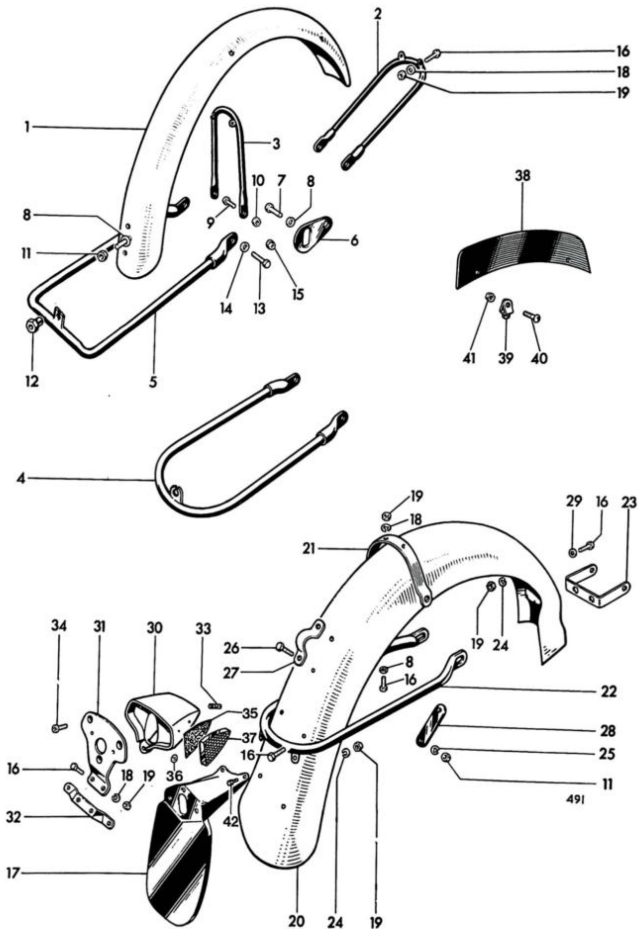
Fig. 22. MUDGUARDS (FENDERS U.S.A.)
