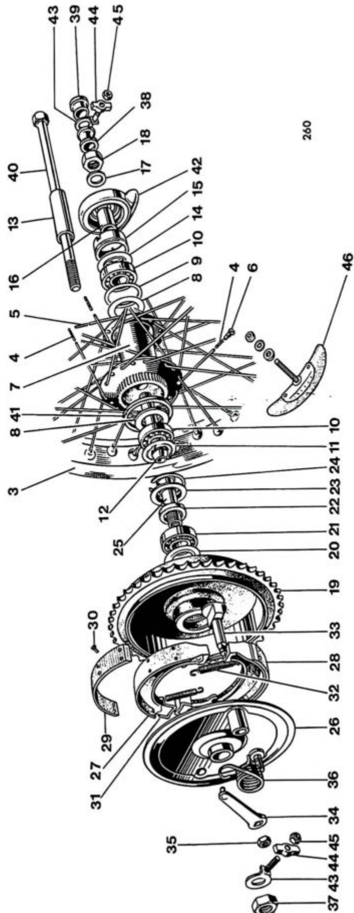
Fig. 21. QUICKLY DETACHABLE REAR WHEEL (NOT U.S.A.)
