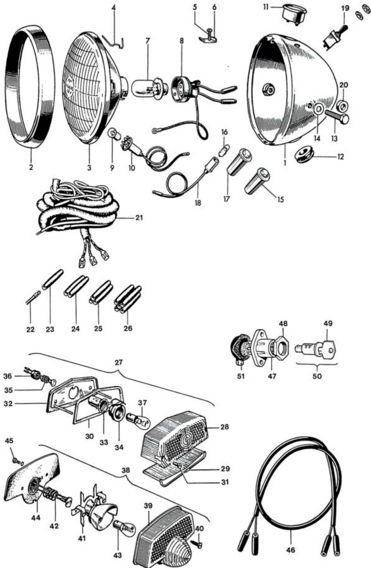
Fig. 33. HEADLAMP, WIRING HARNESS, SWITCHES AND TAIL LAMP
