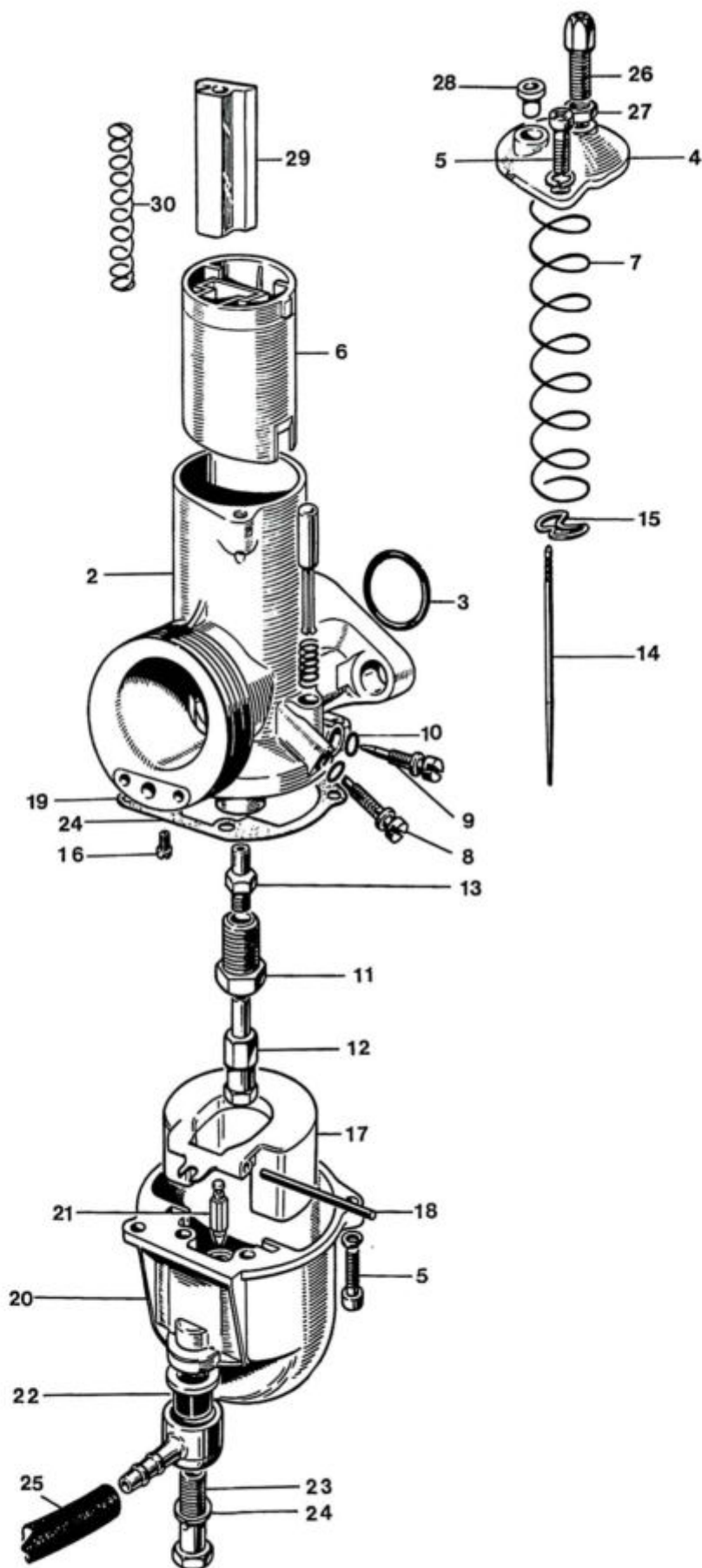
Fig. 30. CARBURETTER, T100T AND T100R
