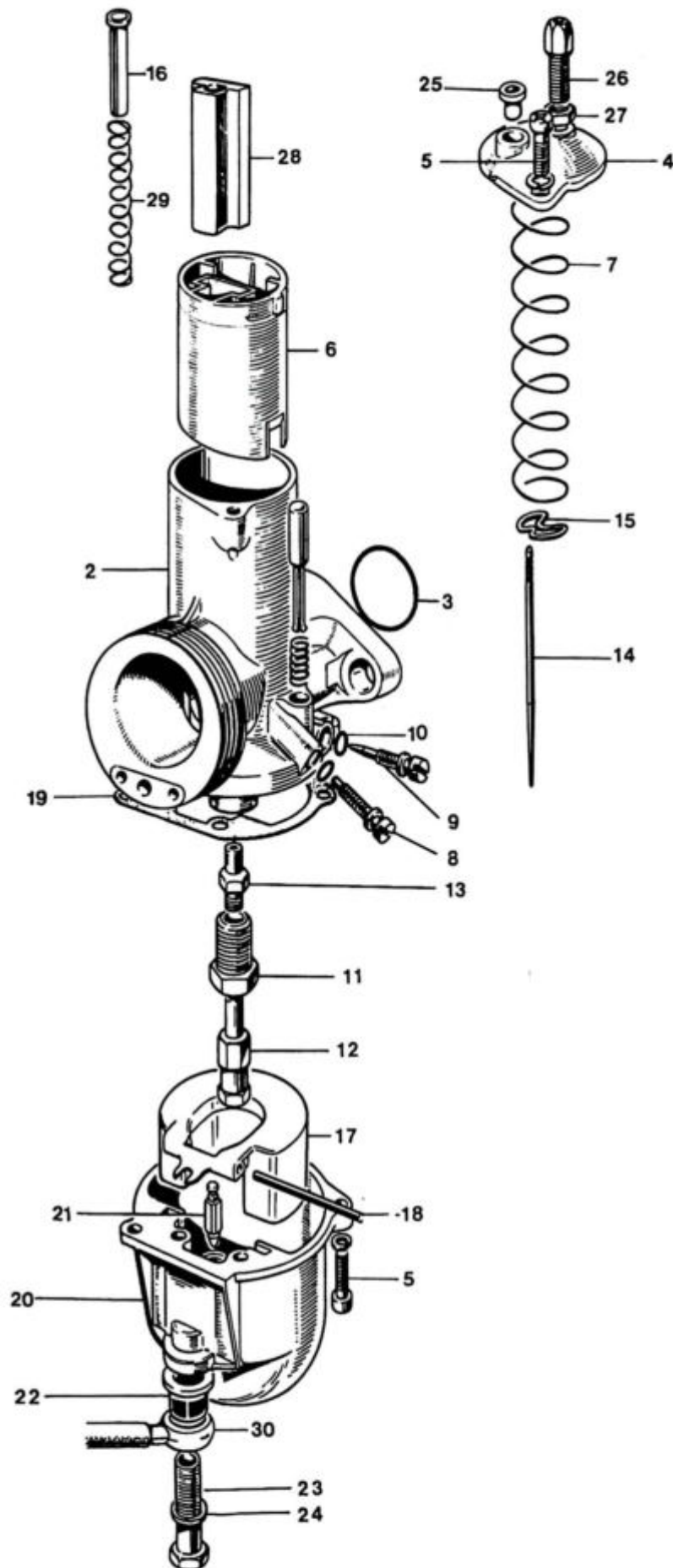
Fig. 31. CARBURETTER, T100T AND T100R
