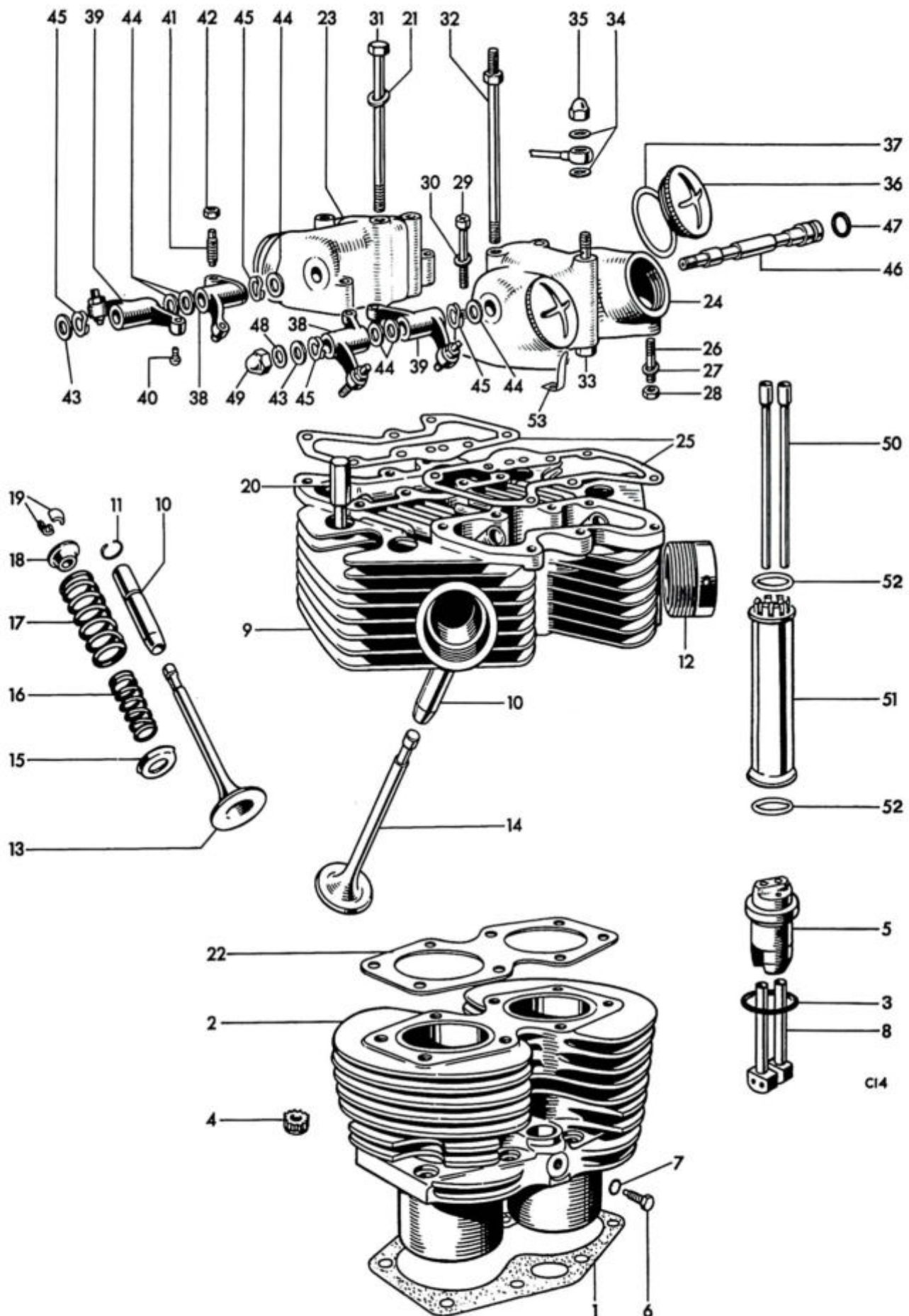
Fig. 7. CYLINDER BLOCK AND HEAD, T100R, T100T
