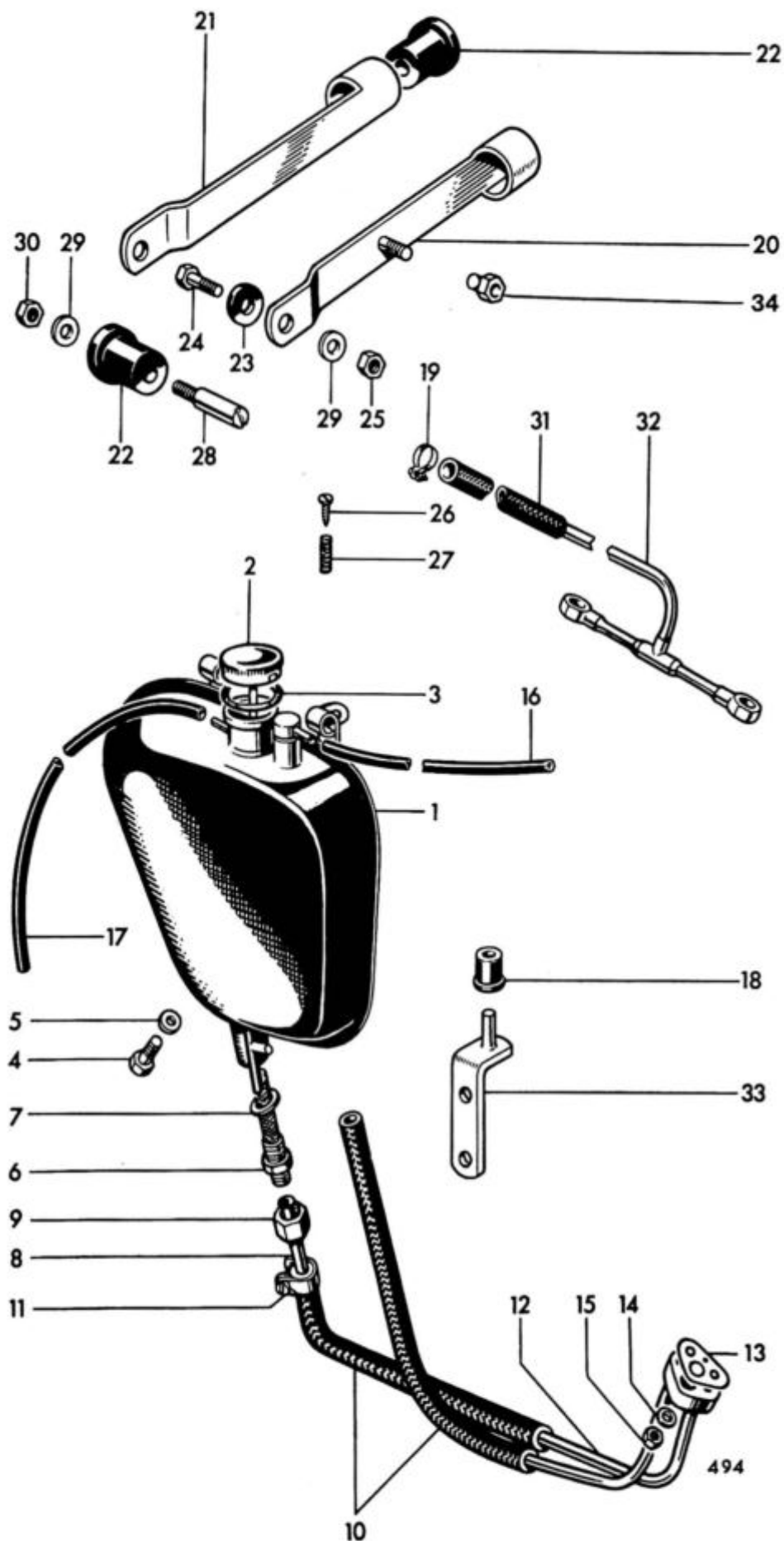
Fig. 26. OIL TANK
