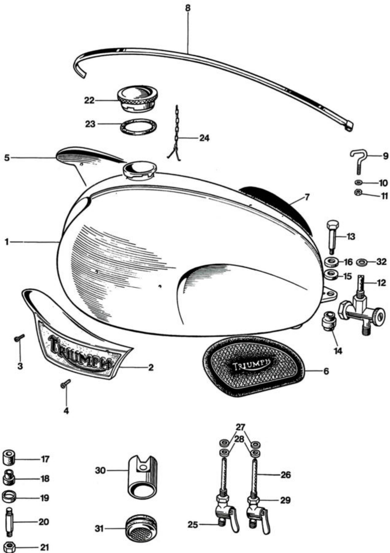
Fig. 25. PETROL TANK
