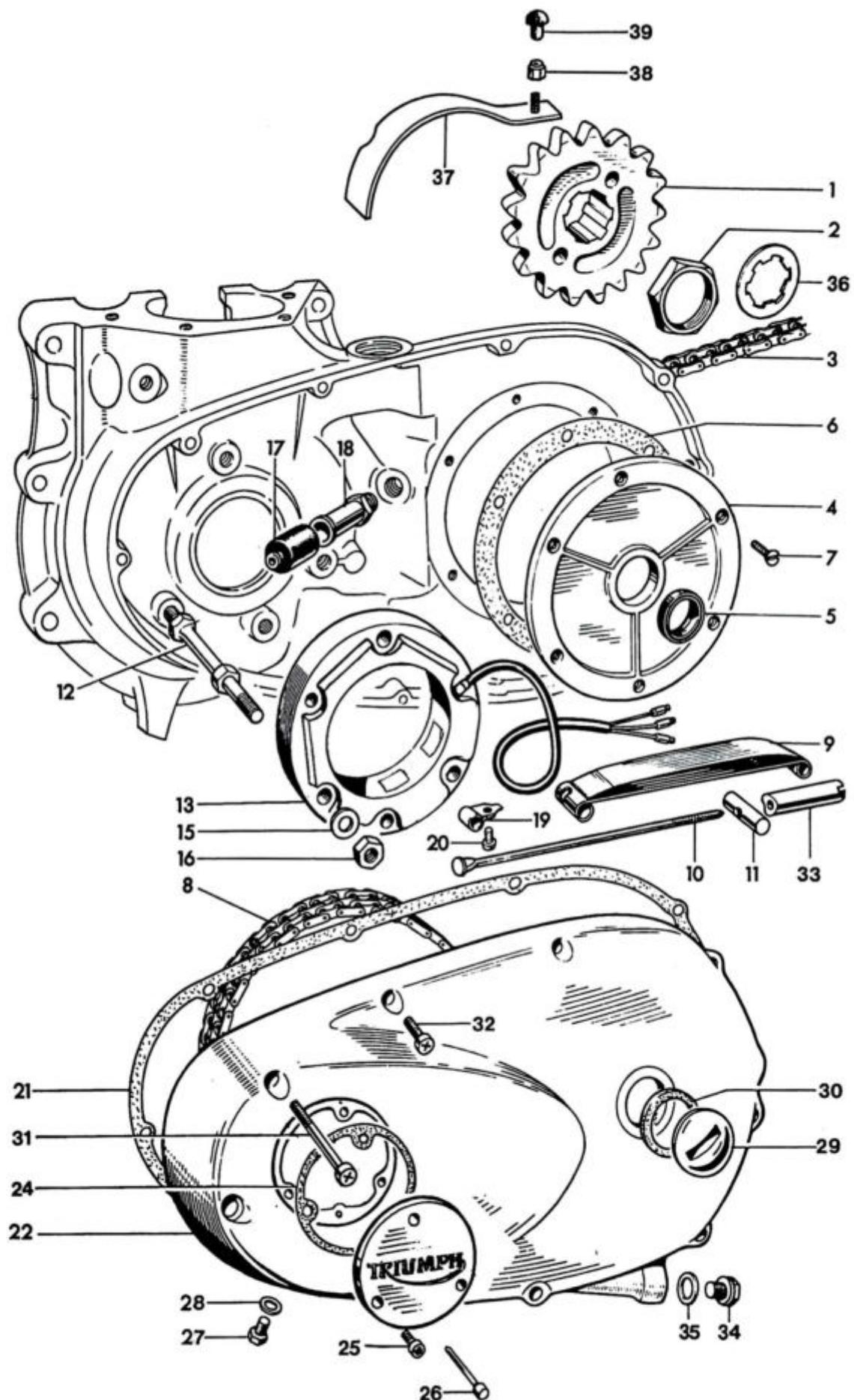
Fig. 12. CHAINCASE AND CHAINS
