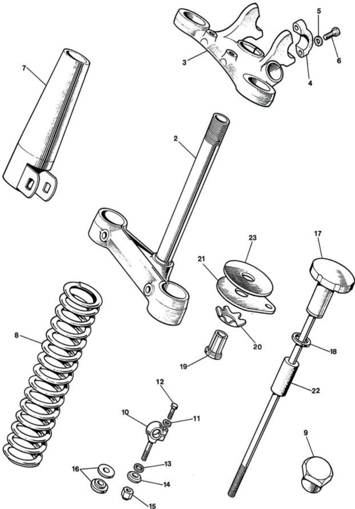
Fig. 18. T100C AND T100R FORK PARTS AND STEERING DAMPER
