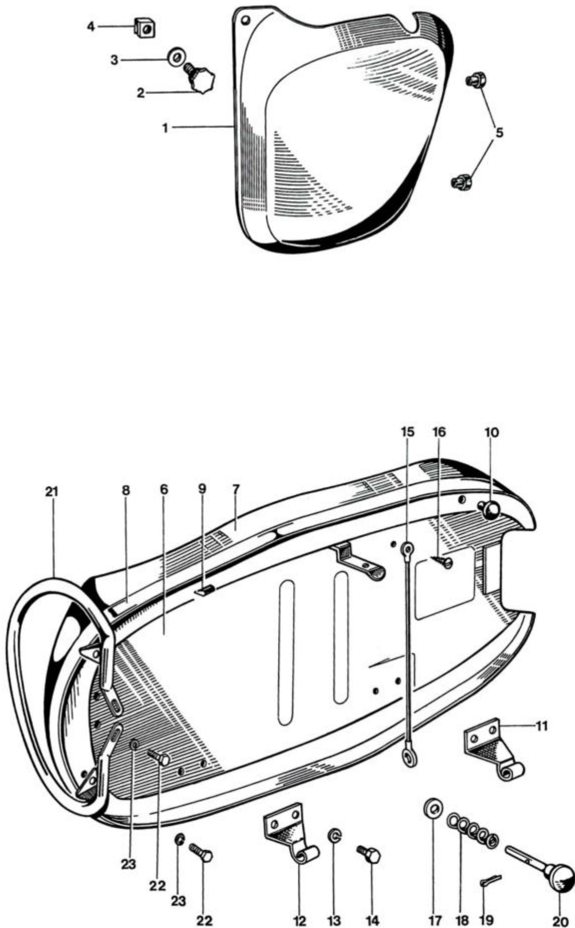
Fig. 24. PANELS AND TWINSEAT
