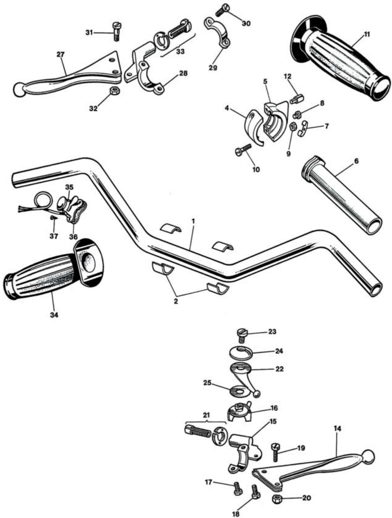
Fig. 28. HANDLEBARS AND CONTROL LEVERS
