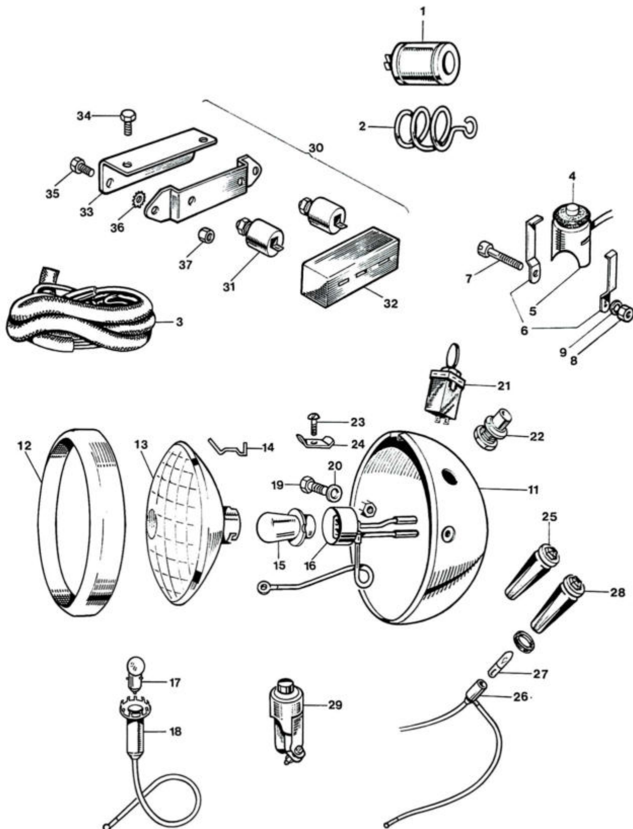
Fig. 32. IGNITION CAPACITOR AND T100C HEADLAMP
