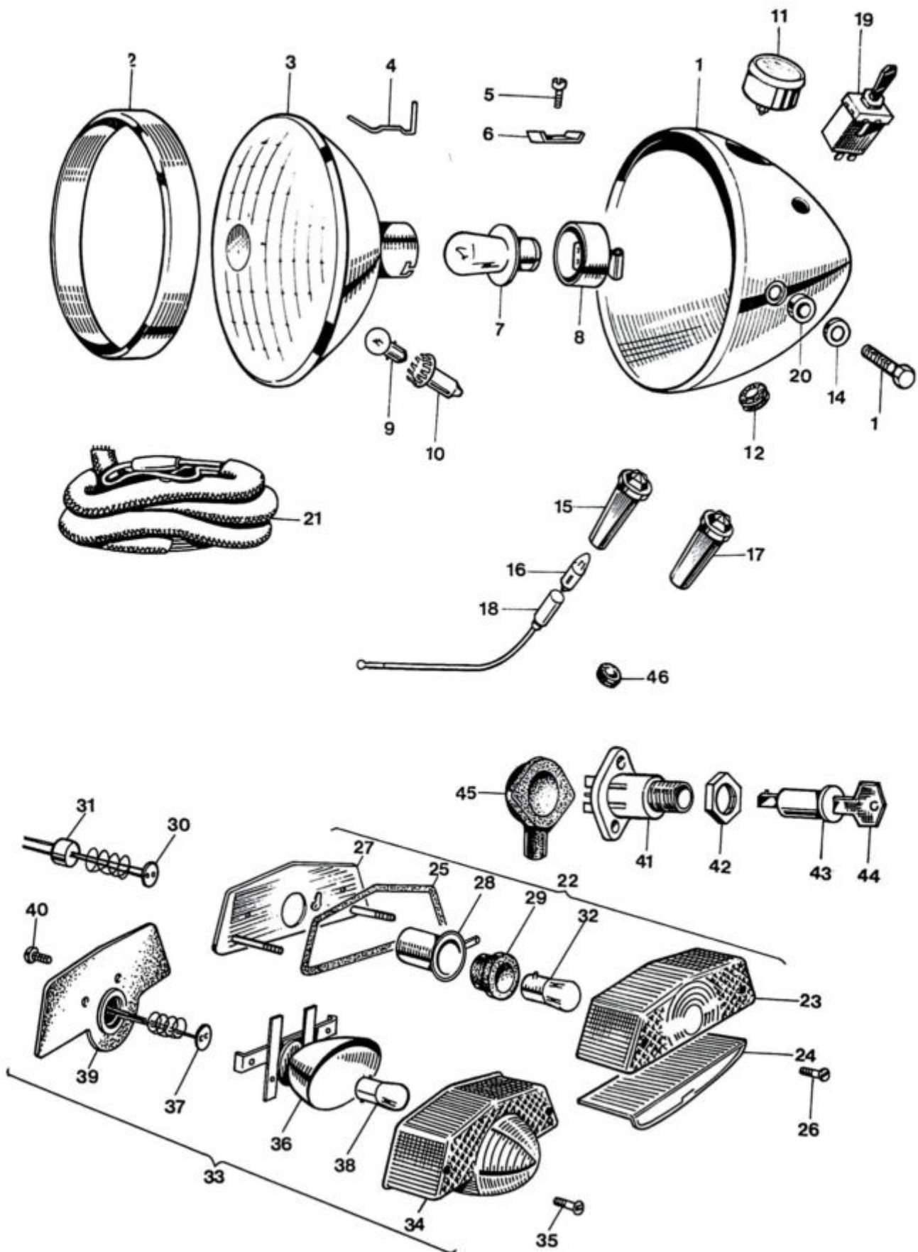
Fig. 33. HEADLAMP, WIRING HARNESS, SWITCHES AND TAIL LAMP
