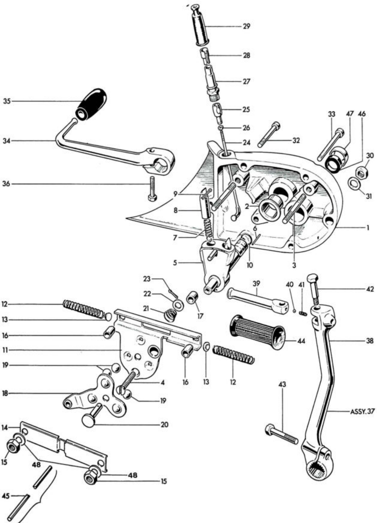
Fig. 10. GEARBOX OUTER COVER AND LEVERS
