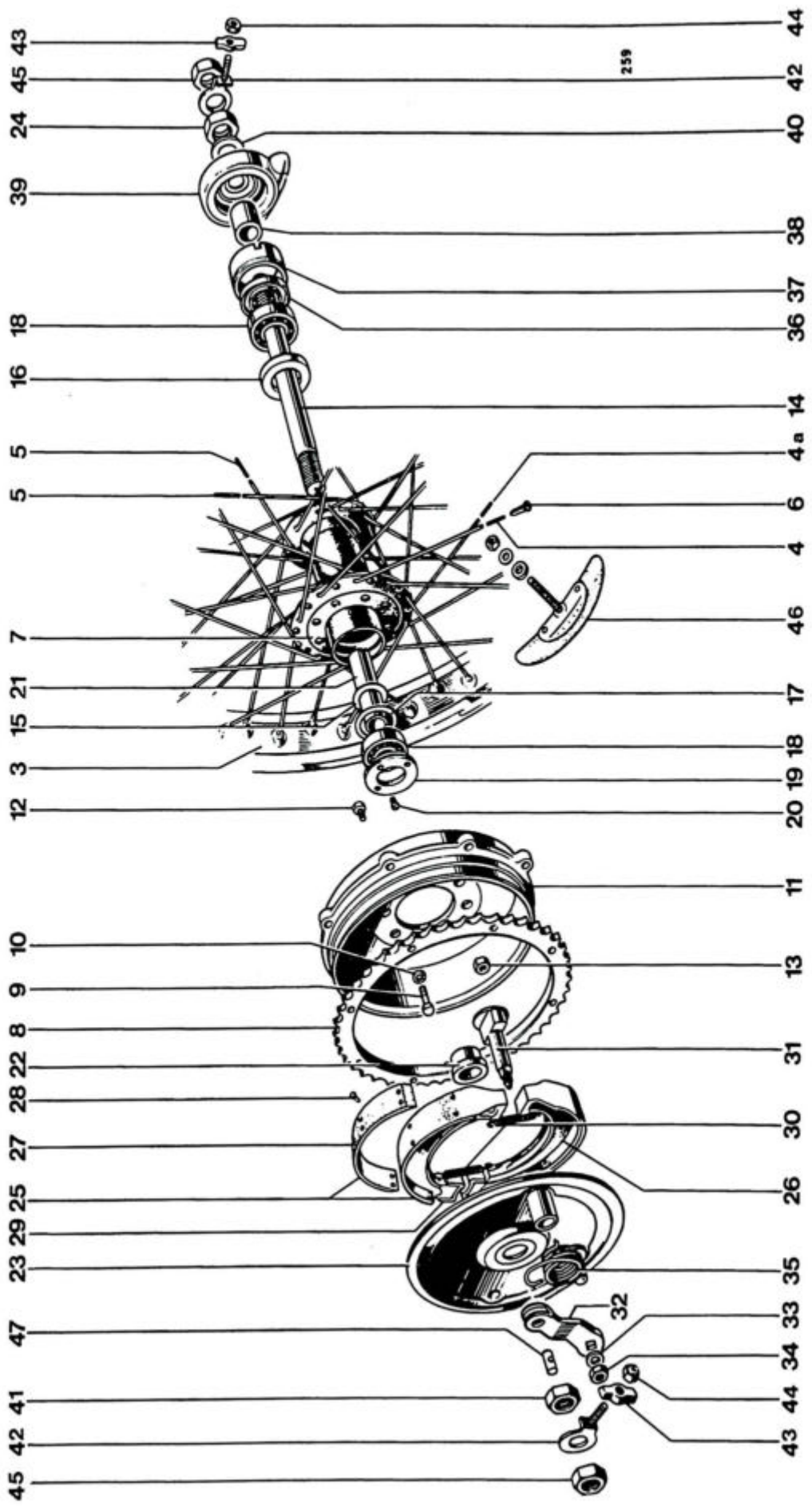
Fig. 21. REAR WHEEL
