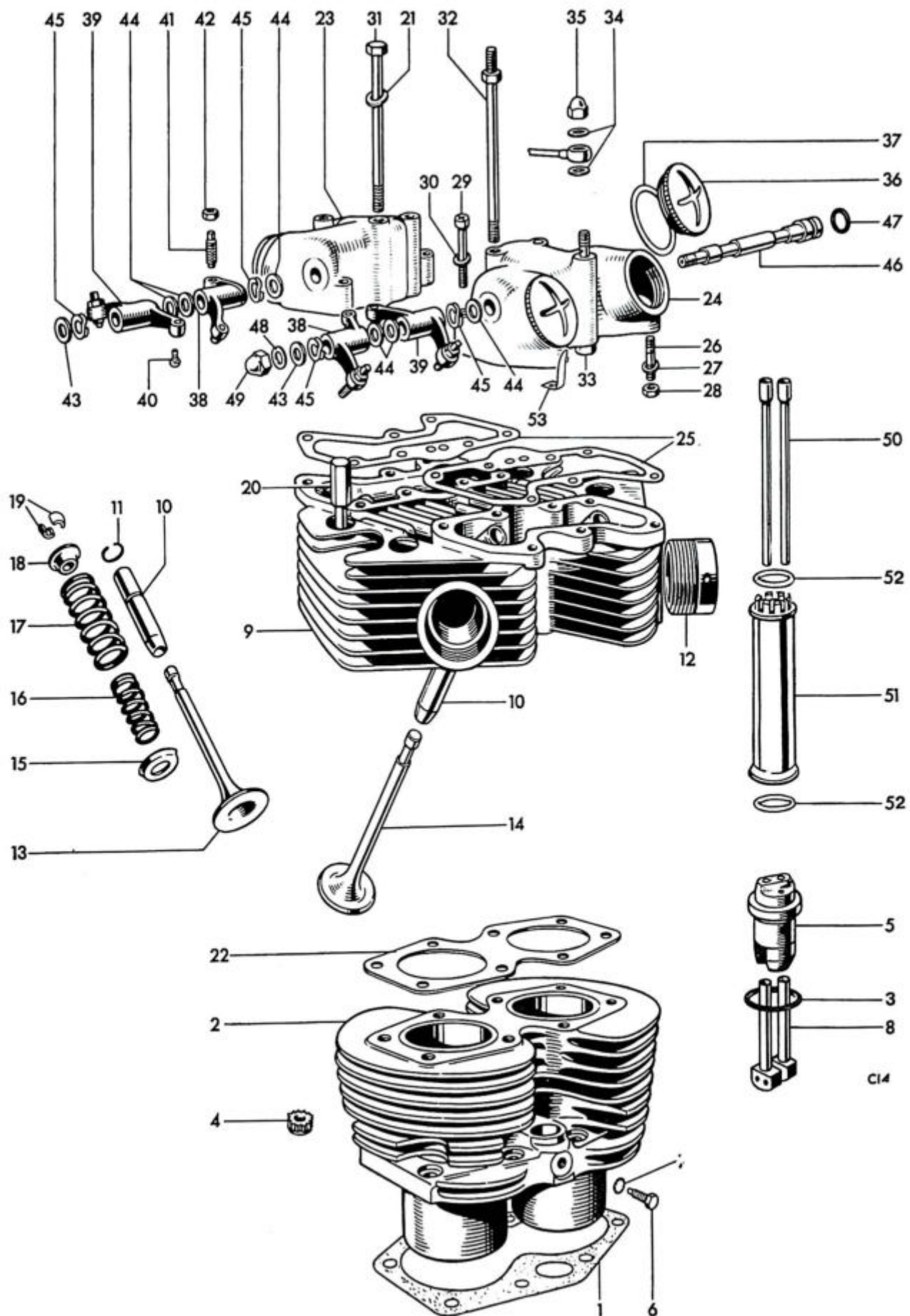
Fig. 6. CYLINDER BLOCK AND HEAD, T100S AND T100C
