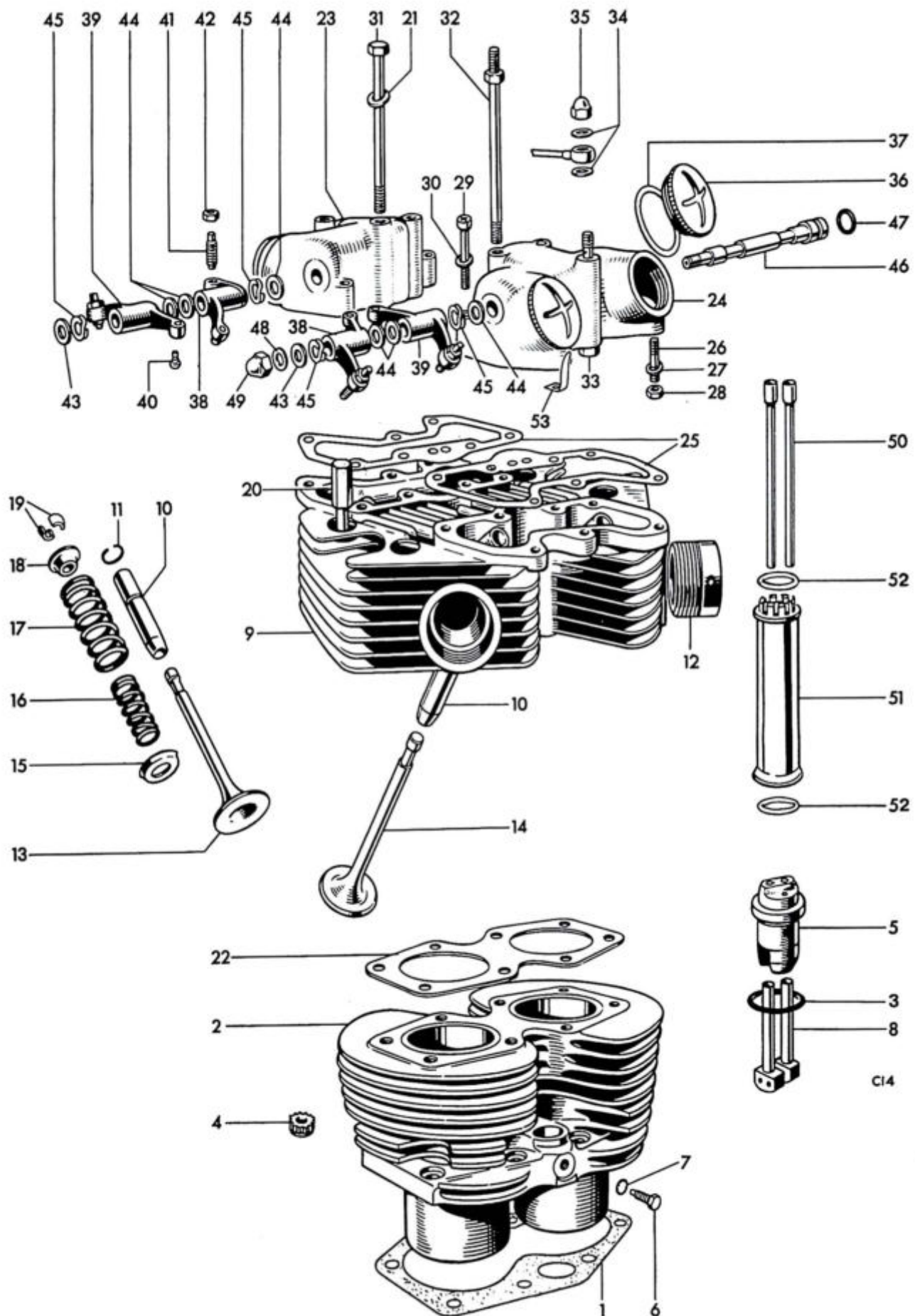
Fig. 5. CYLINDER BLOCK AND HEAD, T90
