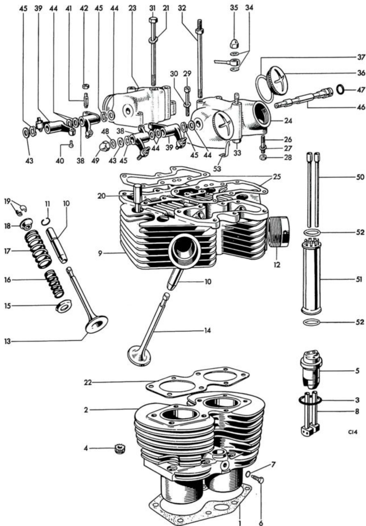
Fig. 5. CYLINDER BLOCK AND HEAD, T90
