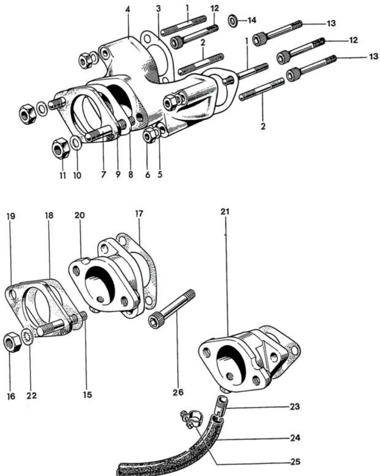
Fig. 4. INLET MANIFOLDS
