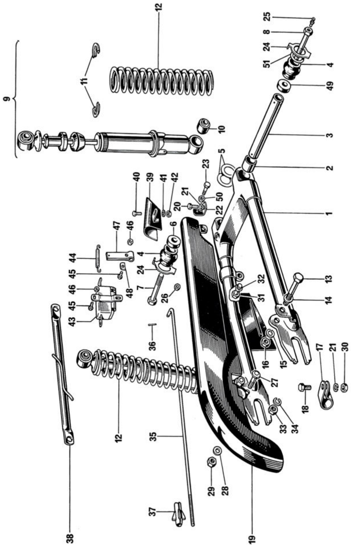
Fig. 16. SWINGING FORK, SUSPENSION UNITS AND CHAINGUARD
