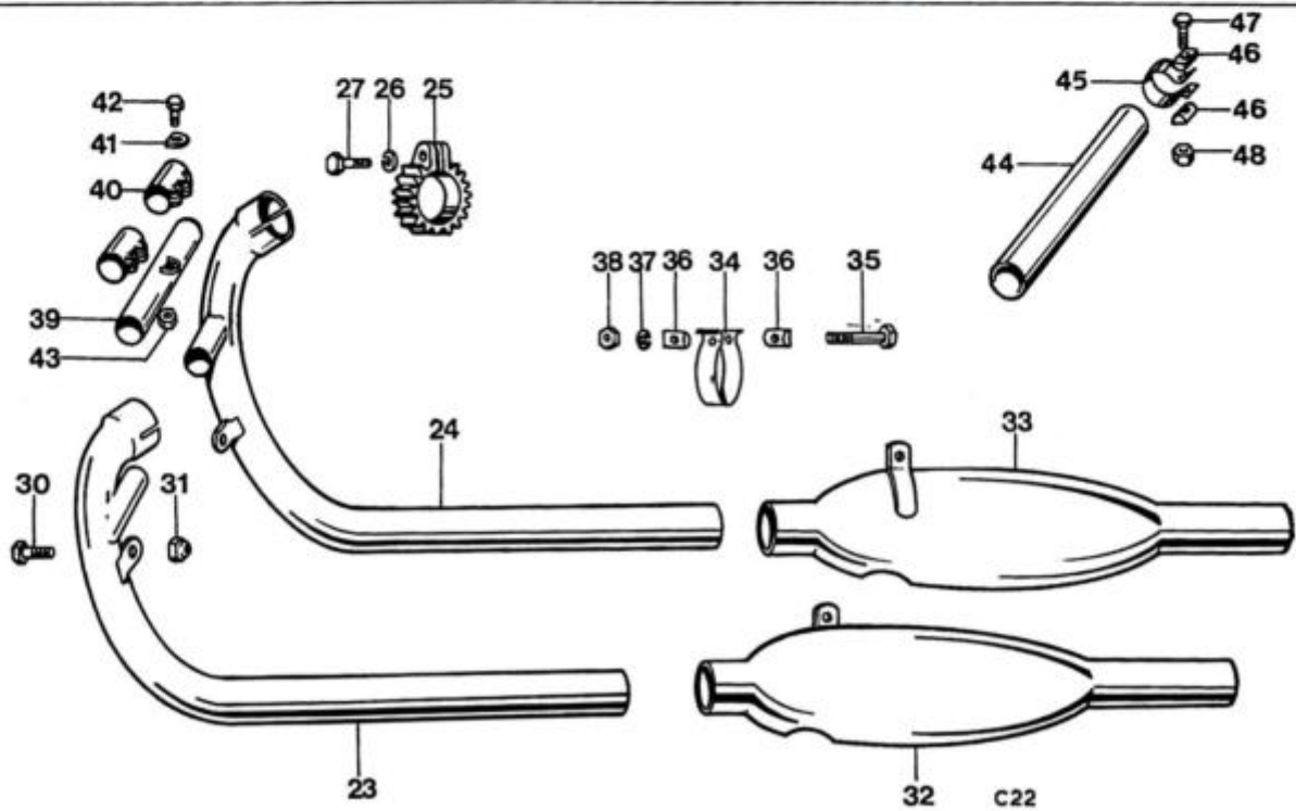
Fig. 13. ENGINE FITTINGS AND EXHAUST SYSTEM
