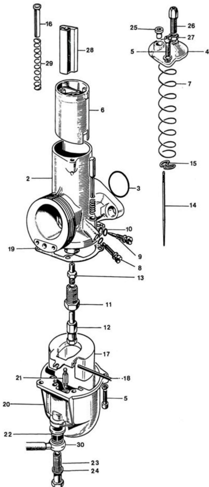
Fig. 30. CARBURETTER, T90, T100 AND T100C
