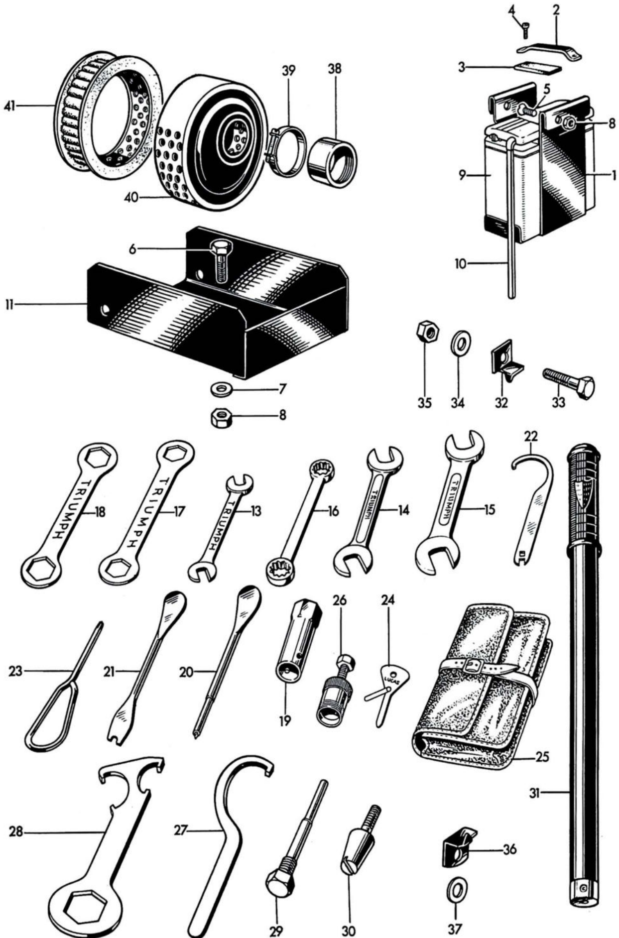
Fig. 24. BATTERY, TOOLKIT AND AIR FILTER
