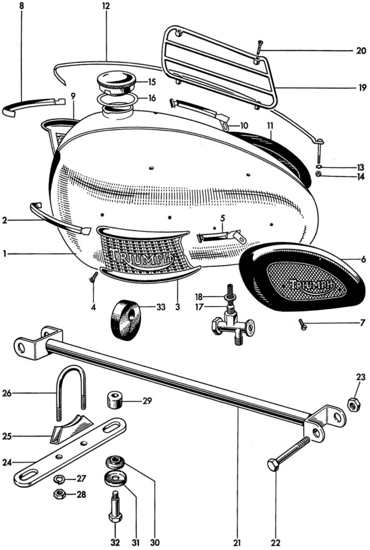
Fig. 22. PETROL TANK
