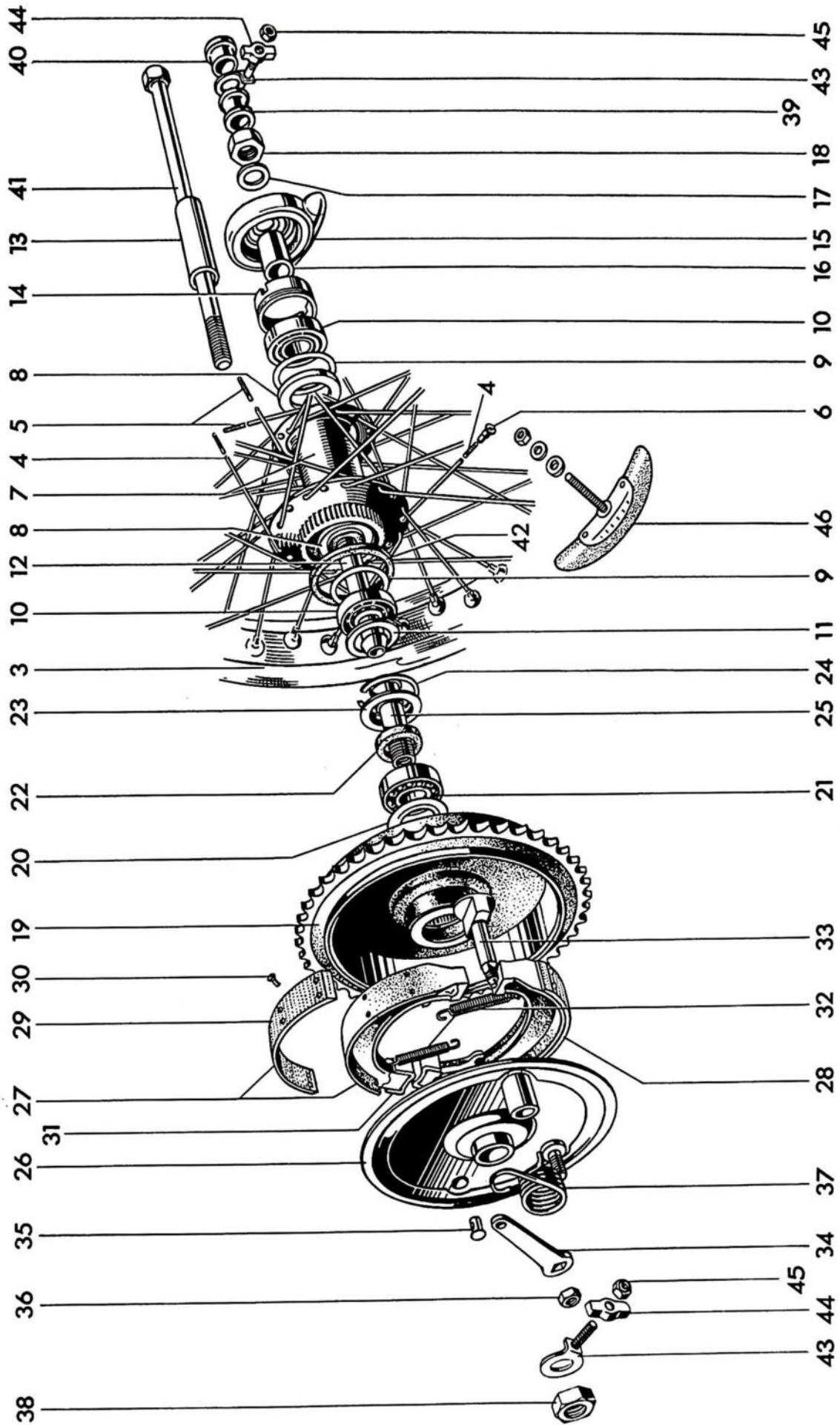
Fig. 19. QUICKLY DETACHABLE REARWHEEL
