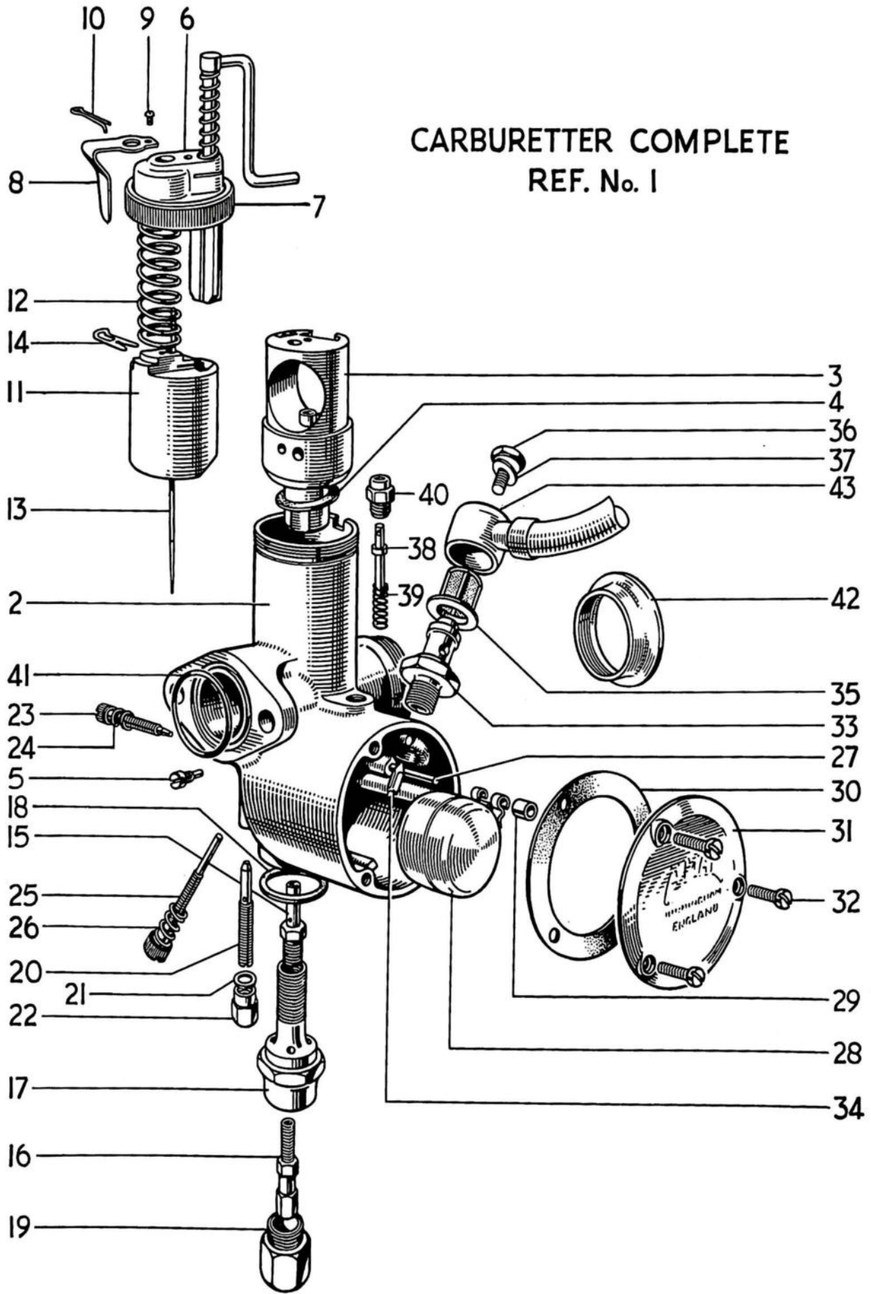
Fig. 27. CARBURETTER, 3TA AND 5TA
