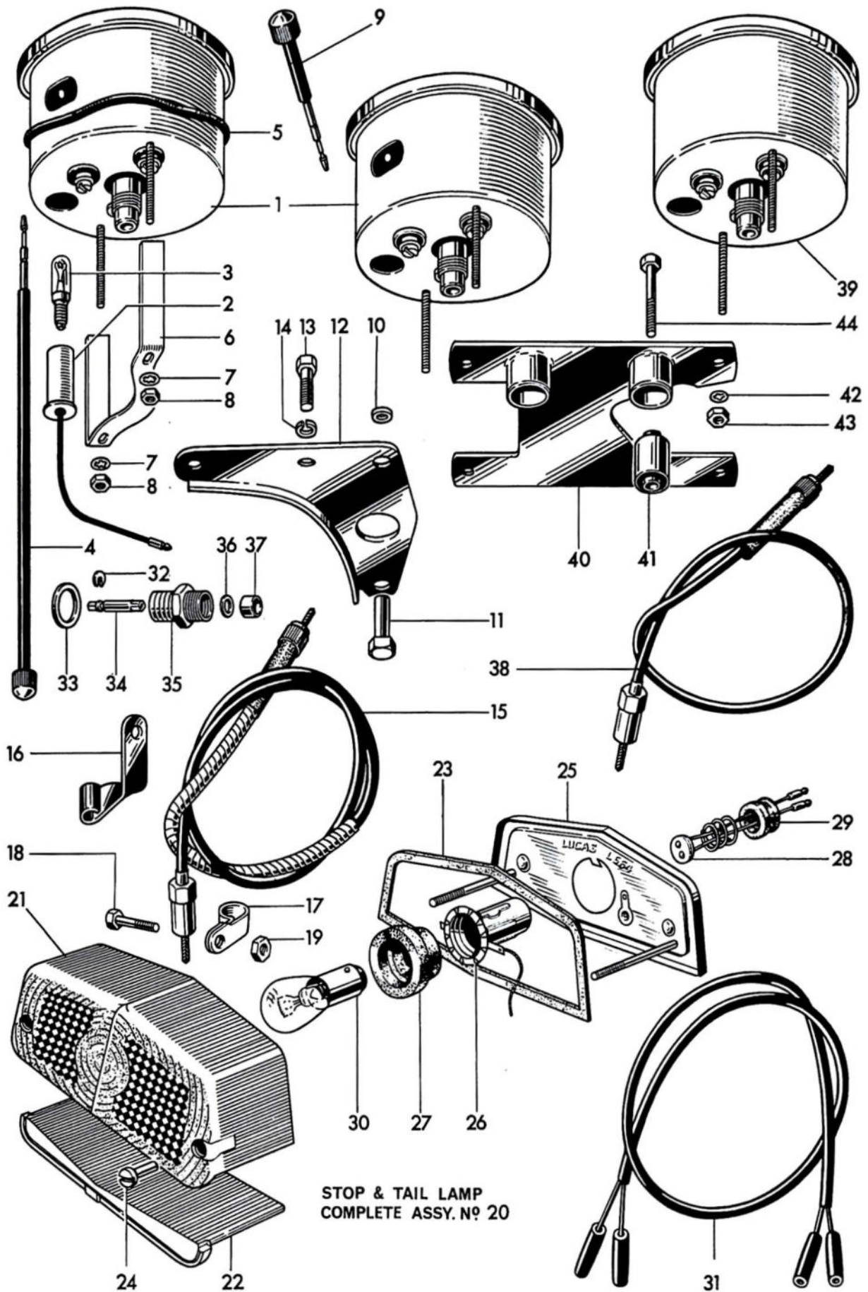
Fig. 30. SPEEDOMETER, TACHOMETER AND TAIL LAMP
