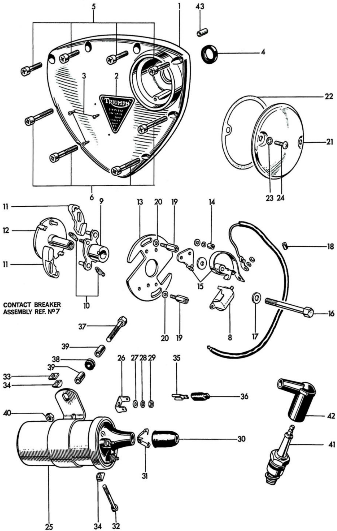
Fig. 6. TIMING COVER, CONTACT BREAKER AND COILS
