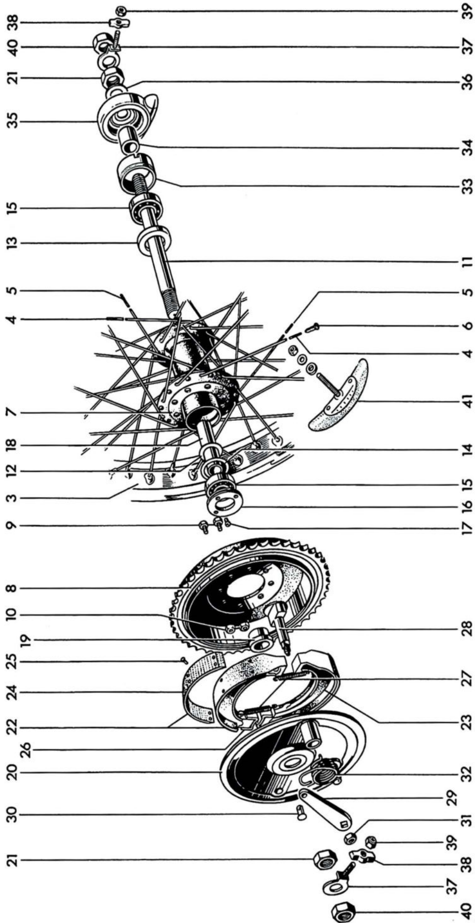
Fig. 18. REAR WHEEL
