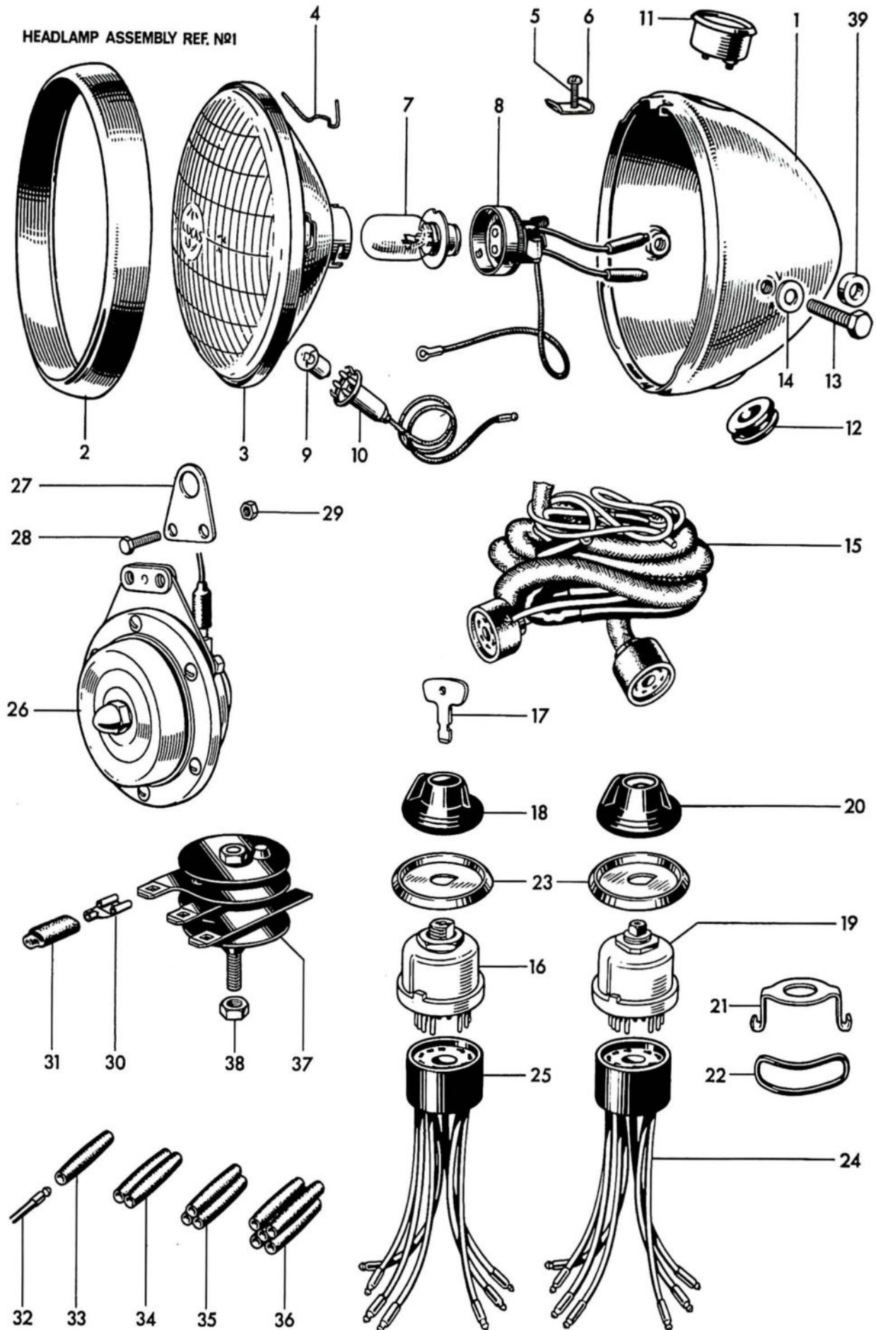
Fig. 29. T90 AND T100SS HEADLAMP, WIRING HARNESS AND SWITCHES
