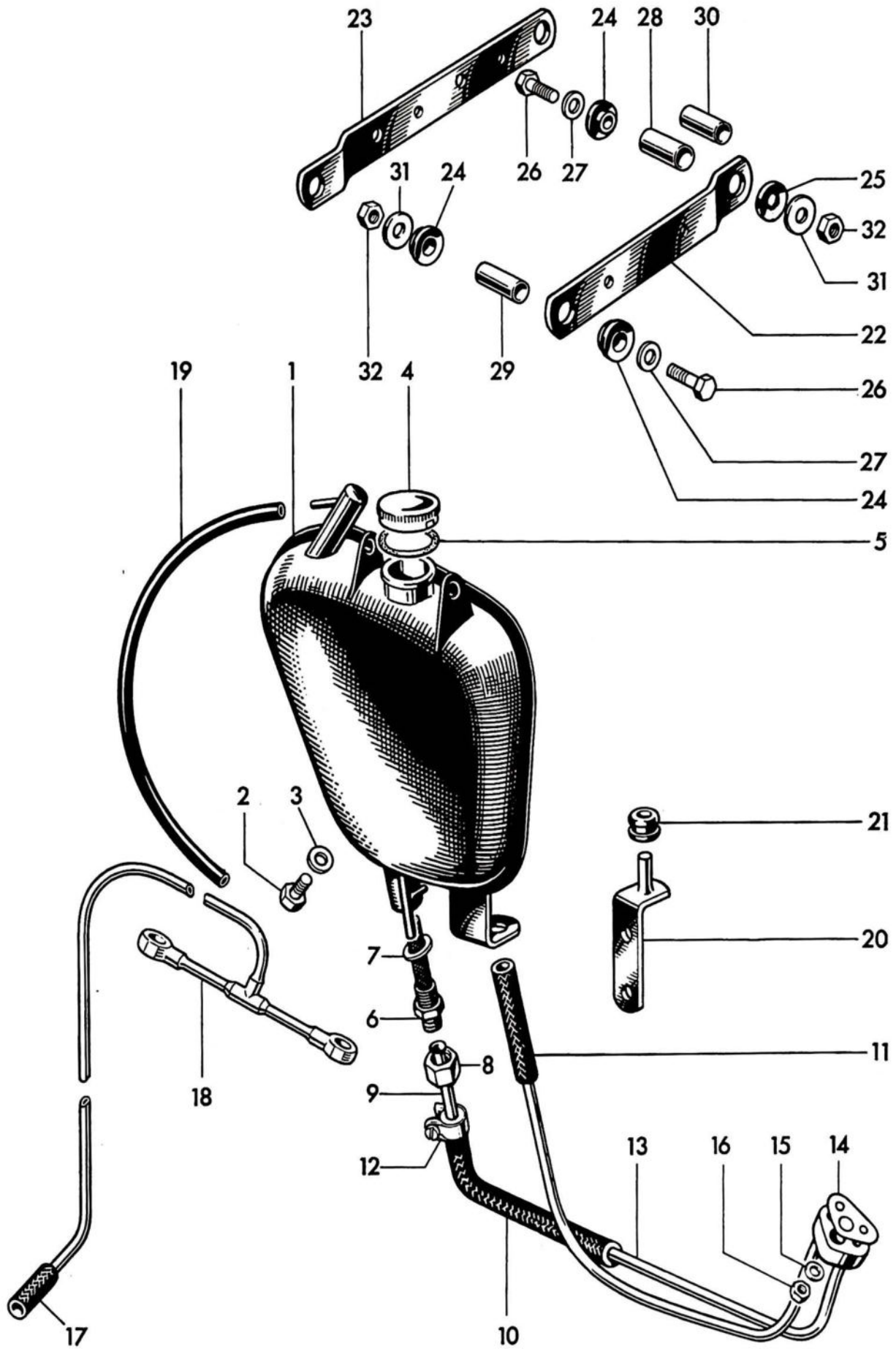
Fig. 23. OIL TANK
