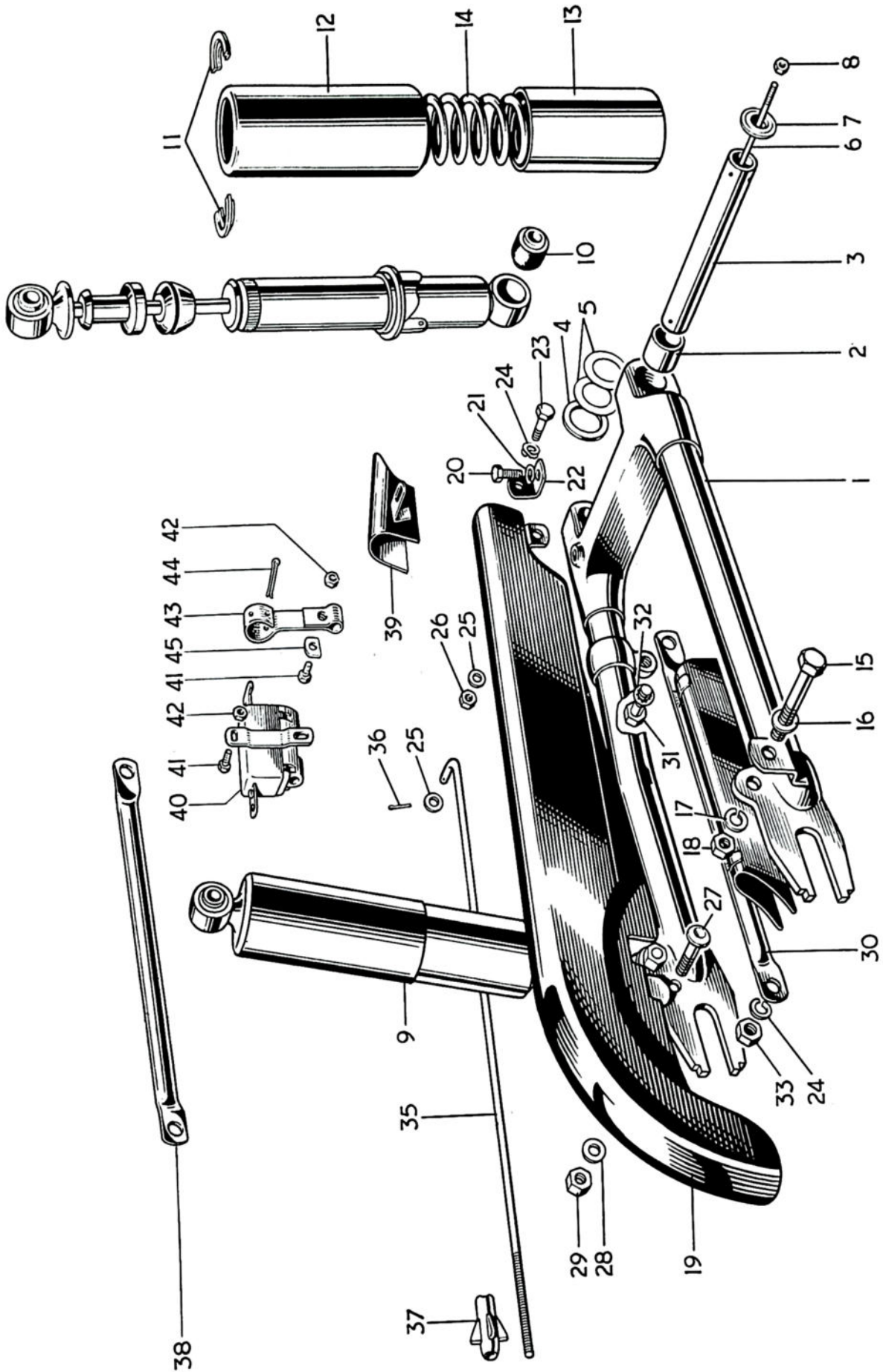
Fig. 13. SWINGING FORK, SUSPENSION UNITS AND CHAINGUARD
