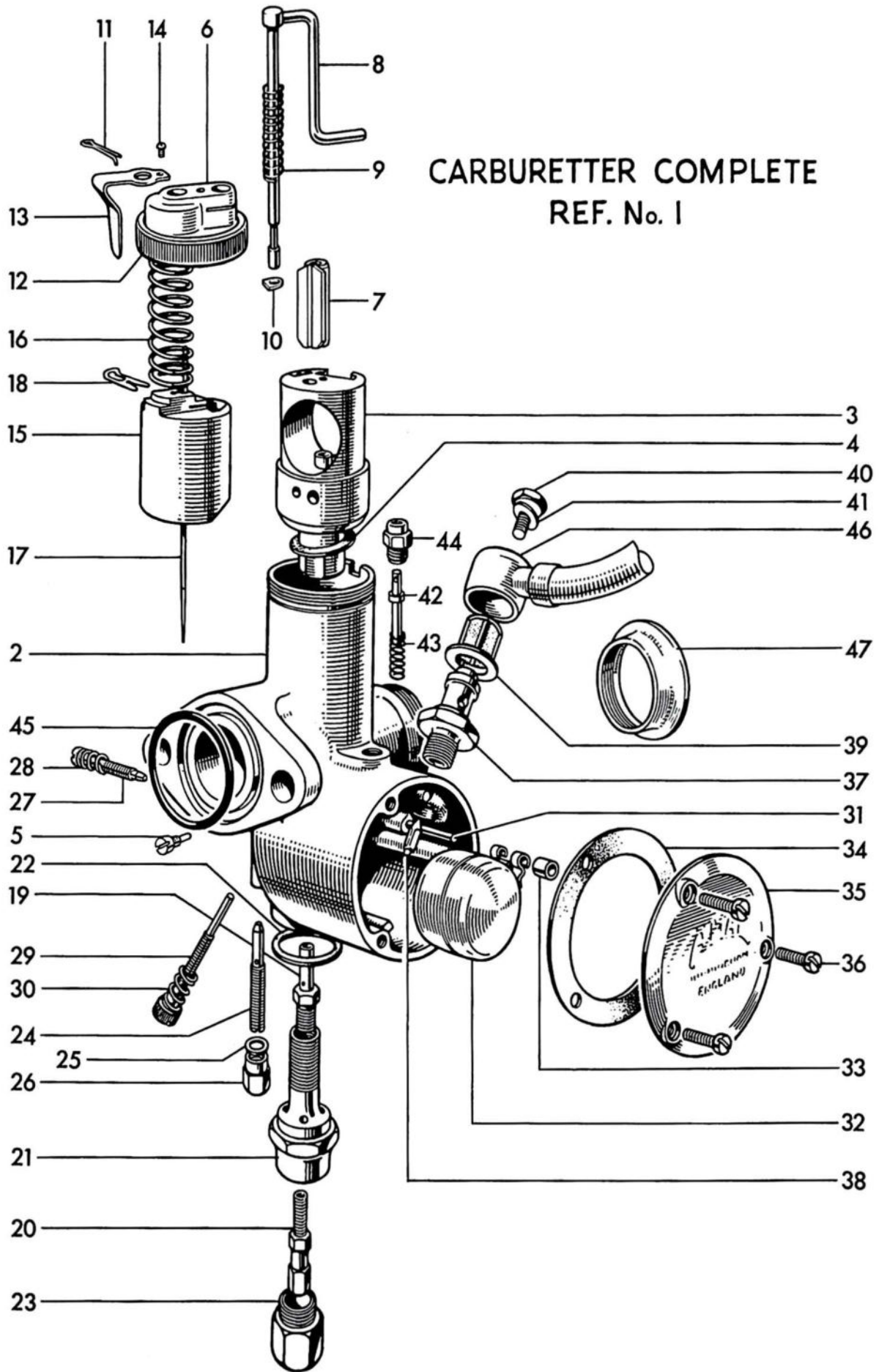
Fig. 28. CARBURETTER, T90 AND T100SS
