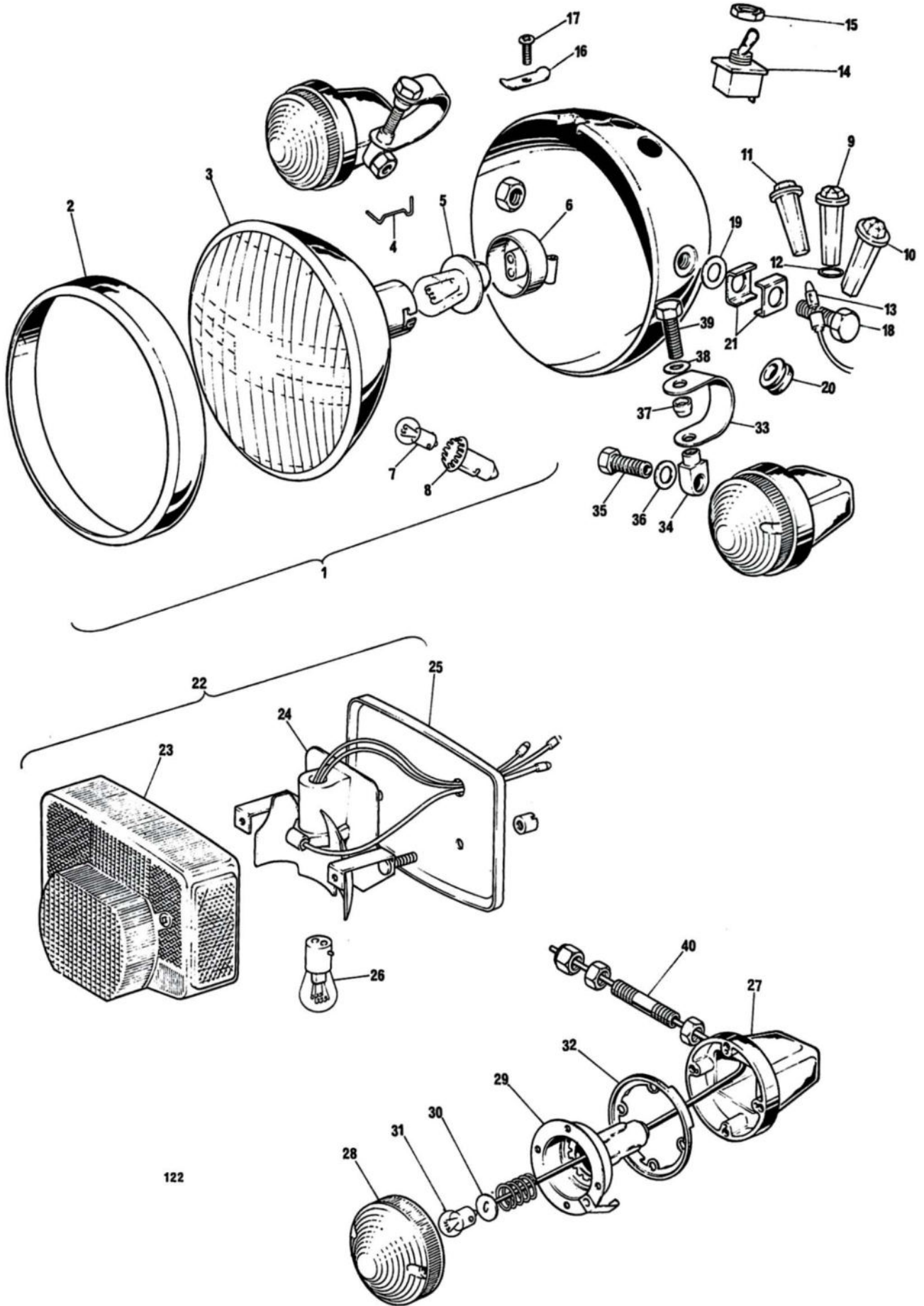
Fig. 23. HEADLAMP, TAIL LAMP AND FLASHERS
