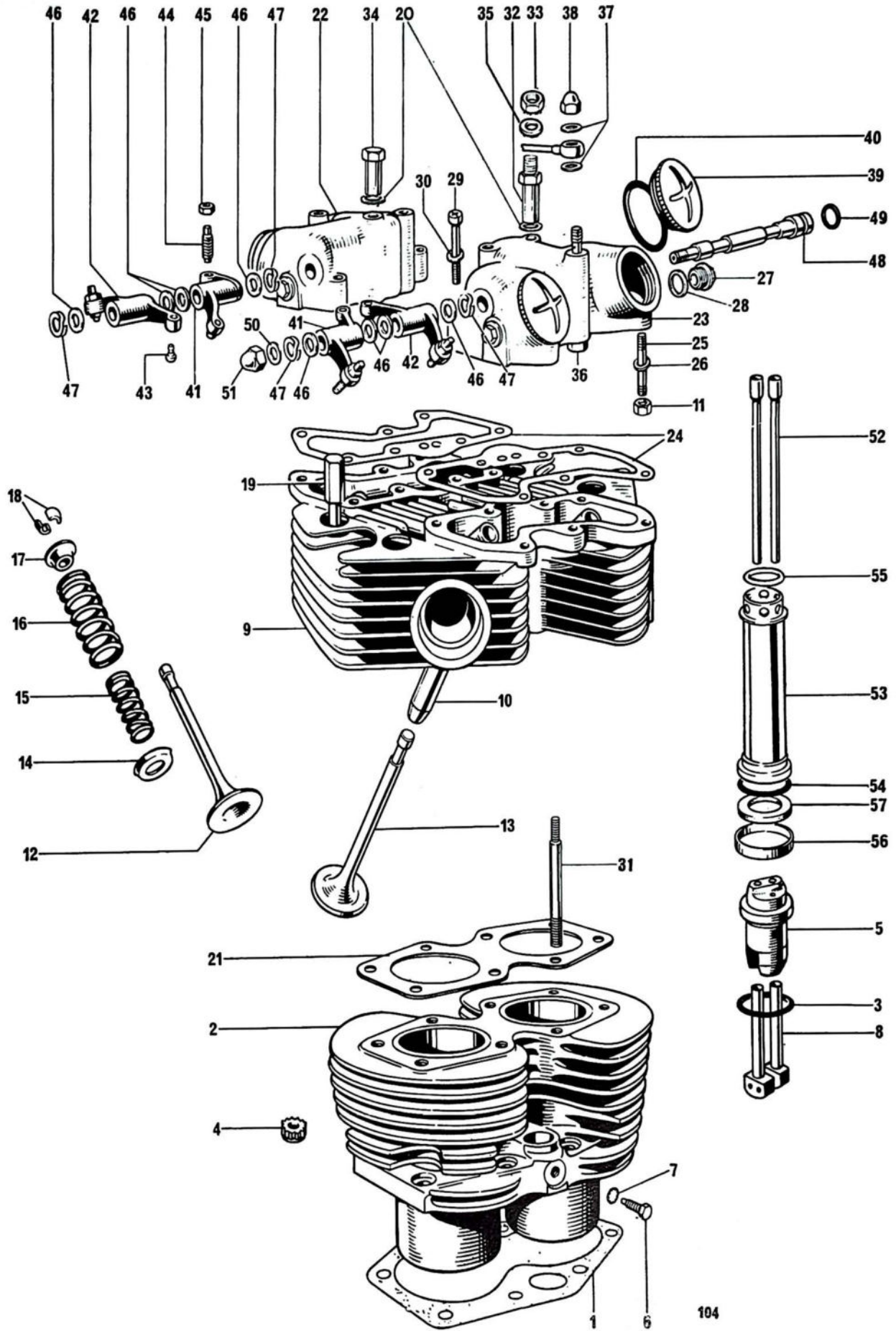
Fig. 5. CYLINDER BLOCK AND HEAD
