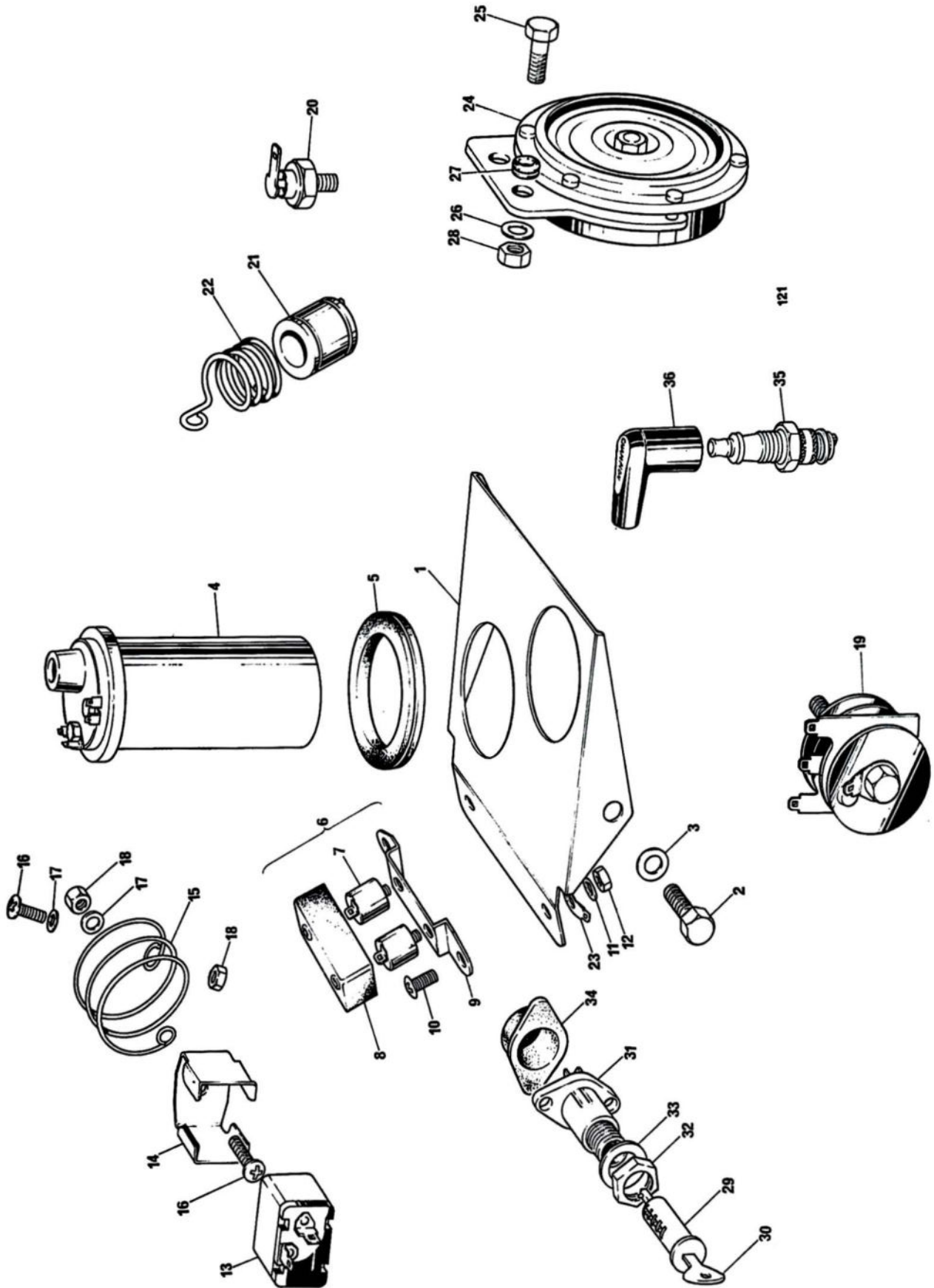
Fig. 22. ELECTRICAL COMPONENTS
