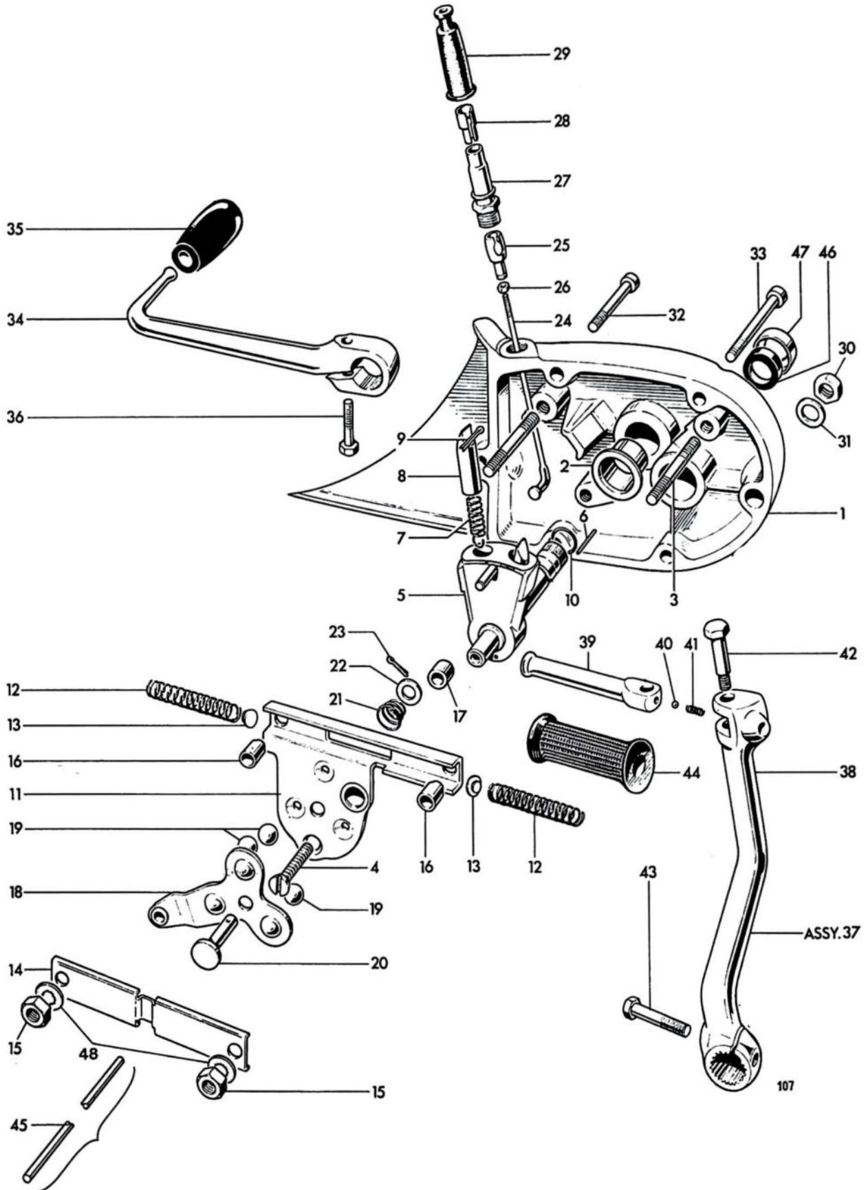
Fig. 8. GEARBOX OUTER COVER AND LEVERS
