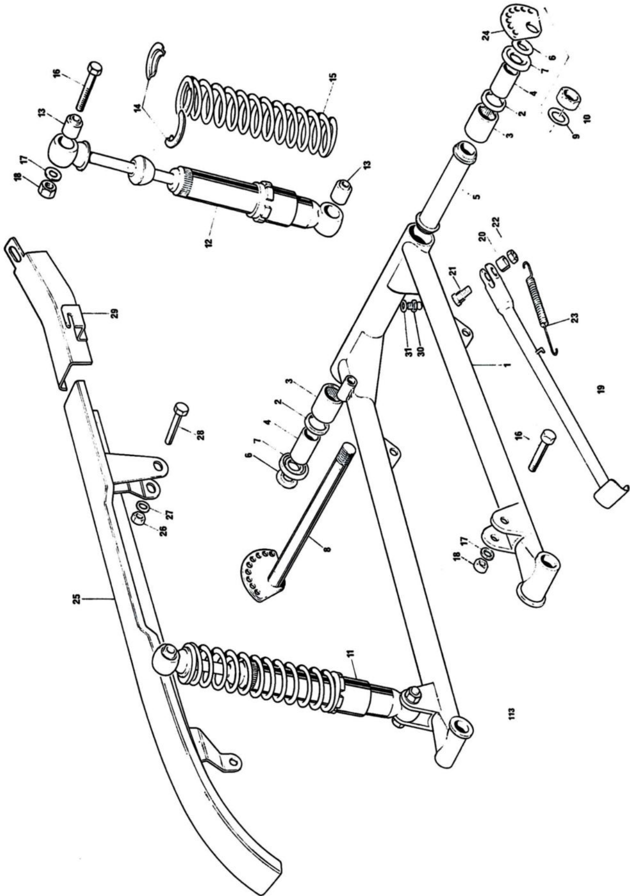
FIG. 14.] SWINGING ARM AND SUSPENSION UNITS
