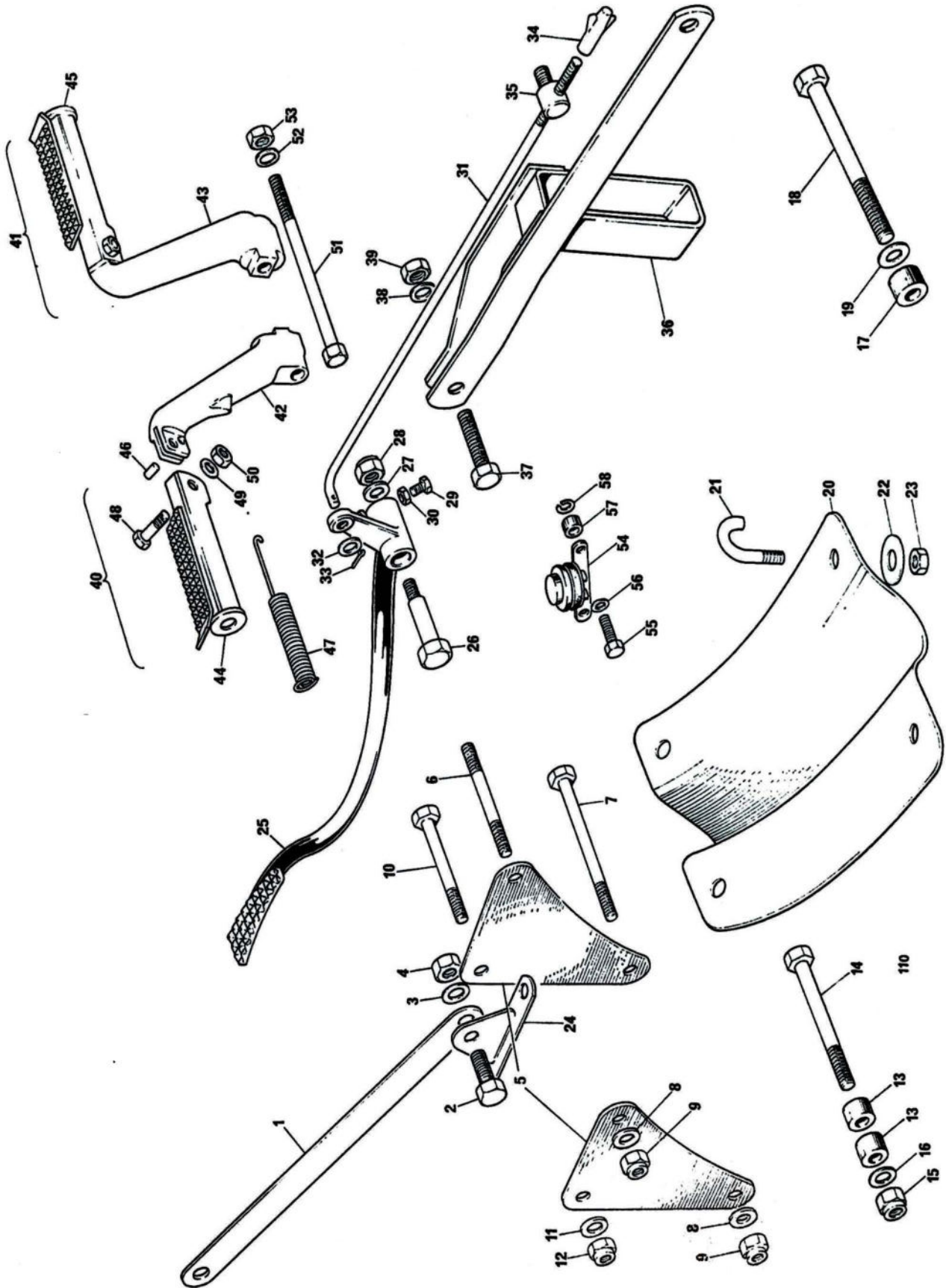
Fig. 11. MOTOR FIXINGS, BRAKE PEDAL AND FOOTRESTS
