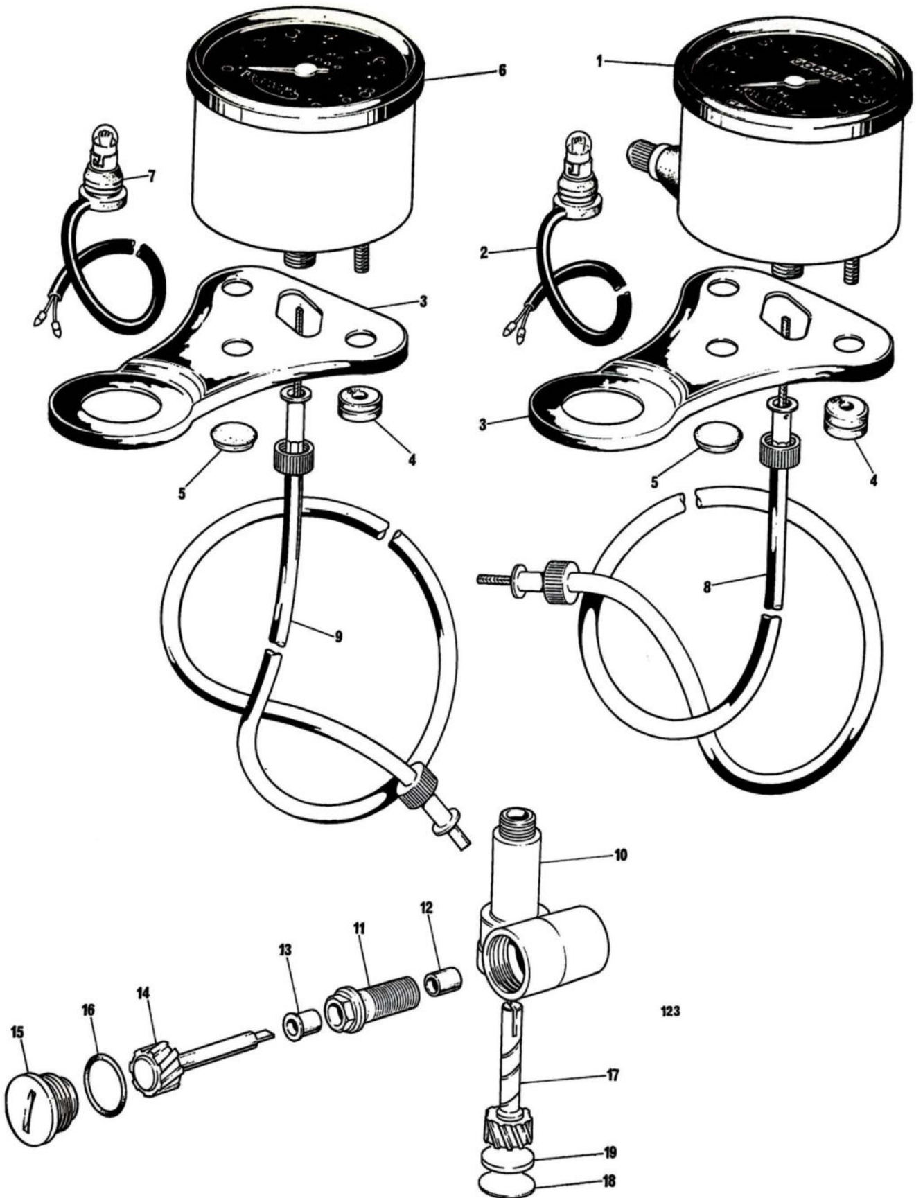
Fig. 24. SPEEDOMETER AND TACHOMETER
