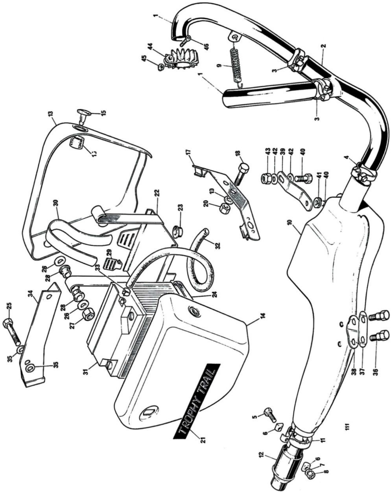
FIG. 12. EXHAUST SYSTEM, SIDE COVERS AND BATTERY
