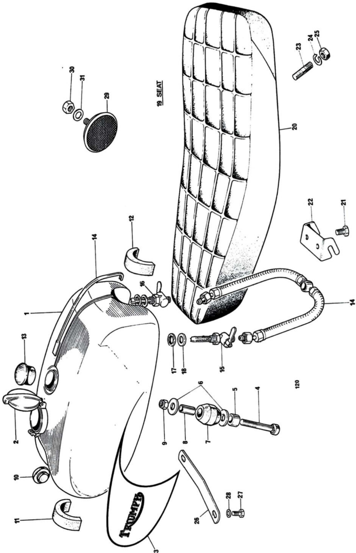
FIG. 21. GAS_TANK AND SEAT
