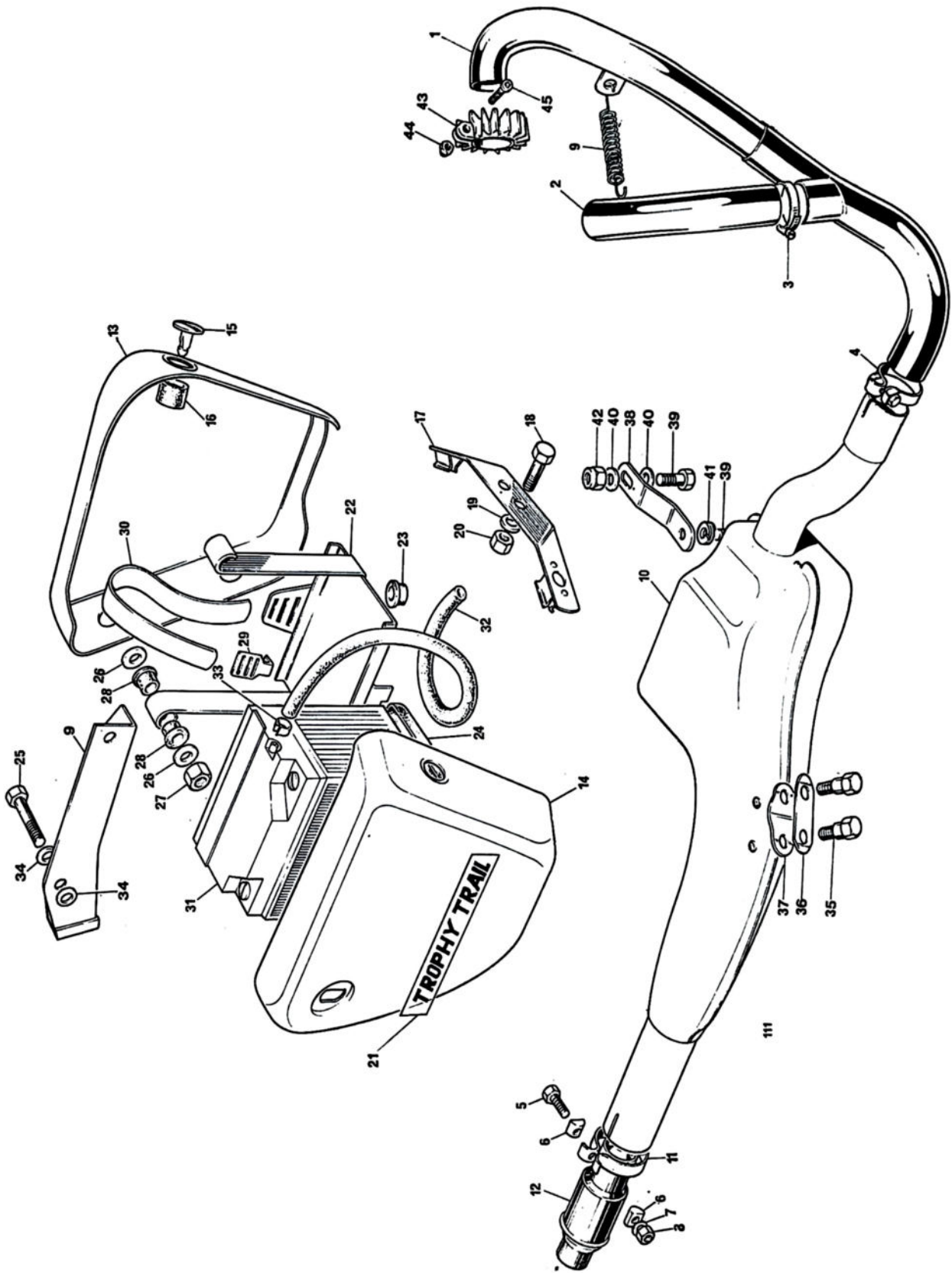
Fig. 13. EXHAUST SYSTEM, SIDE COVERS AND BATTERY
