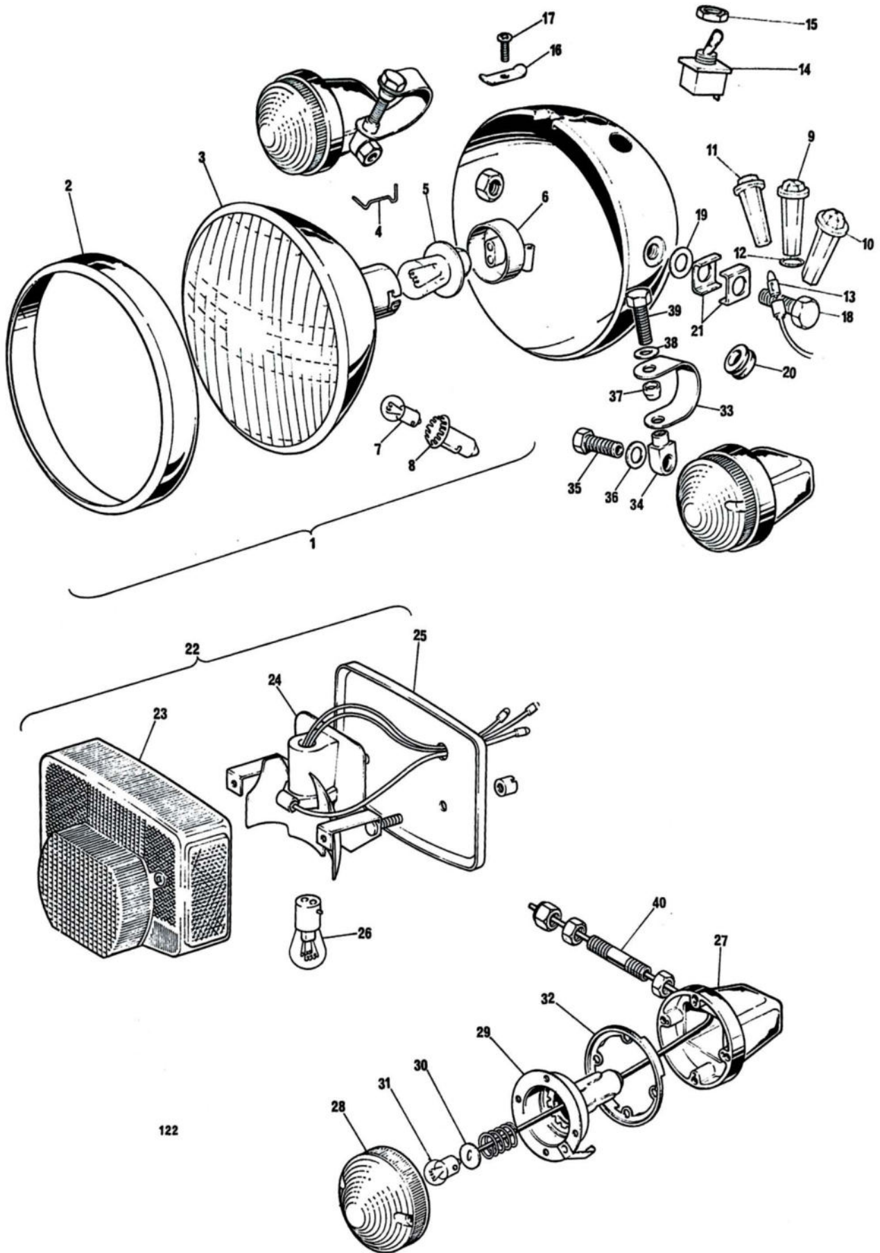
Fig. 24. HEADLAMP, TAIL LAMP AND FLASHERS
