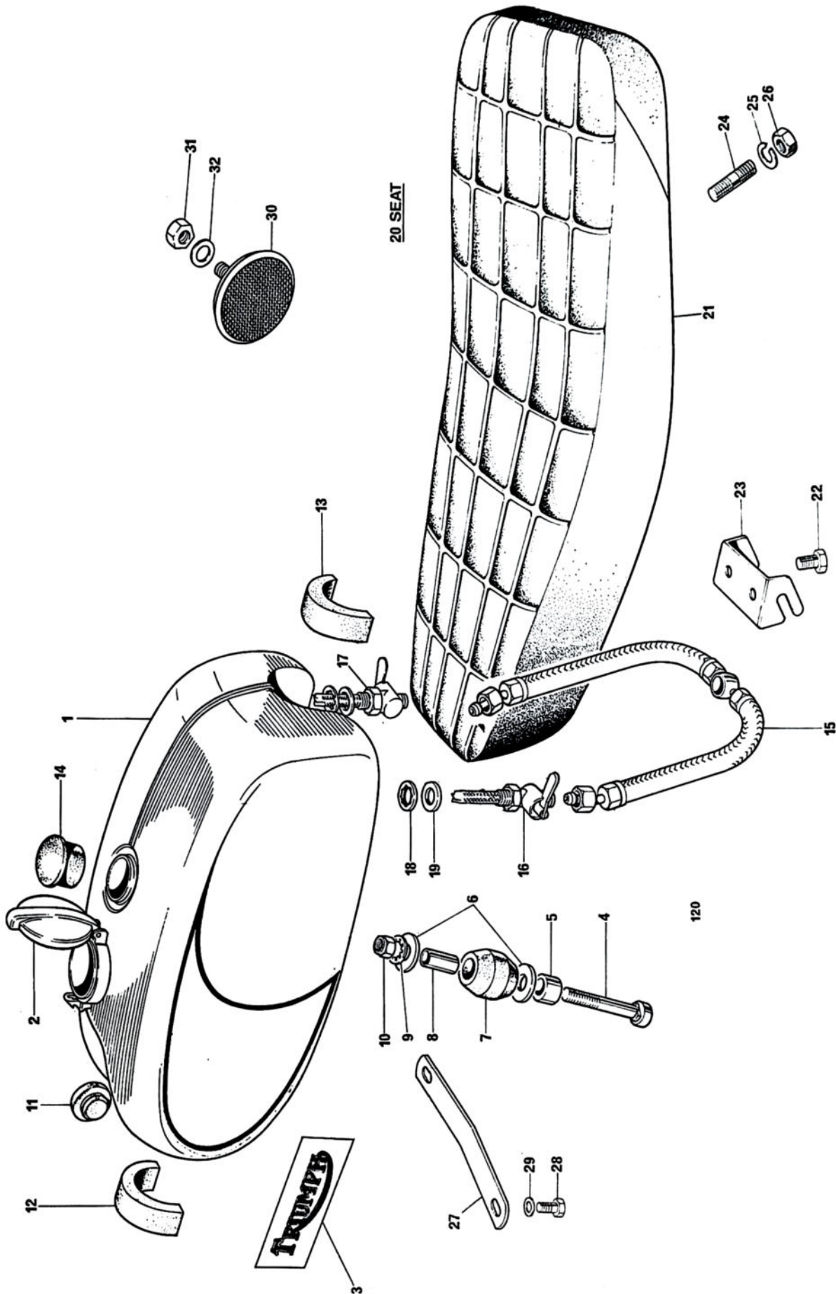
FIG. 22. GAS TANK AND SEAT
