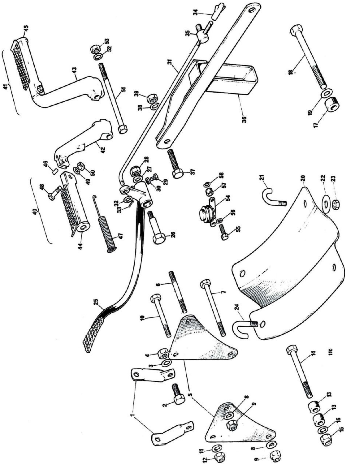
FIG. 12. MOTOR FIXINGS, BRAKE PEDAL AND FOOTRESTS
