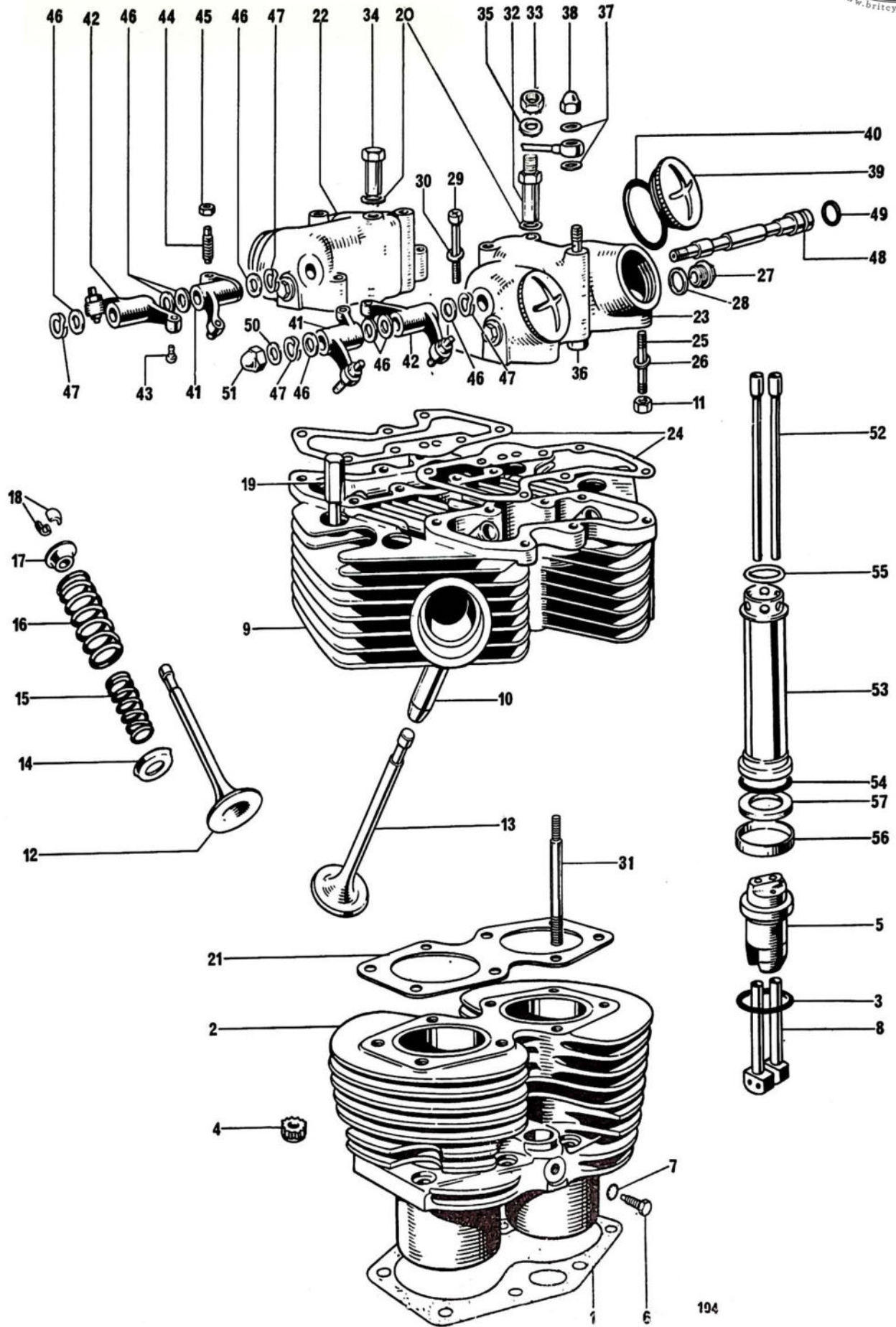
Fig. 6. CYLINDER BLOCK AND HEAD
