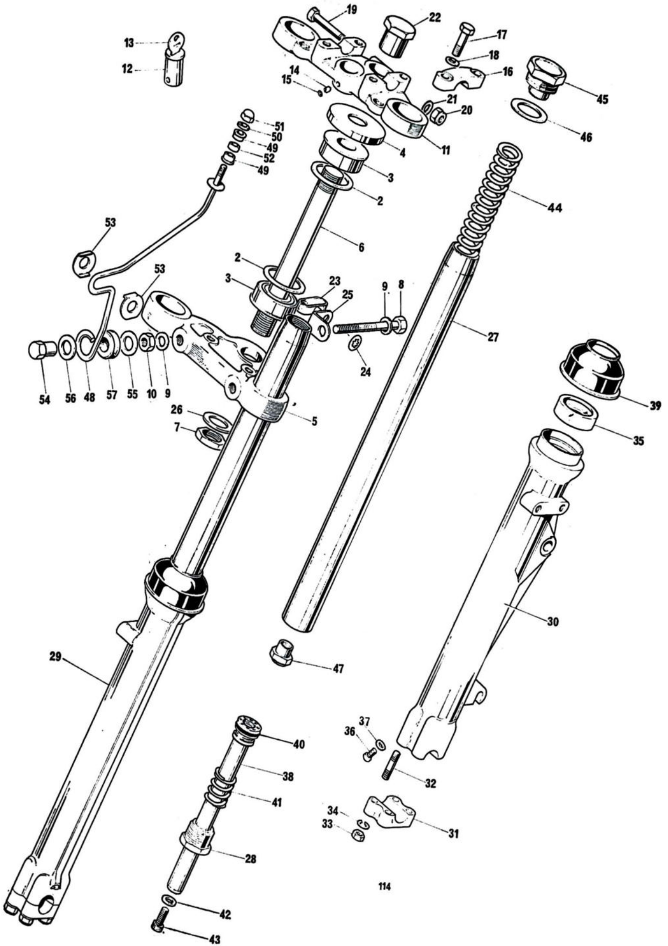
Fig. 16. TELESCOPIC FRONT FORK
