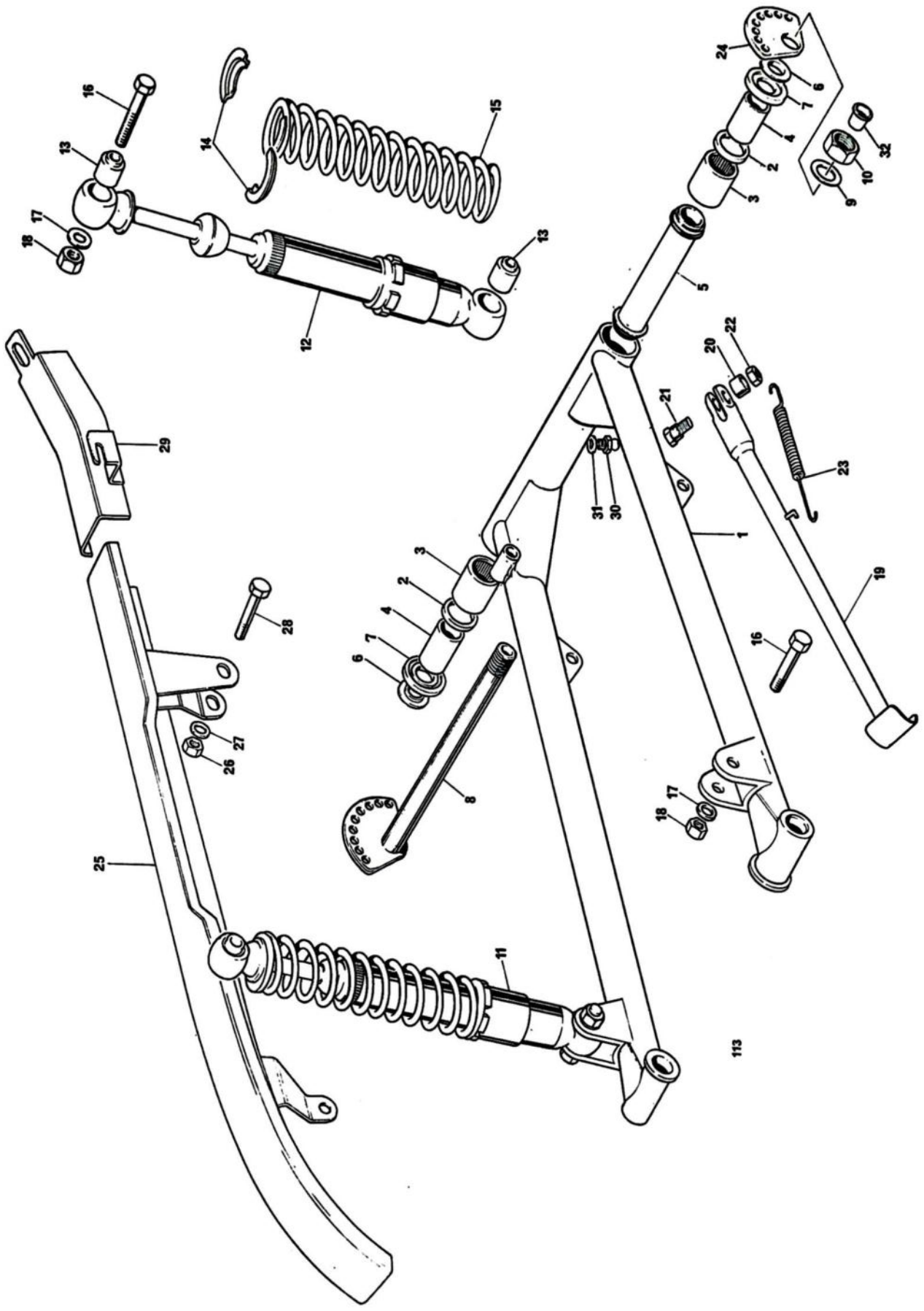
Fig. 15. SWINGING ARM AND SUSPENSION UNITS
