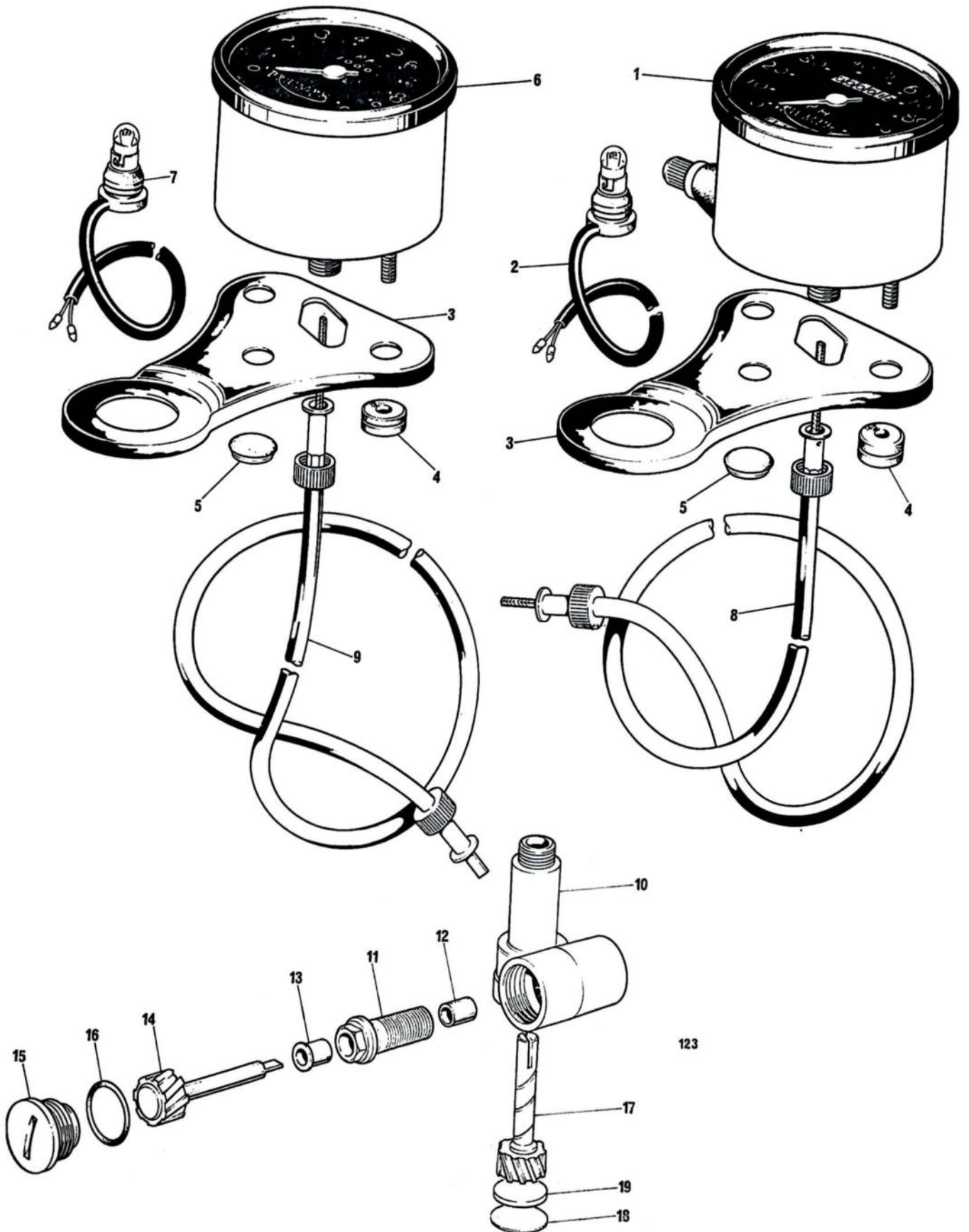
Fig. 25. SPEEDOMETER AND TACHOMETER
