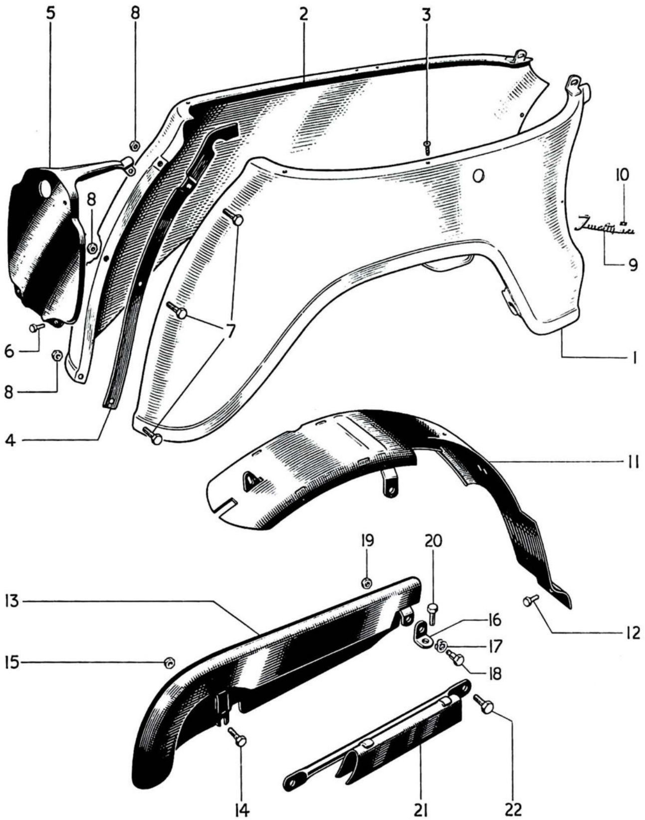
FIG. 13 REAR MUDGUARD, CHAINGUARD AND PANELS
