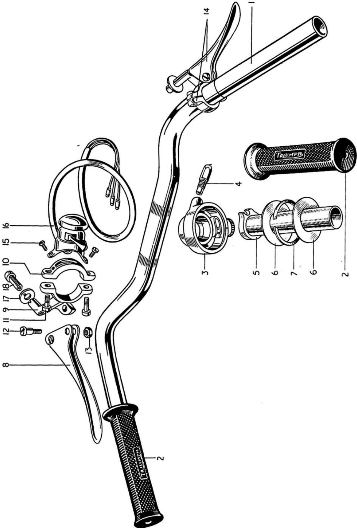
FIG. 17 HANDLEBAR AND CONTROLS
