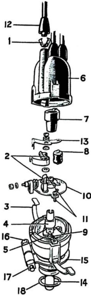
FIG. 19 LUCAS DISTRIBUTOR TYPE 18D2
