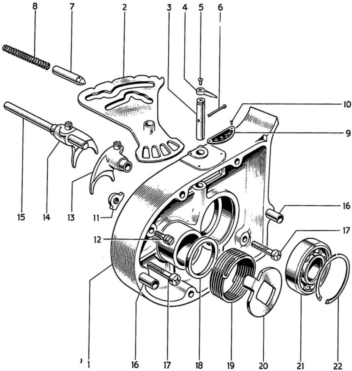
FIG. 6 GEARBOX INNER COVER
