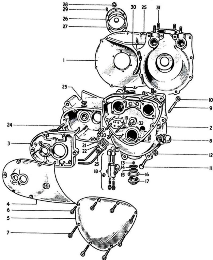
FIG. 4 CRANKCASE AND COVERS
