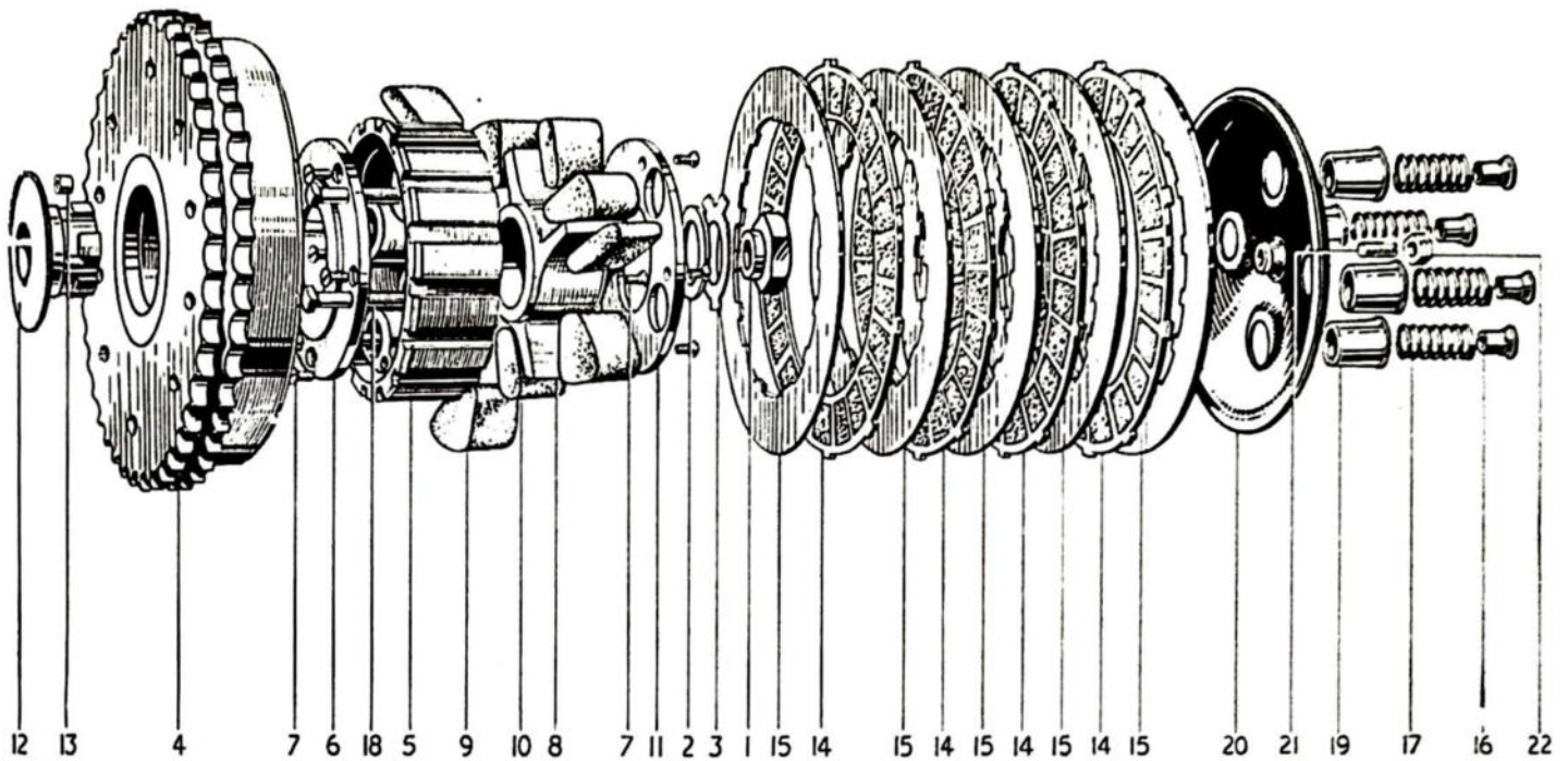
FIG. 8 CLUTCH AND SHOCK ABSORBER
