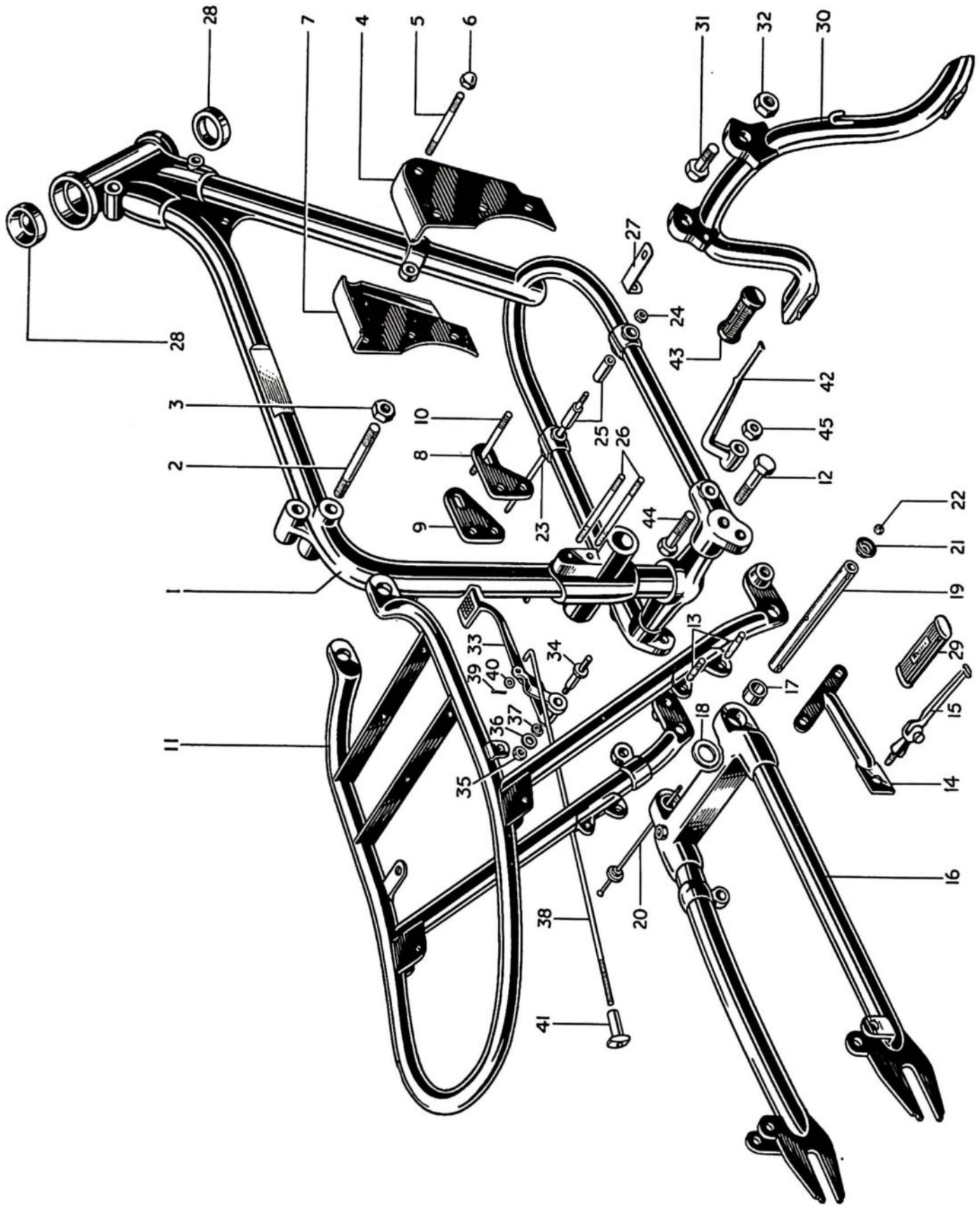
FIG. 9 FRAME AND FITTINGS
