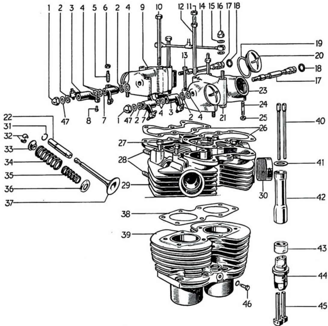
FIG. 2 CYLINDER BLOCK AND HEAD INDEX TO FIG. 2
