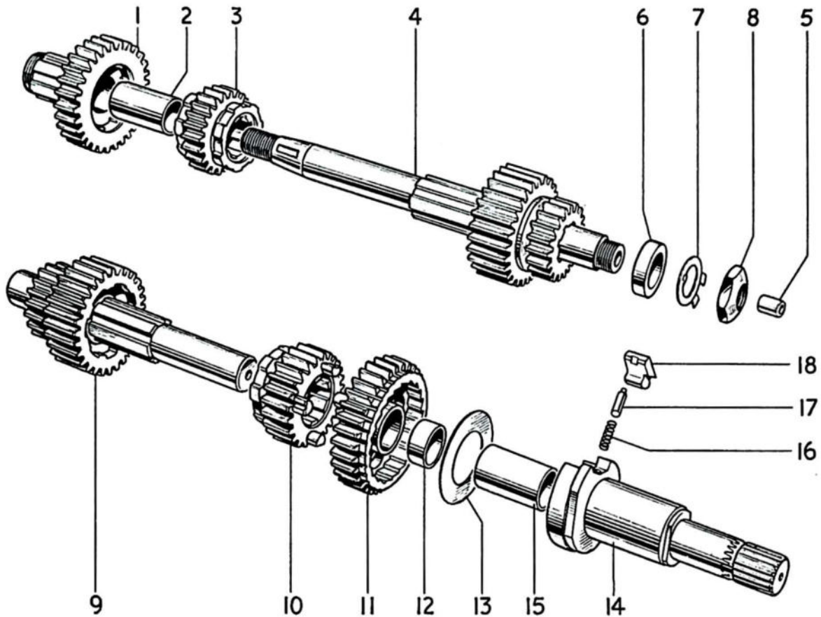
FIG. 5 SHAFTS AND GEARS
