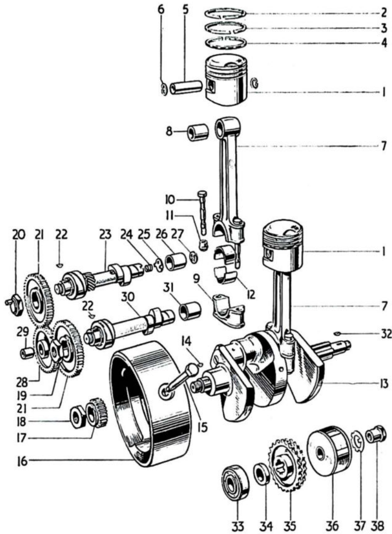
FIG. 3 CRANKSHAFT AND CONNECTING RODS INDEX TO FIG. 3
