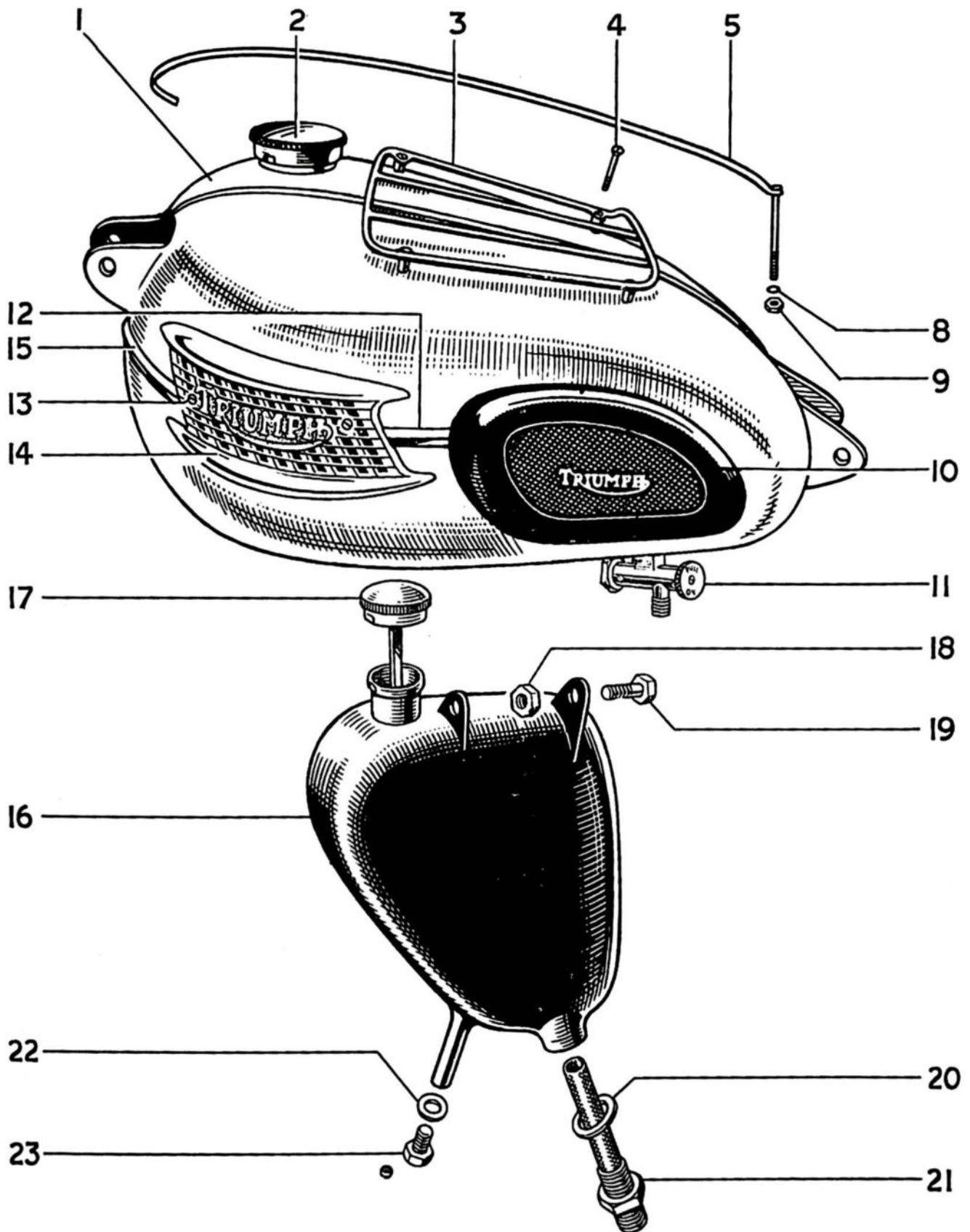
FIG. 14 PETROL AND OIL TANKS
