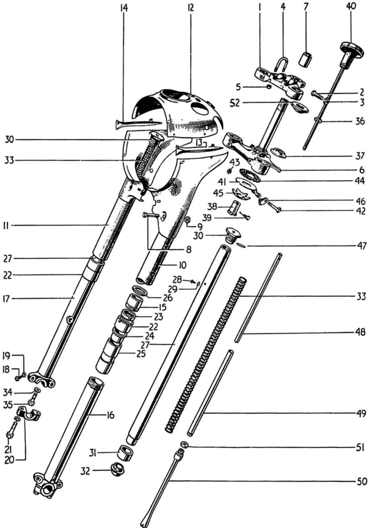
FIG. 10 TELESCOPIC FRONT FORK
