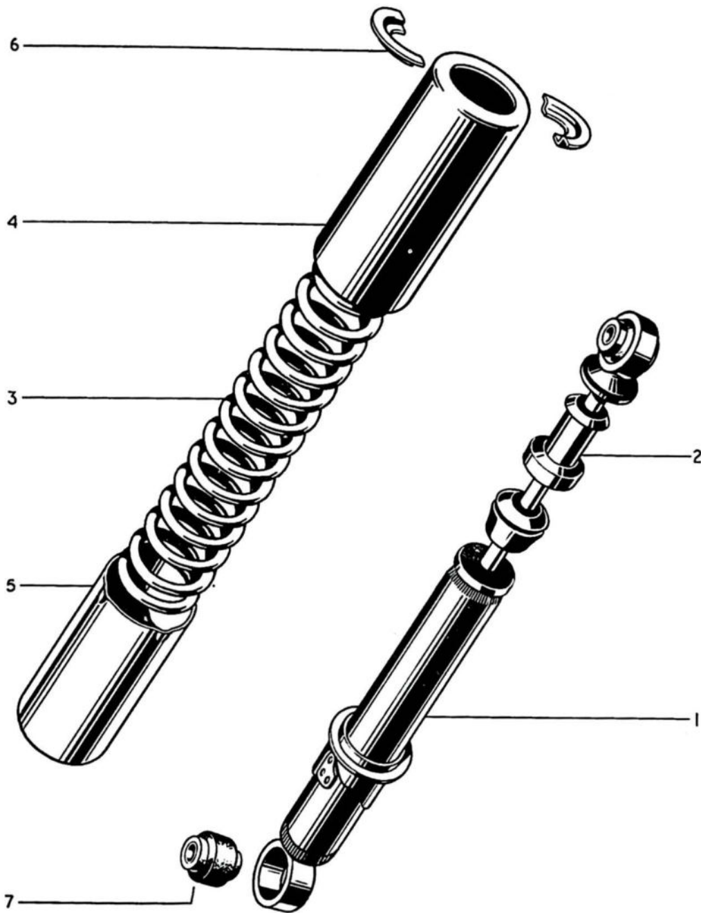
FIG. 21 GIRLING SUSPENSION UNIT
